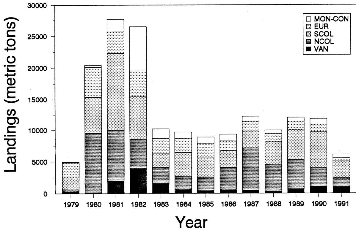
Figure 1. Landings (mt) of widow rockfish for the Vancouver (VAN), northern and southern Columbia (NCOL, SCOL), Eureka (EUR), and Monterey-Conception (MON-CON) INPFC areas from 1979 to 1991. Estimates for 1991 are preliminary.
