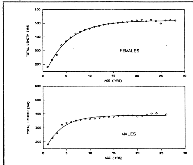
Figure 8. Fit of the growth curve
