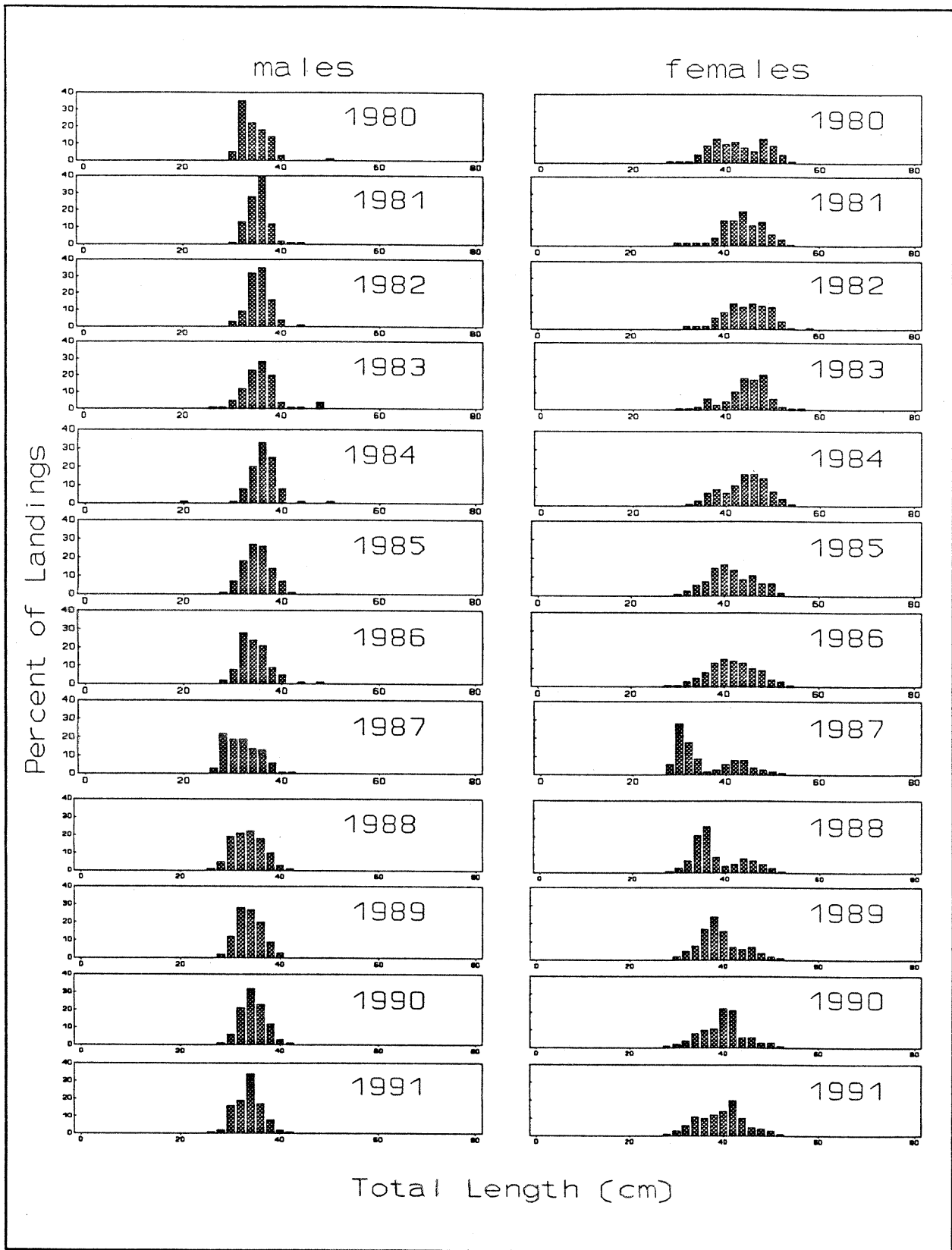
Figure 2. Length composition data for chilipepper based on samples from the California trawl fishery landings.
