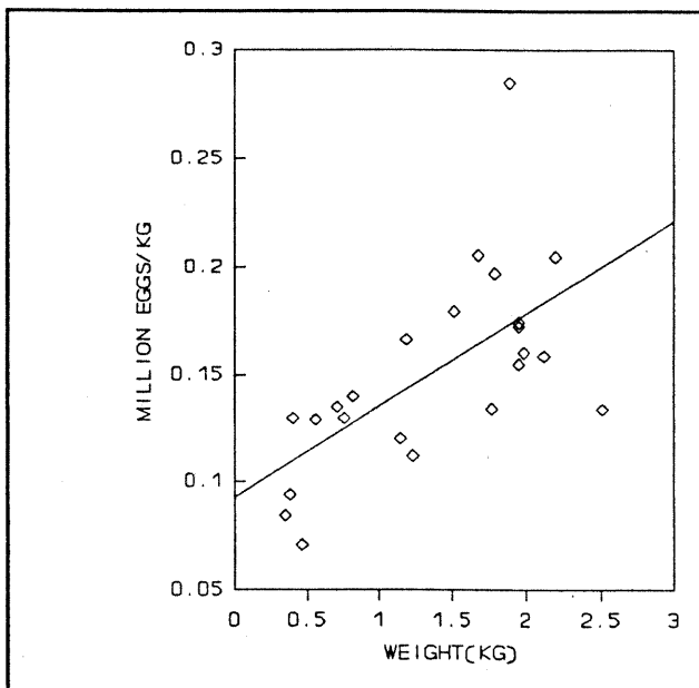
Figure 11. Fit to data from Phillips (1964).
