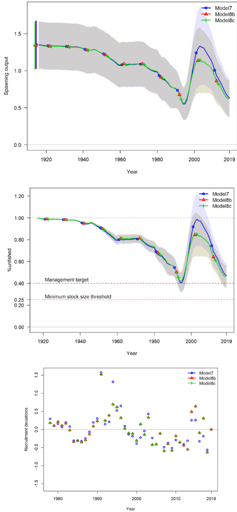
Figure 6. Results of request 7 and 8. Time series of absolute (top) and relative (middle) spawning output and recruitment deviations (now starting in 1978; bottom).
