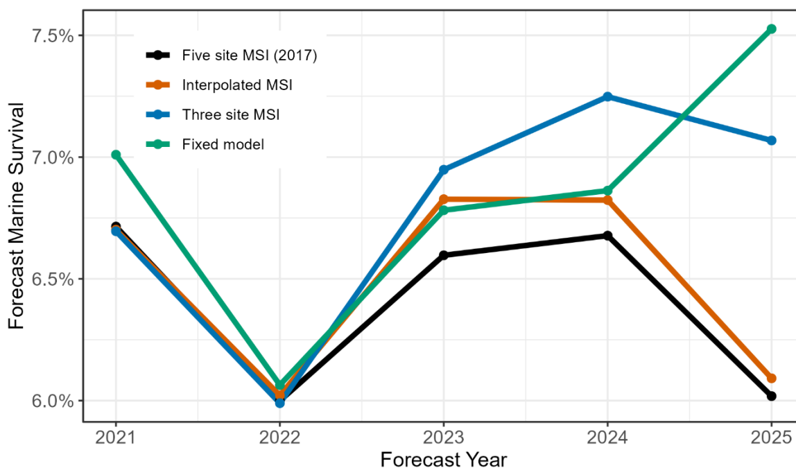
Figure 4. Marine survival forecast results from the two variable GAM ensembles fit to alternative marine survival indexes (MSI). The five site MSI has been the adopted MSI used for forecasts 2018-2025.
