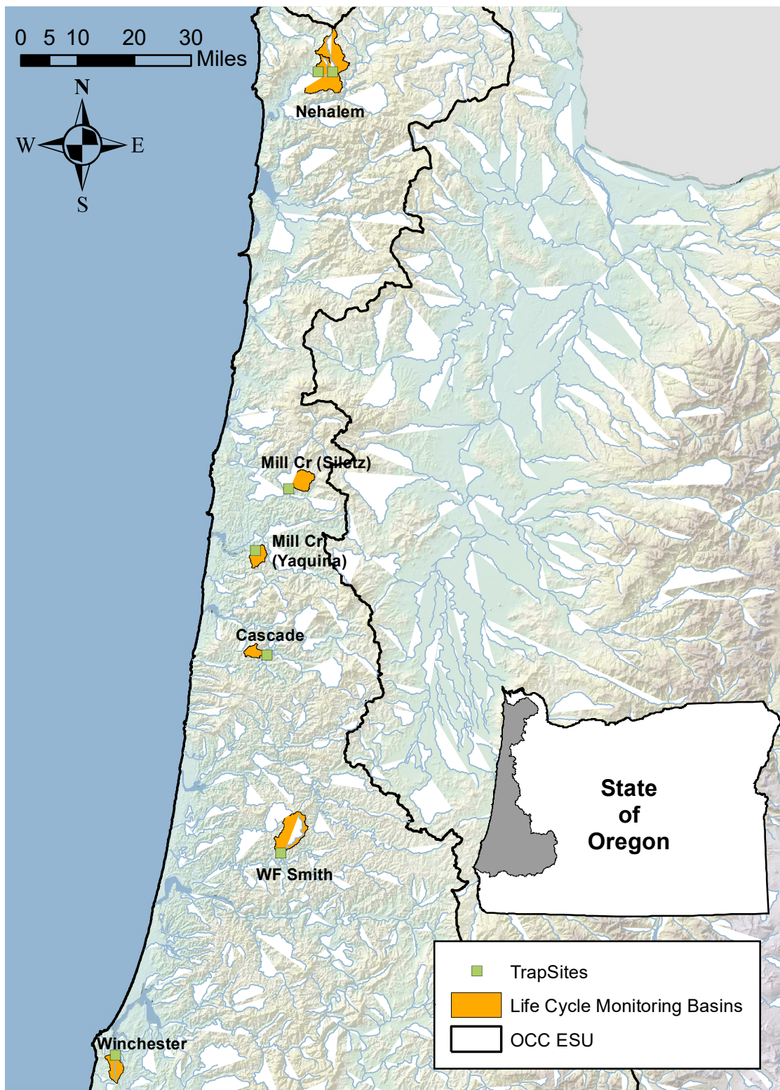
Figure 1. Oregon Department of Fish and Wildlife Life Cycle Monitoring Basins where both Coho Salmon adult returns and juvenile out-migrants are estimated. Monitoring began in 1998, ended at NF Nehalem in 2017, ended at WF Smith and Winchester in 2025, and continues at the three Mid Coast sites.
