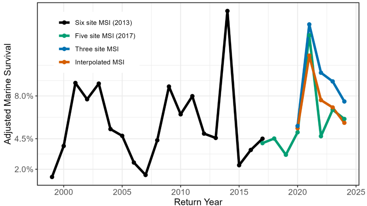
Figure 3. Alternative marine survival index (MSI) estimates using six sites (adopted 2013), five sites (adopted 2017), three sites, and interpolated (MARSS model). The y-axis labels show the matrix category breaks. The interpolated estimate is made with five years of data removed from the two sites discontinued in 2025 to simulate model performance with future missing data.
