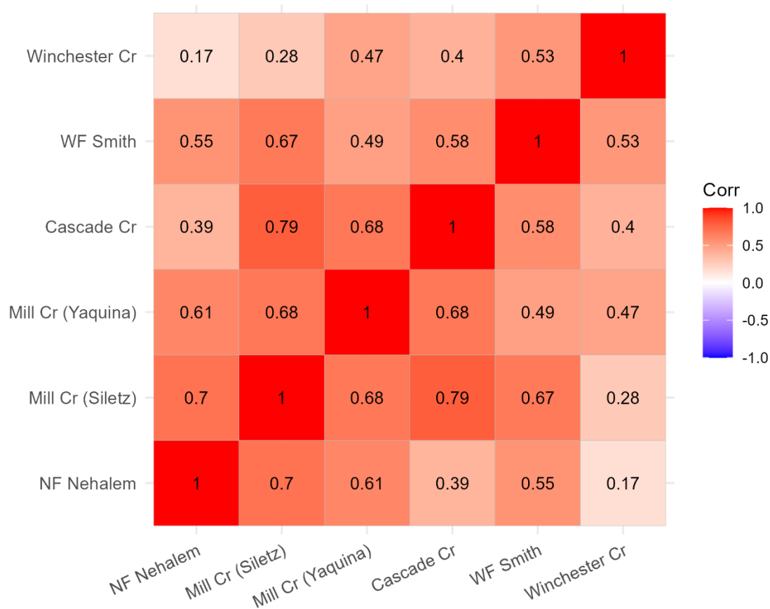
Figure 2. Correlation in marine survival estimates between LCM sites. Sites are ordered from north to south across the bottom. Only the Cascade Cr, Mill Cr (Yaquina), and Mill Cr (Siletz) sites will be operated from 2025 onward.
