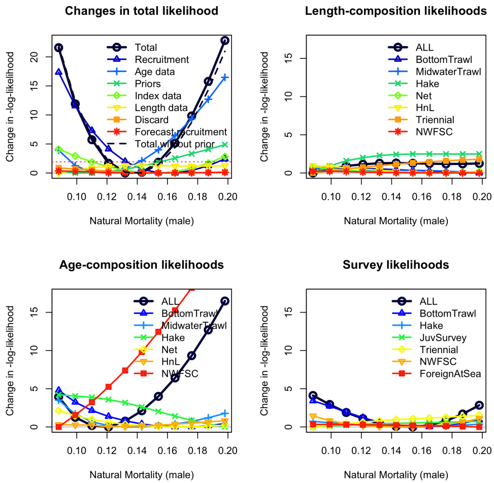
Figure 59: Likelihood components in the likelihood profile for male natural mortality (M). Female natural mortality is set to the same value.
