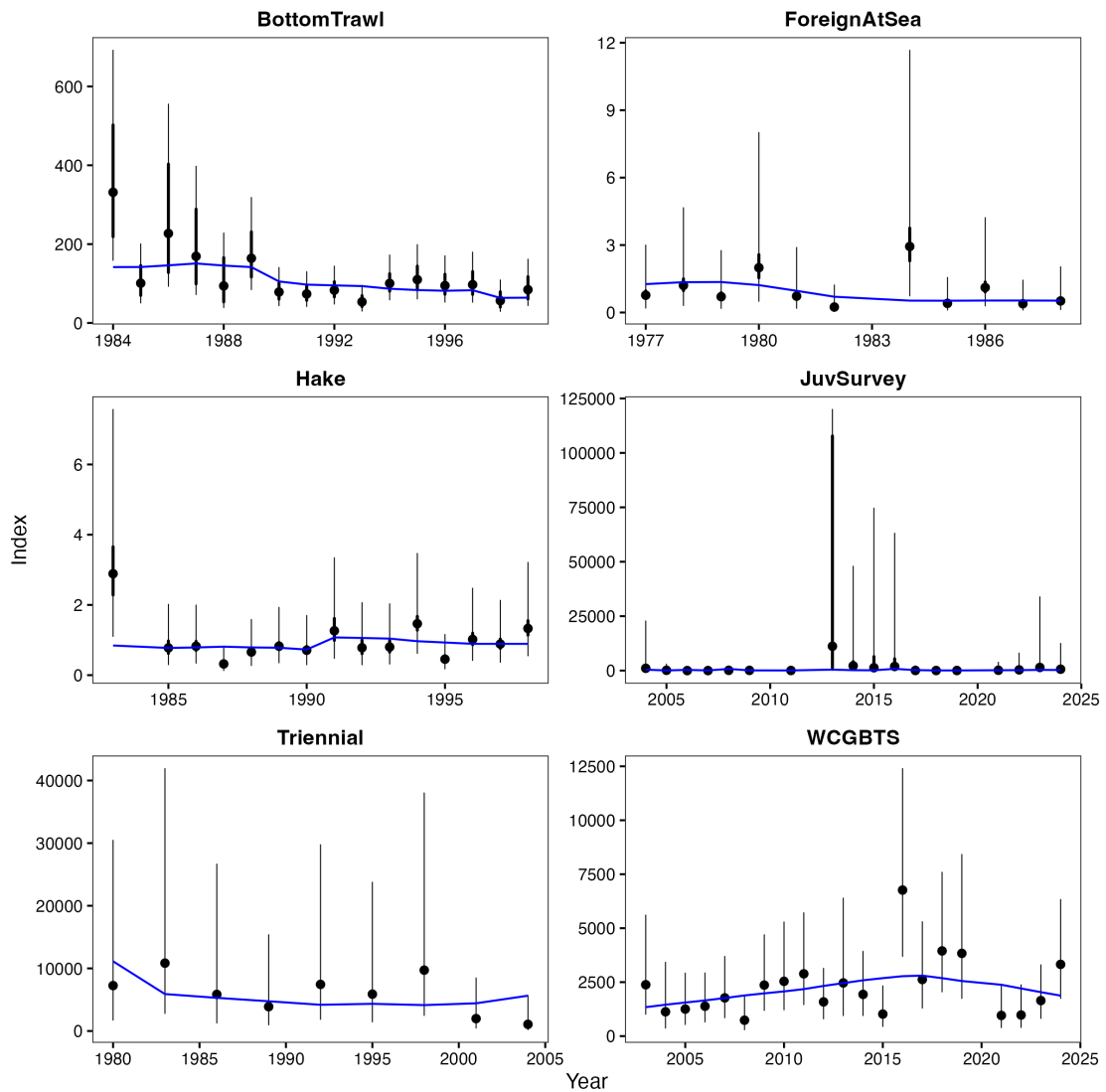
Figure 36: Fits (blue lines) to the abundance estimates (black points) for the base model. A separate q is estimated for the Hake series starting in 1991. Except the juvenile survey (counts) all indices are biomass-based. 95% confidence intervals are shown assuming a normal distribution of the log-estimates. Thicker lines (if present) indicate input uncertainty before addition of the estimated additional uncertainty parameter. The y-axis of the juvenile survey is truncated to highlight interannual variability in counts.
