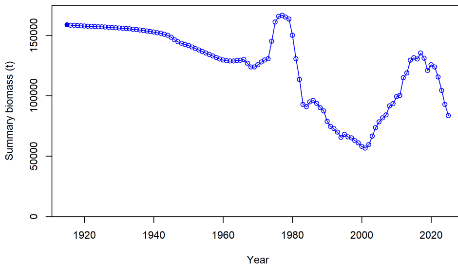
Figure 46: Predicted summary biomass (age 4+) from the base model.
