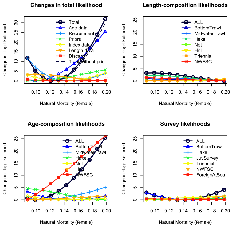
Figure 58: Likelihood components in the likelihood profile for female natural mortality (M). Male natural mortality are set to the same value.
