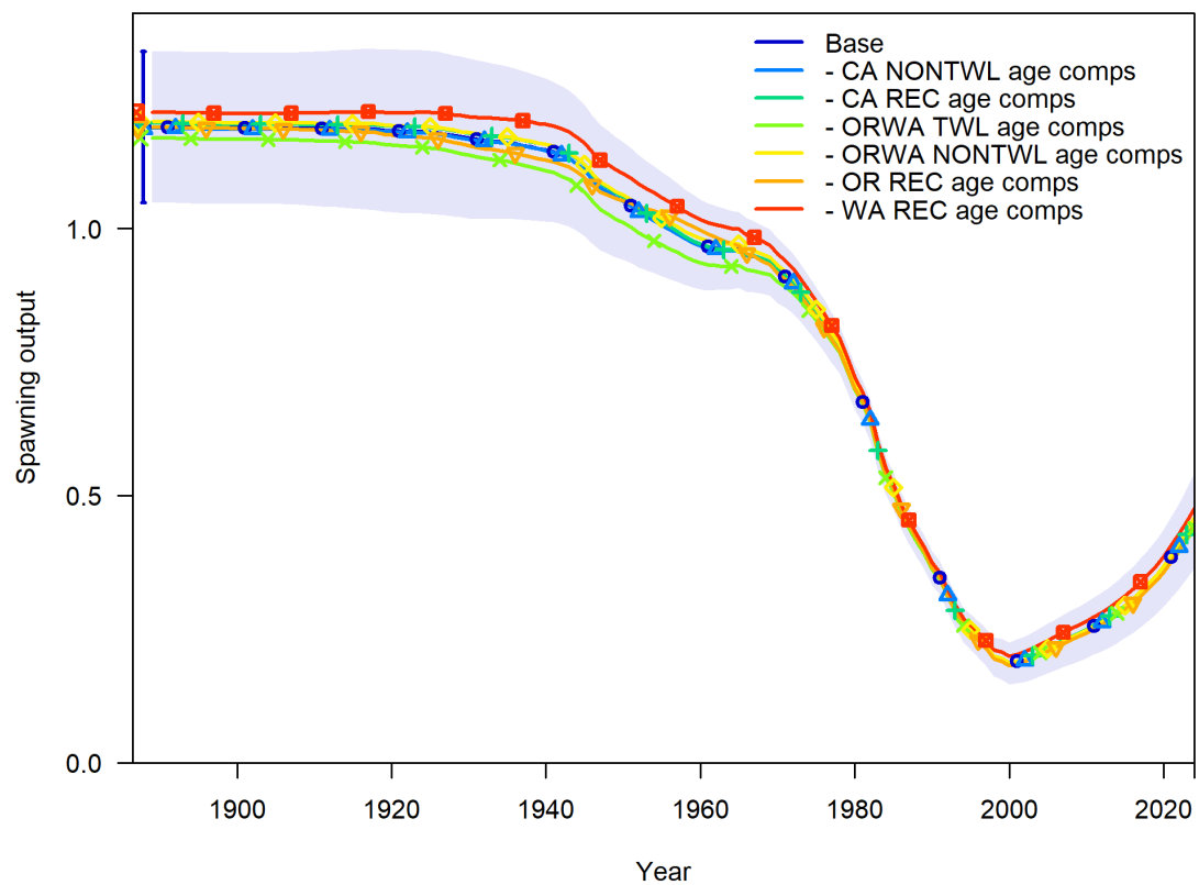
Figure 69: Spawning output (billions of eggs) across age composition inclusion sensitivities (1 of 2).
