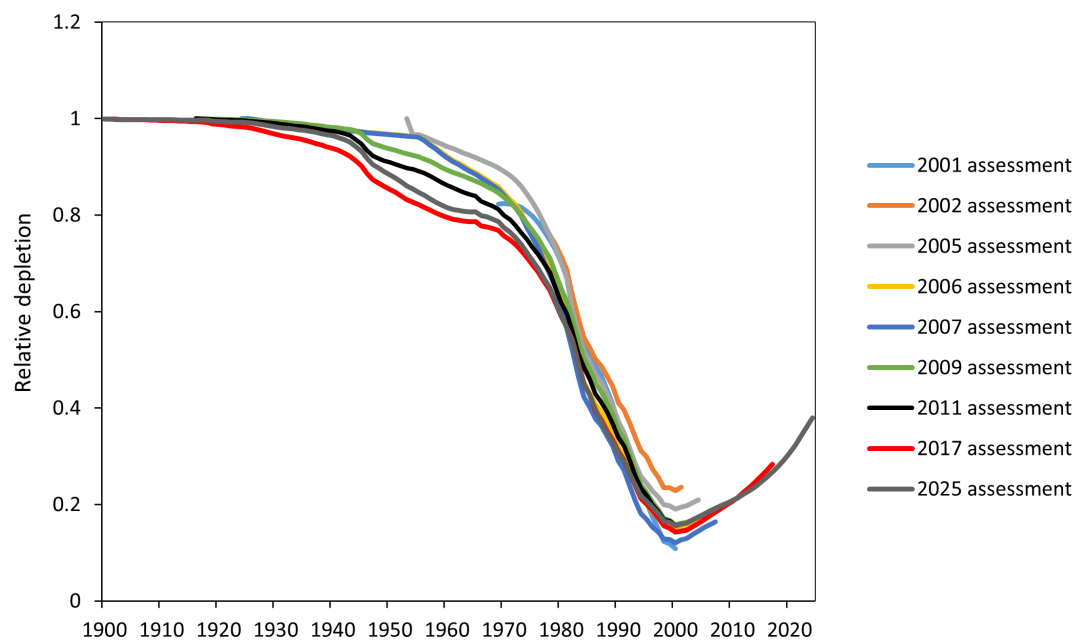
Figure 80: Relative depletion (spawning output) across Yelloweye Rockfish assessments over time.
