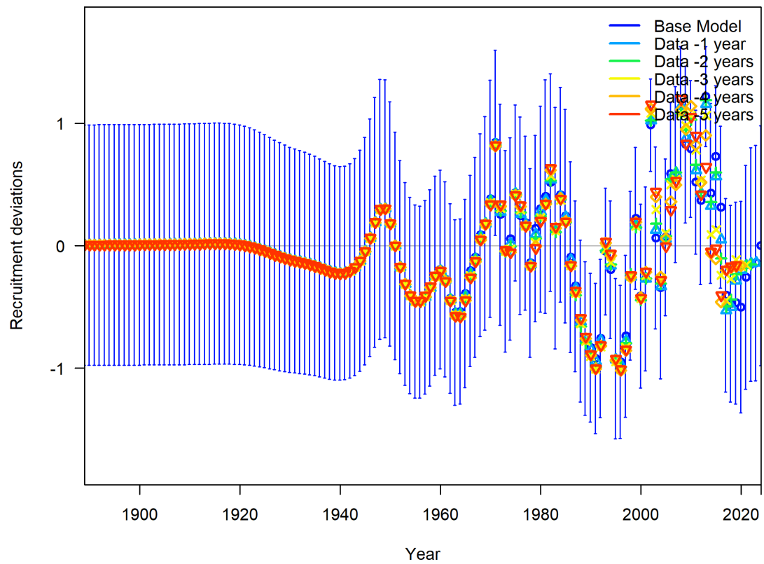
Figure 79: Recruitment deviation time series for each scenario of the retrospective analysis.
