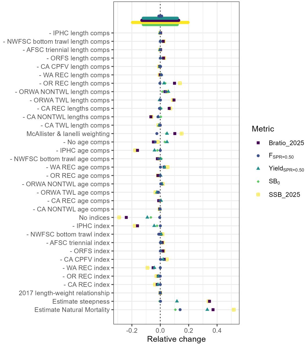
Figure 76: Relative change in management quantities across models conducted as sensitivities, without the removal of all length composition data.
