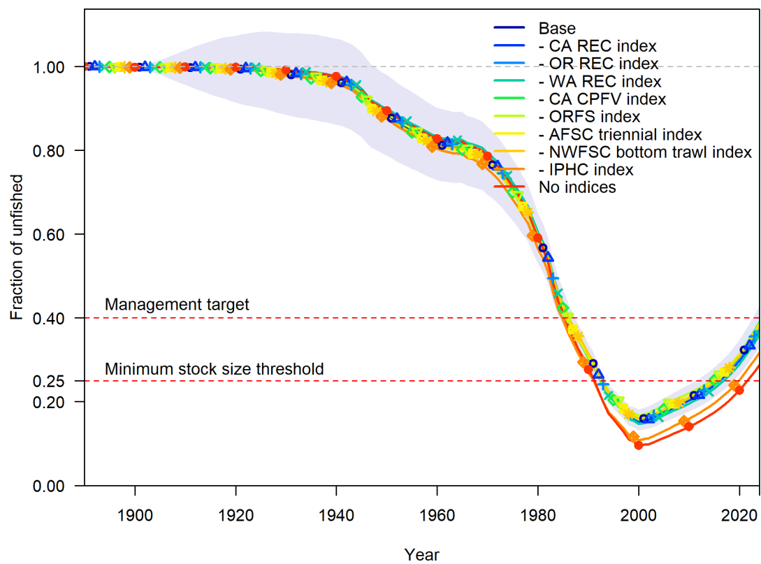
Figure 74: Relative spawning output across index inclusion sensitivities.
