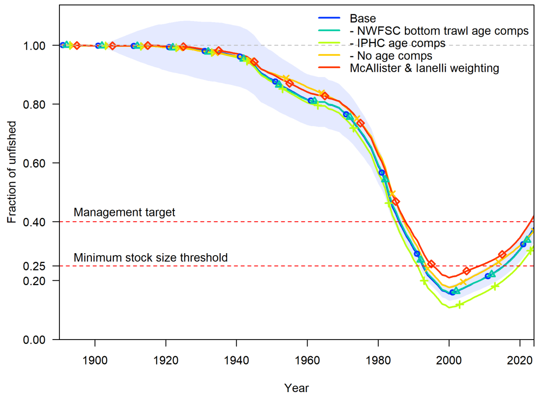
Figure 72: Relative spawning output across age composition inclusion sensitivities (2 of 2).
