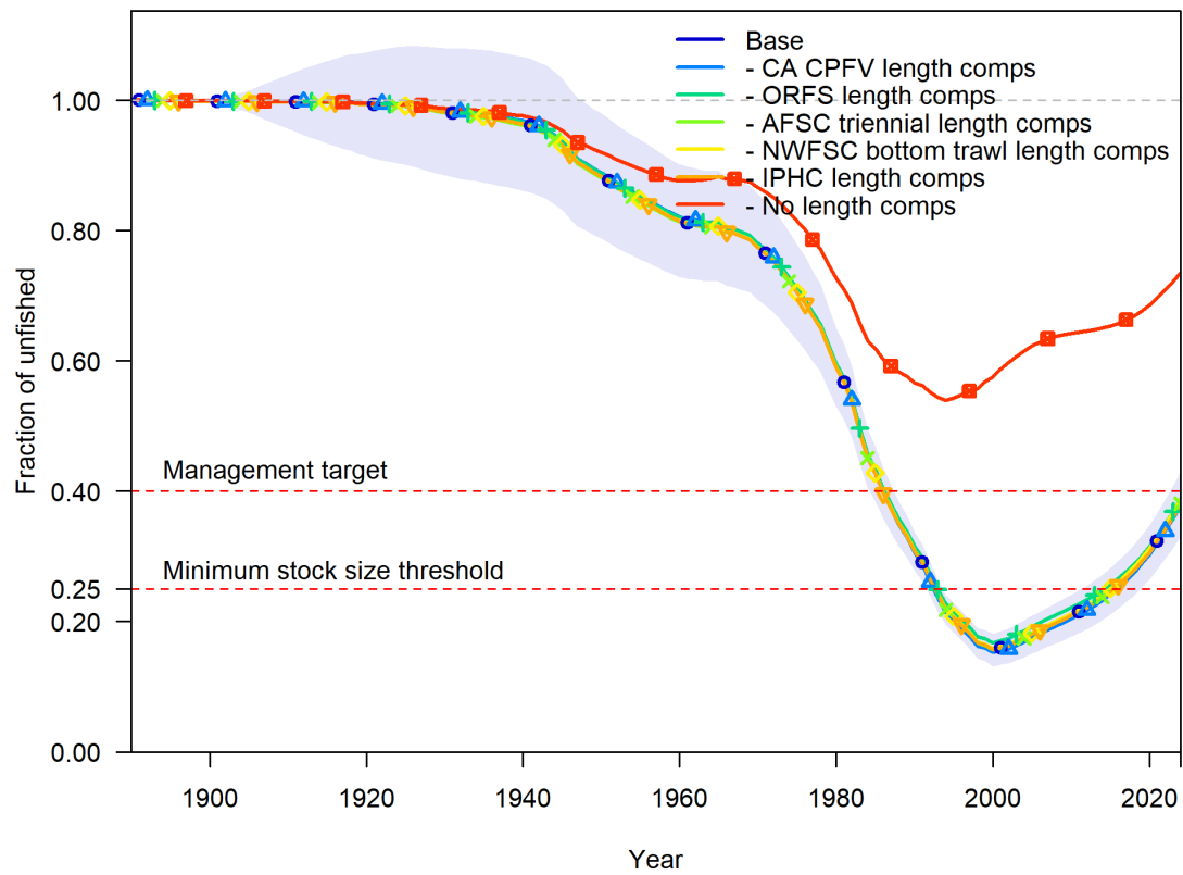
Figure 68: Relative spawning output across length composition inclusion sensitivities (2 of 2).
