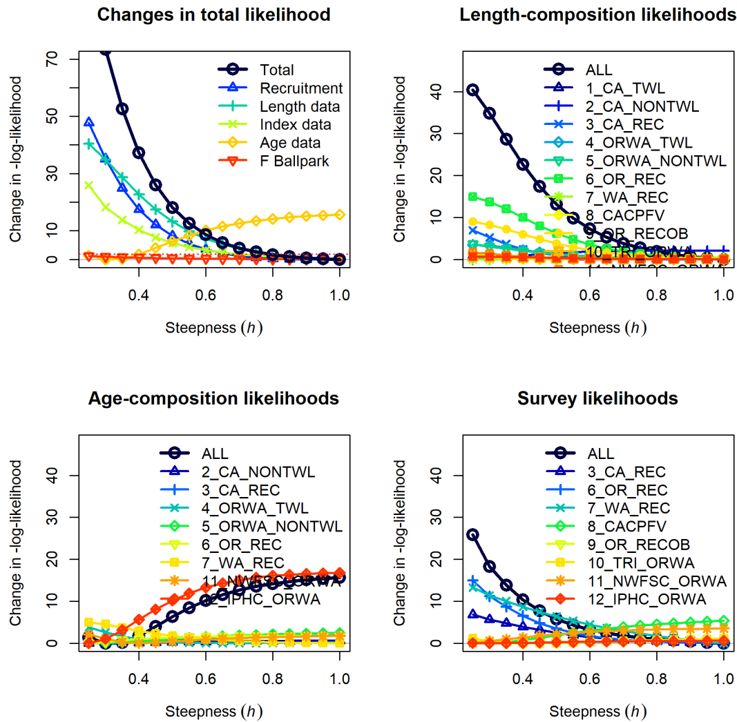
Figure 83: Negative log-likelihood profile for each data component and in total given different values of stock-recruit steepness ranging from 0.25 to 1.0 by increments of 0.05.
