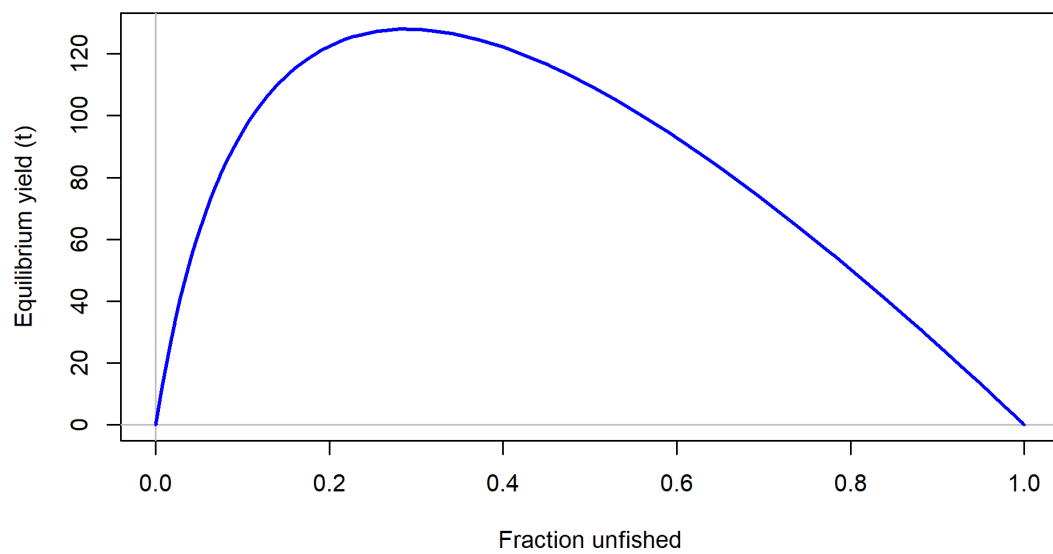
Figure 89: Equilibrium yield curve (derived from reference point values) for the base model. Values are based on 2024 fishery selectivity and distribution with steepness fixed at 0.72. The relative spawning output is relative to unfished spawning biomass.
