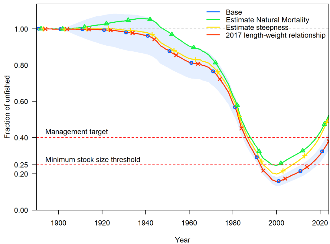
Figure 64: Relative spawning output across model structure sensitivities.
