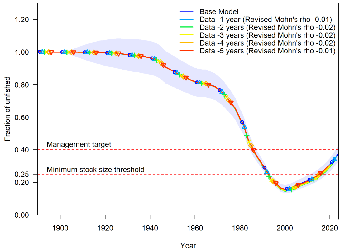
Figure 78: Results of retrospective analysis. Relative spawning output time series of this assesment base model are proved with ~95% interval.
