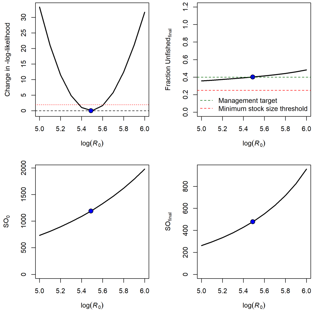
Figure 87: Likelihood profile (top left panel) for \log initial recruitment ( \ln R_0 ), with associated changes in stock status in the current year ( SB_{2025}/SB_0 ; top right panel), initial spawning biomass ( SB_0 ; bottom left panel), and current year spawning biomass ( SB_{2025} ; bottom right panel). Points indicate the base model MLE estimate.
