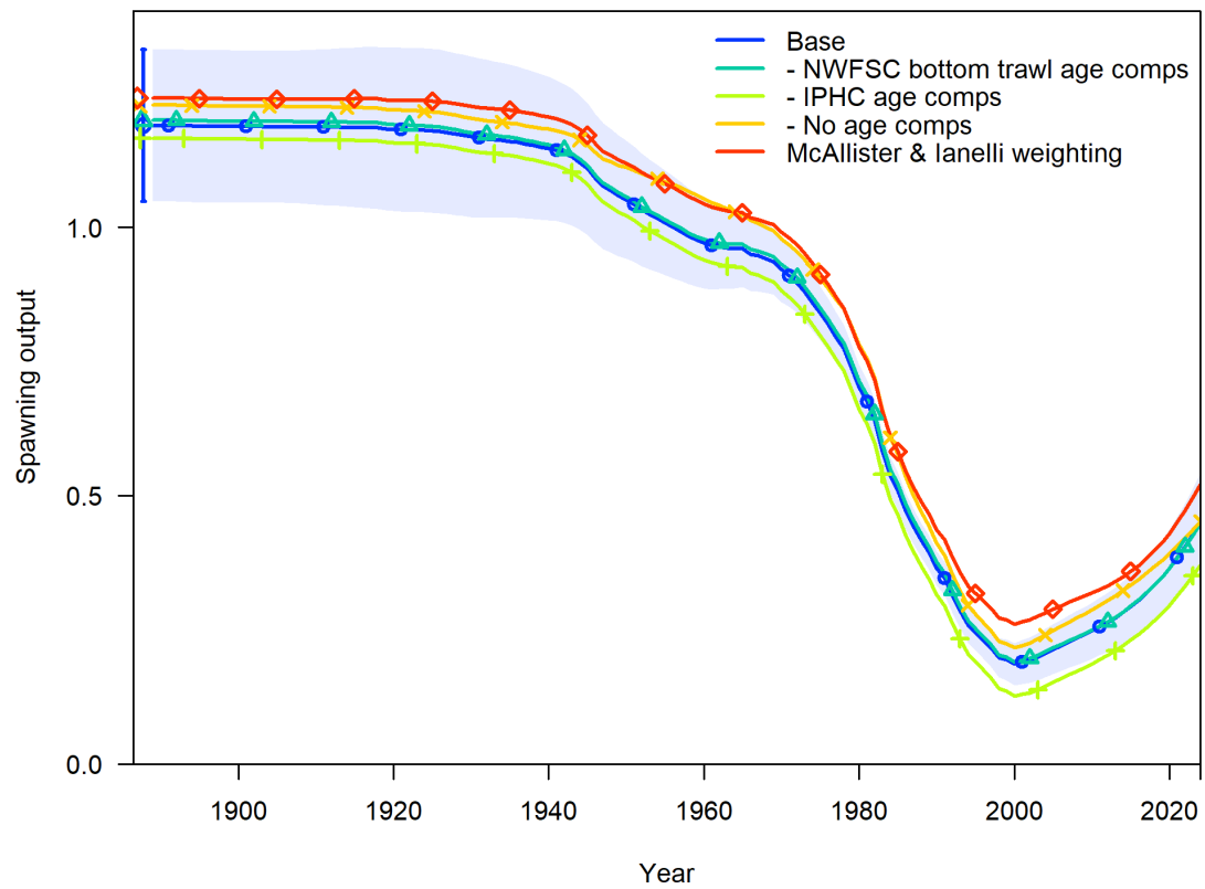
Figure 70: Spawning output (billions of eggs) across age composition inclusion sensitivities (2 of 2).
