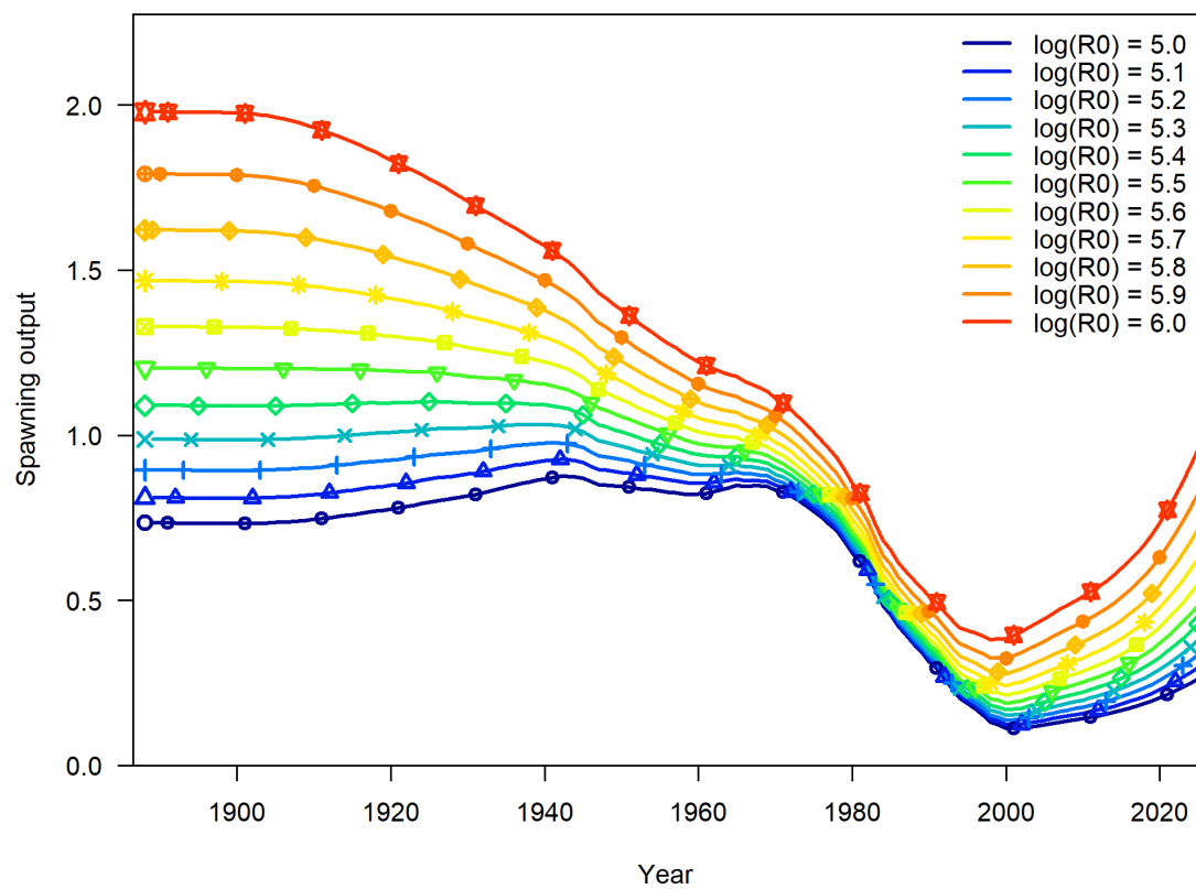
Figure 86: Spawning output (billions of eggs) as profiled over values of \ln R_0 .
