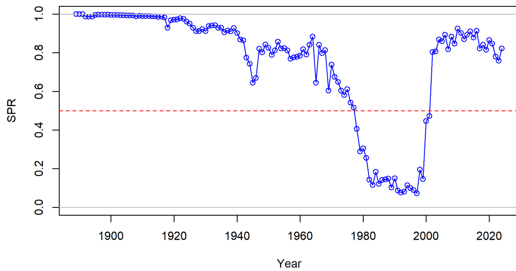
Figure 88: Time series of estimated SPR.
