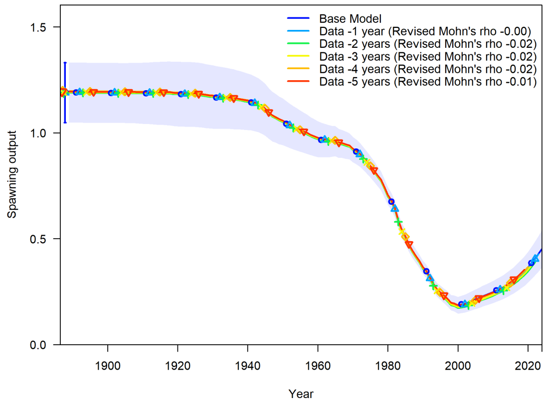
Figure 77: Results of retrospective analysis. Spawning output (billions of eggs) time series of this assesment base model are proved with ~95% interval.
