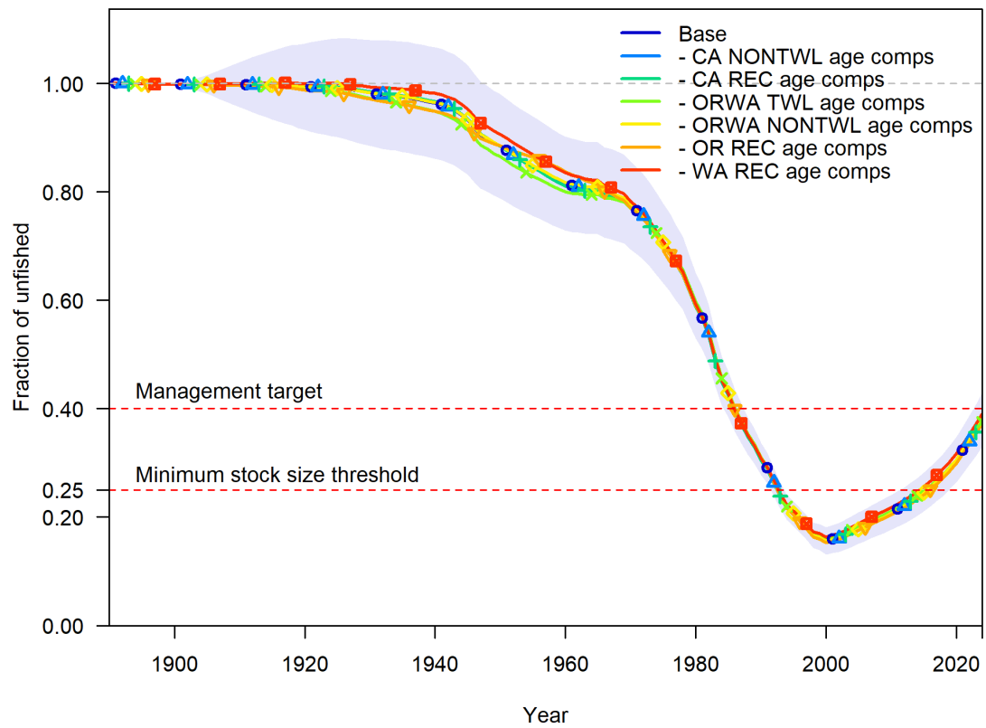
Figure 71: Relative spawning output across age composition inclusion sensitivities (1 of 2).
