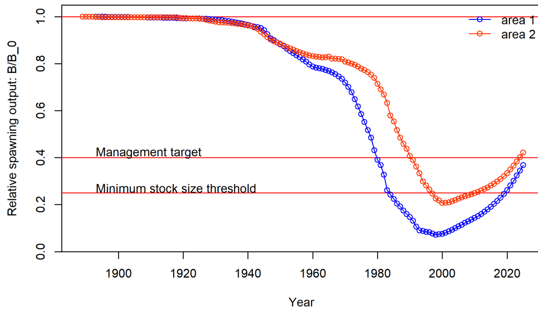
Figure 90: Time series of relative spawning output estimated by area (area 1= California, area 2 = Oregon and Washington).
