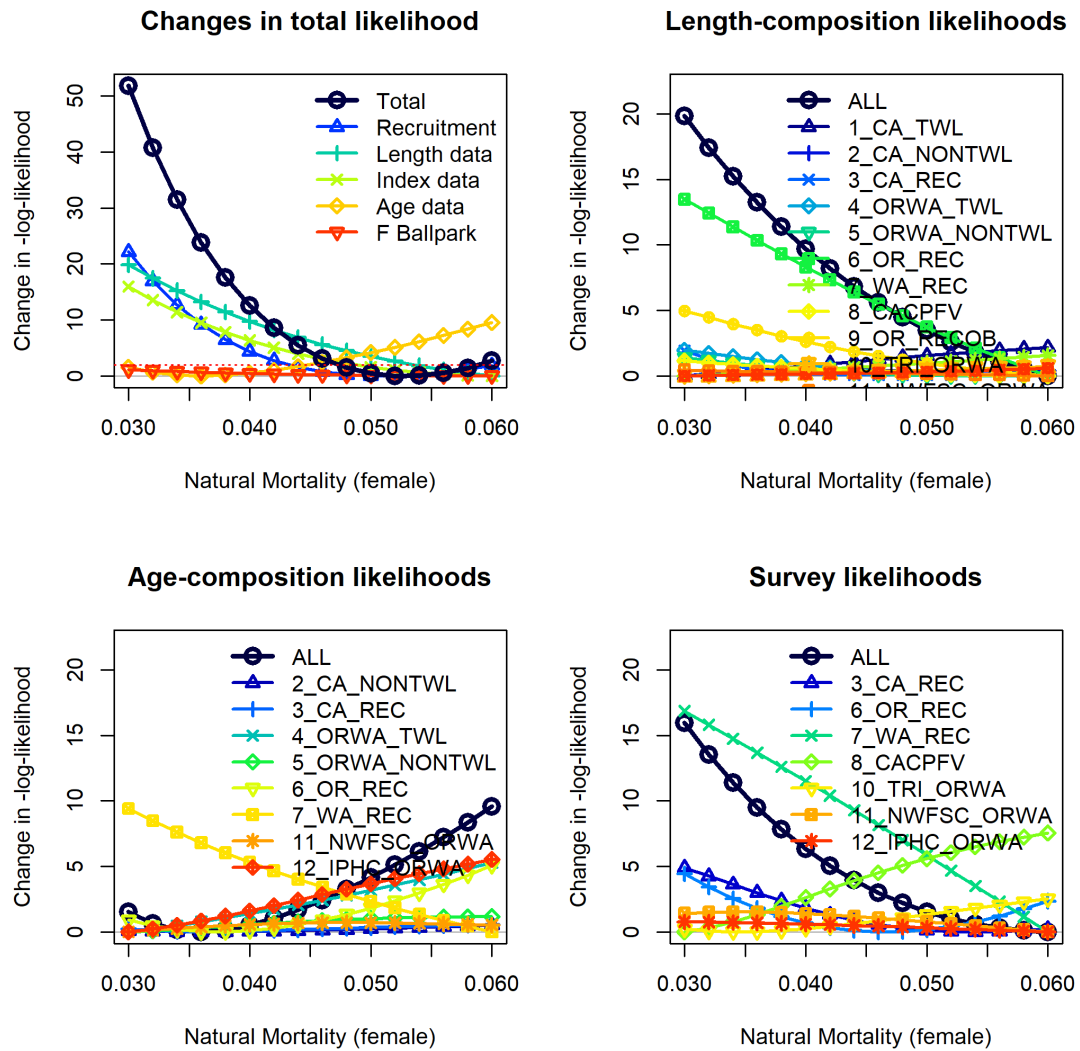
Figure 81: Negative log-likelihood profile for each data component and in total given different values of natural mortality ranging from 0.03 to 0.06 in increments of 0.002.
