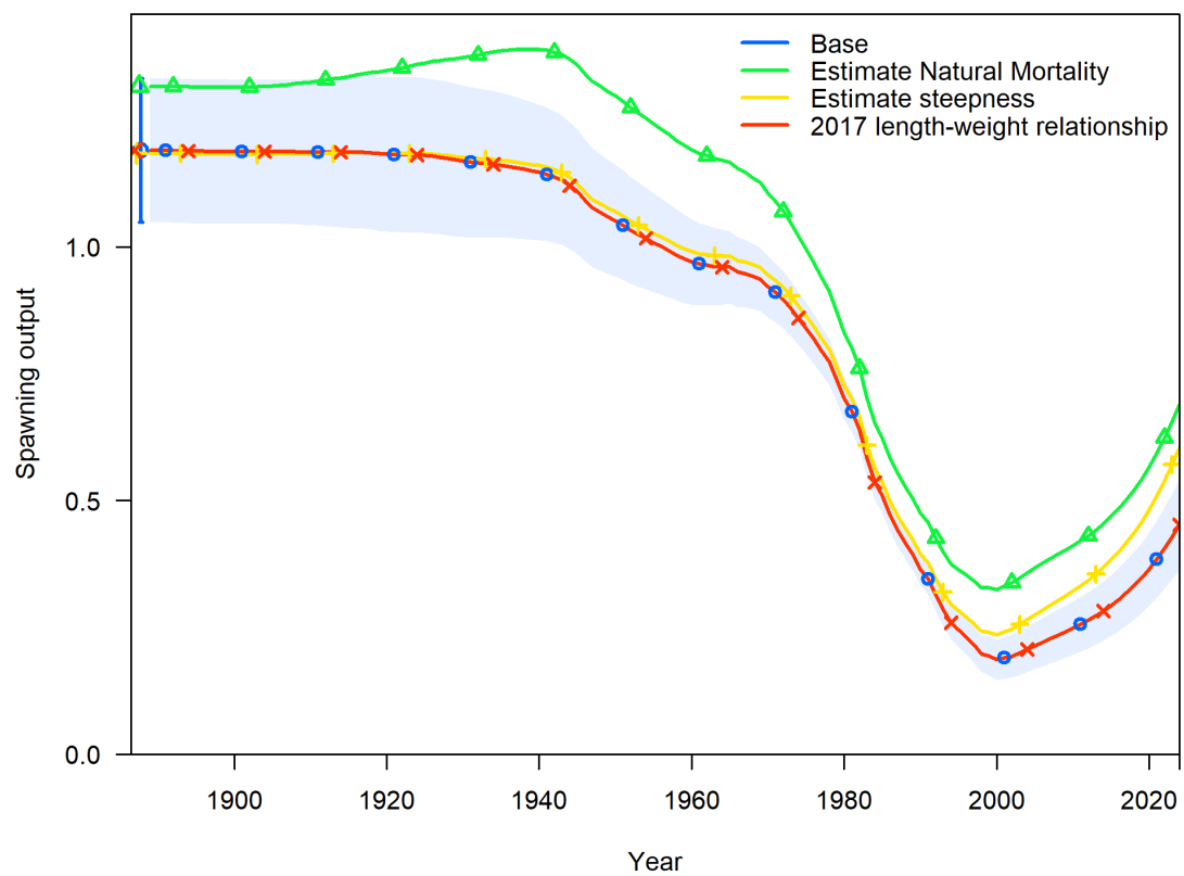
Figure 63: Spawning output (billions of eggs) across model structure sensitivities.
