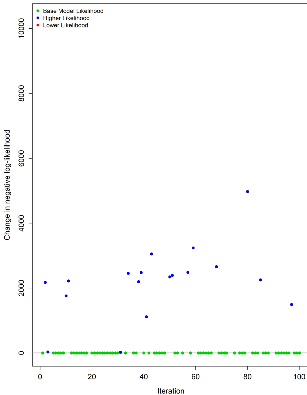
Figure 62: Results from 100 base model runs when starting parameters values are jittered by 0.1 units. Horizontal line indicates base model value.
