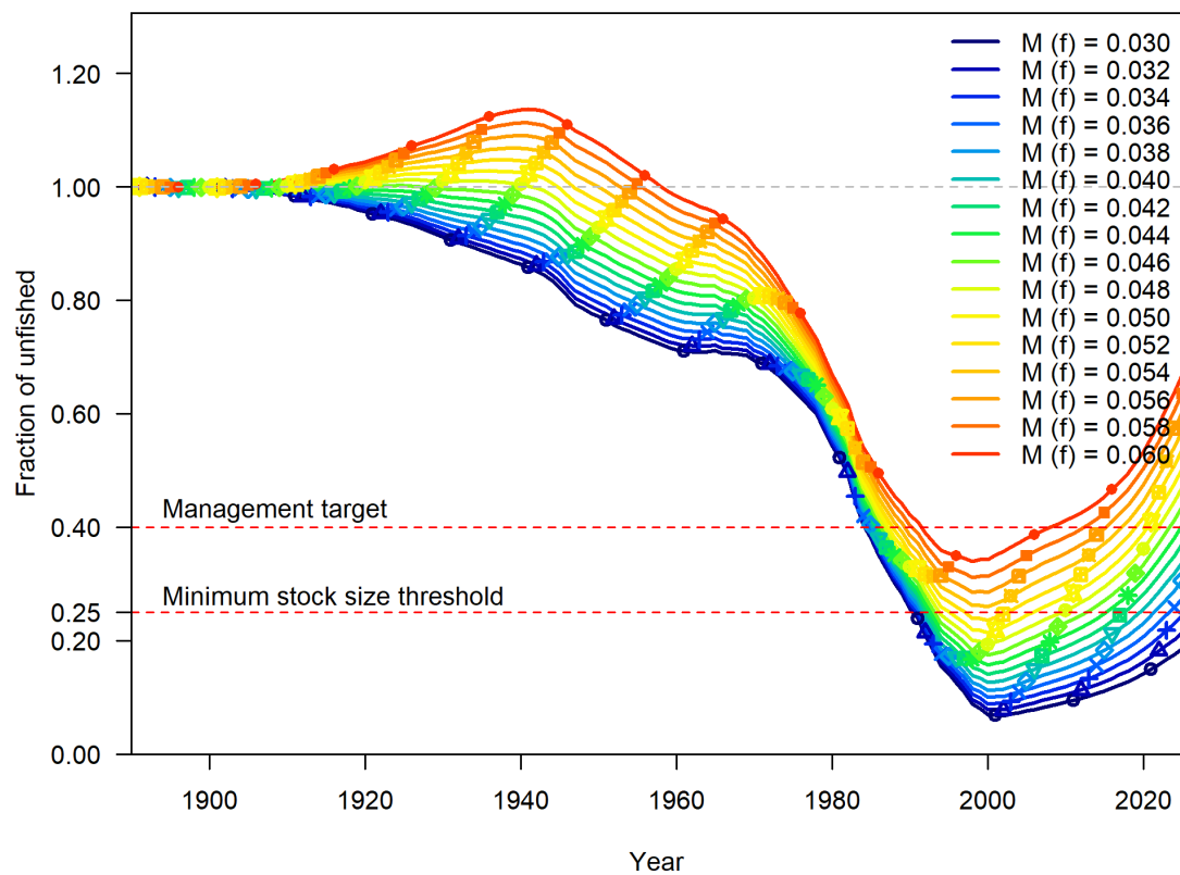
Figure 82: Time series of fraction of unfished biomass output associated with different values of natural mortality ranging from 0.03 to 0.06 in increments of 0.002.
