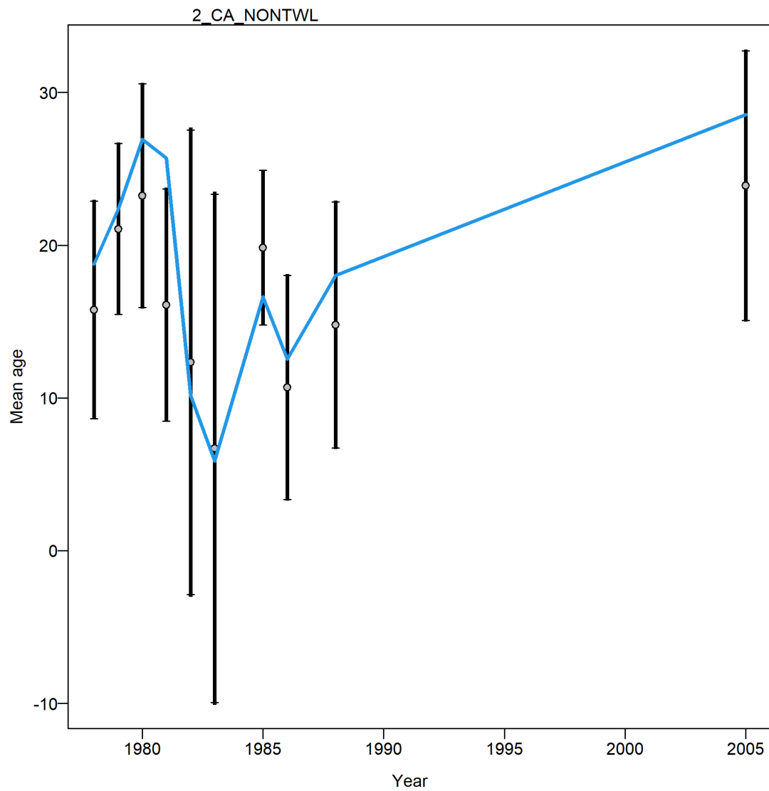
Figure 46: Mean age from conditional data (aggregated across length bins) for the CA NONTWL fleet with 95% confidence intervals based on input sample sizes. The blue line is the model expectation.
