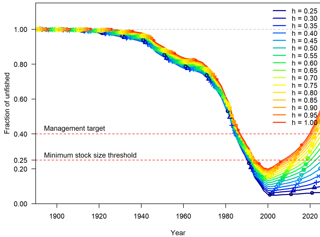
Figure 84: Time series of fraction of unfished biomass output associated with different values of steepness ranging from 0.25 to 1.0 in increments of 0.05.
