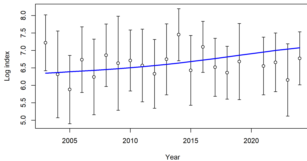
Figure 41: Fit to the log-scale WCBTS index.
