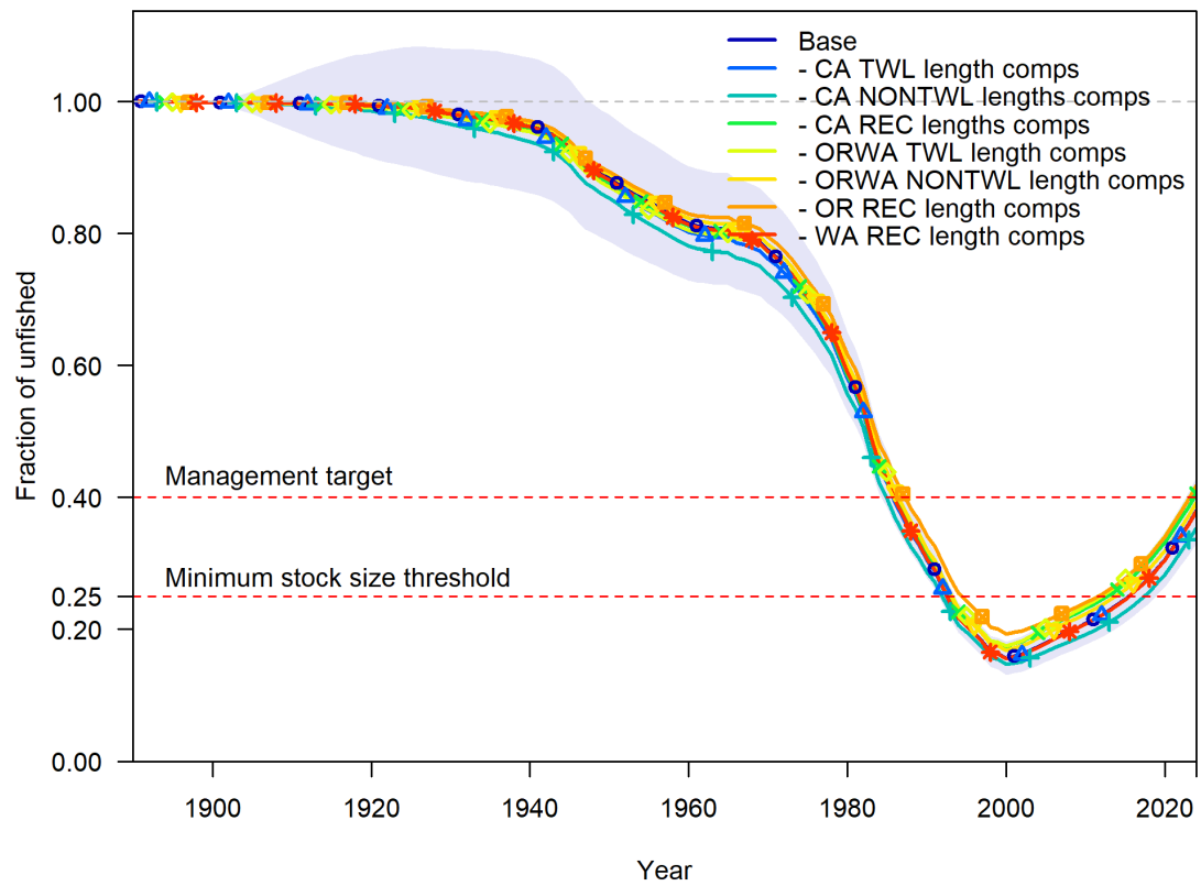
Figure 67: Relative spawning output across length composition inclusion sensitivities (1 of 2).
