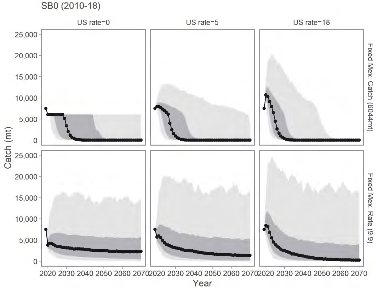
Figure 13. Projected catch (mt) for SB_{0(2010-18)} scenario. Mexico catch was either fixed at 6,044 mt (top row) or fixed at a harvest rate of 9.9% (bottom row). US harvest rate was 0, 5, or 18% (left to right columns). Values displayed are median catch values (black points), 25-75 percentiles (dark gray shading), and 5-95 percentiles (light gray shading).
