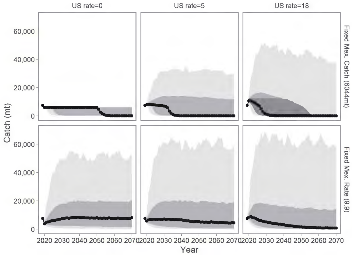
Figure 12. Projected catch (mt) for SB_0(2005-18) scenario. Mexico catch was either fixed at 6,044 mt (top row) or fixed at a harvest rate of 9.9% (bottom row). US harvest rate was 0, 5, or 18% (left to right columns). Values displayed are median catch values (black points), 25-75 percentiles (dark gray shading), and 5-95 percentiles (light gray shading).
