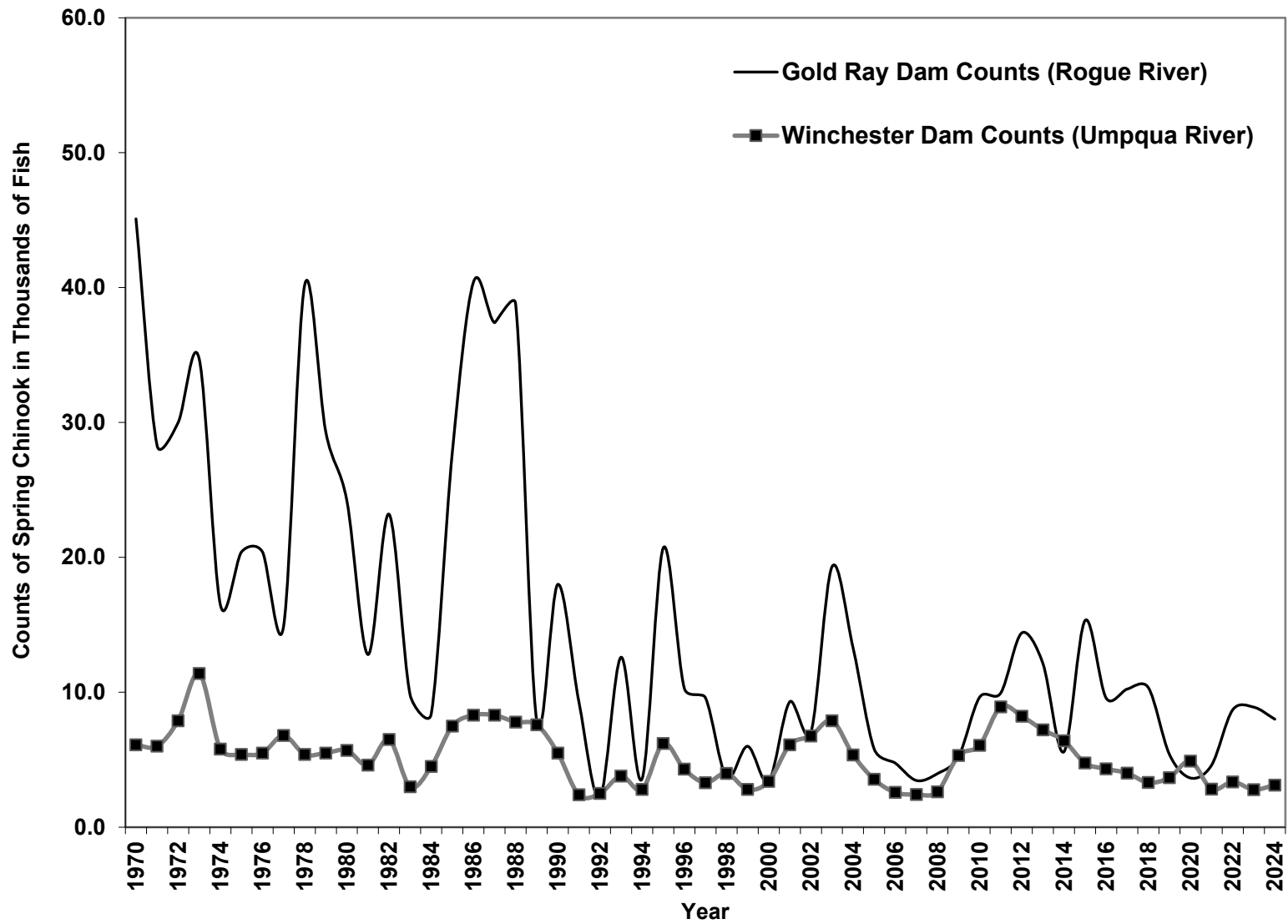
Figure II-4. Escapement indices for naturally produced Oregon coastal south/local migrating spring Chinook, 1970-2024.
