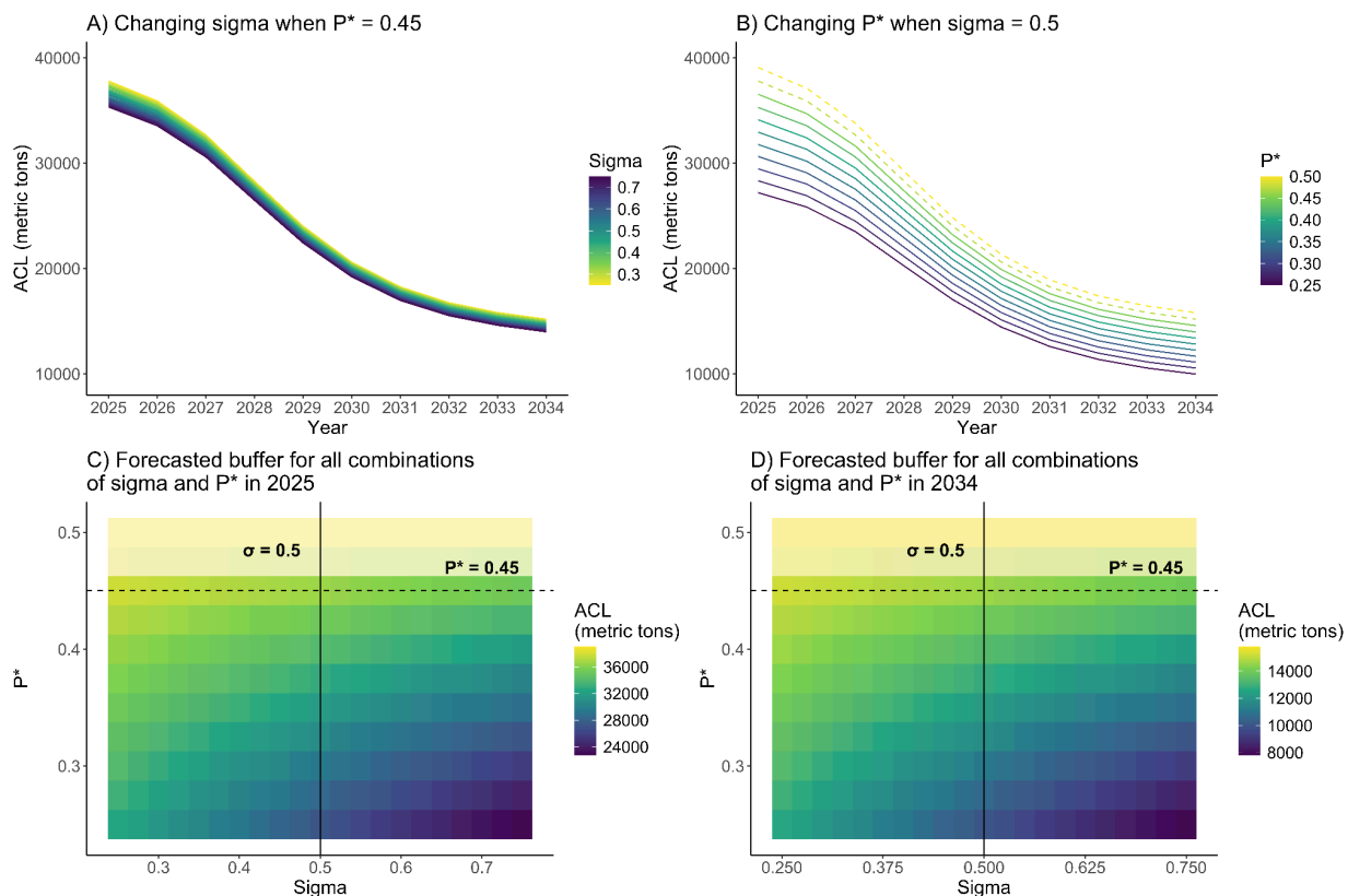
Figure 4. Changes in the projected sablefish ACL in metric tons across the range of values of sigma and P^* explored here. Panel A varies sigma with the PFMC’s default P^* value of 0.45. Panel B varies P^* with the default sigma value of 0.5 for category 1 stocks. Panels C and D show the ACL for all combinations of P^* and sigma in 2025 (the beginning of the projection period) and 2034 (the end of the 10-year projection period), respectively. In Panels C and D, the solid vertical line indicates the current sigma value for sablefish as a category 1 stock, and the dashed horizontal line indicates the P^* value chosen for sablefish in 2023. All other color scales and line types are as in Figure 2.
