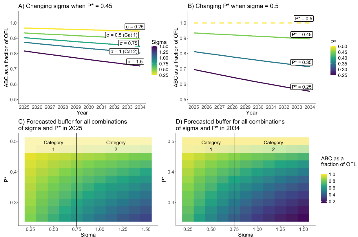
Figure 2. Changes in Acceptable Biological Catch (ABC) calculated as a fraction of the overfishing limit (OFL) across a range of reasonable values of sigma and P*. Panel A varies
