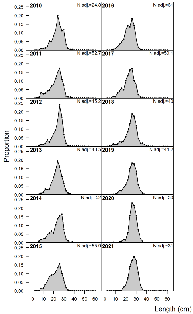
Figure 5: Coastwide current fishery length compositions of discarded fish for Rex Sole (unsexed).
