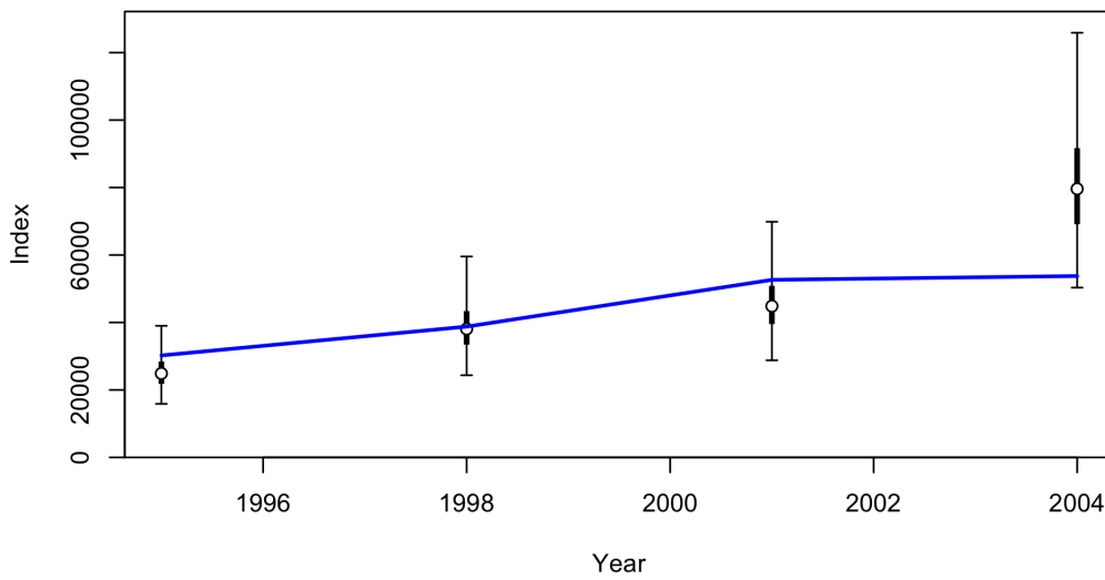
Figure 27: Fit to index data for the late period of the AFSC/NWFSC West Coast Triennial Shelf Survey (Triennial Survey). Lines indicate 95 percent uncertainty interval around index values. Thicker lines indicate input uncertainty before addition of estimated additional uncertainty.
