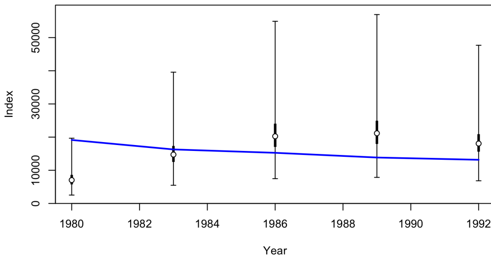
Figure 26: Fit to index data for the early period of the AFSC/NWFSC West Coast Triennial Shelf Survey (Triennial Survey). Lines indicate 95 percent uncertainty interval around index values. Thicker lines indicate input uncertainty before addition of estimated additional uncertainty.
