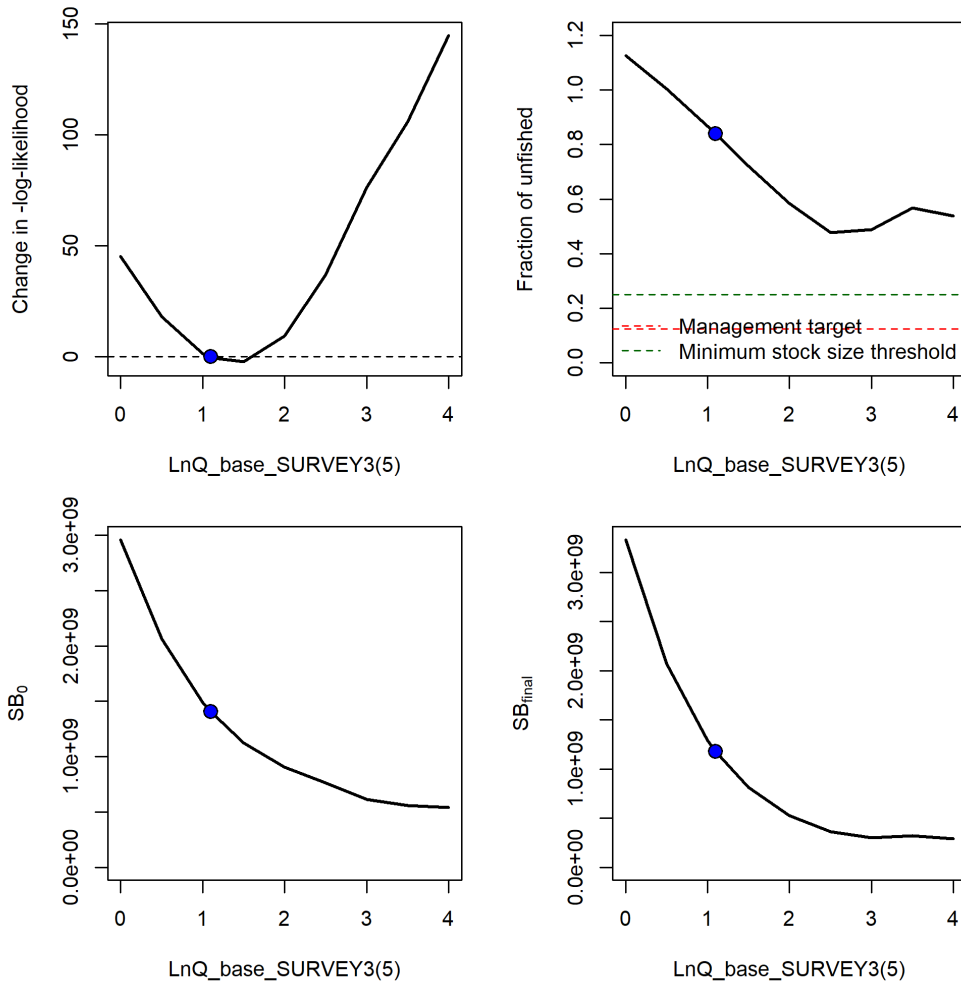
Figure 64: WCGBTS Q likelihood profiles (change in the negative log-likelihood across a range of Q values) and derived quantities.
