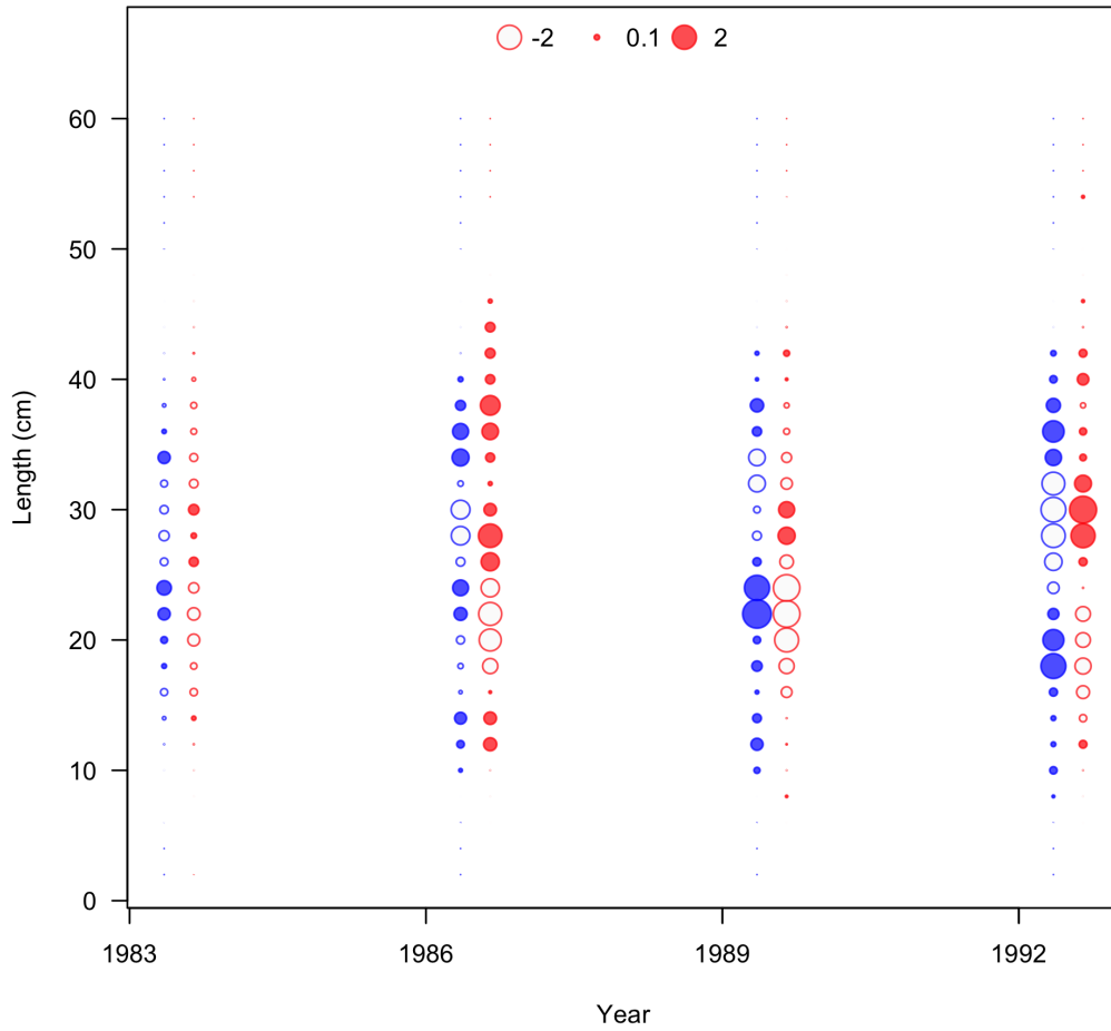
Figure 29: Pearson residuals for length composition from the early period of the AFSC/NWFSC West Coast Triennial Shelf Survey (Triennial Survey) for males (blue) and females (red). Closed bubbles are positive residuals and open bubbles are negative residuals.
