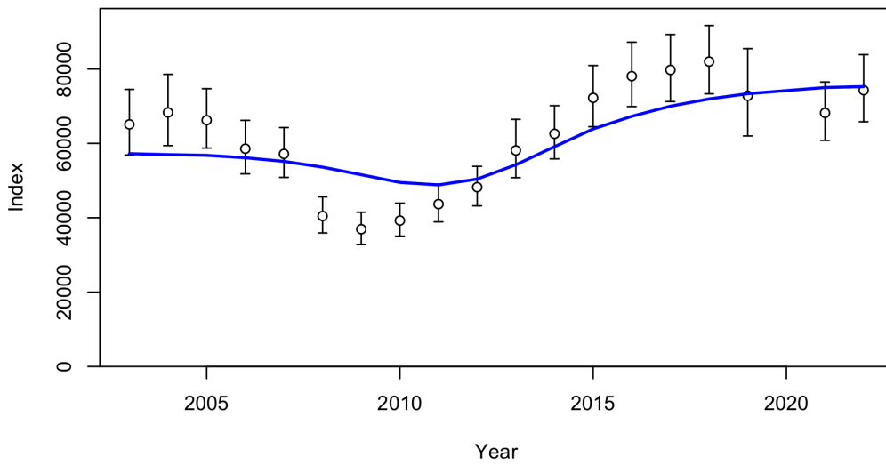
Figure 28: Fit to index data for the late period of the West Coast Groundfish Bottom Trawl Survey (WCGBTS). Lines indicate 95 percent uncertainty interval around index values.
