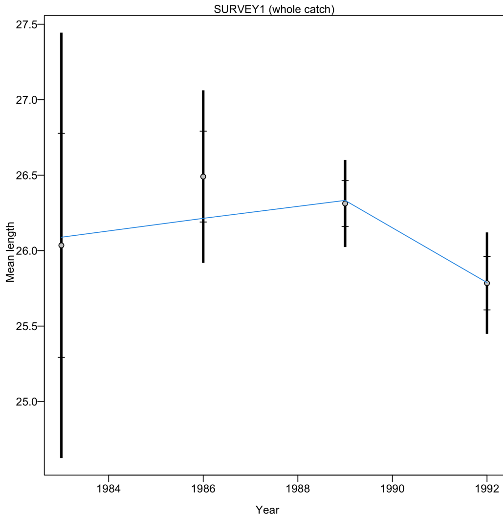
Figure 32: Fit to mean length from the early period of the AFSC/NWFSC West Coast Triennial Shelf Survey (Triennial Survey) with 95 percent confidence intervals.
