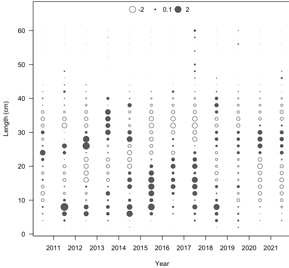
Figure 39: Pearson residuals, discard, current fishery (max=7.8). Closed bubbles are positive residuals (observed > expected) and open bubbles are negative residuals (observed < expected).
