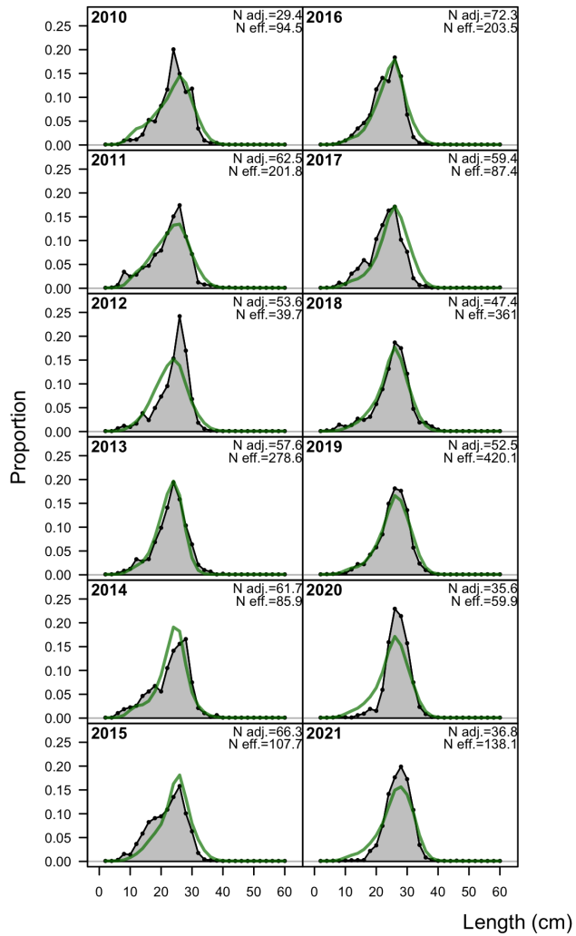
Figure 67: Length comps, discard, current fishery (2002-2022). ‘N adj.’ is the input sample size after data-weighting adjustment. N eff. is the calculated effective sample size used in the McAllister-Ianelli tuning method.
