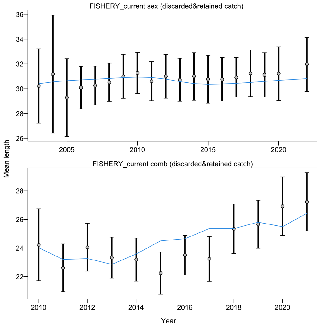
Figure 36: Fit to mean length from the fishery with 95 percent confidence intervals.
