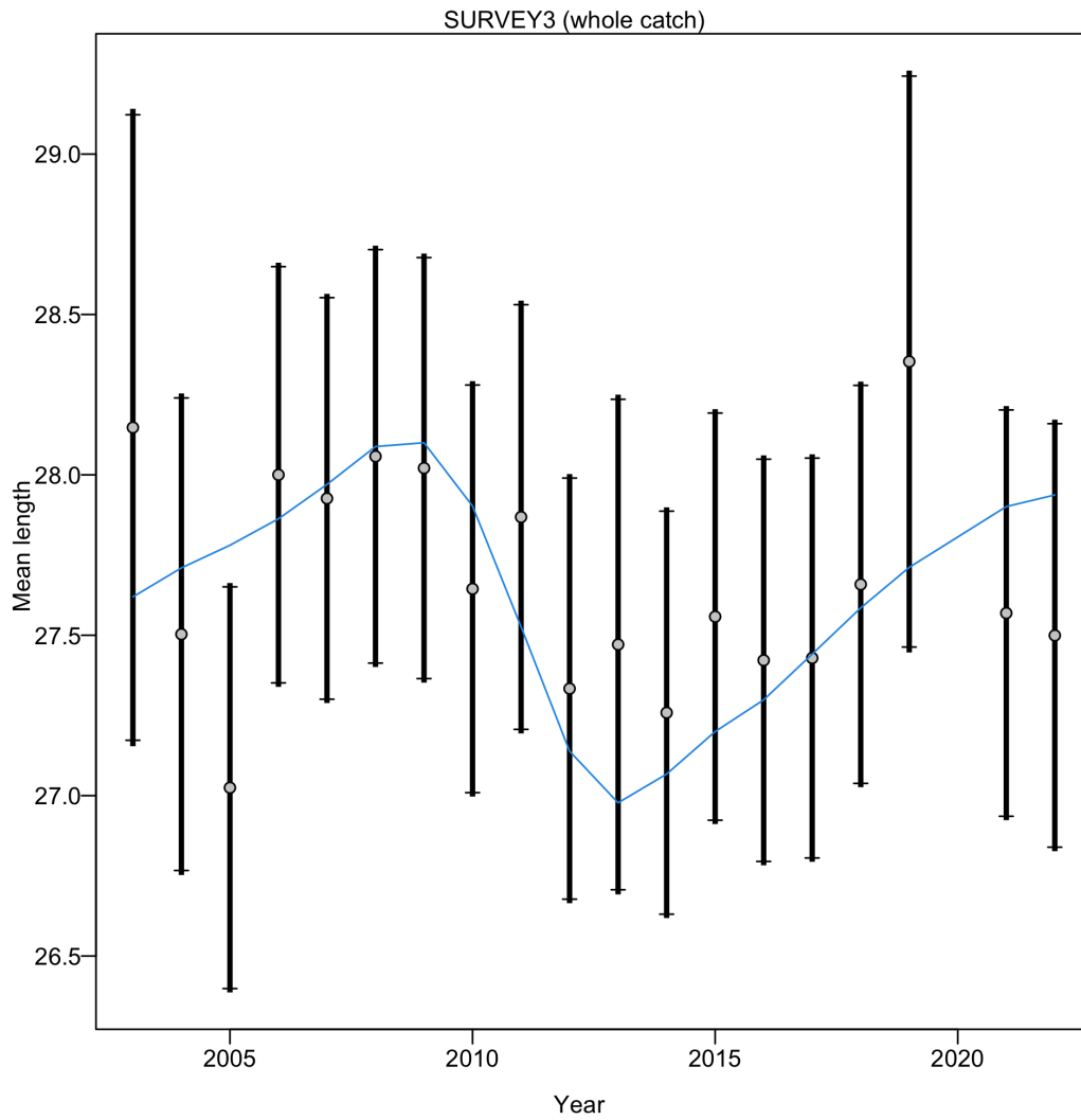
Figure 34: Fit to mean length from the West Coast Groundfish Bottom Trawl Survey (WCGBTS) with 95 percent confidence intervals.
