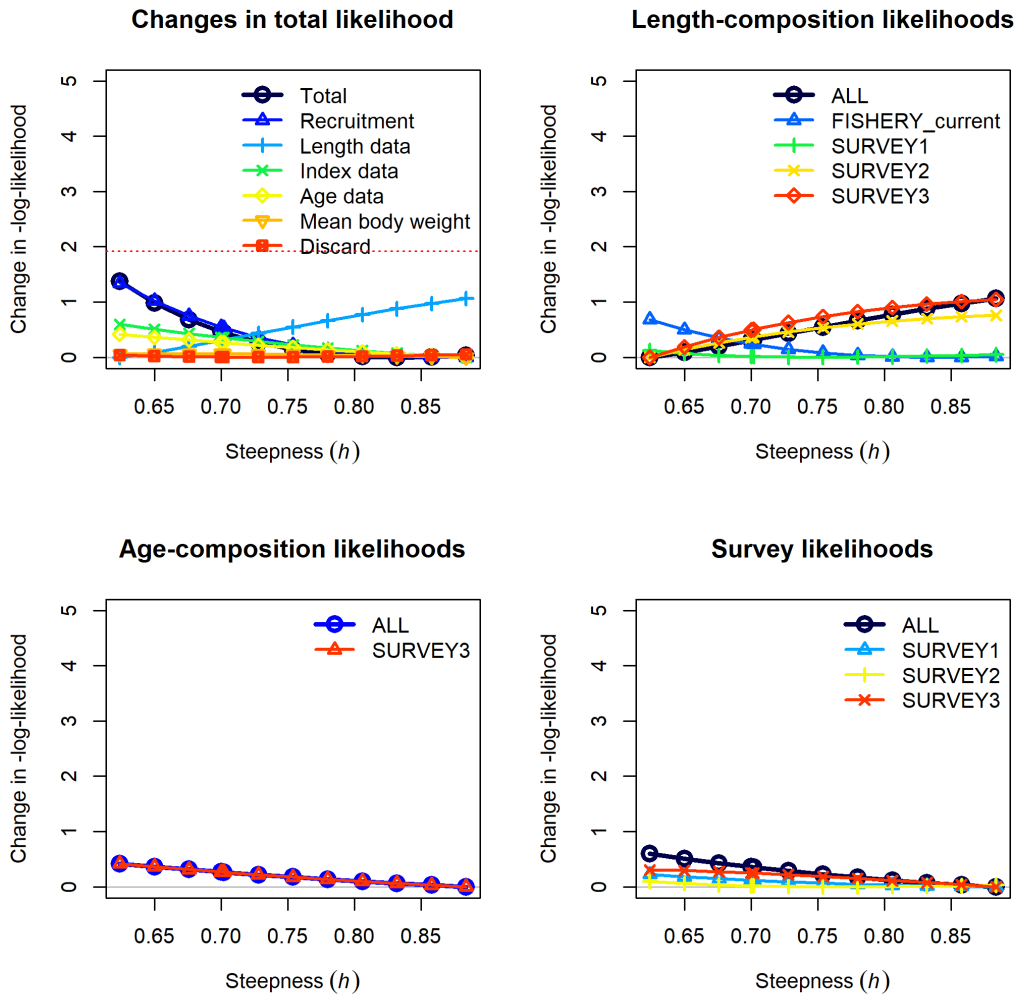
Figure 61: Steepness likelihood component contributions.
