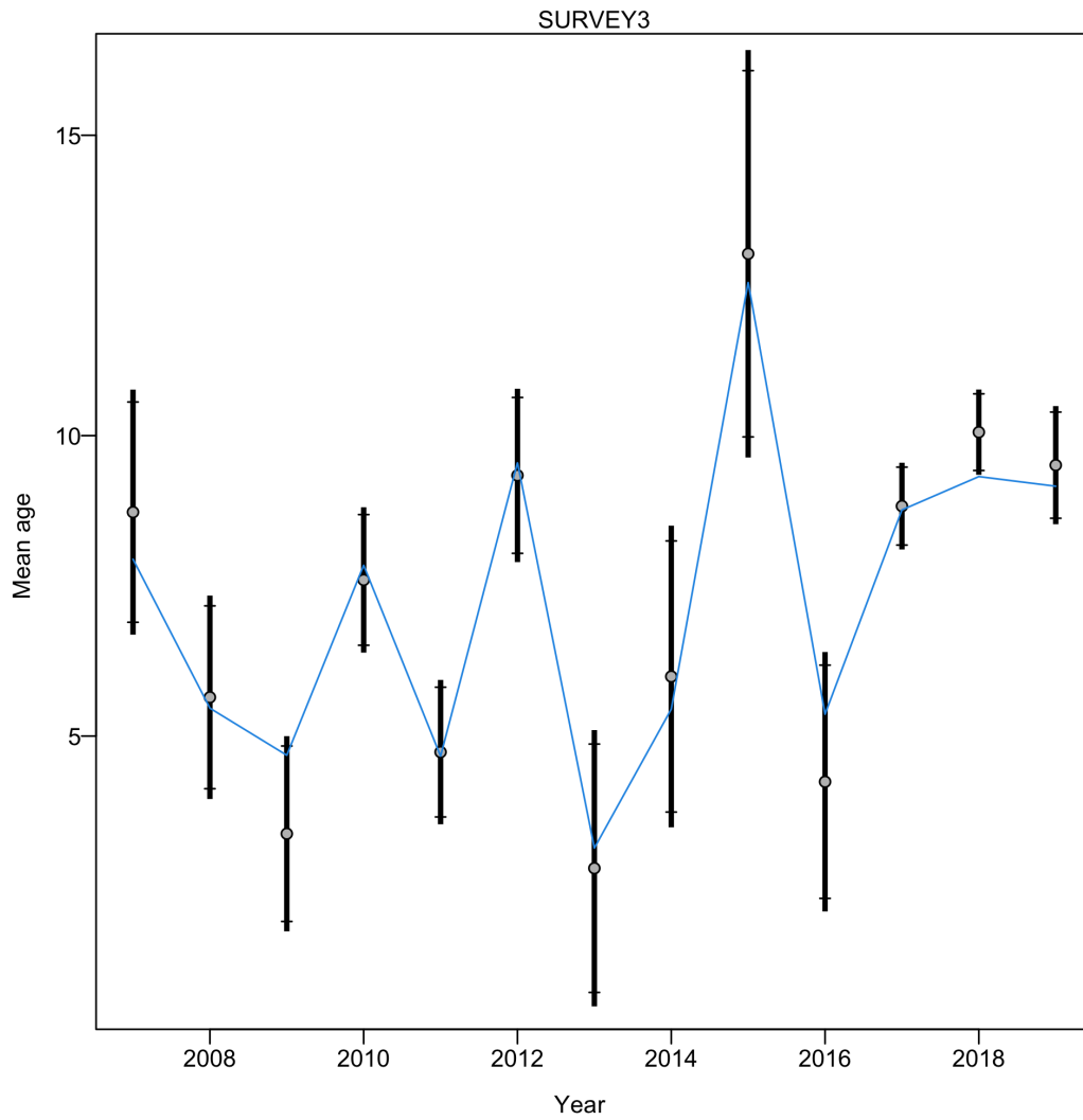
Figure 42: Fit to the mean age from the West Coast Groundfish Bottom Trawl Survey (WCGBTS) with 95 percent confidence intervals.
