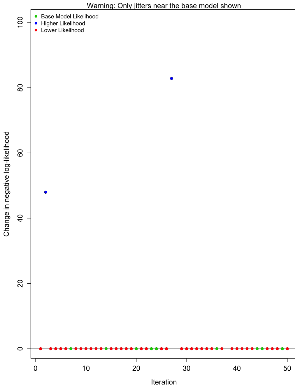
Figure 66: Change of negative log-likelihood for 50 iterations with 10 percent jitter.
