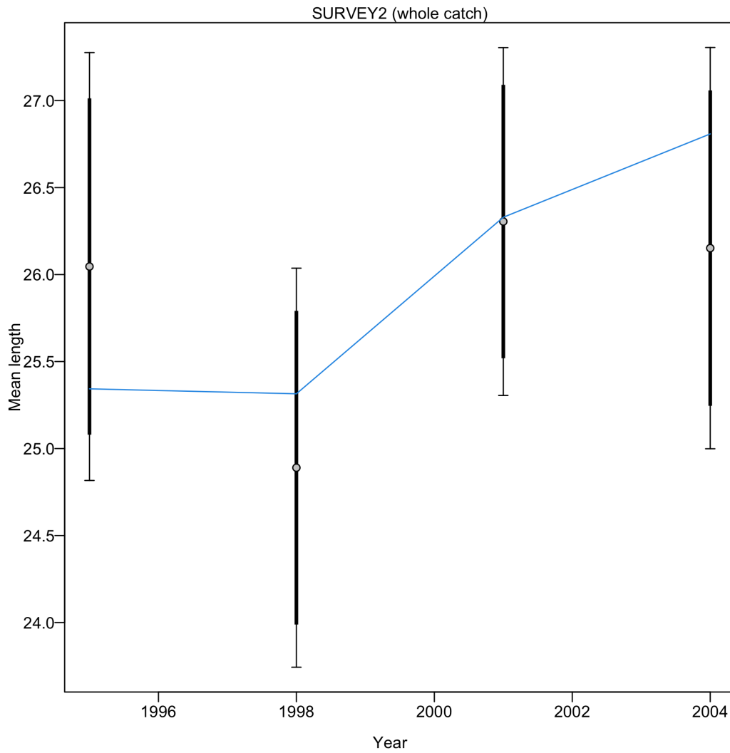
Figure 33: Fit to mean length from the late period of the AFSC/NWFSC West Coast Triennial Shelf Survey (Triennial Survey) with 95 percent confidence intervals.
