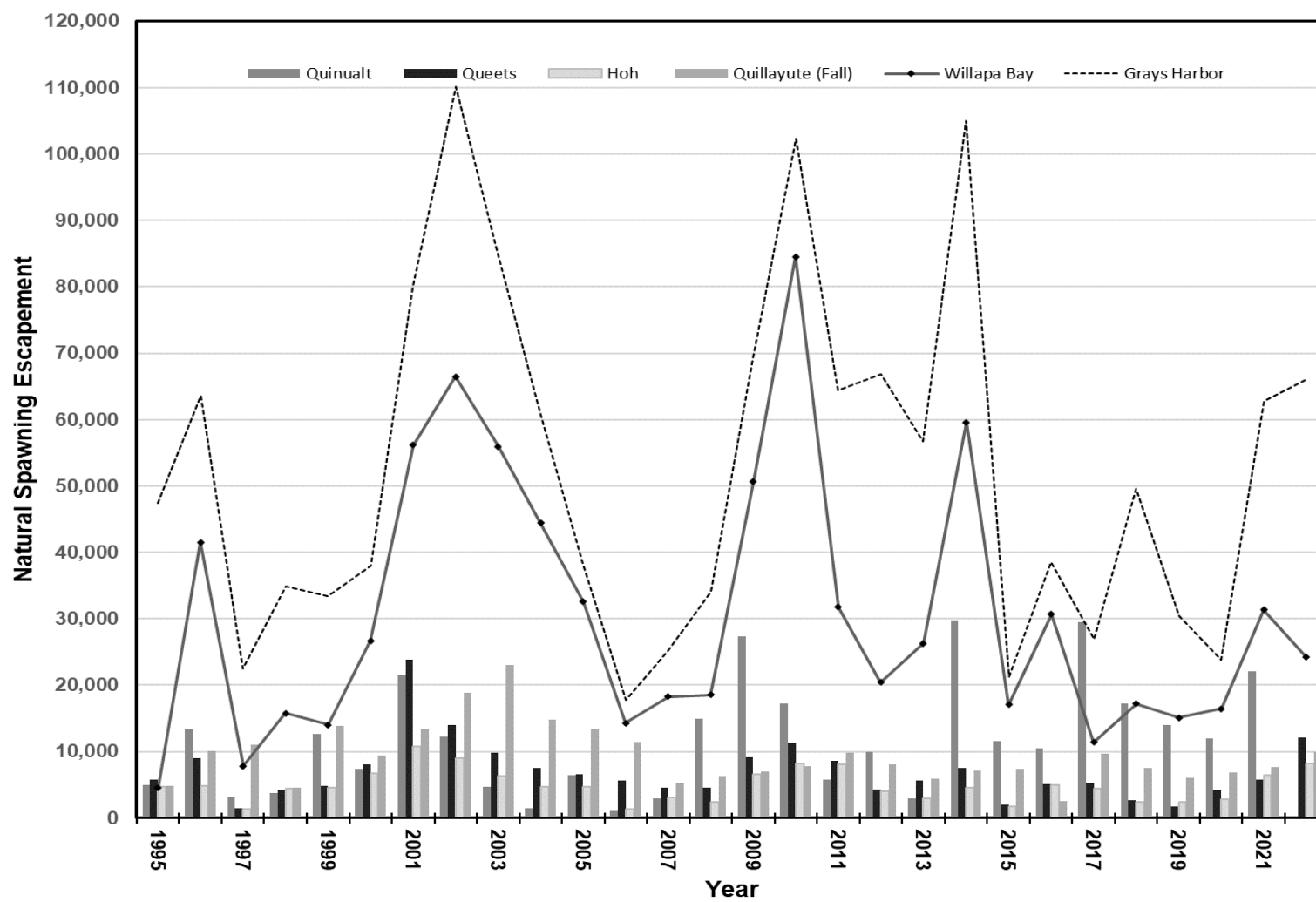
Figure III-3. Washington Coast adult coho natural spawning escapement, 1995-2022.
