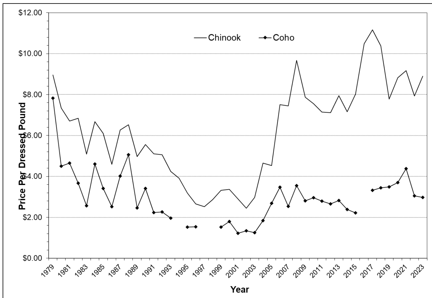
Figure IV-3. West Coast ocean non-Indian commercial salmon average annual exvessel prices (inflation adjusted, 2023 dollars).
