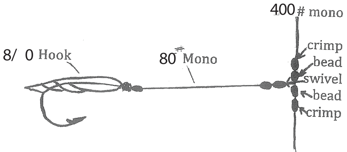
Hook Setup
