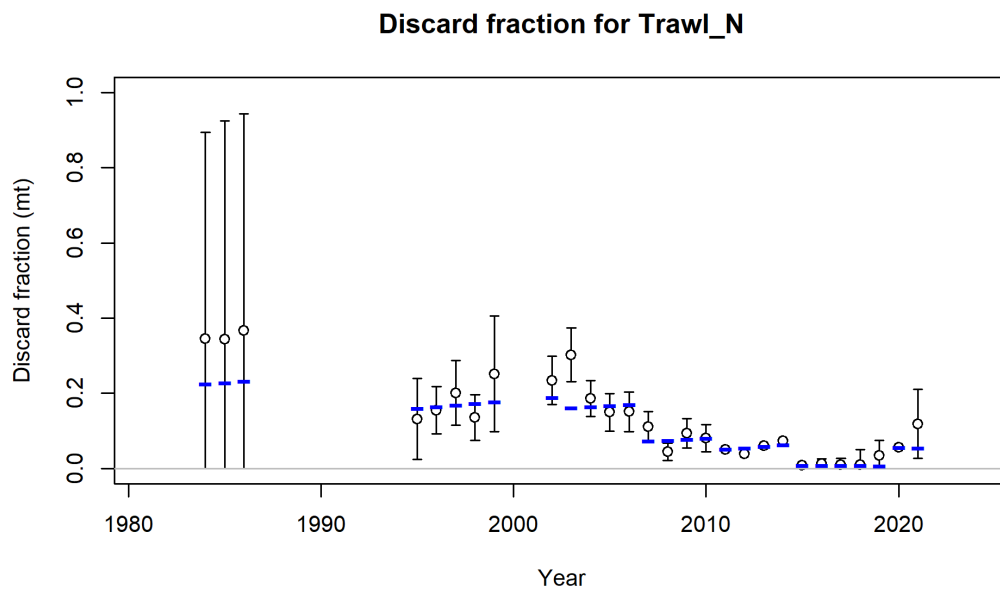
Figure 29: Discard fraction (percent of total catch that is not landed) for the North trawl fleet.
