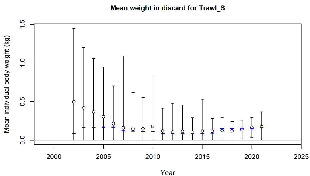
Figure 45: Mean individual body weight (kg) in discard for the South trawl fleet.
