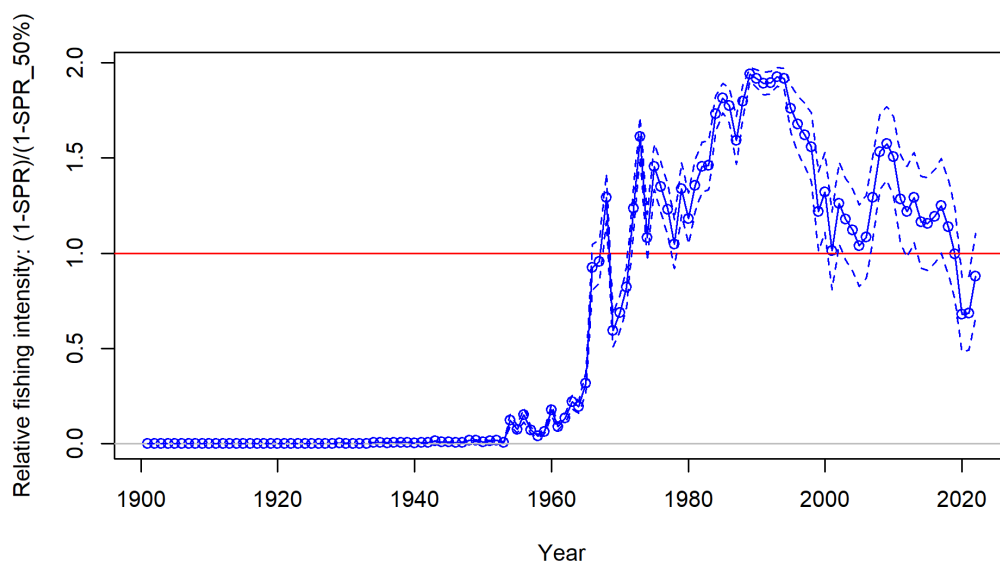
Figure vii: Estimated relative fishing intensity as a function of spawning potential ratio (SPR).
