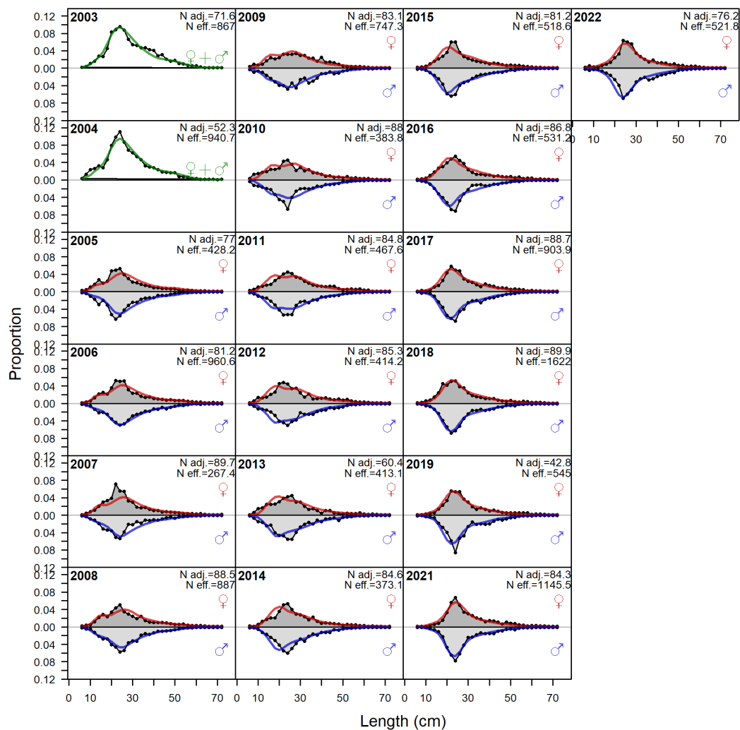
Figure 41: Length comps, whole catch, for the WCG BTS. ‘N adj.’ is the input sample size after data-weighting adjustment. N eff. is the calculated effective sample size used in the McAllister-Ianelli tuning method.
