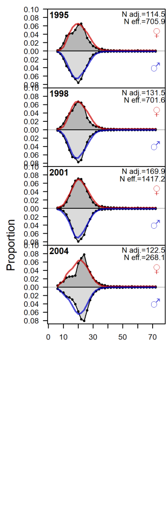
Figure 40: Length comps, whole catch, for the late-Triennial Survey (1995-2004). ‘N adj.’ is the input sample size after data-weighting adjustment. N eff. is the calculated effective sample size used in the McAllister-Ianelli tuning method.
