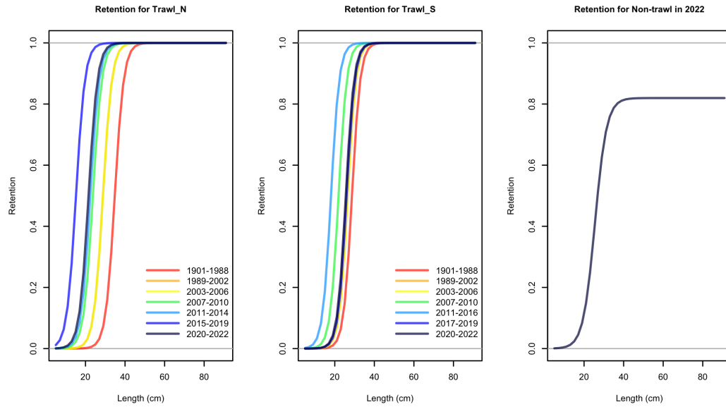
Figure 26: Retention curves for time blocks in the North Trawl, South Trawl, and Non-Trawl fleets.
