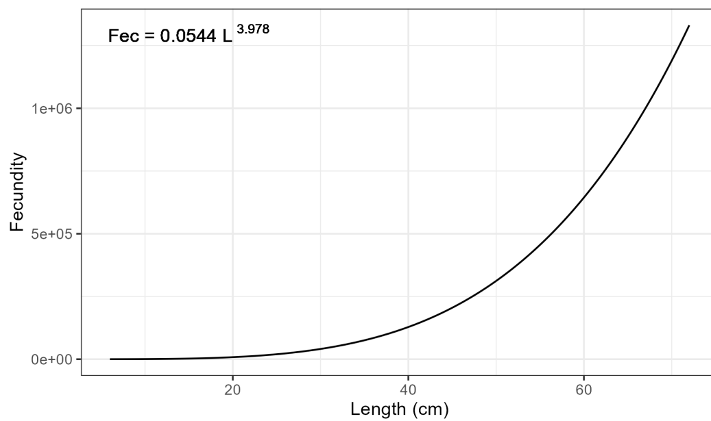
Figure 16: Fecundity-at-length relationship.
