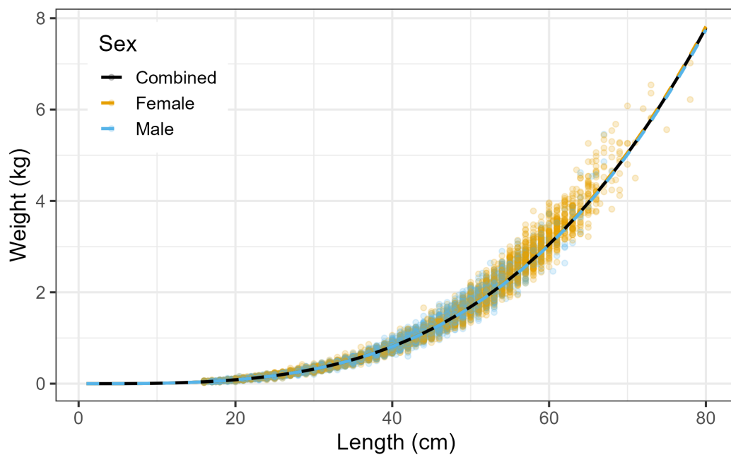
Figure 13: 2023 length-weight relationship and fits to WCGBTS weight-length data.
