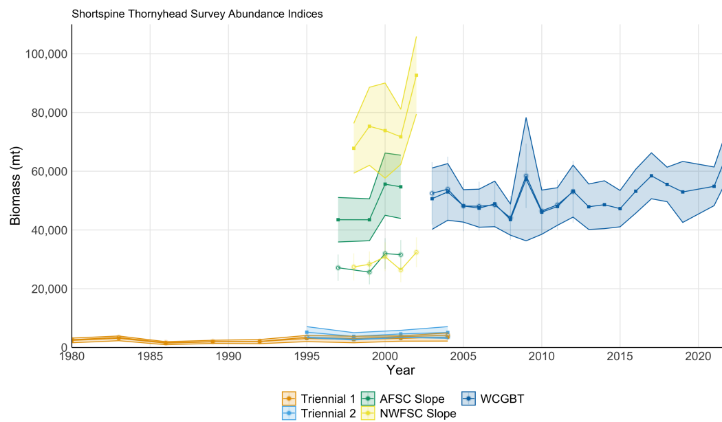
Figure 8: Abundance index timeseries. Points with shaded regions were calculated with survey data through 2023 using the nwfscSurvey R package, while points with errorbars are taken directly from the 2013 assessment which used GLMs.
