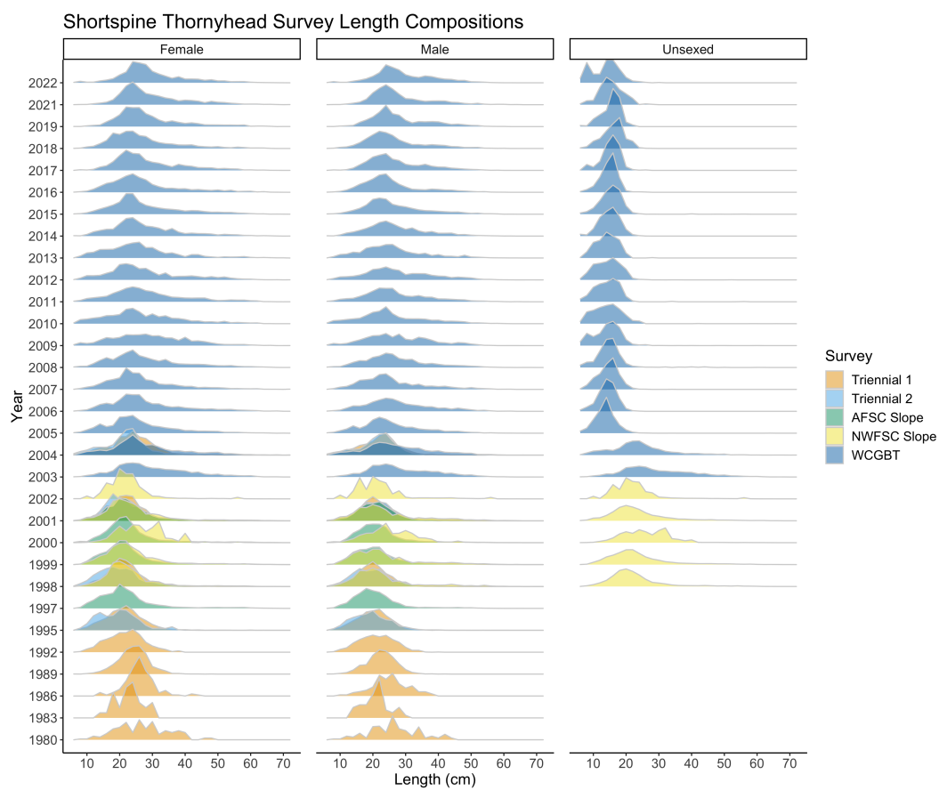
Figure 11: Summary of annual length composition data from available scientific surveys.
