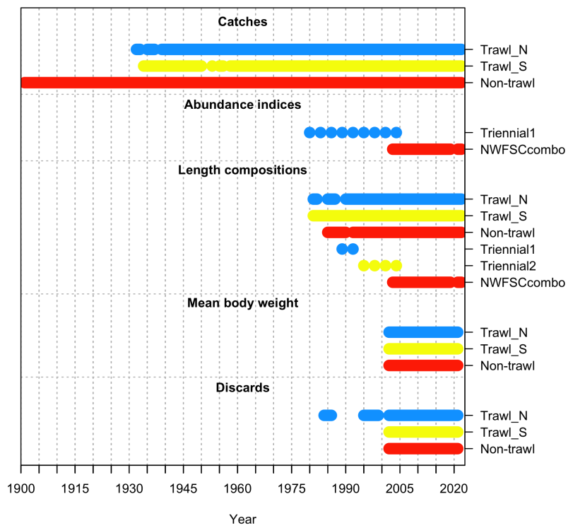
Figure ii: Summary of data sources used in the base model.
