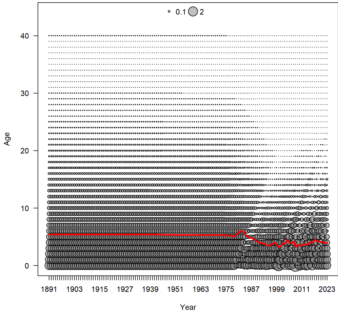
Figure 131: Male black rockfish mean age over time.
