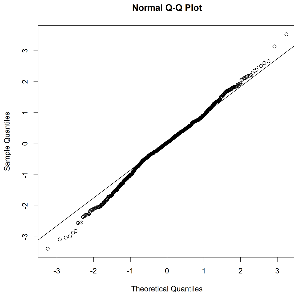
Figure 21: Q-Q plot for the marine reserves hook and line survey.
