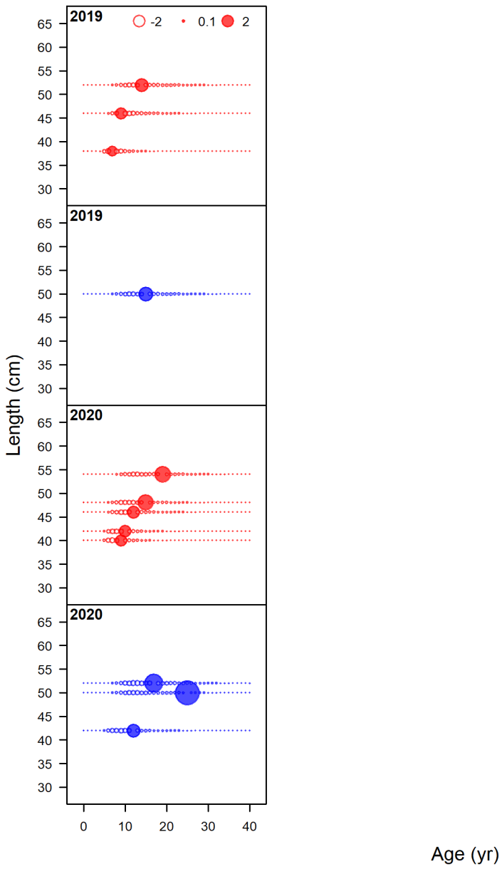
Figure 101: Pearson residuals, whole catch, Trawl_wdis (max=13.1) (plot 3 of 3).
