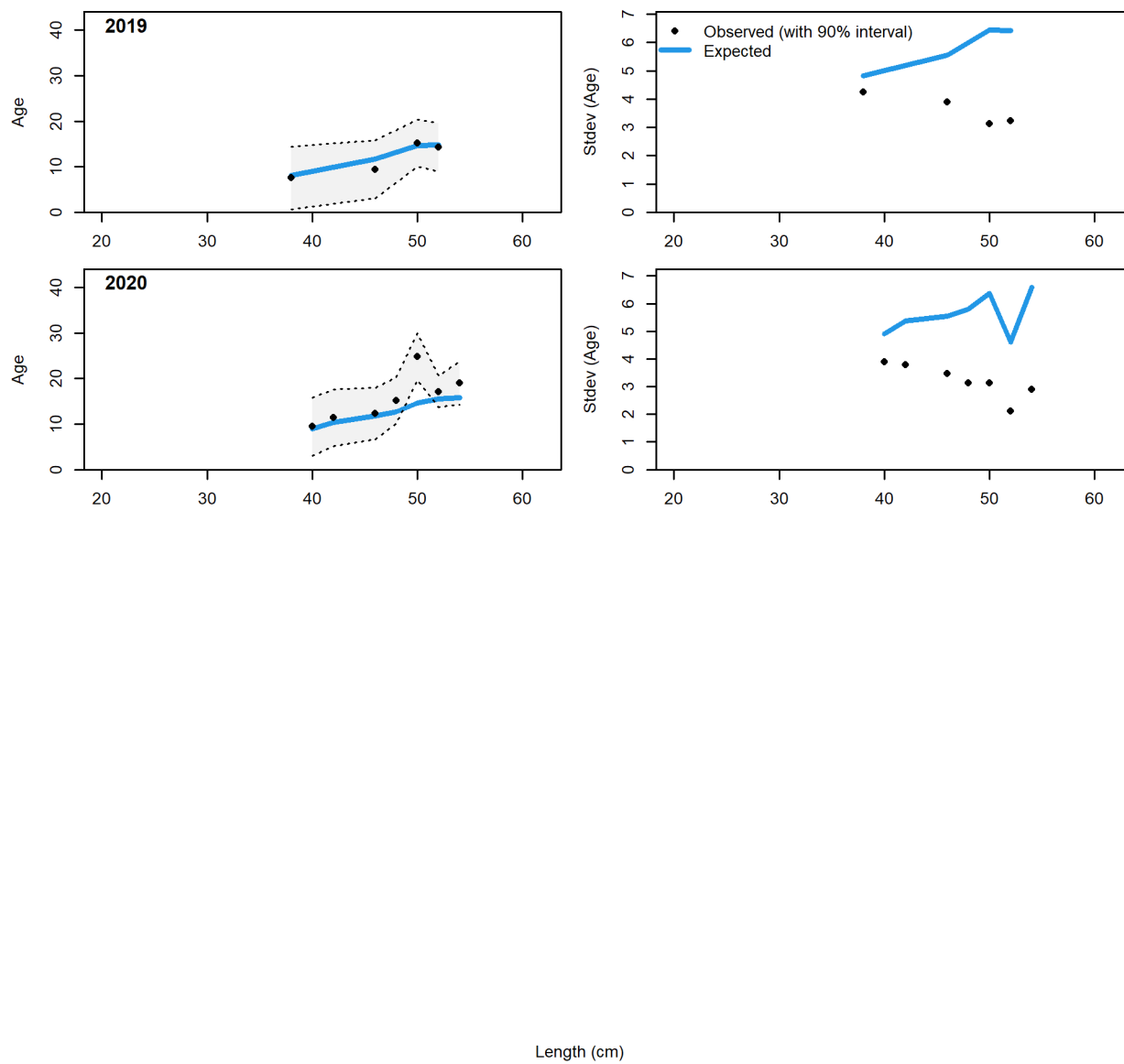
Figure 116: Trawl conditional AAL plot (plot 5 of 5).
