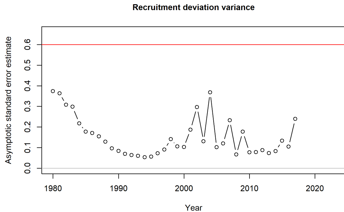
Figure 65: Recruitment deviations variance check. Low standard deviations indicate years with informative deviations .
