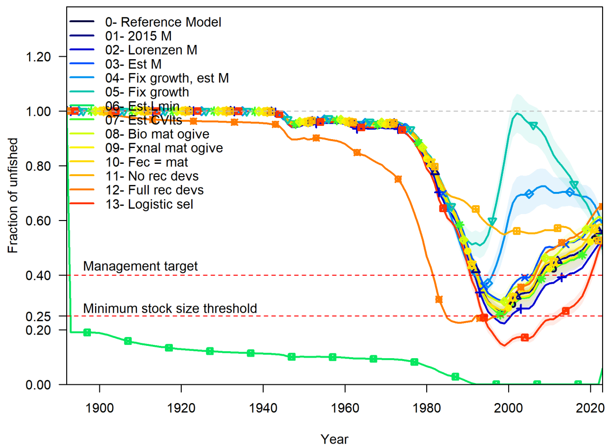
Figure 33: Relative spawning output time series by model specification scenario compared to the pre-STAR reference model. See section 3.5.1.2 for more details on each scenario.
