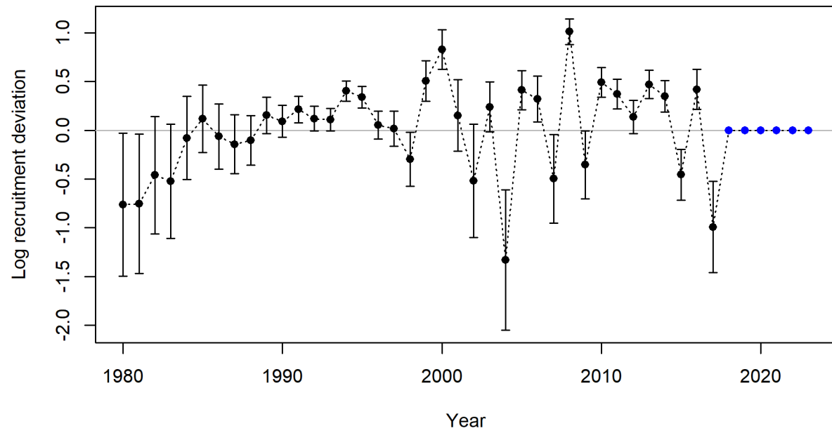
Figure iv: Estimated time series of recruitment deviations.
