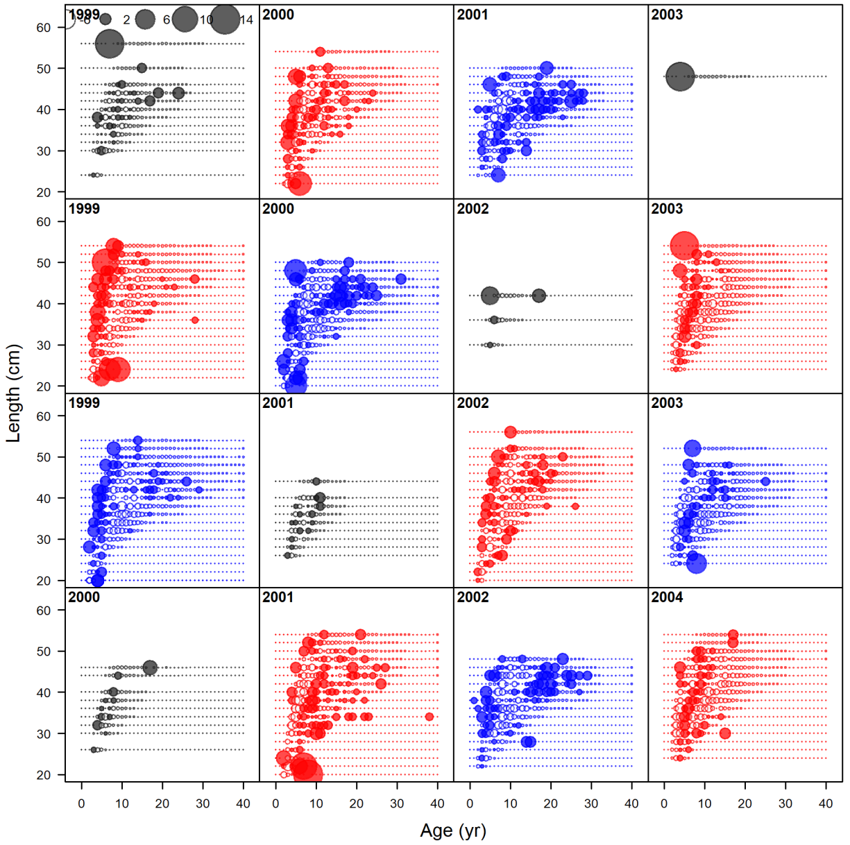
Figure 107: Pearson residuals, whole catch, Ocean (max=95.66) (plot 1 of 5).
