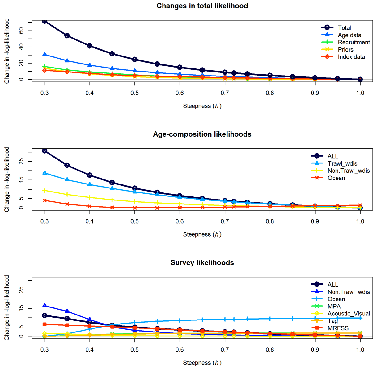
Figure 81: Beverton-Holt steepness parameter likelihood profile for each of the likelihood components.
