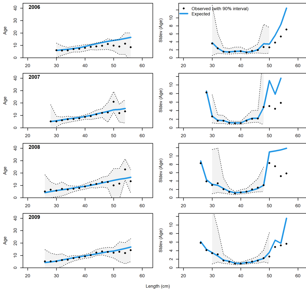
Figure 119: Non-trawl conditional AAL plot (plot 3 of 7).
