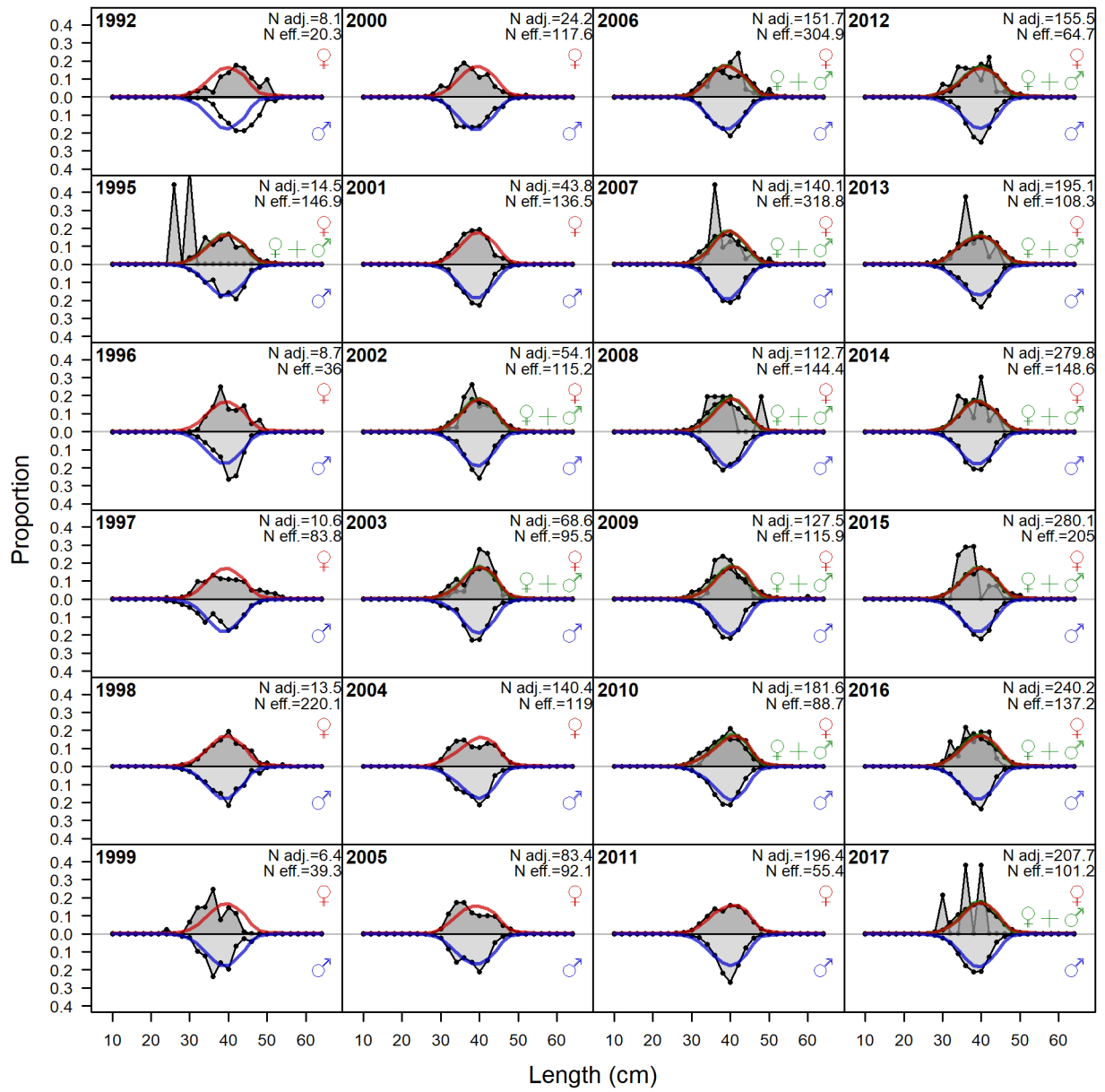
Figure 93: Length comps, whole catch, Non-Trawl_wdis (plot 1 of 2). 'N adj.' is the input sample size after data-weighting adjustment. N eff. is the calculated effective sample size used in the McAllister-Ianelli tuning method.
