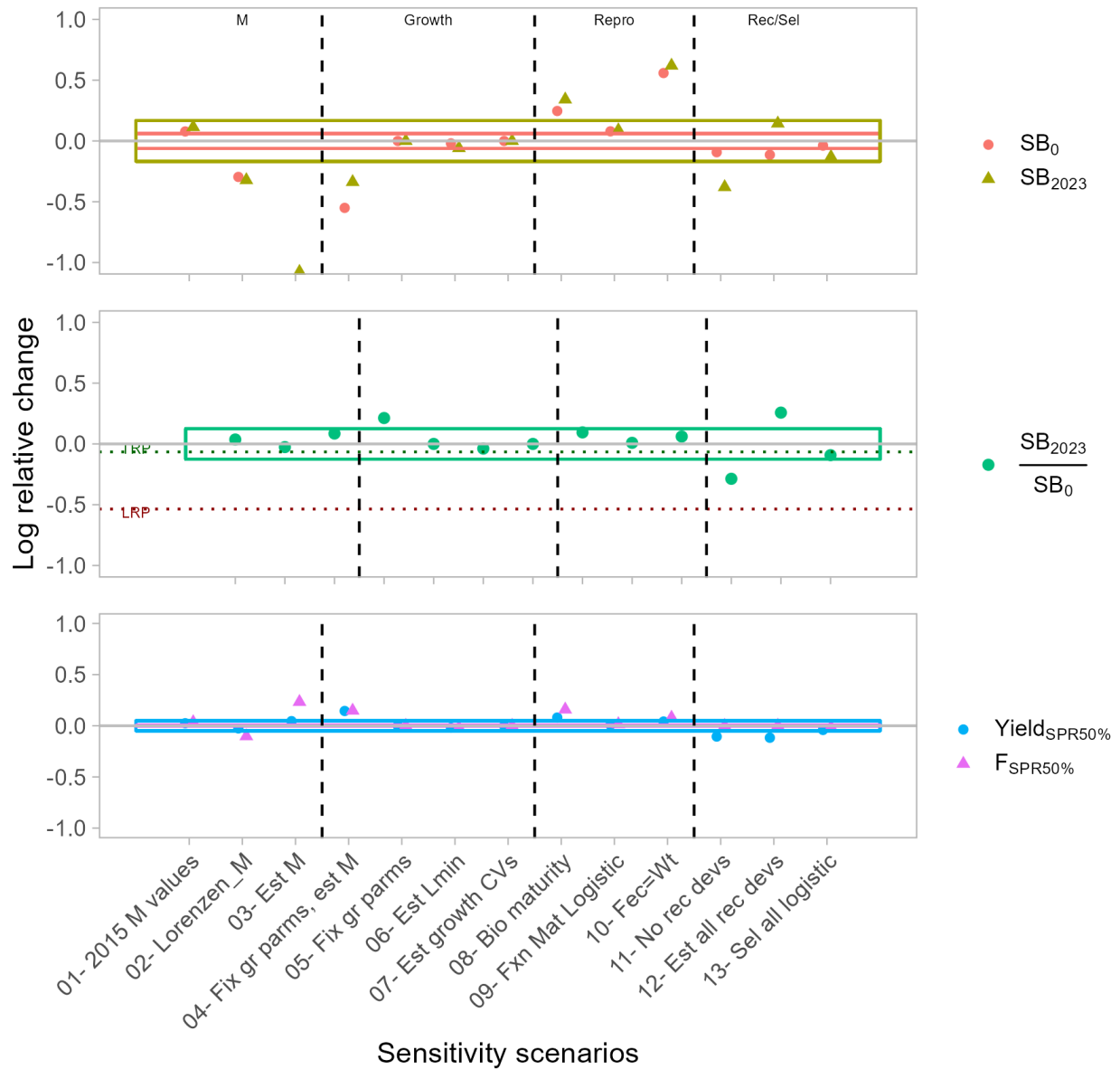
Figure 75: Log relative change ( \log((\text{Model\_sensi}-\text{Model\_ref})/\text{Model\_ref}) ) in model specification scenario for 5 derived quantities. Colored boxes indicate 95 percent confidence interval of the reference model. See ‘Sensitivity Analysis’ section for more details on each scenario.
