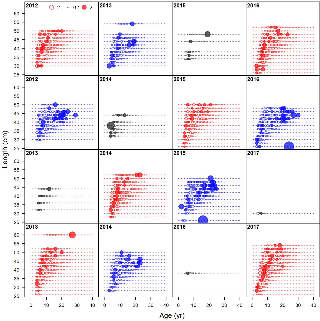
Figure 104: Pearson residuals, whole catch, Non-Trawl_wdis (max=10.69) (plot 3 of 5).
