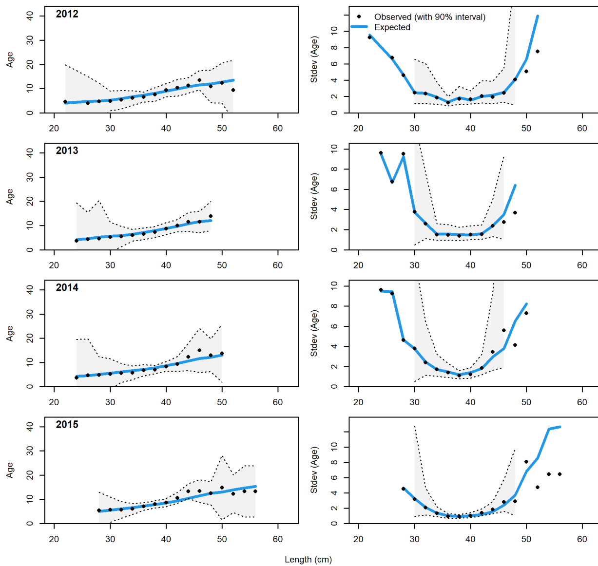
Figure 127: Ocean boat conditional AAL plot (plot 3 of 6).
