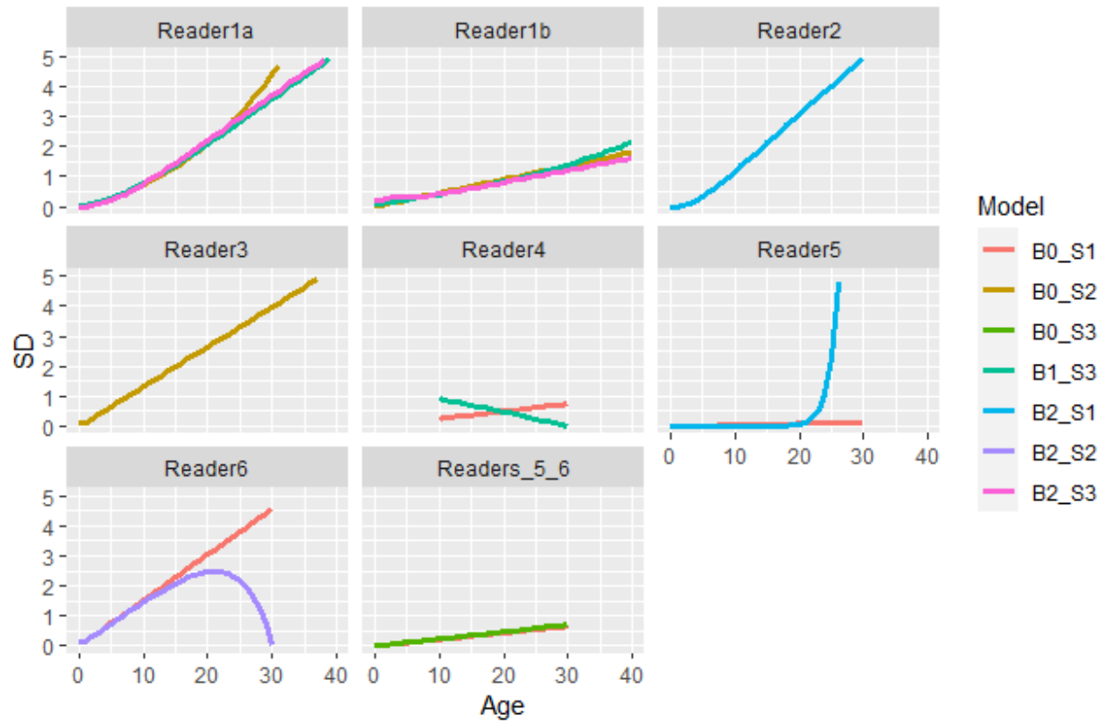
Figure 13: Ageing error matrix standard deviation (SD) values by comparison. B refers to the bias type and S refers to the imprecision type in the model selection for the ageing error matrix.
