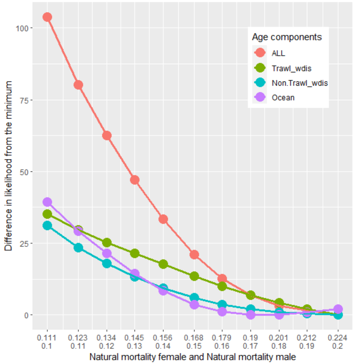
Figure 41: Age likelihood component values for the female and male M multi-parameter likelihood profile.
