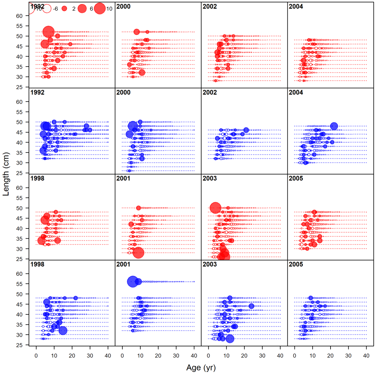
Figure 102: Pearson residuals, whole catch, Non-Trawl_wdis (max=10.69) (plot 1 of 5).
