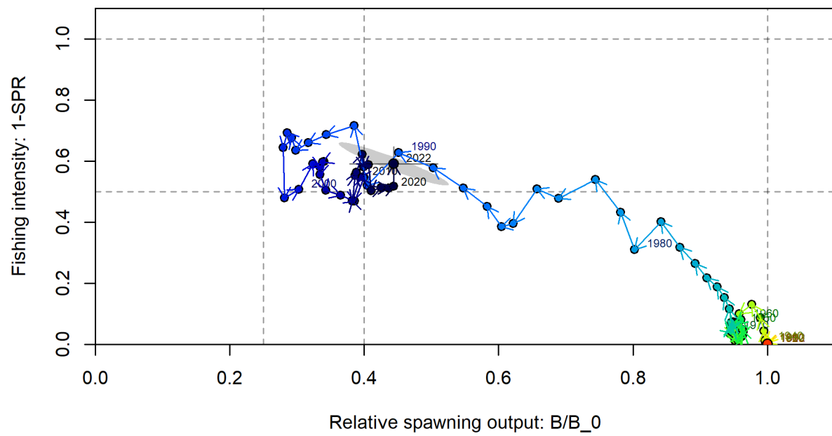
Figure vi: Phase plot of estimated 1-SPR versus fraction unfished for the reference model.
