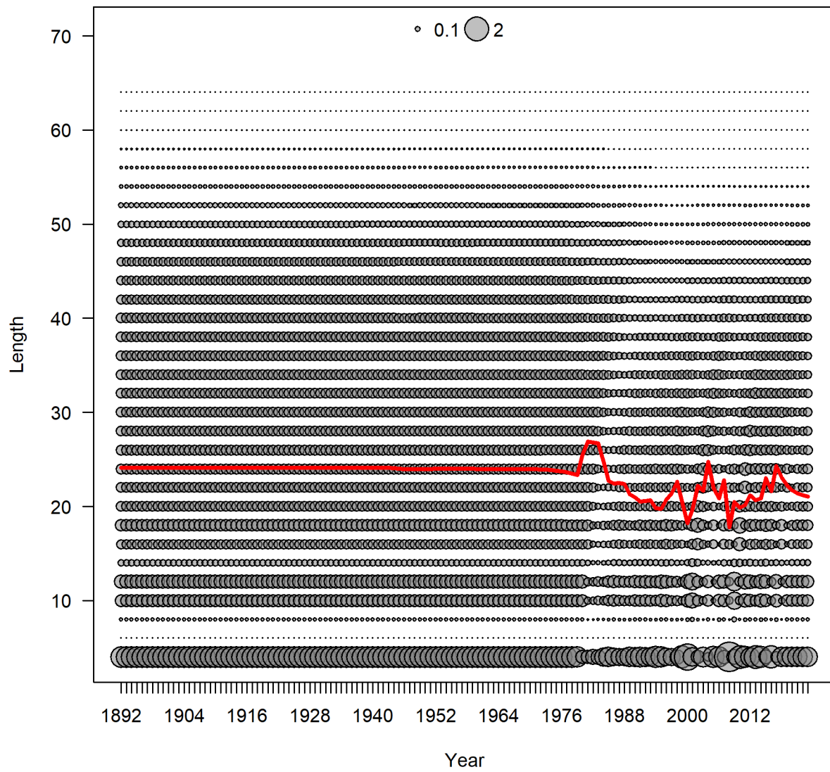
Figure 132: Female black rockfish mean length (cm) over time.
