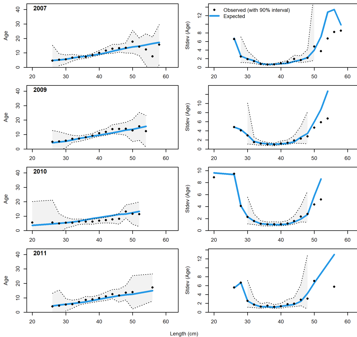
Figure 126: Ocean boat conditional AAL plot (plot 2 of 6).
