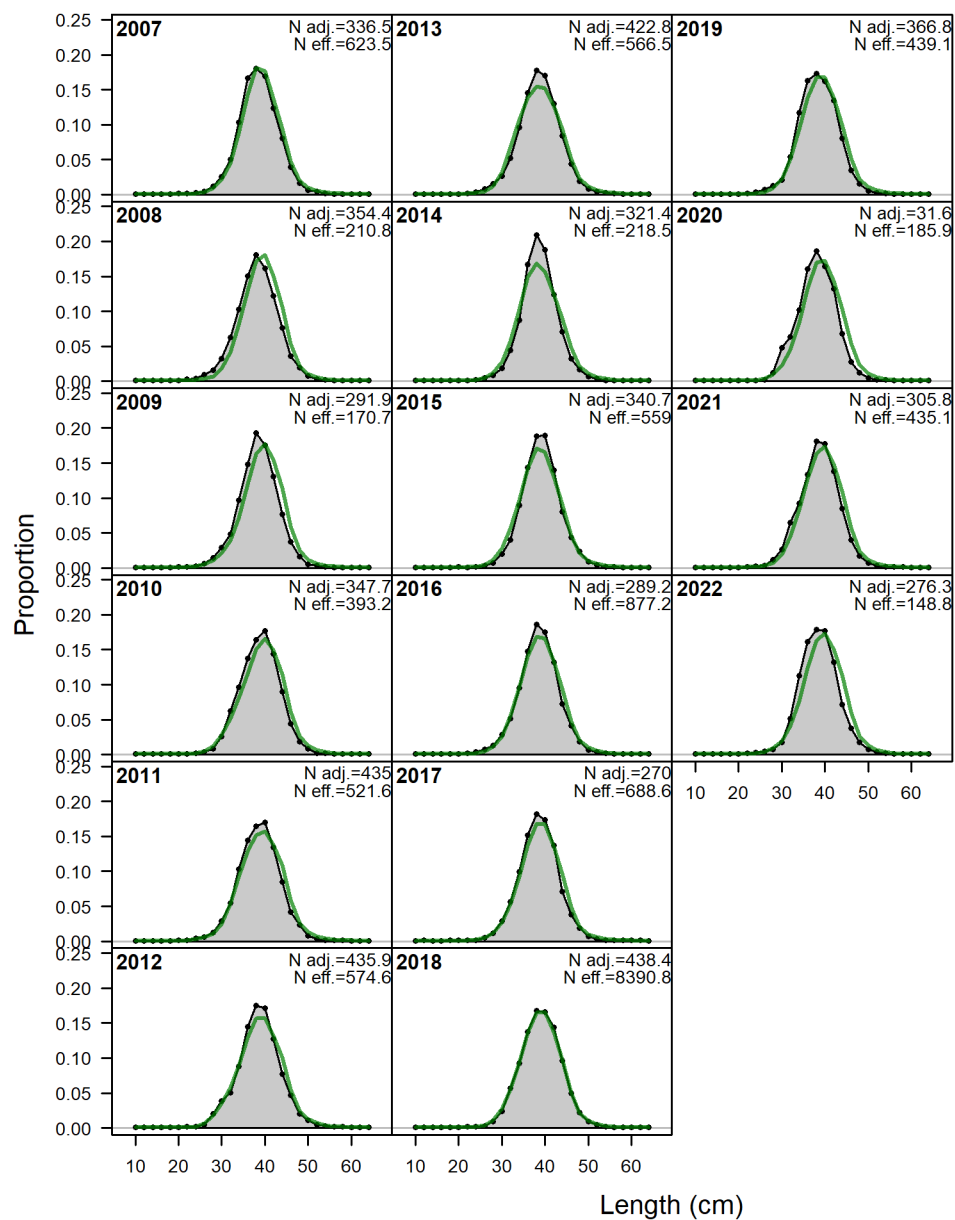
Figure 96: Length comps, whole catch, Ocean (plot 1 of 2): 'N adj.' is the input sample size after data-weighting adjustment. N eff. is the calculated effective sample size used in the McAllister-Ianelli tuning method. (plot 2 of 2).
