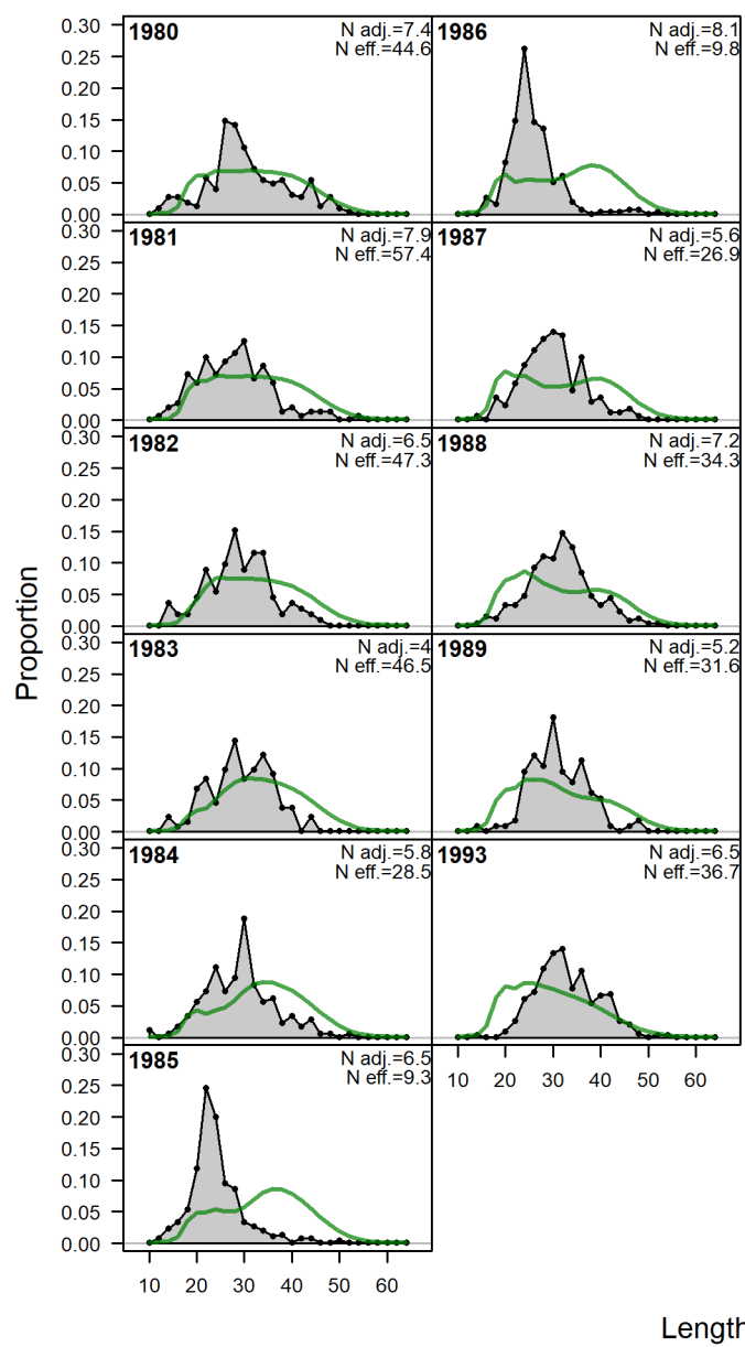
Figure 97: Length comps, whole catch, Shore. 'N adj.' is the input sample size after data-weighting adjustment. N eff. is the calculated effective sample size used in the McAllister-Ianelli tuning method.
