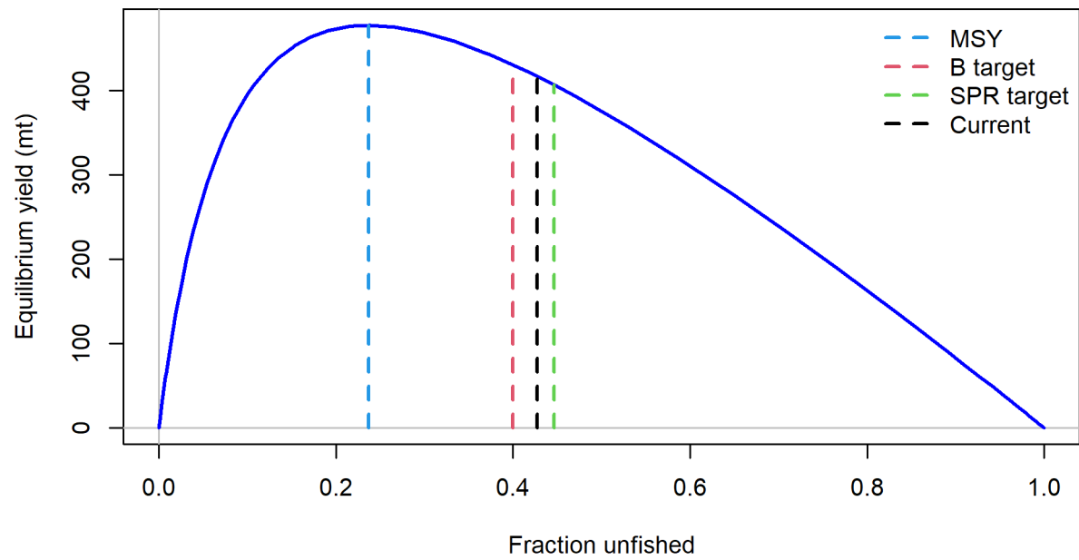
Figure vii: Equilibrium yield curve for the reference model. Values are based on (the time invariant) fishery selectivities and with steepness fixed at 0.72.
