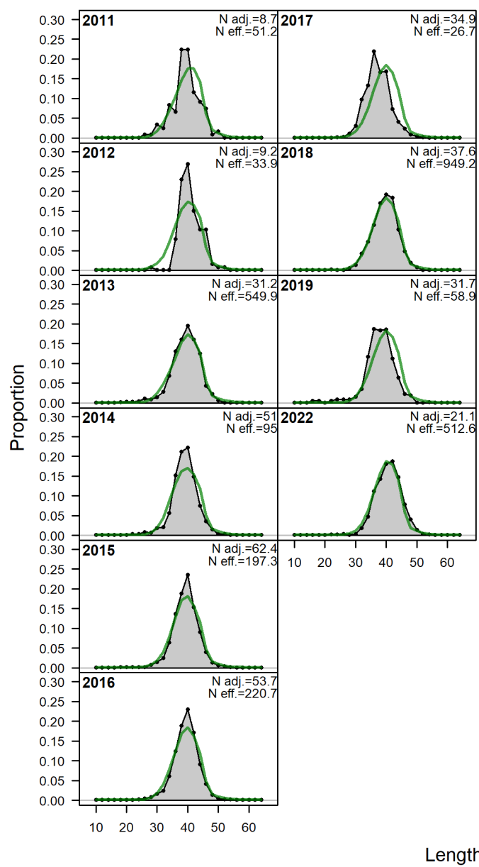
Figure 98: Length comps, whole catch, MPA: 'N adj.' is the input sample size after data-weighting adjustment. N eff. is the calculated effective sample size used in the McAllister-Ianelli tuning method.
