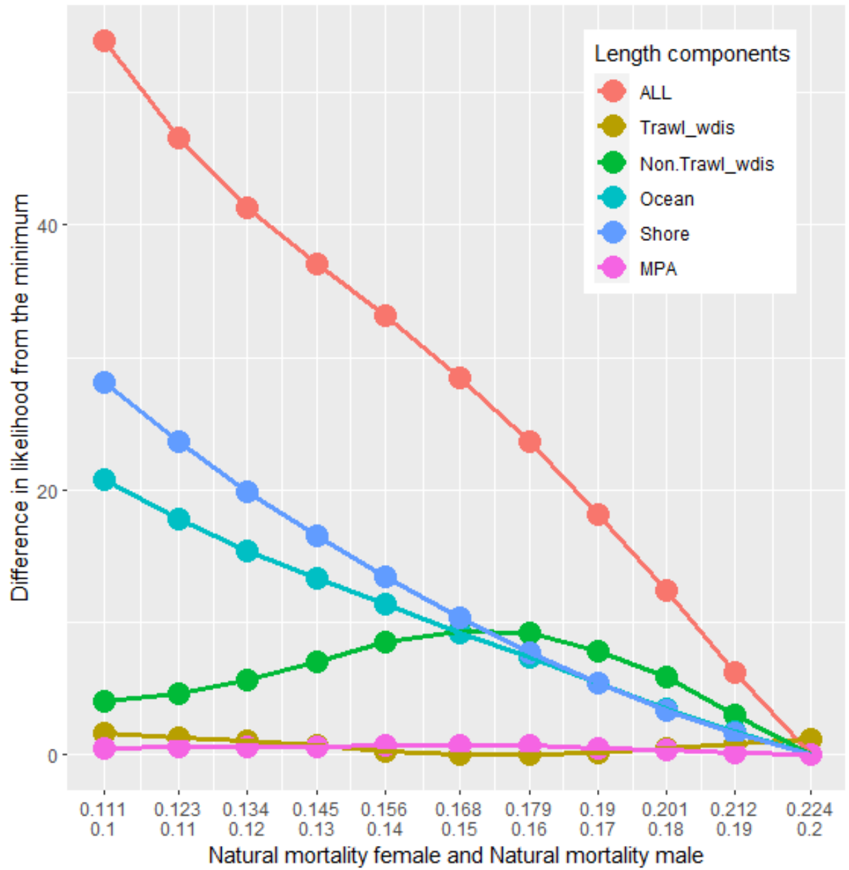
Figure 40: Length likelihood component values for the female and male M multi-parameter likelihood profile.
