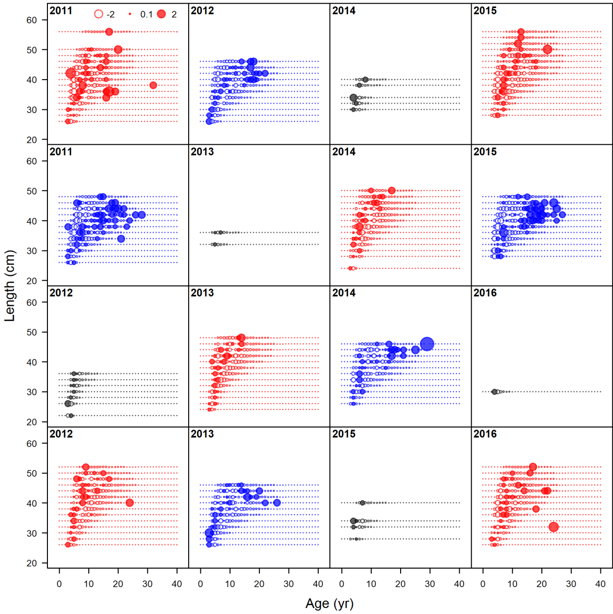
Figure 109: Pearson residuals, whole catch, Ocean (max=95.66) (plot 3 of 5).
