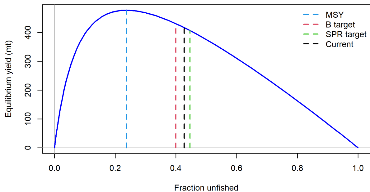
Figure 89: Equilibrium yield curve for the reference model. Values are based on the 2020 fishery selectivities and with steepness fixed at 0.72.
