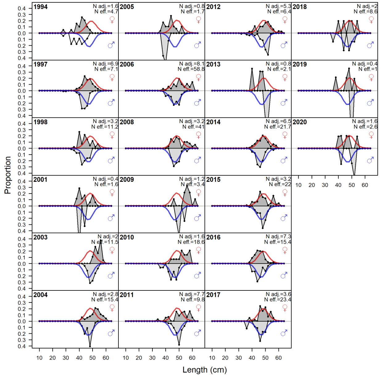
Figure 92: Length comps, whole catch, Trawl_wdis. 'N adj.' is the input sample size after data-weighting adjustment. N eff. is the calculated effective sample size used in the McAllister-Ianelli tuning method.
