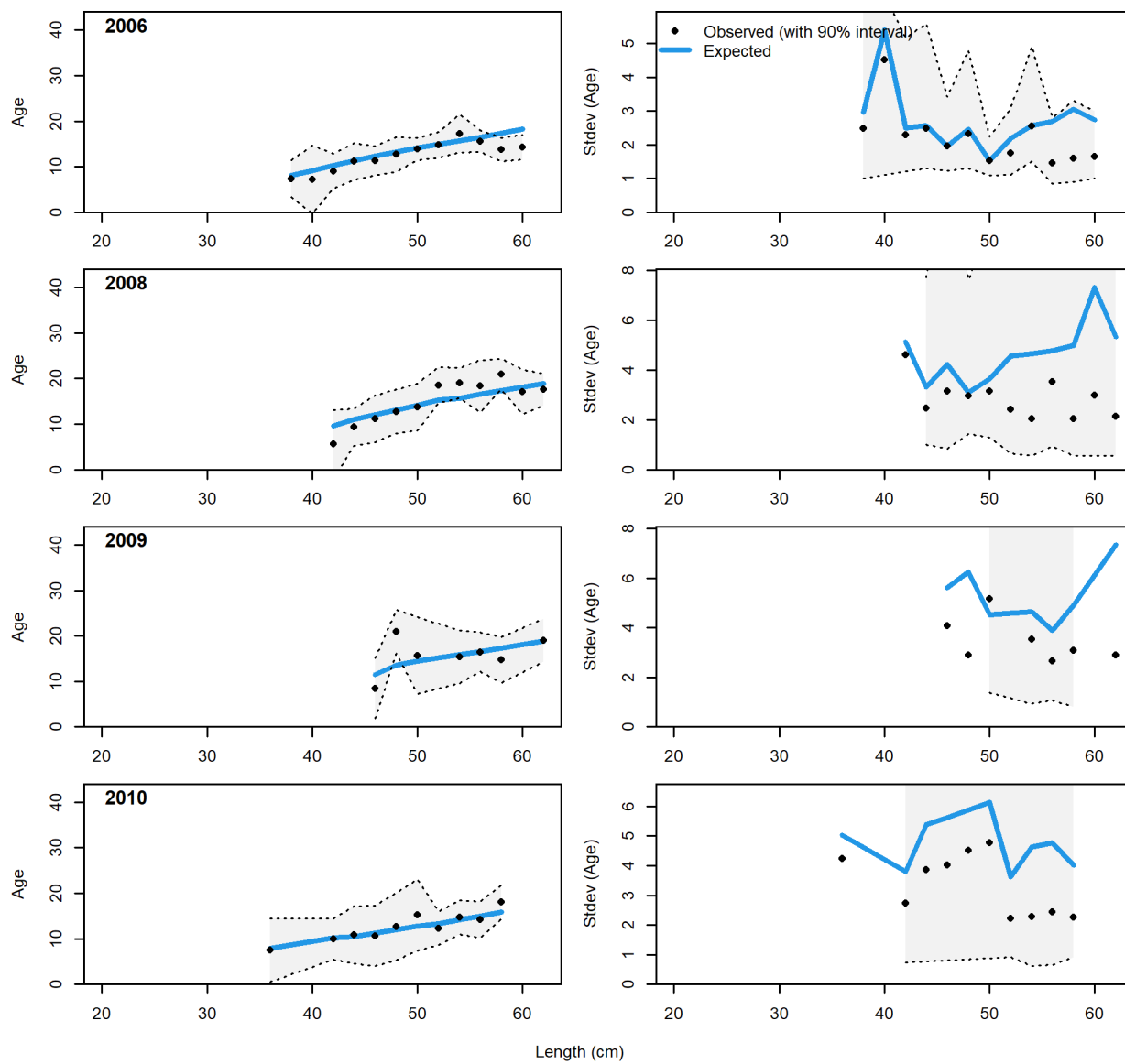
Figure 113: Trawl conditional AAL plot (plot 2 of 5).
