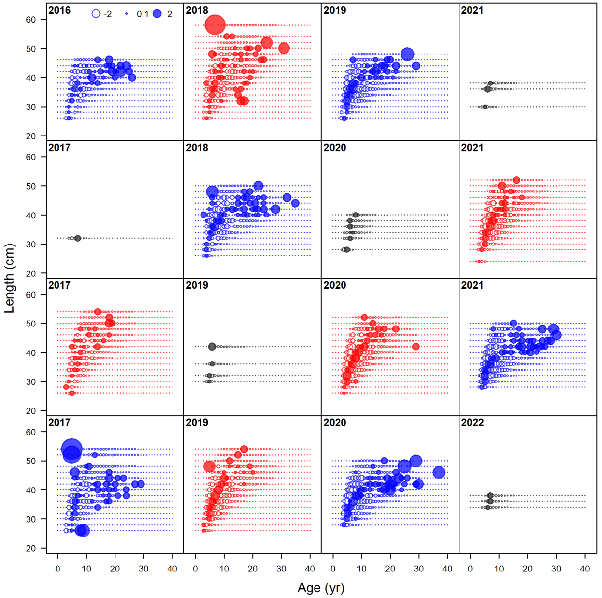
Figure 110: Pearson residuals, whole catch, Ocean (max=95.66) (plot 4 of 5).
