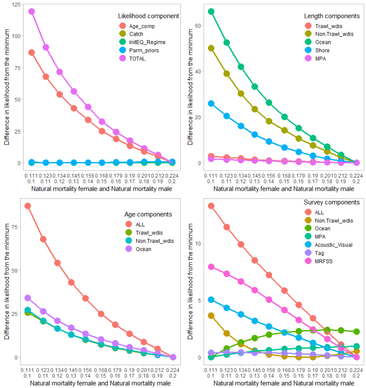
Figure 83: Likelihood values by component and within components for the female and male M multi-parameter likelihood profile.
