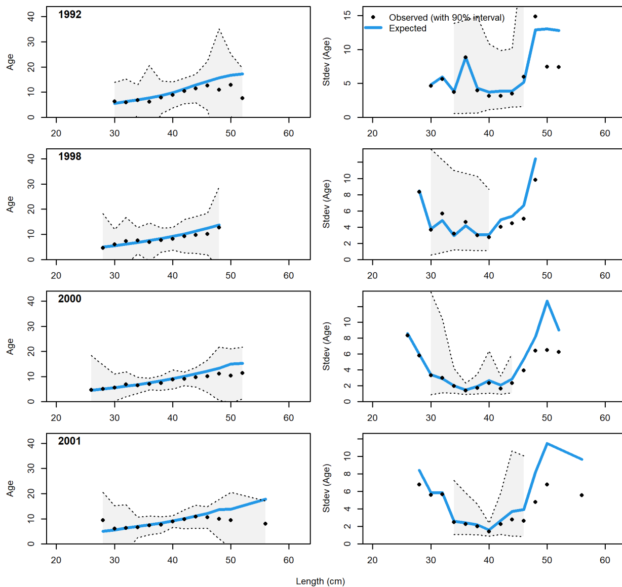
Figure 117: Non-trawl conditional AAL plot (plot 1 of 7) showing mean age (left panel) and standard deviation (right panel). Shaded areas are 90 percent CIs).
