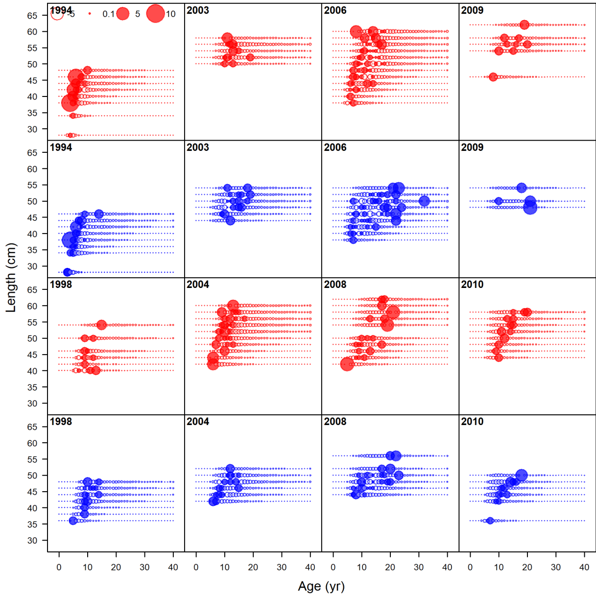
Figure 99: Pearson residuals, whole catch, Trawl_wdis (max=13.1) (plot 1 of 3).
