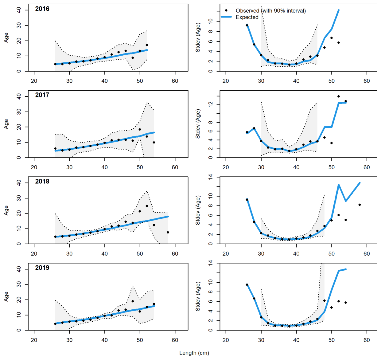
Figure 128: Ocean boat conditional AAL plot (plot 3 of 6).
