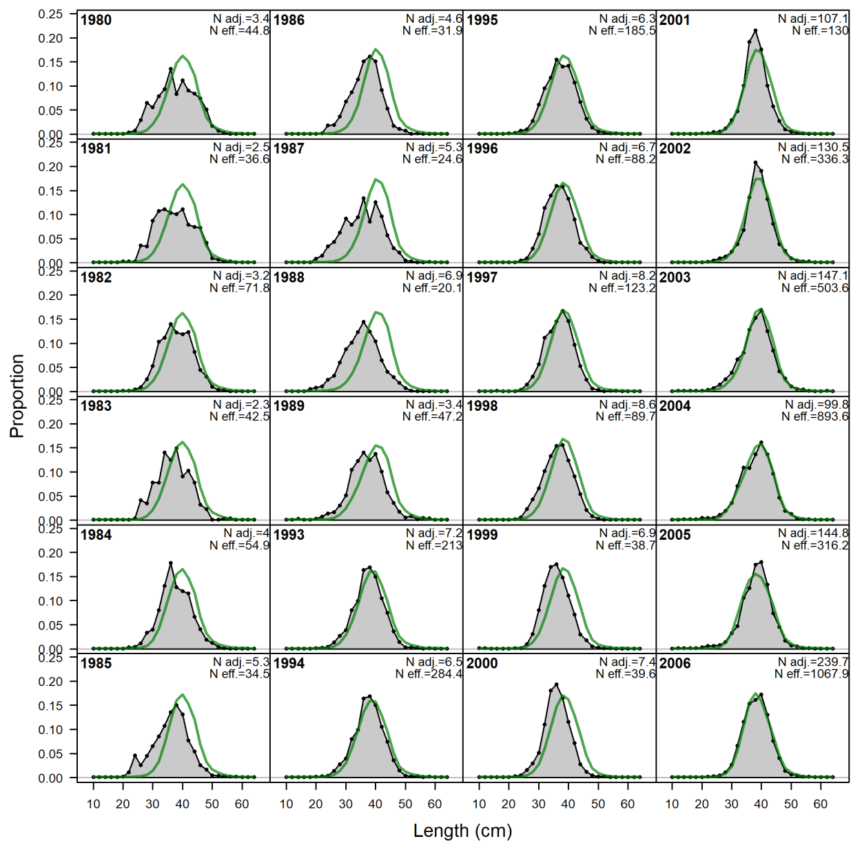
Figure 95: Length comps, whole catch, Ocean (plot 1 of 2):'N adj.' is the input sample size after data-weighting adjustment. N eff. is the calculated effective sample size used in the McAllister-Ianelli tuning method.
