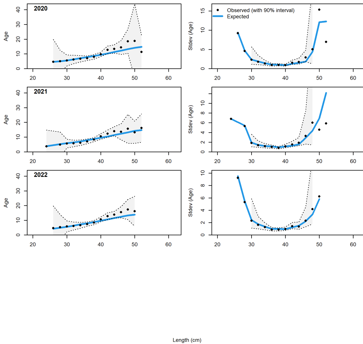
Figure 129: Ocean boat conditional AAL plot (plot 4 of 6).
