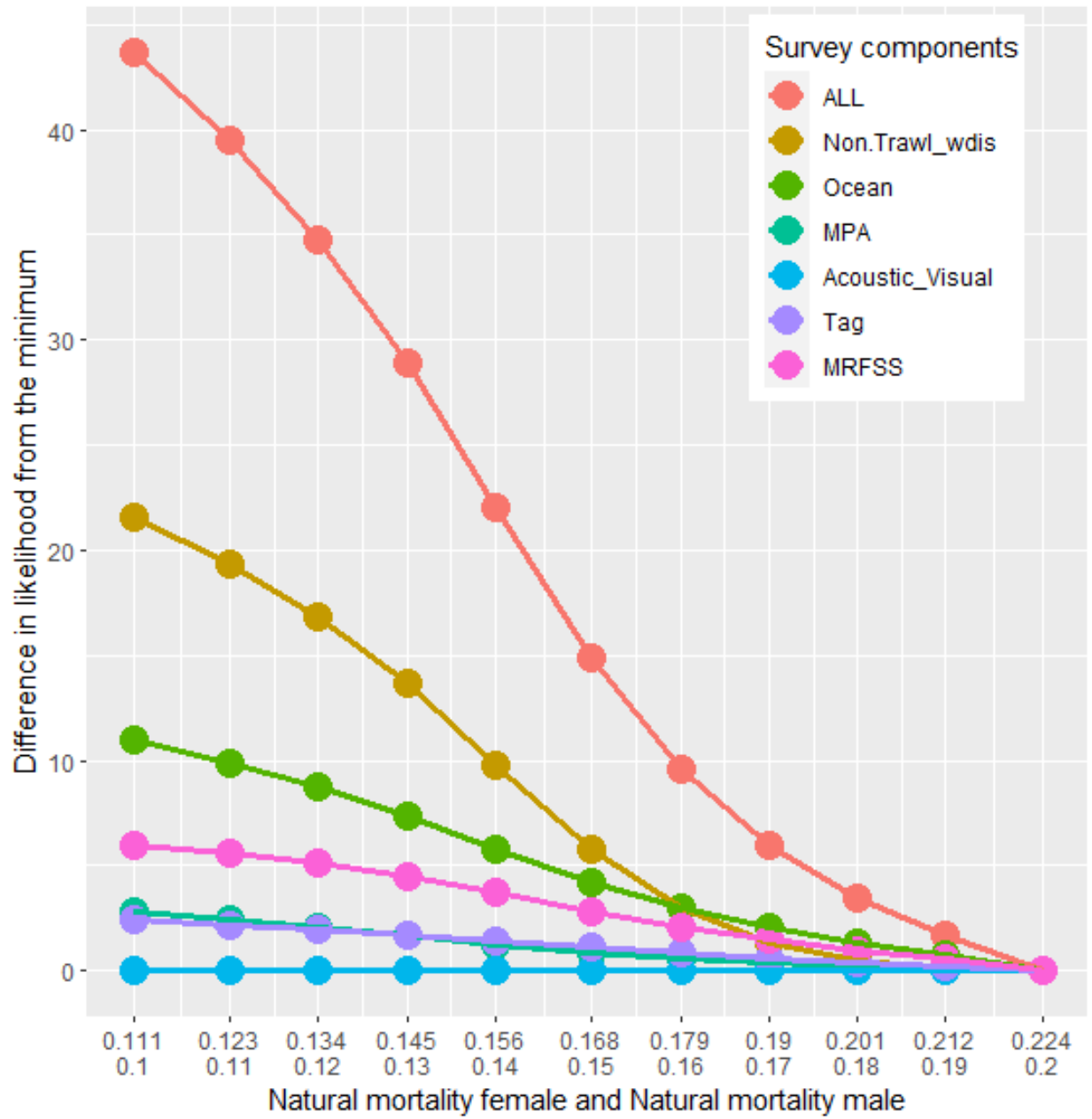
Figure 42: Survey likelihood component values for the female and male M multi-parameter likelihood profile.
