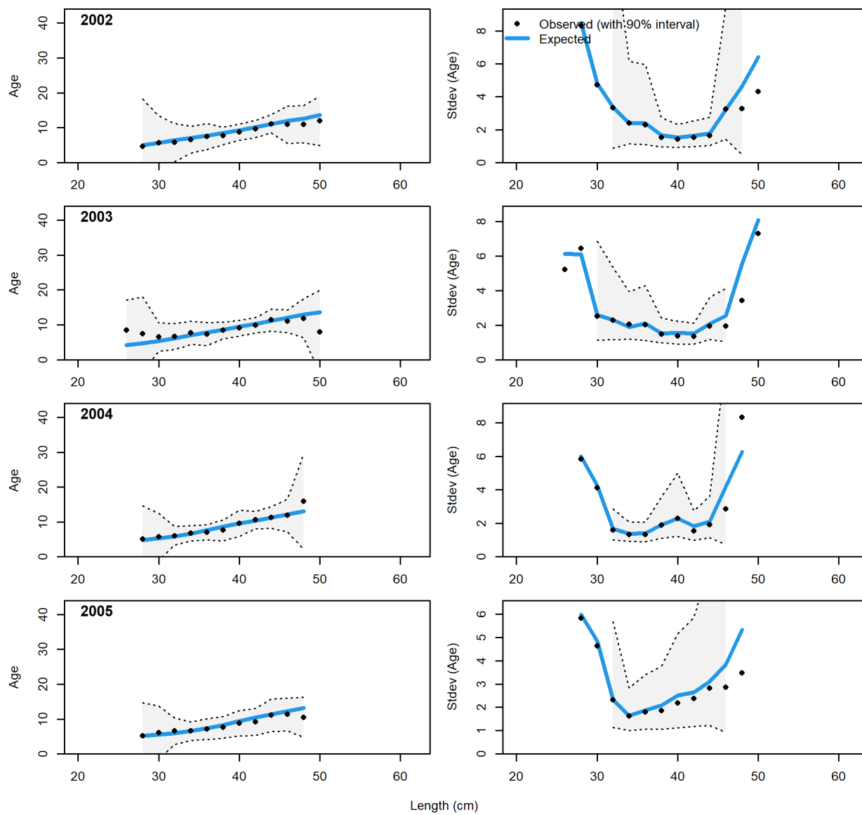
Figure 118: Non-trawl conditional AAL plot (plot 2 of 7).
