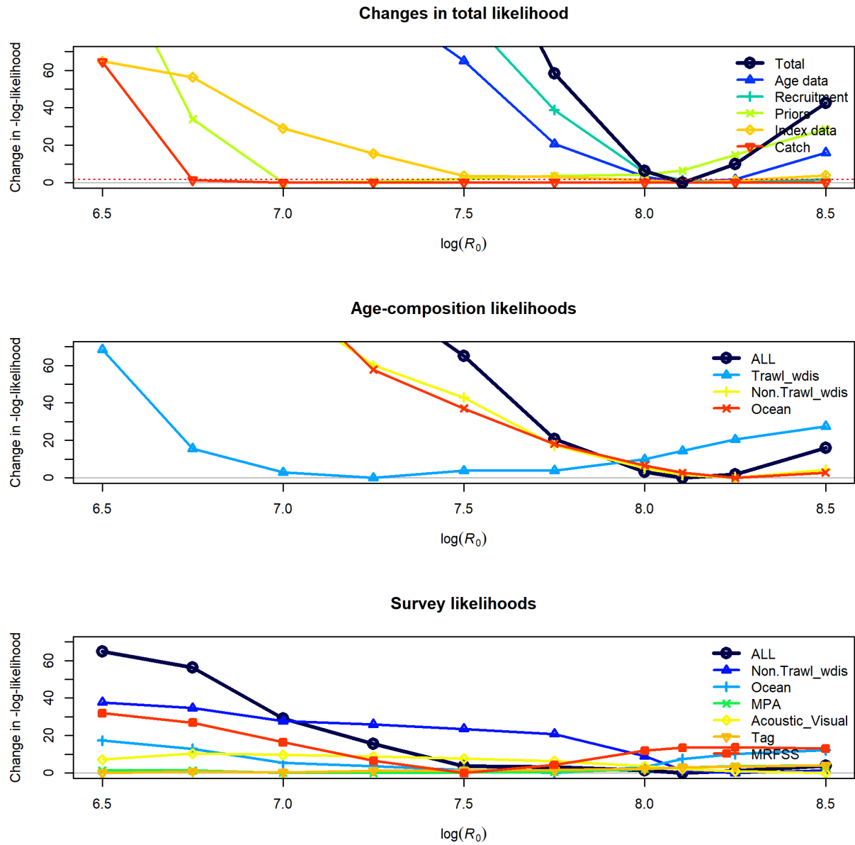
Figure 79: Initial recruitment ( \ln(R_0) ) likelihood profile for each of the likelihood components.
