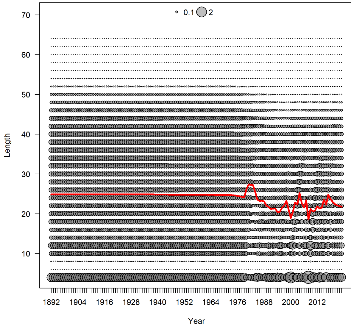
Figure 133: Male black rockfish mean length over time.
