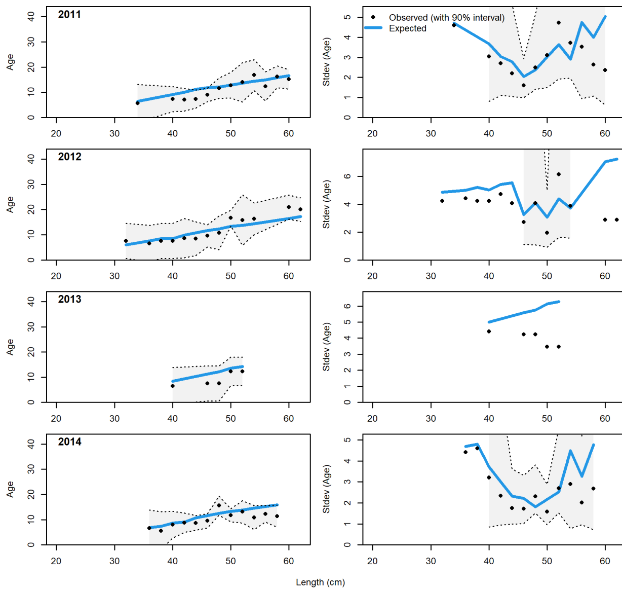
Figure 114: Trawl conditional AAL plot (plot 3 of 5).
