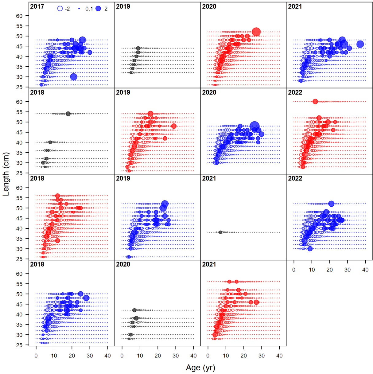
Figure 105: Pearson residuals, whole catch, Non-Trawl_wdis (max=10.69) (plot 4 of 5).
