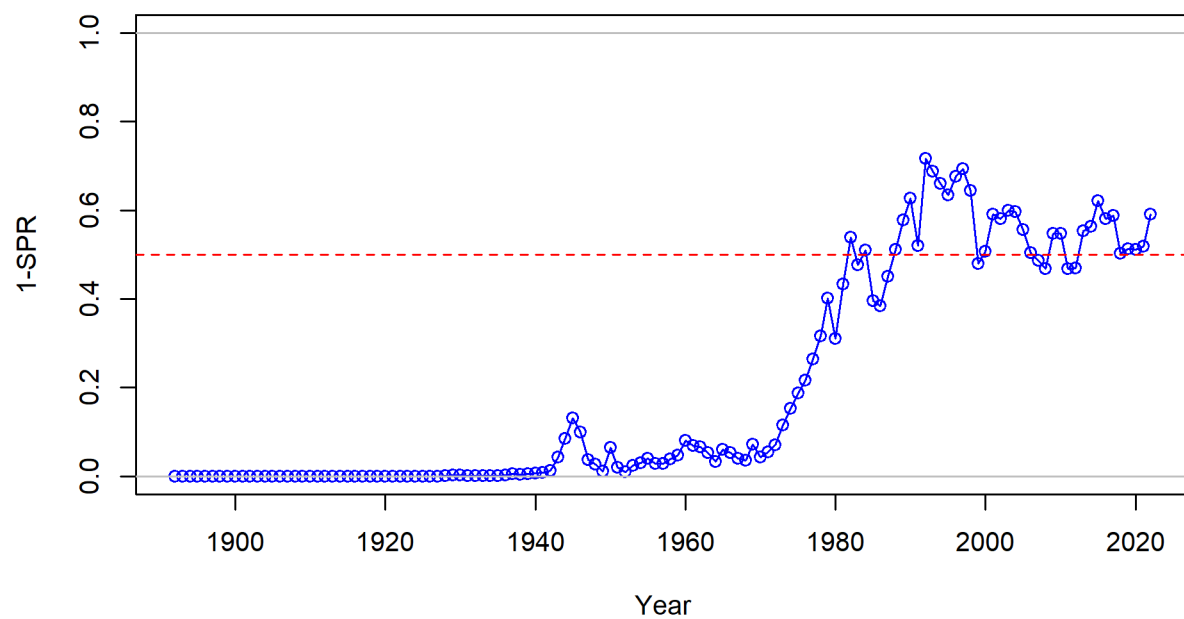
Figure v: Estimated 1 - relative spawning ratio (SPR) by year for the reference model. The management target is plotted as a red horizontal line and values above this reflect harvest in excess of the proxy harvest rate.
