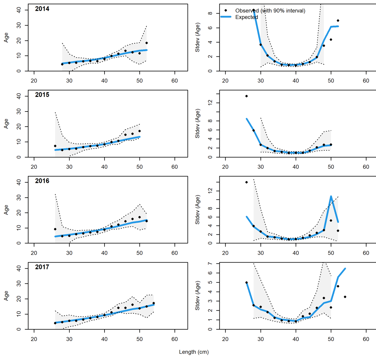
Figure 121: Non-trawl conditional AAL plot (plot 4 of 7).
