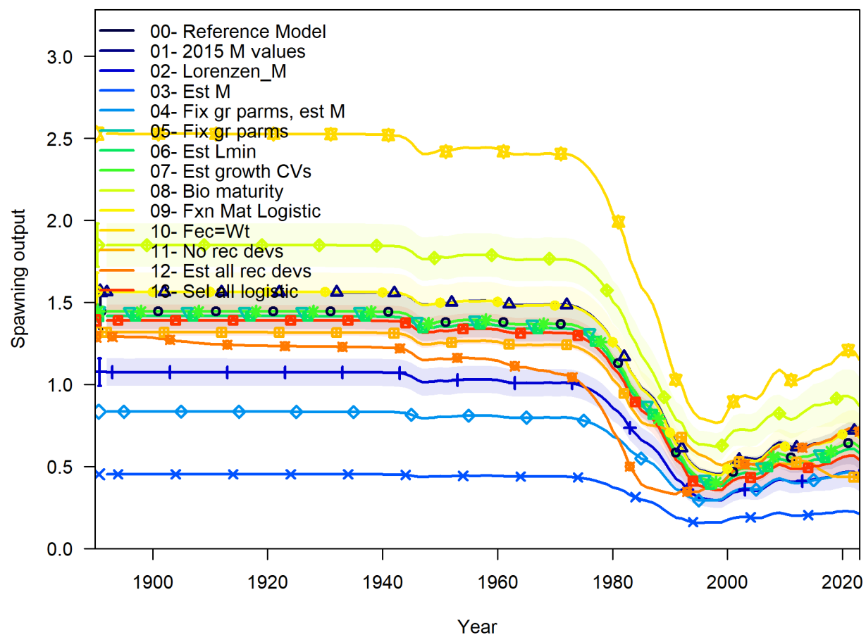
Figure 76: Spawning output (in millions of eggs) time series by model specification scenario compared to the reference model. See ‘Sensitivity Analysis’ section for more details on each scenario.
