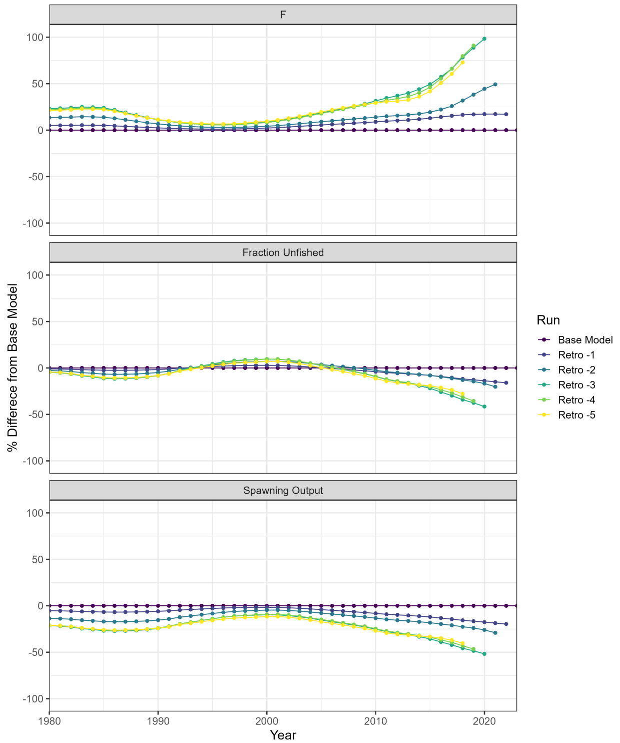
Figure 86: Relative error from the reference model for each of the 5 data peels in the retrospective analysis for 3 derived outputs.
