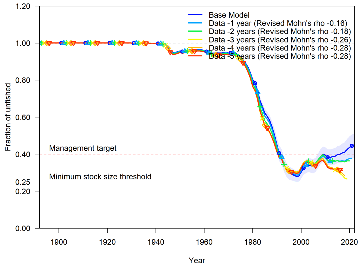
Figure 85: Change in the estimate of fraction unfished when the most recent 5 years of data area removed sequentially.
