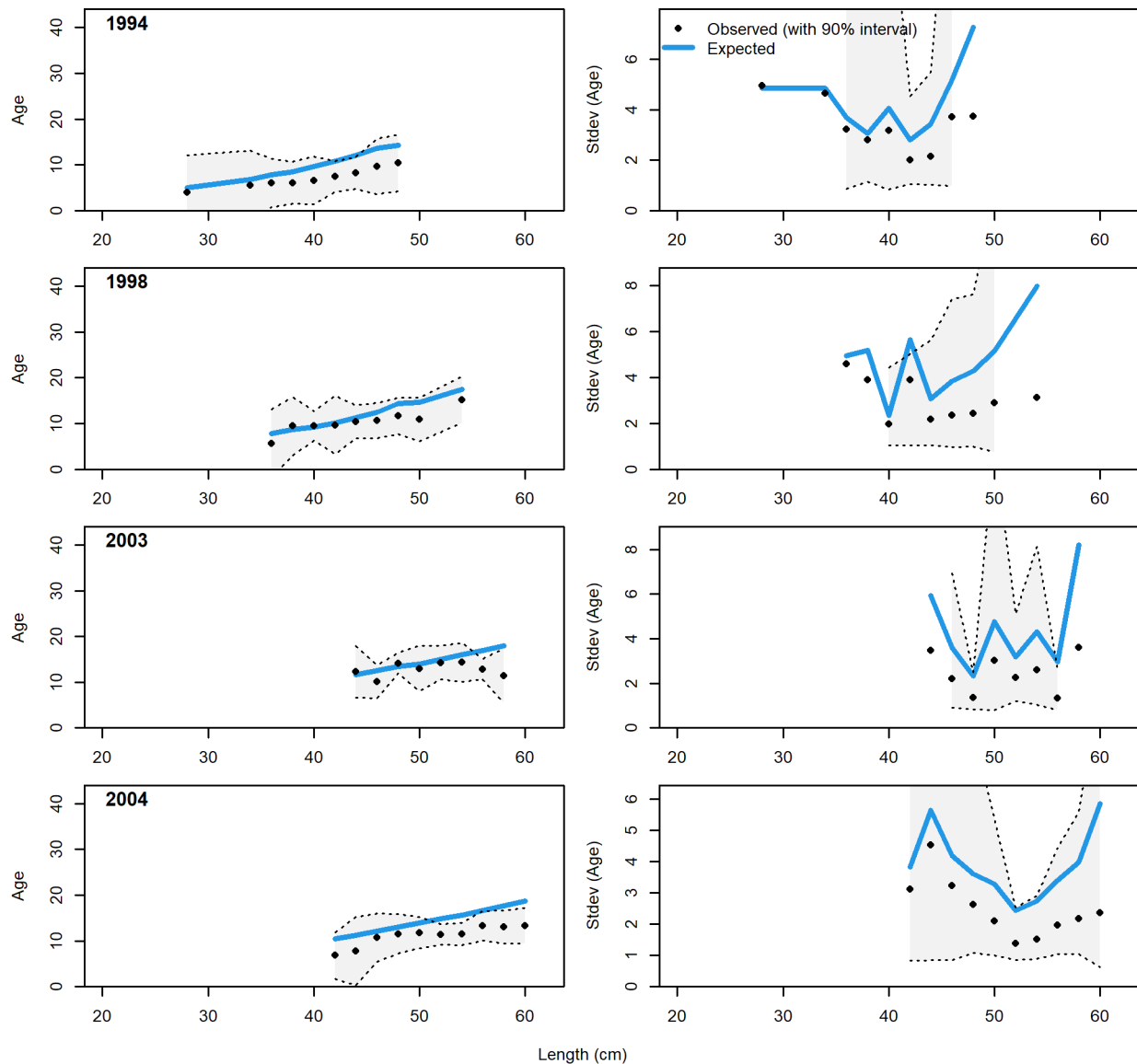
Figure 112: Trawl conditional AAL plot (plot 1 of 5) showing mean age (left panel) and standard deviation (right panel. Shaded areas are 90 percent CIs).
