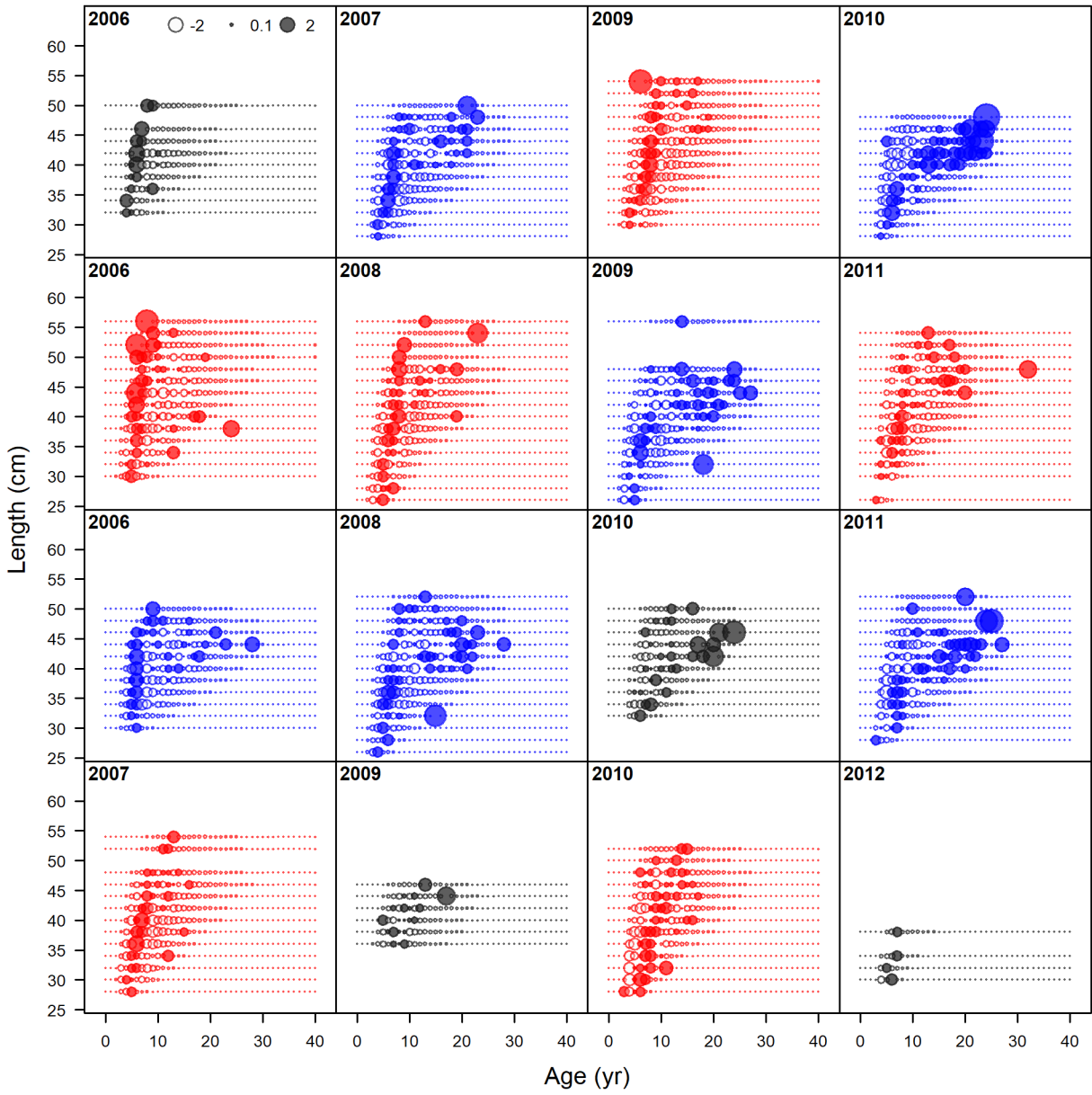
Figure 103: Pearson residuals, whole catch, Non-Trawl_wdis (max=10.69) (plot 2 of 5).
