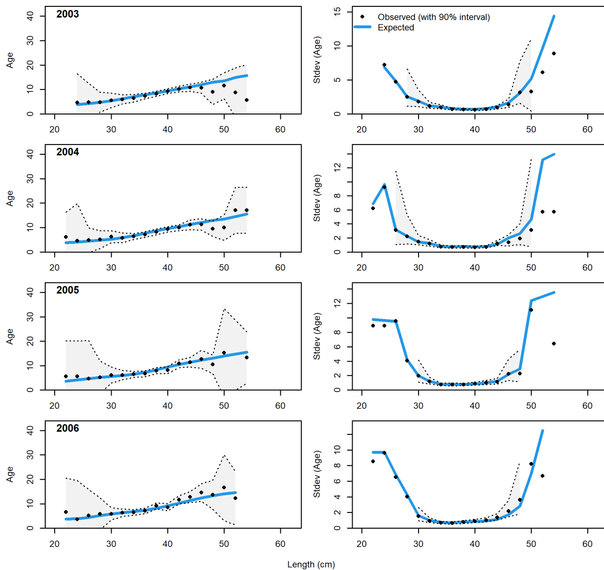
Figure 125: Ocean boat conditional AAL plot (plot 1 of 6) showing mean age (left panel) and standard deviation (right panel). Shaded areas are 90 percent CIs).
