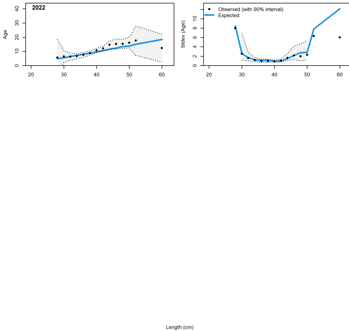
Figure 123: Non-trawl conditional AAL plot (plot 6 of 7).
