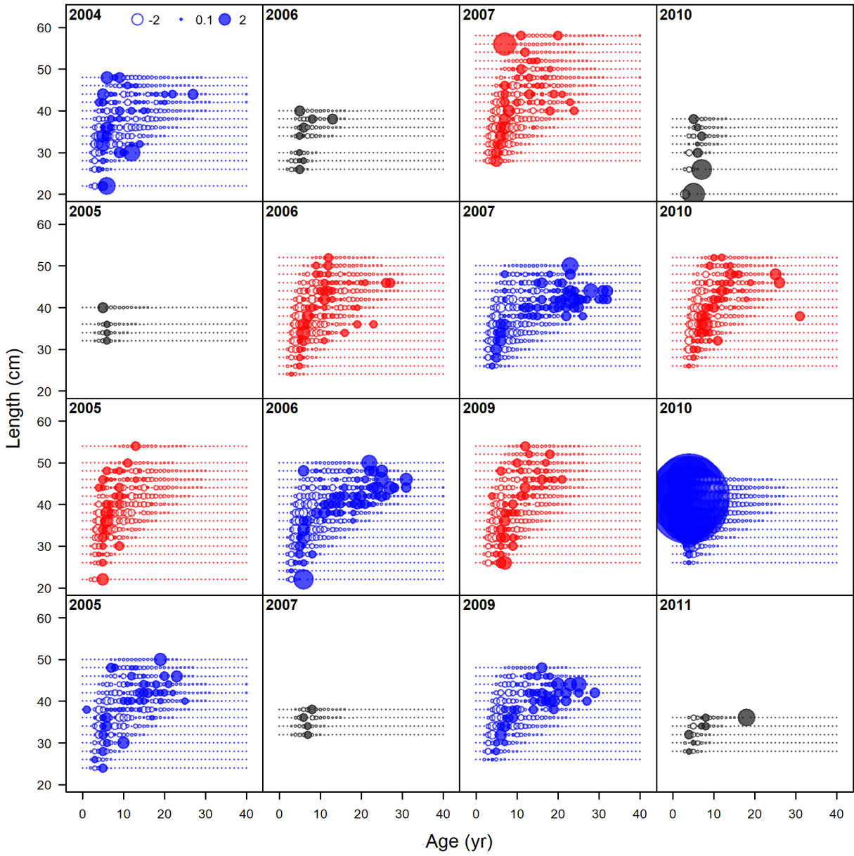
Figure 108: Pearson residuals, whole catch, Ocean (max=95.66) (plot 2 of 5).
