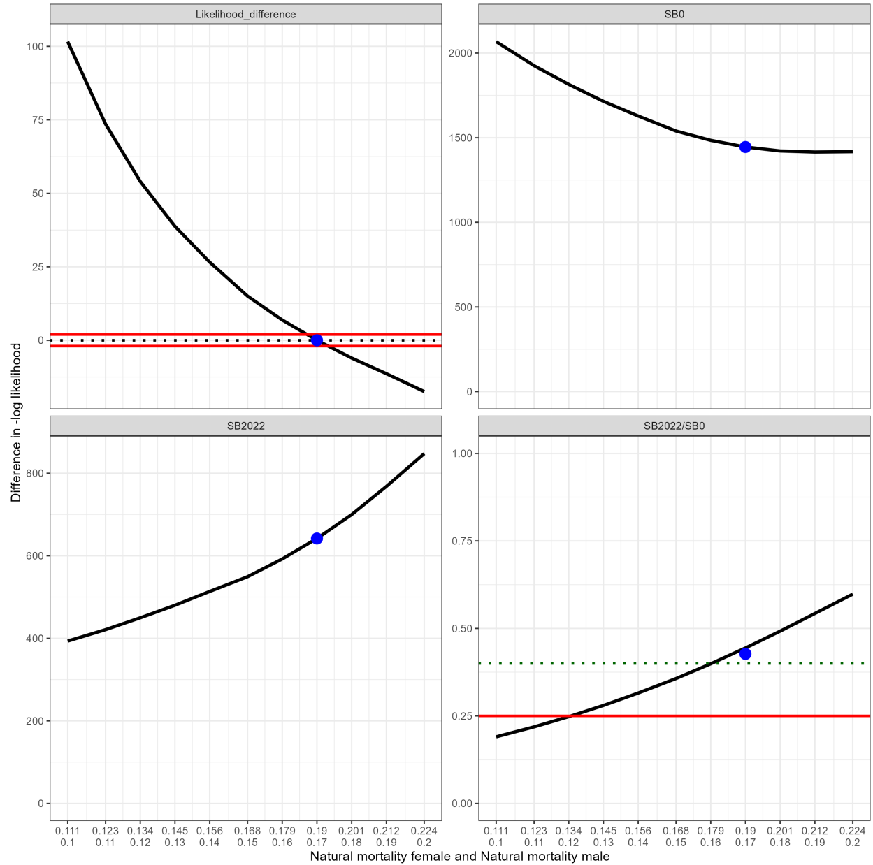
Figure 82: Female and male M multi-parameter likelihood profile and derived quantities. Red lines in the top left figure indicate significantly similar values compared to the reference model. Broken and solid lines in the bottom right figure indicate target and limit reference points, respectively.
