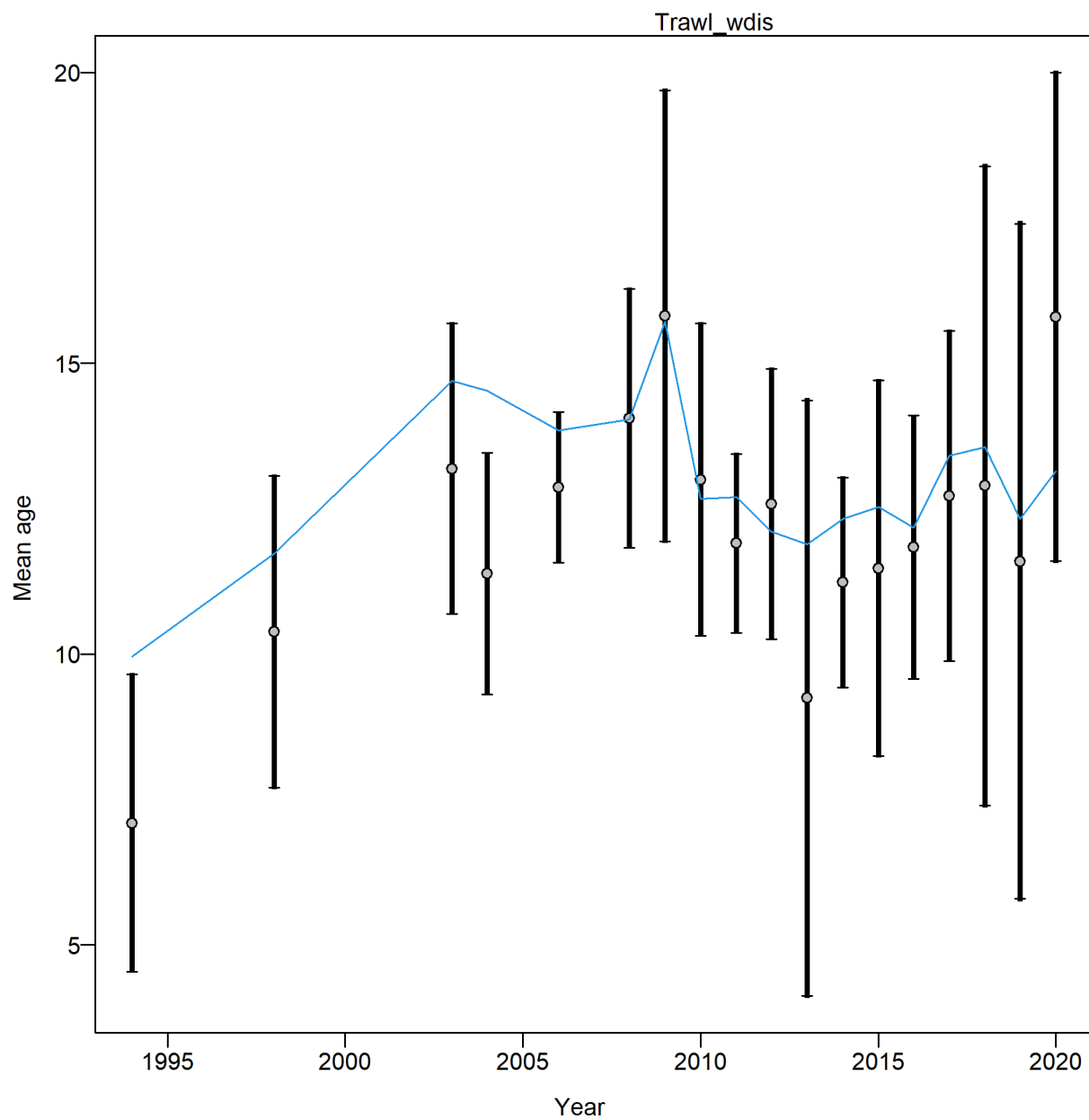
Figure 52: Mean age from conditional age-at-length data for the commercial trawl fishery.
