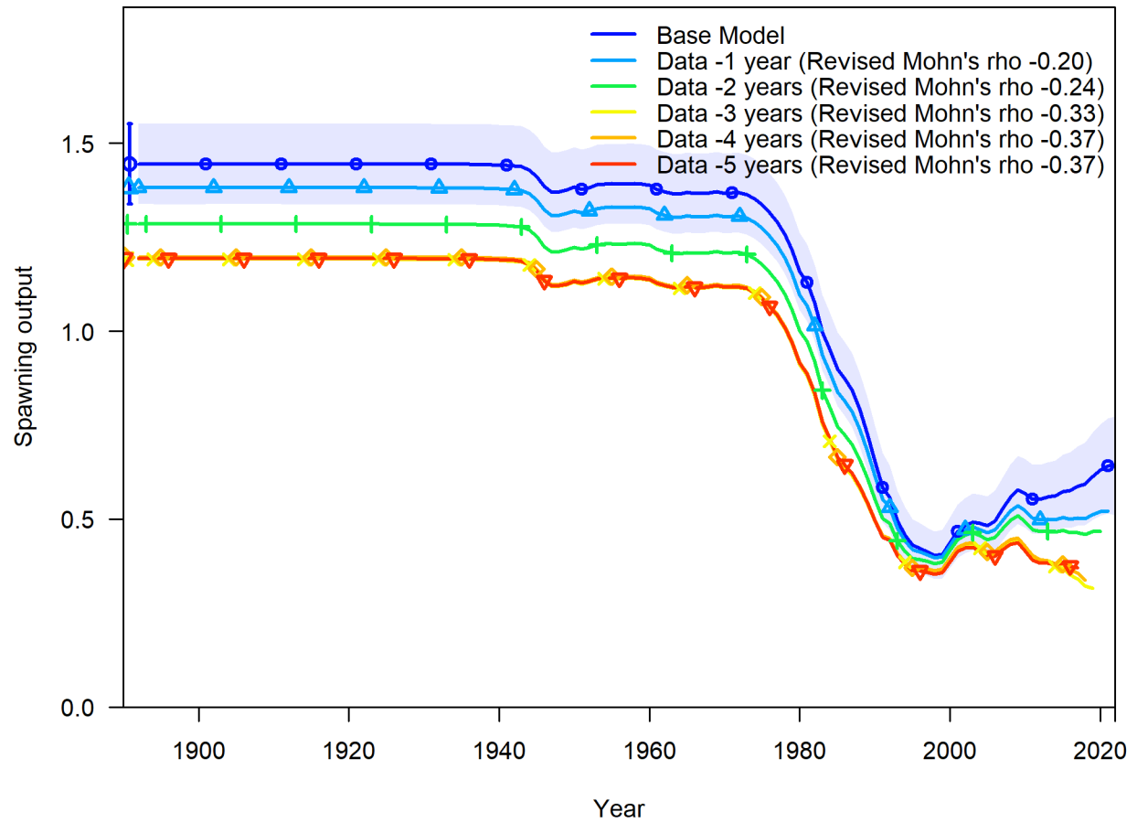
Figure 84: Change in the estimate of spawning output when the most recent 5 years of data area removed sequentially.
