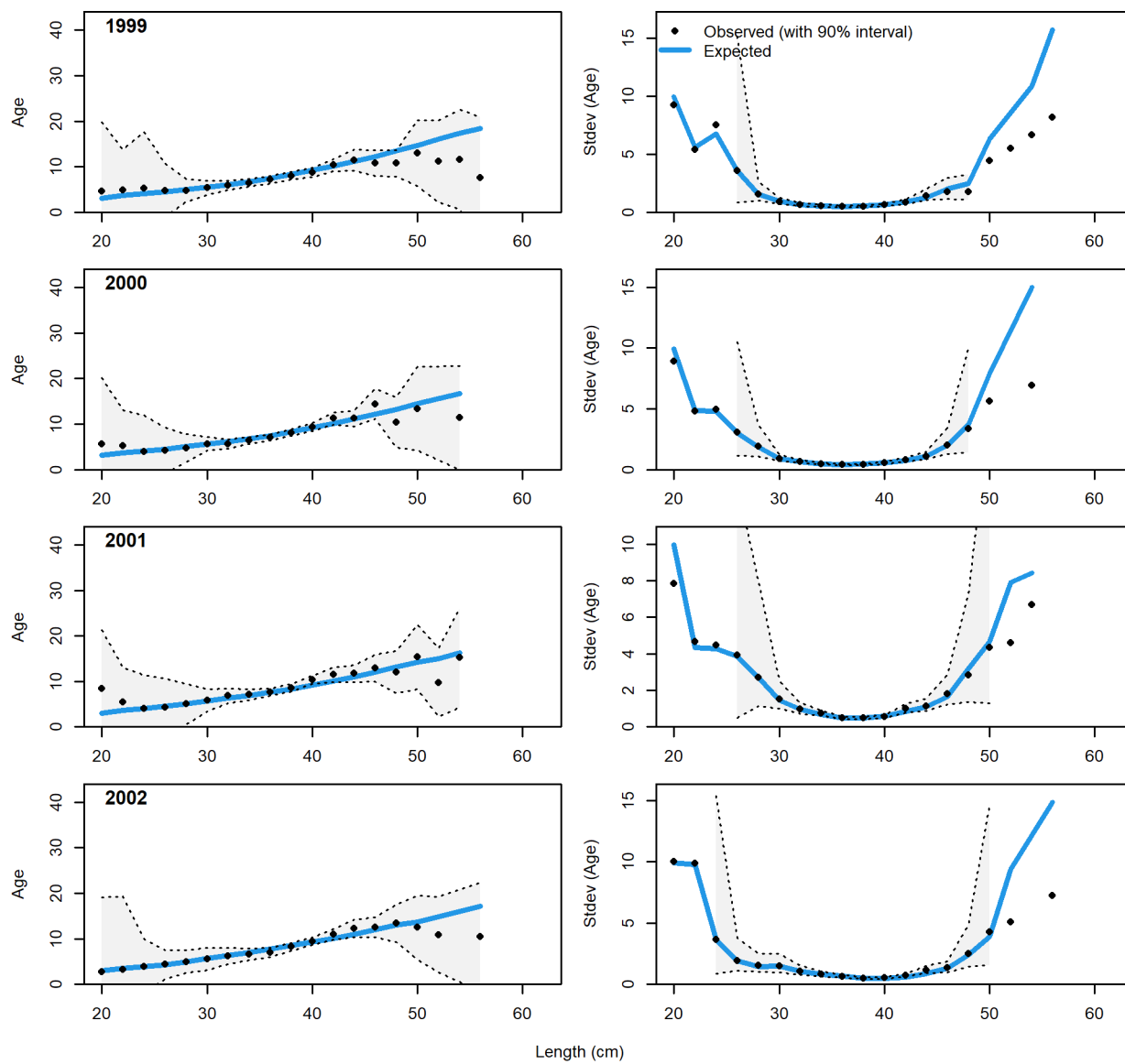
Figure 124: Non-trawl conditional AAL plot (plot 7 of 7).
