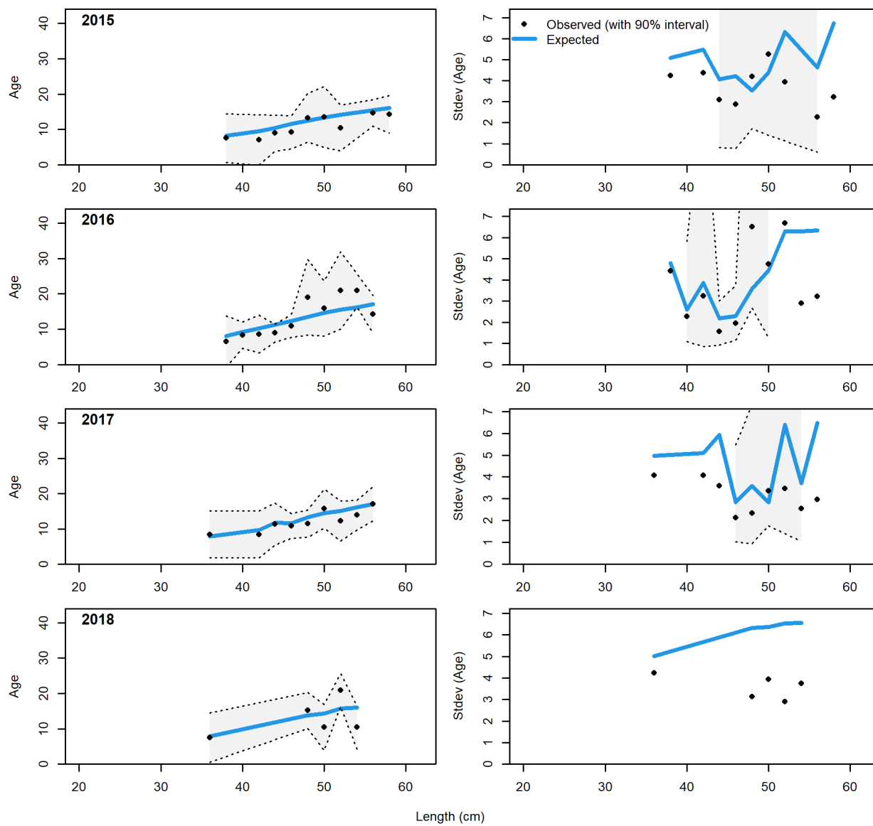
Figure 115: Trawl' conditional AAL plot (plot 4 of 5).
