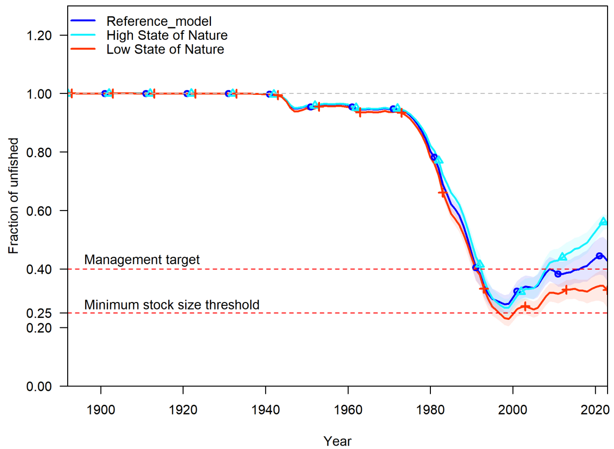
Figure 91: Time series of relative stock status (with 95% uncertainty envelopes) for three states of nature, based on the treatment of the acoustic visual survey catchability, of Oregon black rockfish.
