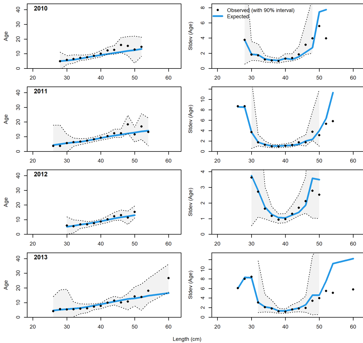
Figure 120: Non-trawl conditional AAL plot (plot 3 of 7).
