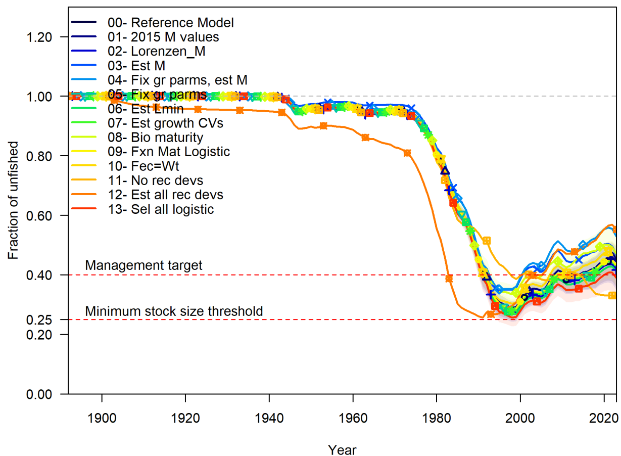
Figure 77: Relative spawning output time series by model specification scenario compared to the reference model. See ‘Sensitivity Analysis’ section for more details on each scenario.
