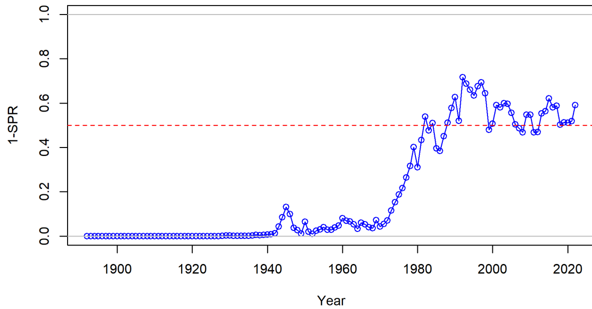
Figure 87: Estimated 1 - relative spawning ratio (SPR) by year.
