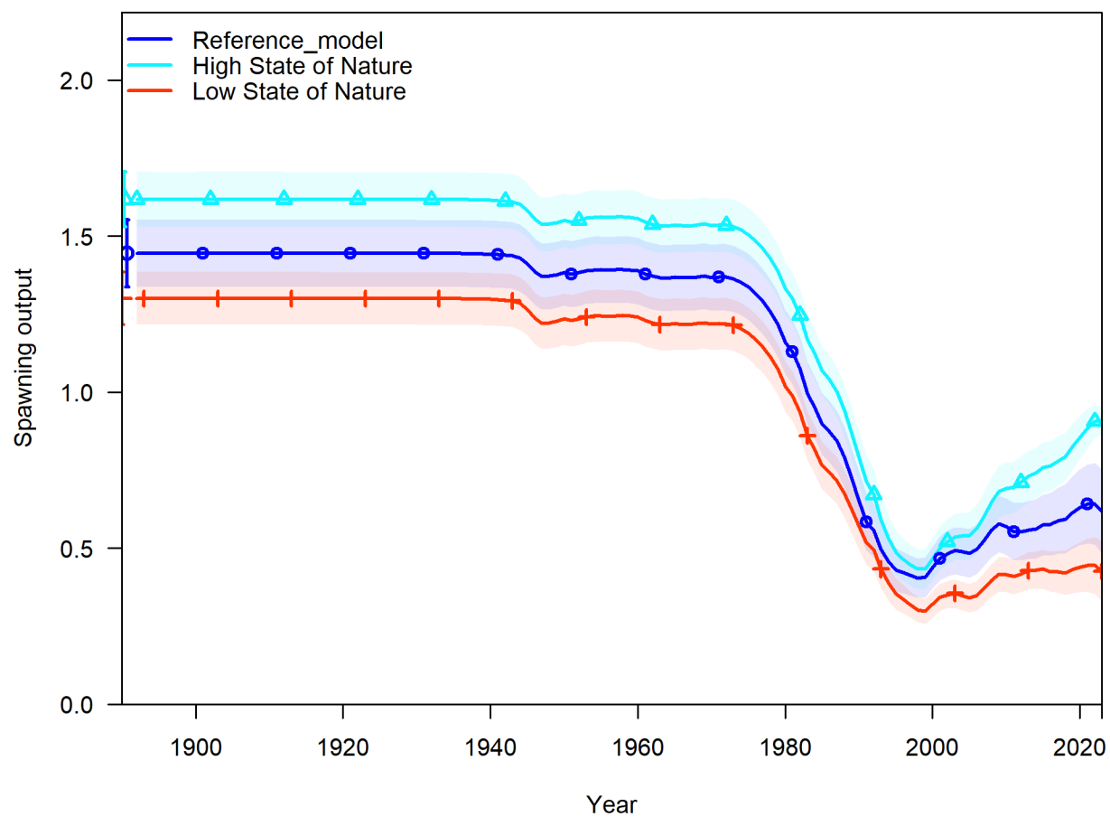
Figure 90: Time series of spawning output (with 95% uncertainty envelopes) for three states of nature, based on the treatment of the acoustic visual survey catchability, of Oregon black rockfish.
