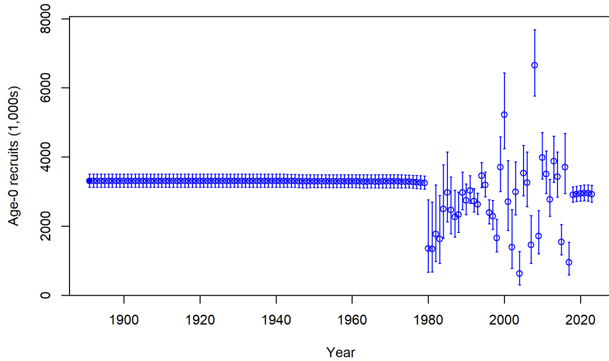
Figure 60: Estimated time series of age-0 recruits (1000s).
