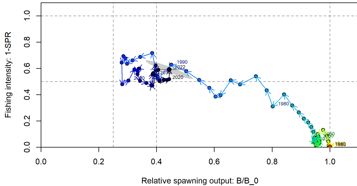
Figure 88: Phase plot of the relative biomass (also referred to as fraction unfished) versus the SPR ratio where each point represents the biomass ratio at the start of the year and the relative fishing intensity in that same year. Lines through the final point show the 95 percent intervals based on the asymptotic uncertainty for each dimension. The shaded ellipse is a 95 percent region which accounts for the estimated correlations between the biomass ratio and SPR ratio.
