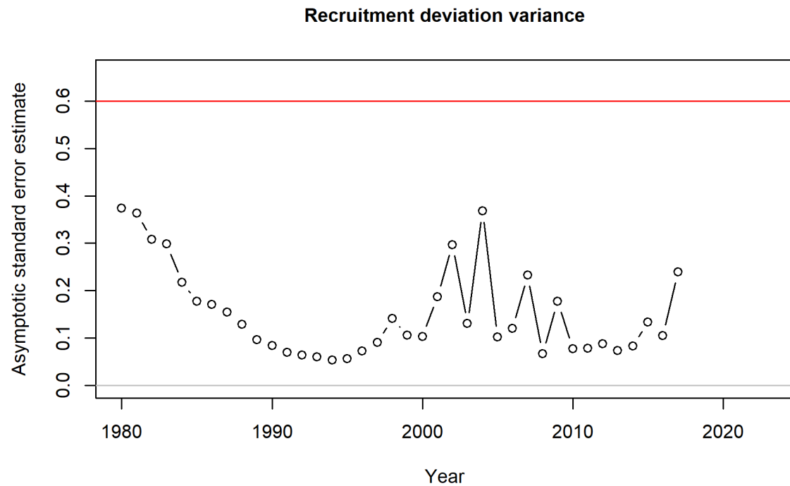
Figure 62: Recruitment deviations variance by year. This plot tracks the information content contained in each recruitment deviation. Values below the red line (assumed recruitment variability) indicates years with more informed recruitment deviations.
