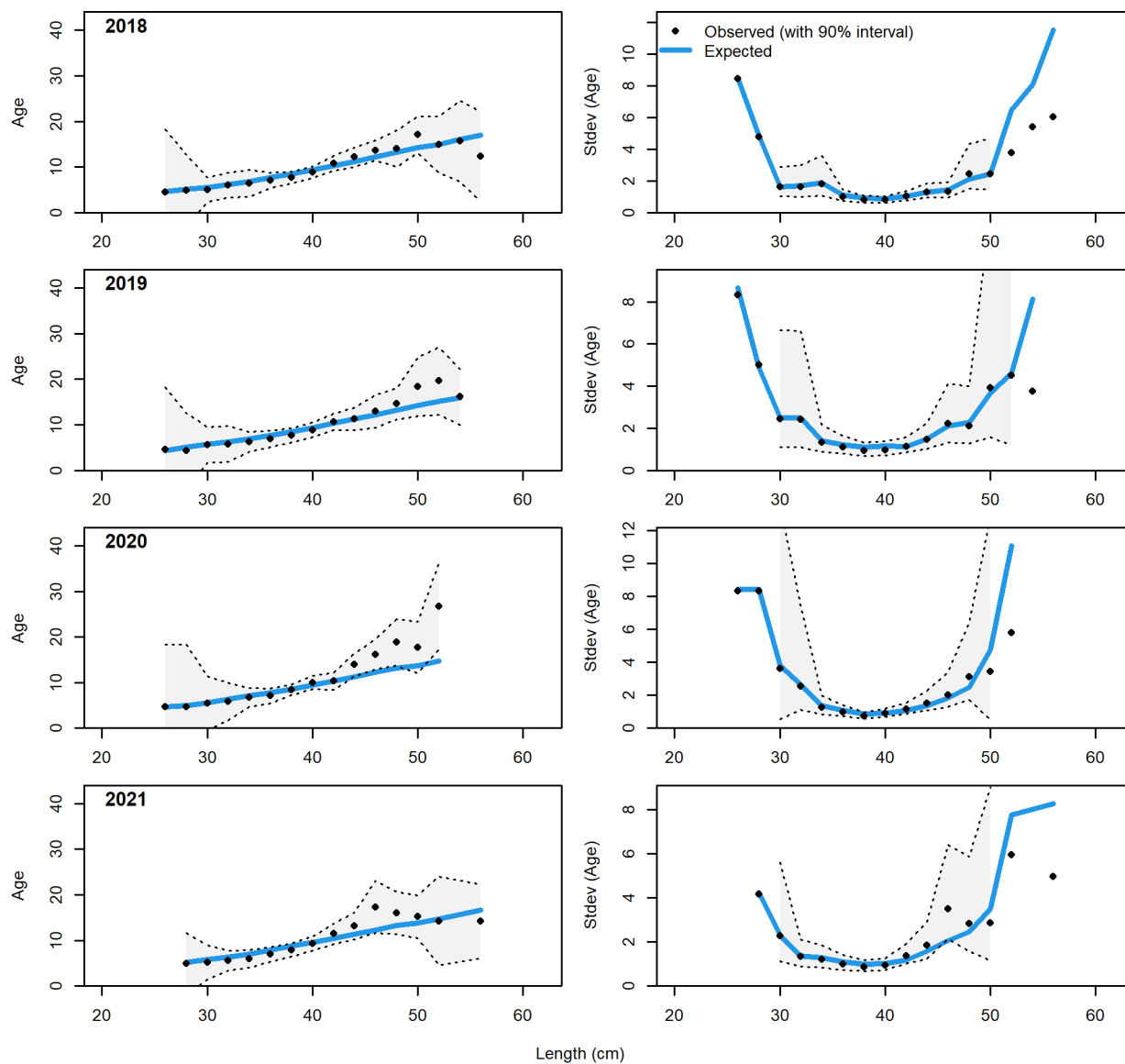
Figure 122: Non-trawl conditional AAL plot (plot 5 of 7).
