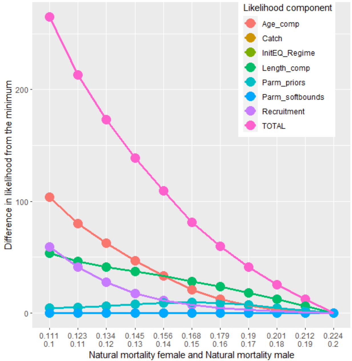
Figure 39: Likelihood component values for the female and male M multi-parameter likelihood profile.
