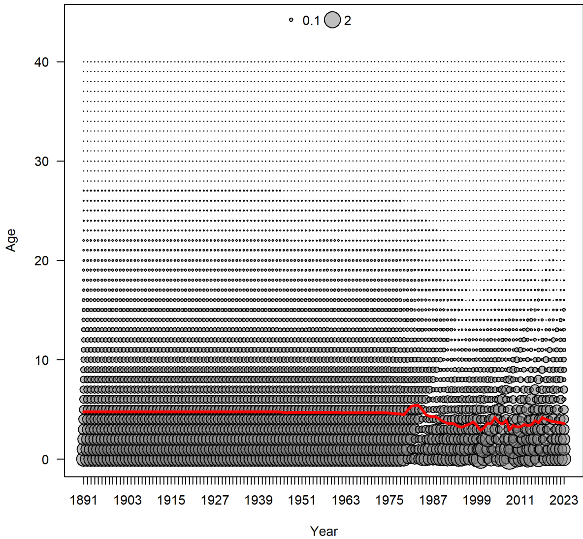
Figure 130: Female black rockfish mean age over time.
