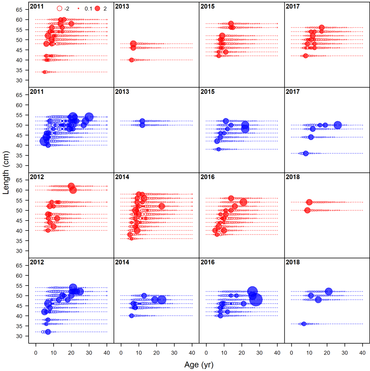
Figure 100: Pearson residuals, whole catch, Trawl_wdis (max=13.1) (plot 2 of 3).
