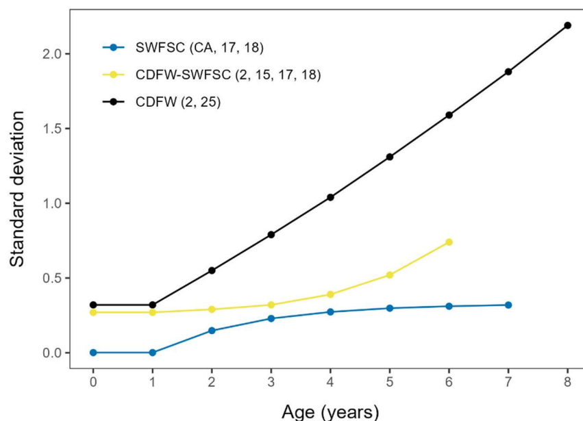
Figure 6. Survey and fishery ageing error vectors used in the final assessment model (CDFW and SWFC vectors) and sensitivity tests (CDFW-SWFSC vector). Blue dotted line shows ageing errors estimated from 2012-2022 summer survey samples; orange dotted line shows ageing errors estimated from summer 2012-2017 survey samples; and black dotted line shows ageing error estimated from 2008-2017 fishery samples. Numbers in parentheses indicate SWFSC and CDFW readers that produced age readings for estimating ageing errors.
