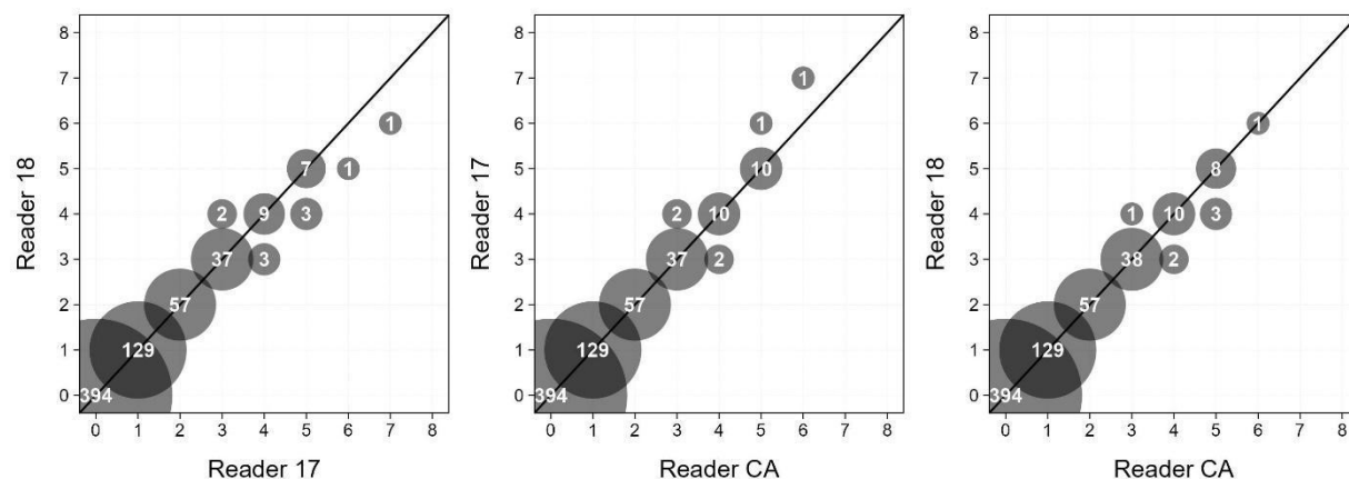
Figure 4. Age bias plots from the Agetat model for readers CA, 17, and 18 for Pacific Mackerel ( Scomber japonicus ) collected from summer SWFSC acoustic trawl surveys (2012-2022).
