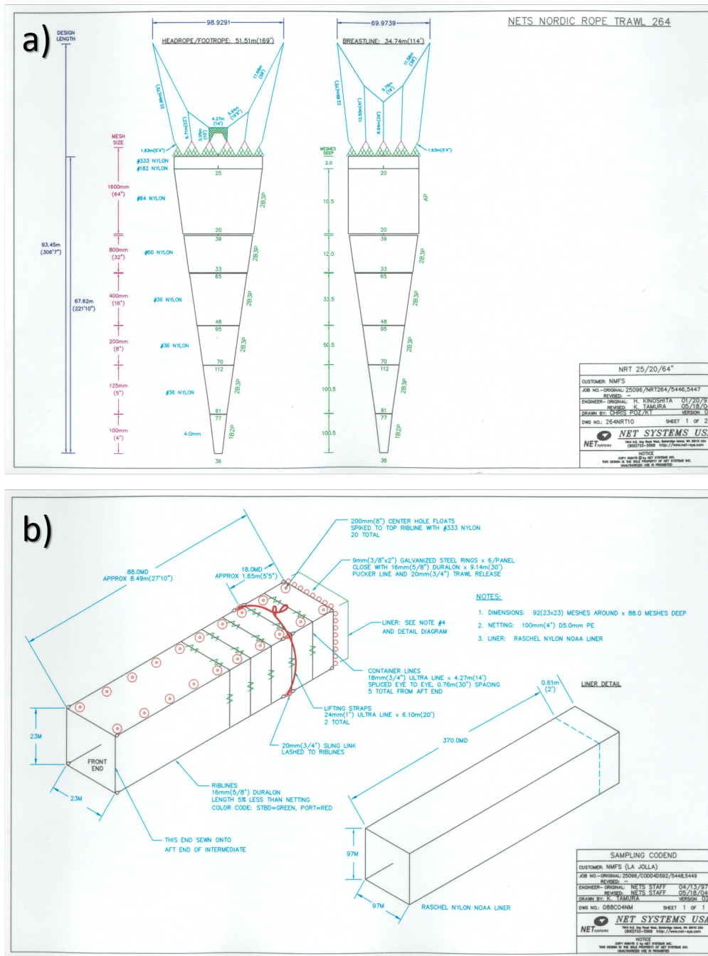
Figure 7: Schematic drawings of the Nordic 264 rope trawl net (a) and cod-end (b) on Lasker .
