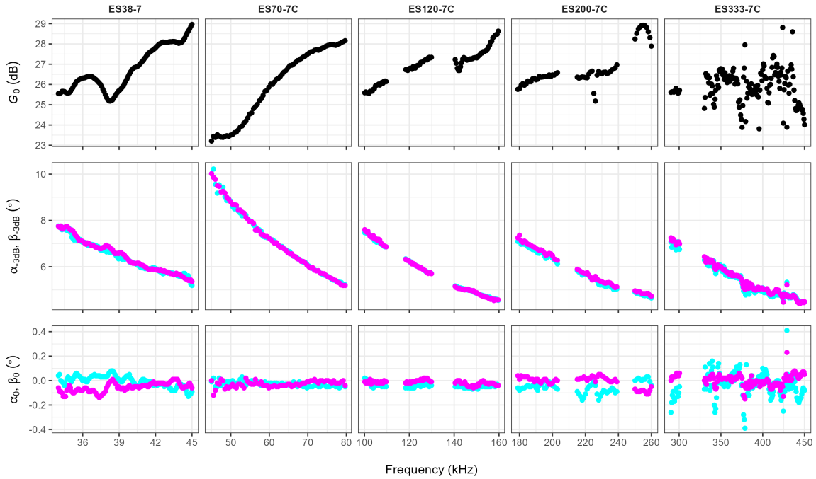
Figure 9: Measurements of on-axis gain ( G_0 , dB); alongship ( \alpha_{-3\text{dB}} , cyan) and athwartship ( \beta_{-3\text{dB}} , magenta) beamwidths (deg); and alongship ( \alpha_0 , cyan) and athwartship ( \beta_0 , magenta) offset angles (deg) measured during calibrations of EK80 wideband transceivers aboard Lasker (WBT; 38, 70, 120, 200, and 333 kHz) in frequency modulation (FM, or broadband) mode.
