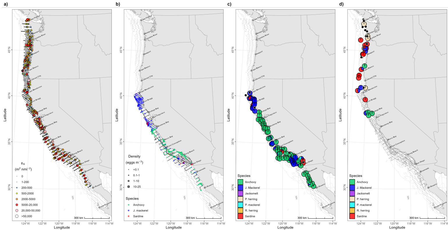
Figure 12: Survey transects overlaid with the distributions of: 38-kHz integrated backscattering coefficients ( s_A , \text{m}^2 \text{nmi}^{-2} ; averaged over 2000-m distance intervals and from 5- to 70-m deep) ascribed to CPS (a); egg densities (eggs \text{m}^{-3} ) for Northern Anchovy, Jack Mackerel, and Pacific Sardine from the CUFES (b); and proportions, by weight, of CPS species in each nighttime Lasker trawl (c) or daytime Lisa Marie seine catch (d; black points indicate trawls with no CPS). Species with low catch weights are not visible at this scale.
