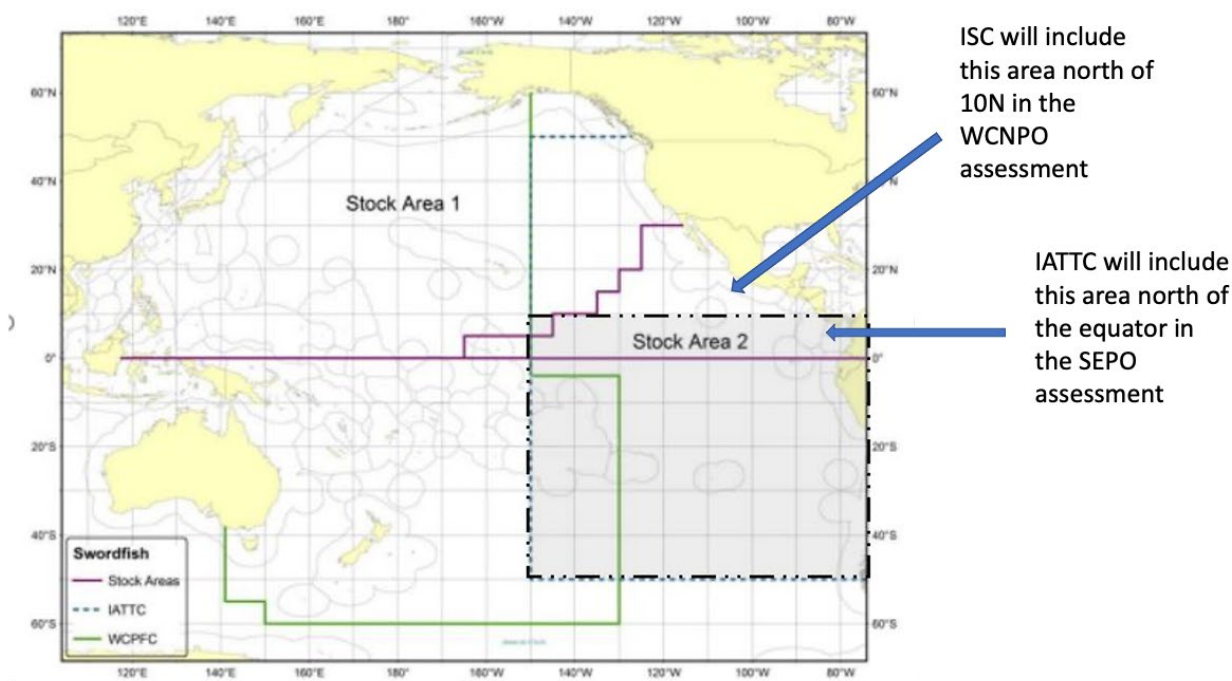
Figure 8-1. Stock Area 1 depicts boundaries used in the 2018 Western and Central North Pacific Ocean swordfish stock assessment. Stock Area 2 depicts boundaries for the Eastern Pacific Ocean stock in the North Pacific Ocean. The green line indicates the Western Central Pacific Fisheries Commission convention area and the blue dashed line indicates the Inter-American Tropical Tuna Commission convention area. The square area
