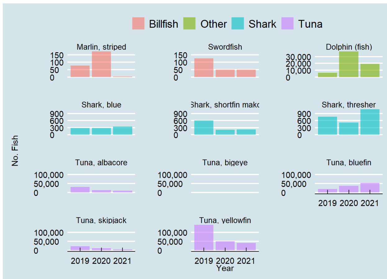
Figure 5-2. Total catch (retained plus discarded) by species (retained plus discarded) aggregated by fleet and zone, 2019 - 2021.
