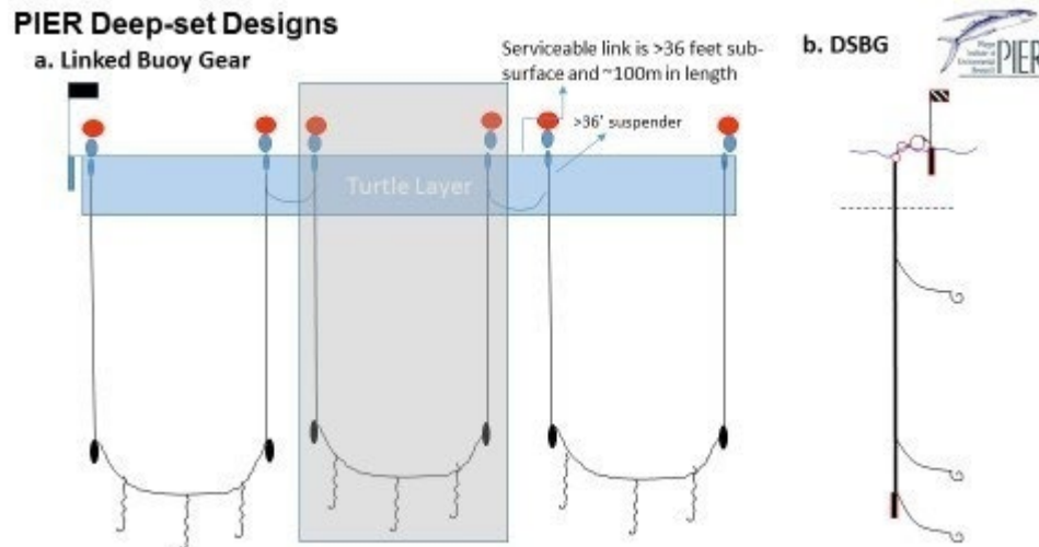
Figure 4-12. Standard and linked DSBG configurations. (Source: Pflieger Institute of Environmental Research.)
