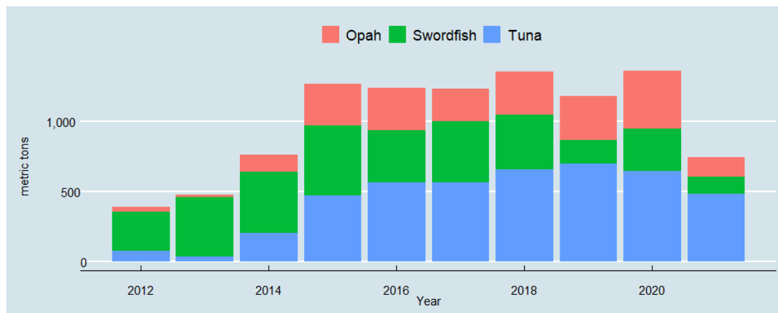
Figure 4-8. Landings trends for opah, swordfish, and tuna (mt) in the pelagic longline fishery, 2012-2021.
