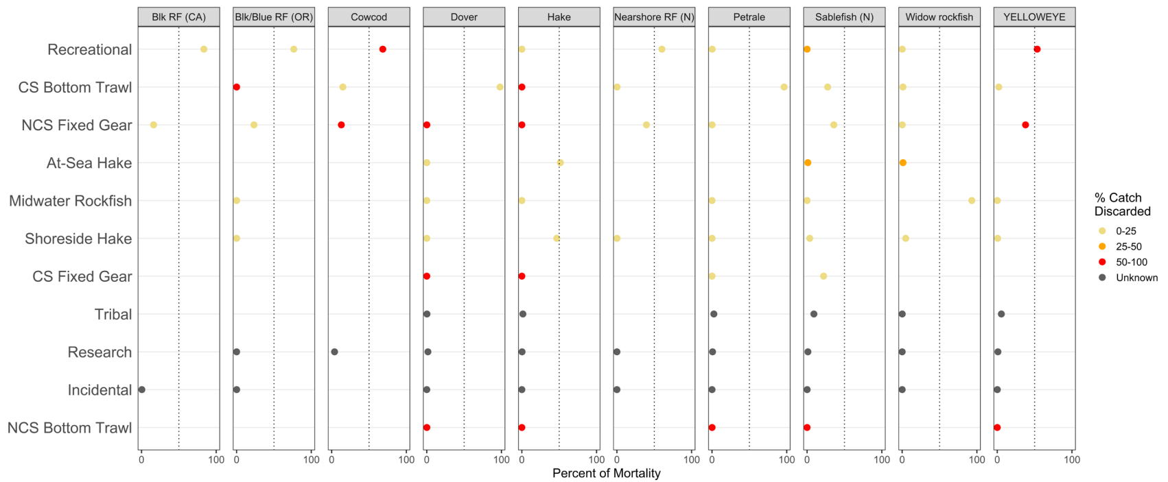
Figure 4. Sector-level contributions to 2021 mortality. Sablefish is managed north and south of lat 36°N; the minor nearshore rockfish complex is managed north and south of lat 40°10'N. Rebuilding species are capitalized.
