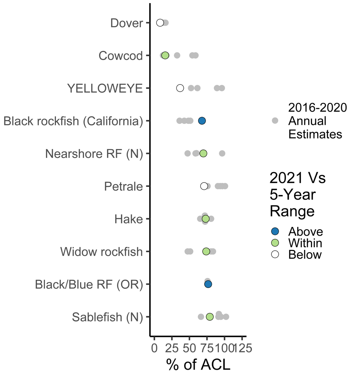
Figure 3. Proportion of ACL attained in 2021 compared to 2016–20 for select species that are highly targeted, highly attained, or rebuilding. Gray points display annual estimates from 2016 to 2020; 2021 points are colored as indicated in the legend. Hake attainment is shown as proportion of TAC. Sablefish is managed north and south of lat 36°N; the minor nearshore rockfish complex is managed north and south of lat 40°10'N. Black/blue rockfish (OR) was defined as a management grouping in 2019, so only three reference points are available. Rebuilding species are capitalized.
