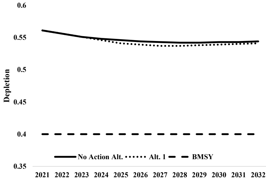
Figure 1-1. Predicted depletion of Oregon black rockfish under two alternative harvest control rules, 2021-2032.
