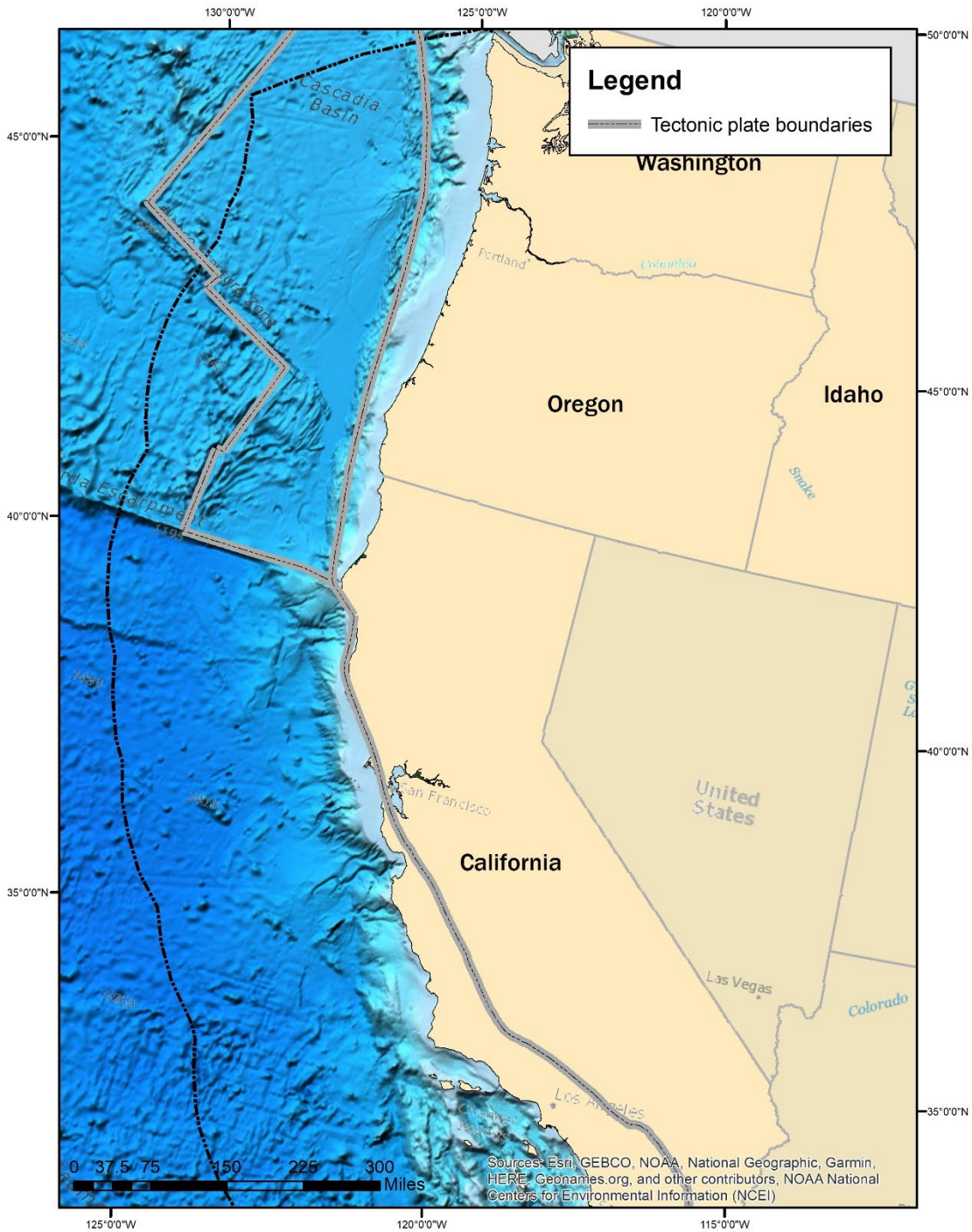
Figure 3-4. Important geological features in the CCE.
