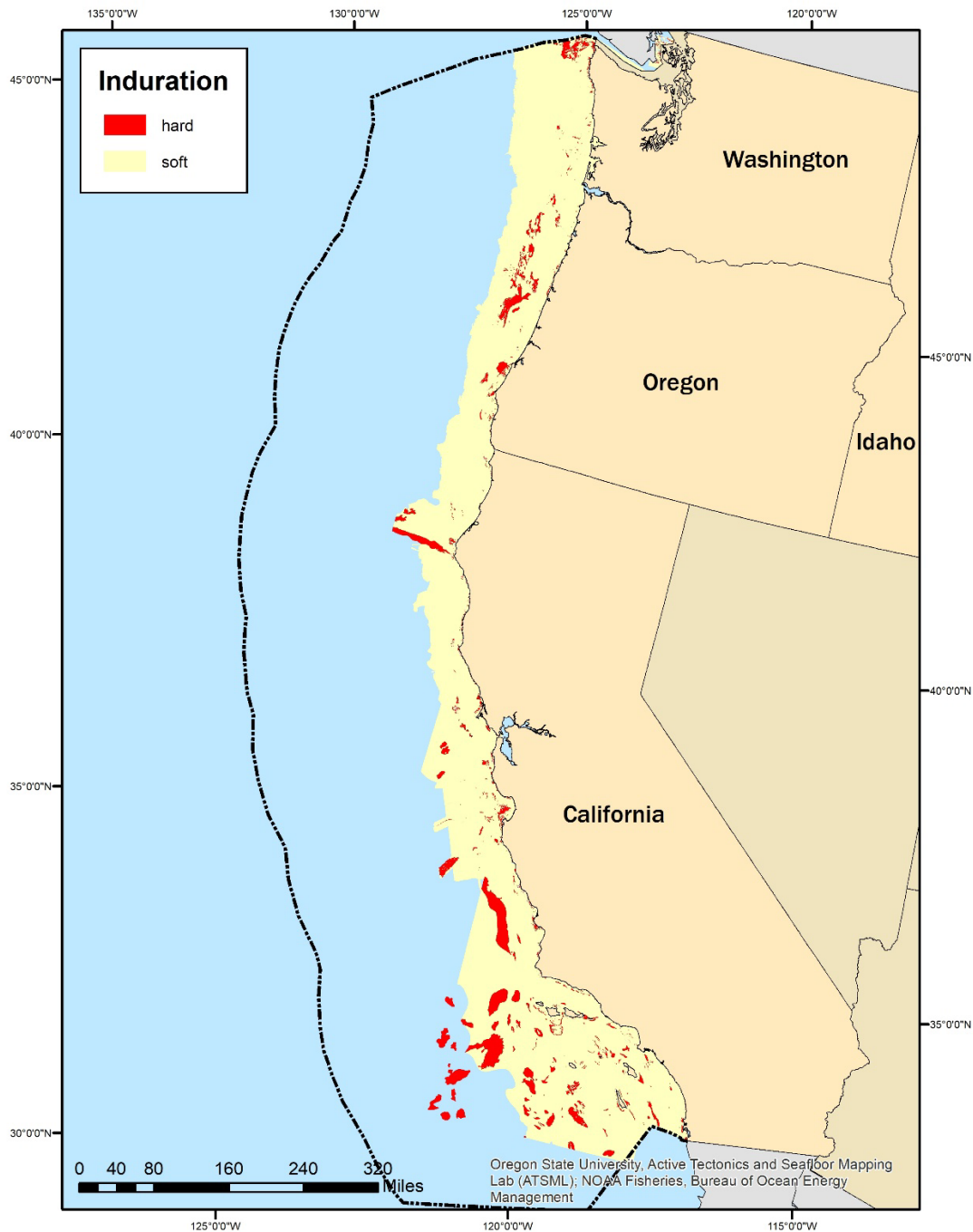
Figure 3-3. Benthic habitat in the CCE.
