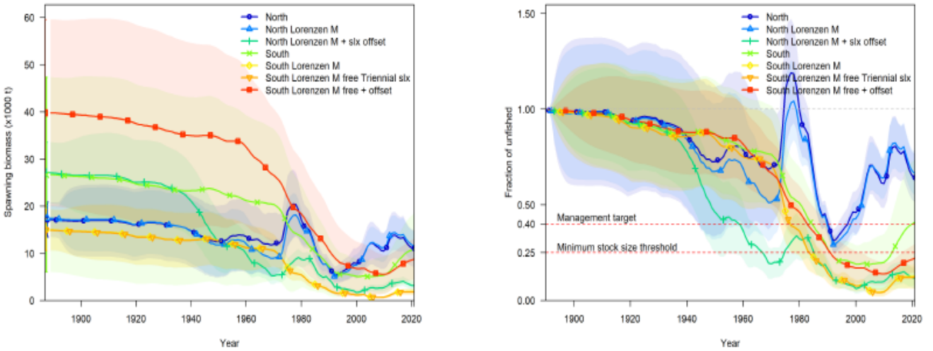
Figure 2. Comparison between using the Lorenzen mortality function, with and without sex selectivity offset, for Northern and Southern stocks compared to the base run.
