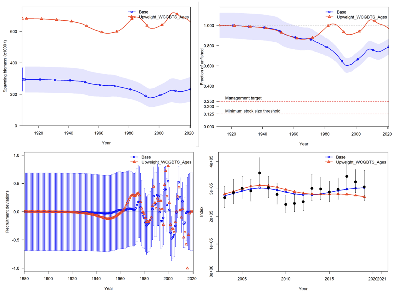
Figure 8. Comparison of spawning biomass (top left), stock status (top right), recruitment (lower left), and the fit to the WCGBTS index (lower right) for the base model and the sensitivity model where the WCGBTS mean age data are forced to fit better than in the base model.
