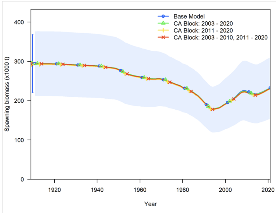
Figure 4 Spawning biomass estimated across selectivity block sensitivities.
