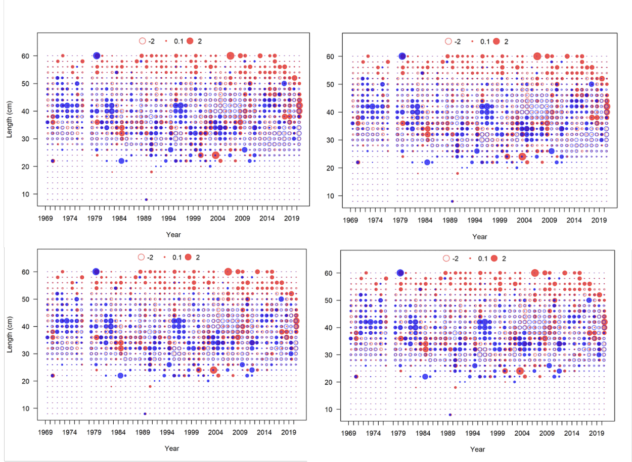
Figure 3 Pearson residuals of length data by year for the California fleet. The top-right panel is the base model, top-left is the sensitivity with a block from 2003 - 2020, bottom-left is the sensitivity with a block from 2011 - 2020, and the bottom-right is the sensitivity with a block from 2003 - 2010 and 2011 - 2020.
