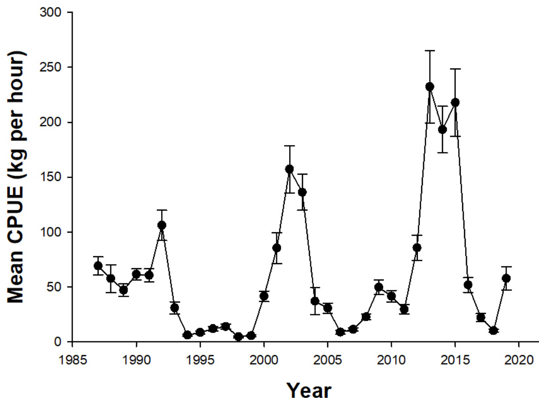
Figure 5. Total mean ( \pm SE) catch per unit effort (CPUE; kg/h) of eulachon across all surveyed Shrimp Management Areas off West Coast Vancouver Island (WCVI) from 1987–2020. Data for 2020 are unavailable due to fieldwork restrictions during the COVID-19 pandemic. CPUE is based on bycatch of eulachon in multispecies small mesh bottom trawl surveys (aka fishery-independent shrimp surveys) offshore of WCVI. Data courtesy of Sean MacConnachie, Vanessa Hodes, and most recently, Linnea Flostrand (Fisheries and Oceans Canada, Pacific Biological Station, Nanaimo, BC, Canada, pers. commun., 25 January 2021).
