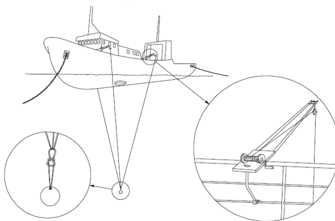
Figure A8. The EK60 system is calibrated by suspending a metal sphere directly beneath the transducer at a range of more than 20 feet. The sphere is tethered using two or three monofilament lines. It is positioned by manually adjusting the line positions and lengths. Note: prior to the calibration, the transducer face must be cleaned of all biofouling.
