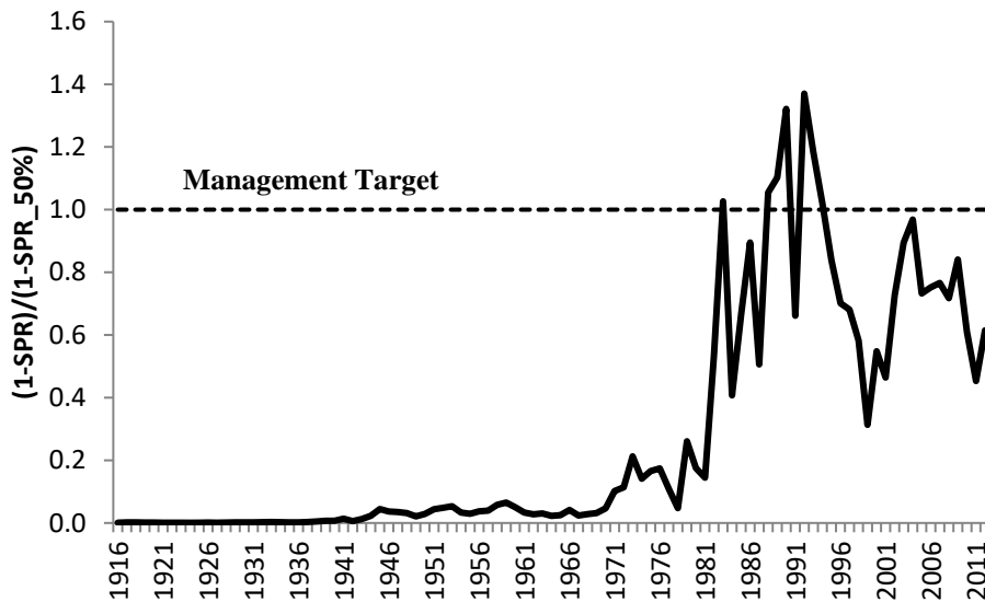
Figure 2-78. Time series of estimated relative spawning potential ratio ( 1-SPR/1-SPR(\text{Target}=0.50) ) for aurora rockfish, 1916-2012. Values of relative SPR above 1.0 reflect harvests in excess of the current overfishing proxy.
