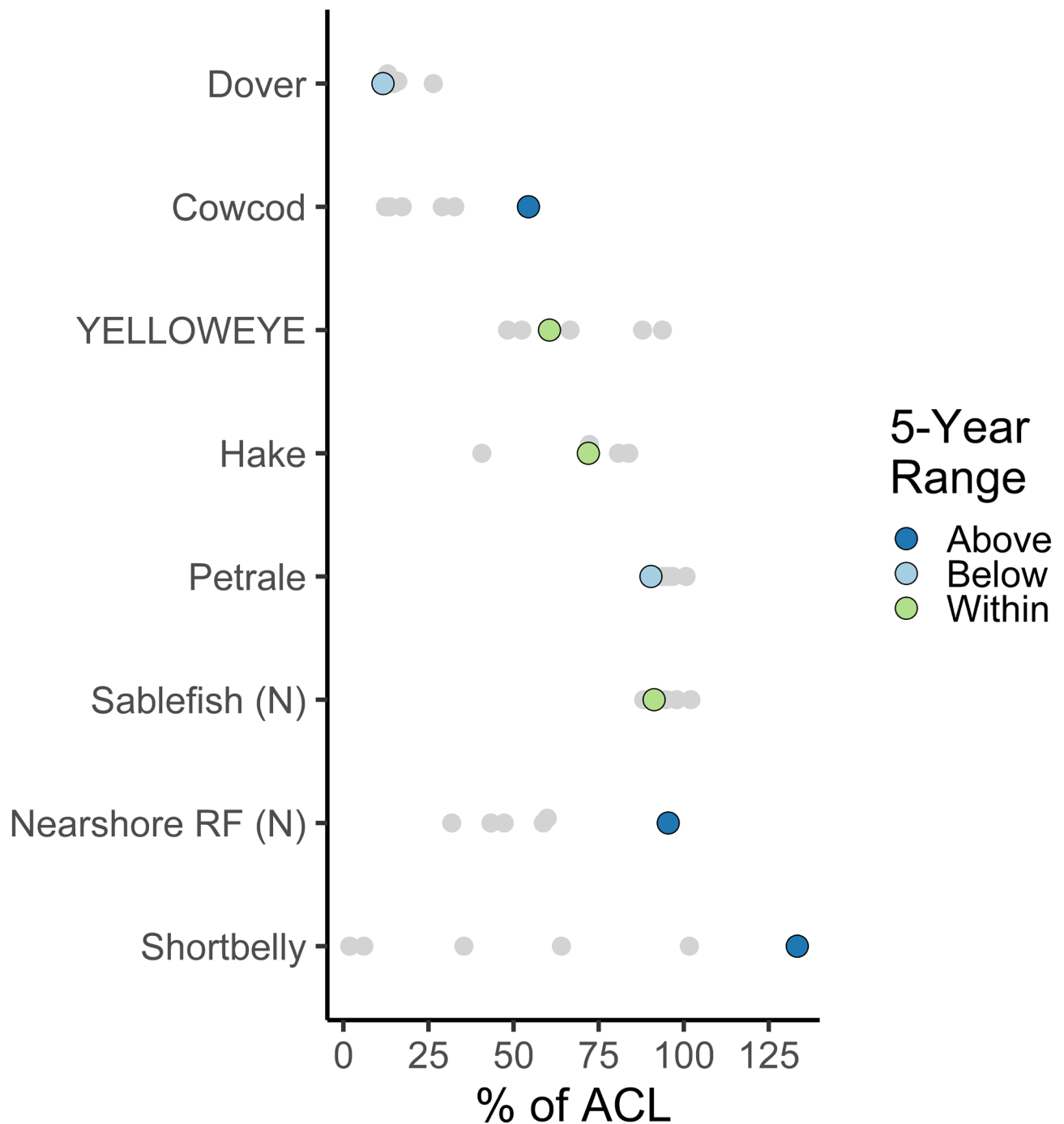
Figure 3. Proportion of ACL attained in 2019 compared to 2014 to 2018 for select species that are highly targeted or attained or rebuilding. Grey points display of annual estimates from 2014 to 2018; 2019 points are colored as indicated in the legend. Hake attainment is shown as proportion of TAC. Sablefish is managed north and south of lat 36°N; the minor nearshore rockfish complex is managed north and south of lat 40° 10'N. Rebuilding species are capitalized.
