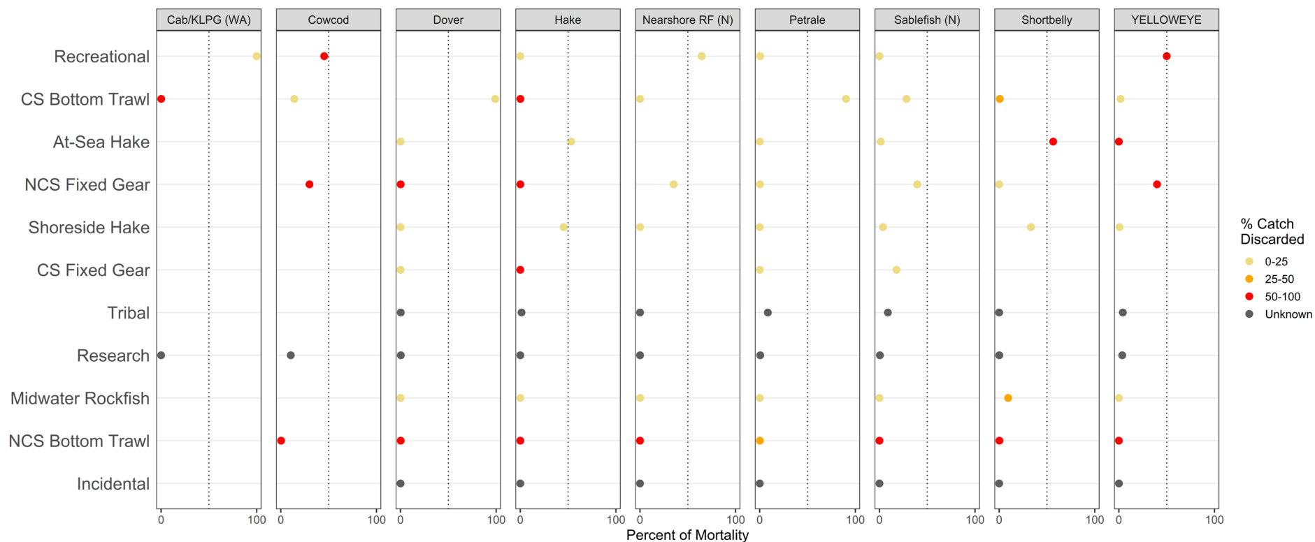
Figure 4. Sector-level contributions to 2019 mortality. Sablefish is managed north and south of lat 36°N; the minor nearshore rockfish complex is managed north and south of lat 40° 10'N. Rebuilding species are capitalized.
