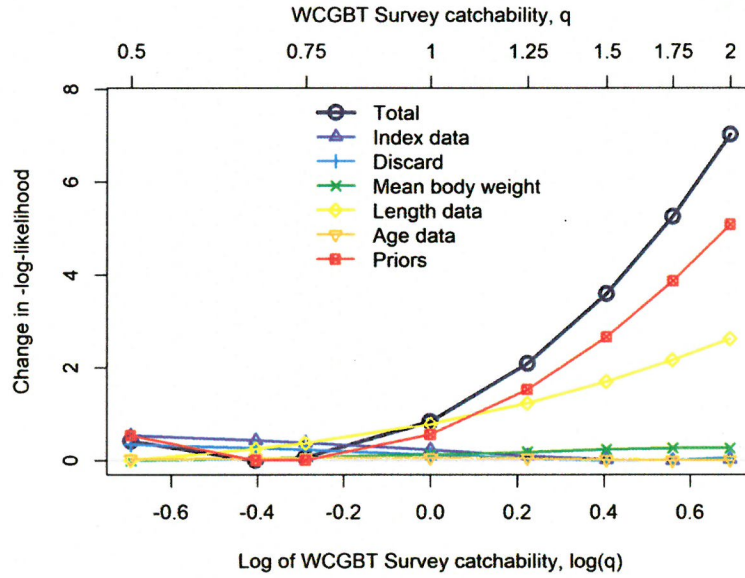
Figure 7. Likelihood profile over WCGBT \ln(\text{survey-}Q) including the new prior on the WCGBT catchability coefficient, with \ln(\text{survey-}Q) mean = -0.355 and SD = 0.326 (median catchability of 0.701).
