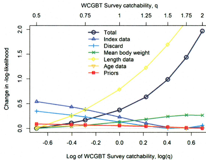
Figure 6. Likelihood profile over WCGBT \ln(\text{survey-}Q) with no prior on the WCGBT catchability coefficient (survey- Q ).
