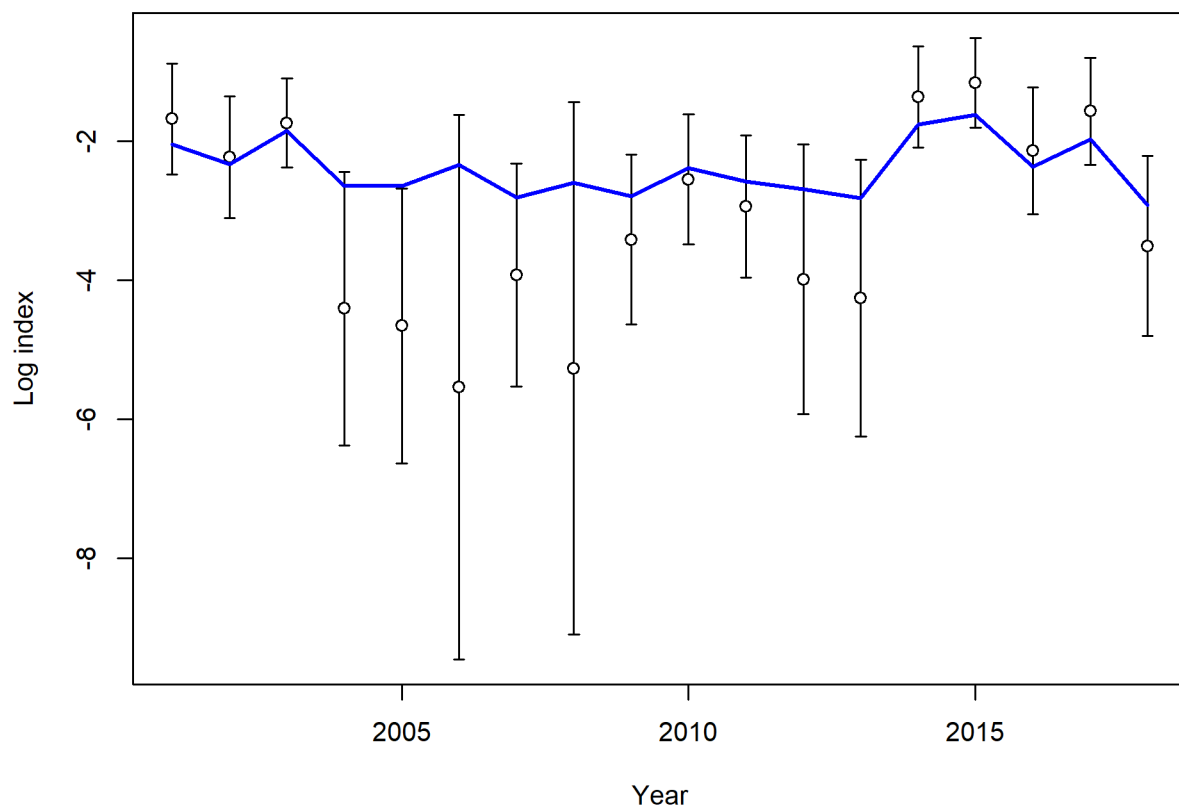
Figure 68: Fit to log index data on log scale for the fishery-independent PISCO age-0 (6 cm or less) kelp forest fish survey for fish 15 cm and larger. Lines indicate 95% uncertainty interval around index values.
