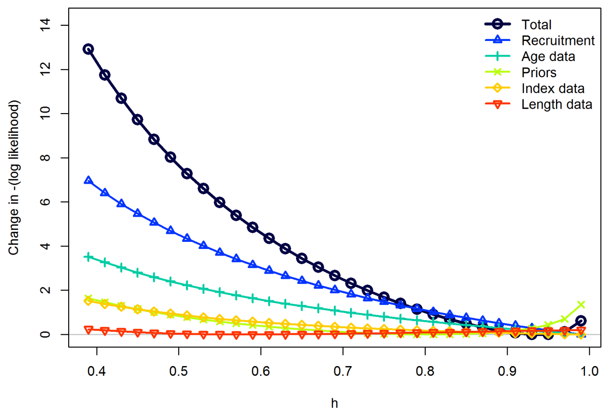
Figure 82: Likelihood profile across steepness values for each data type.
