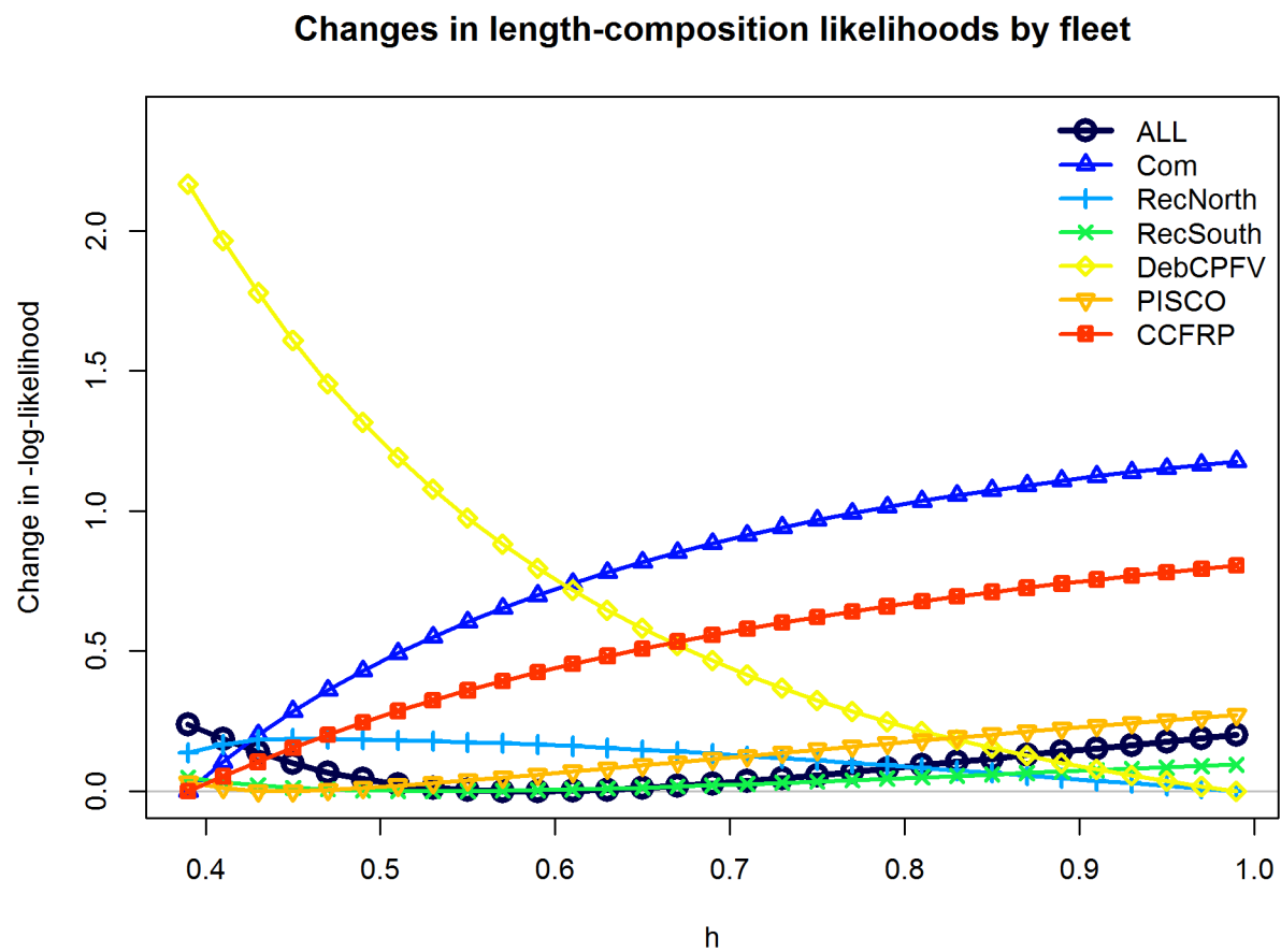
Figure 80: Likelihood profile across steepness values by fleet length composition.
