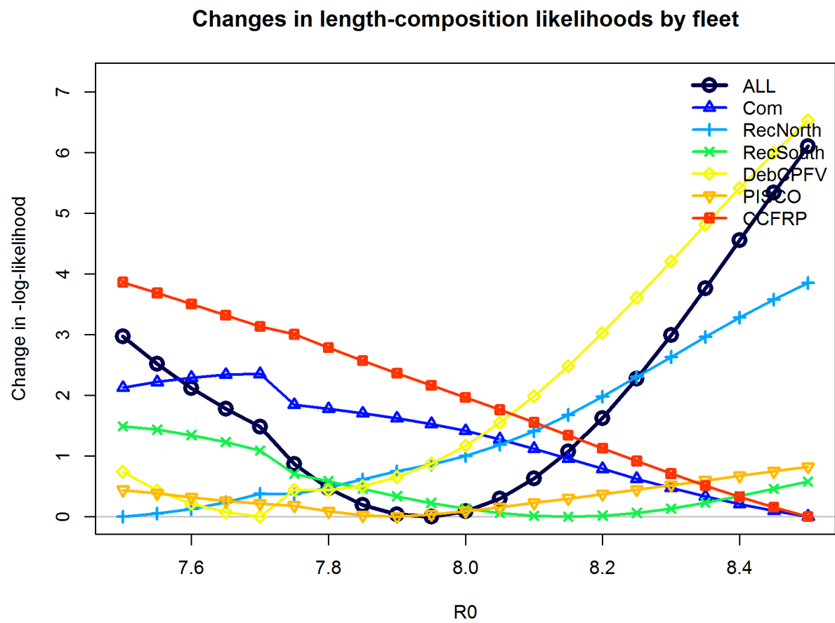
Figure 76: Likelihood profile across R_0 values of length composition by fleet.
