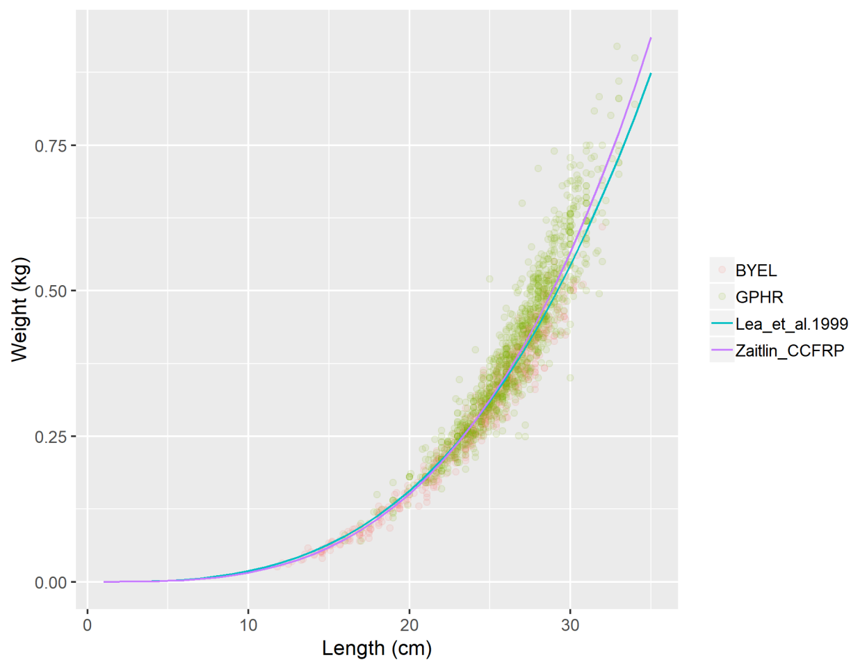
Figure 41: Comparison of the gopher rockfish weight-length curves from Lee et al. (1999) and the estimated from black-and-yellow rockfishes from Zaitlin (1986), and gopher rockfishes from Loury (2011) and Meyers-Cherry(2014). The estimated curve from the current data is used in this assessment.
