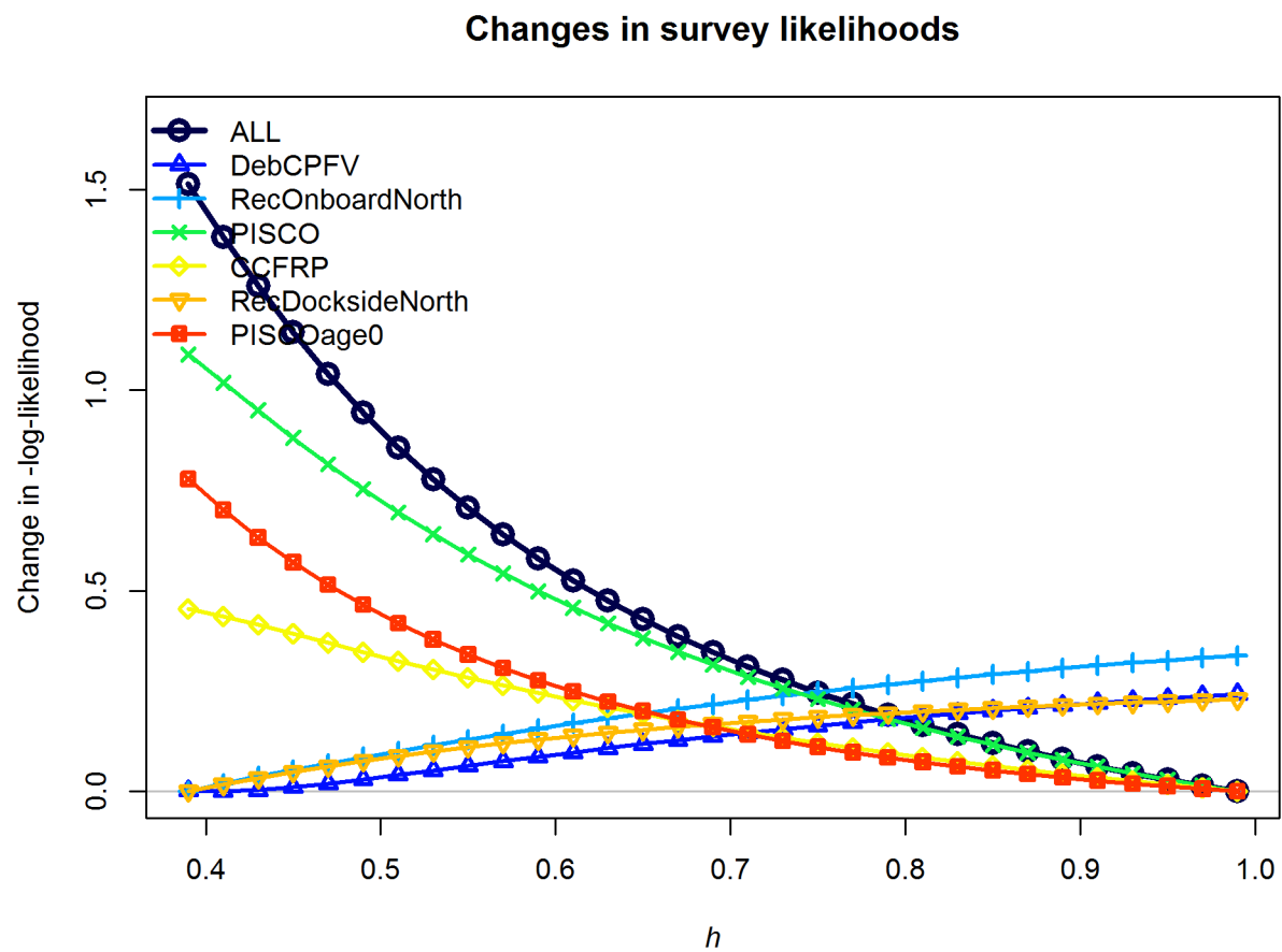
Figure 81: Likelihood profile across steepness values by surveys.
