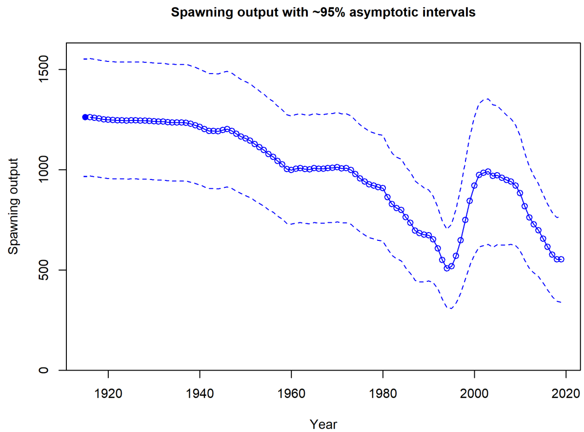
Figure 92: Estimated spawning output with approximate 95% asymptotic intervals.
