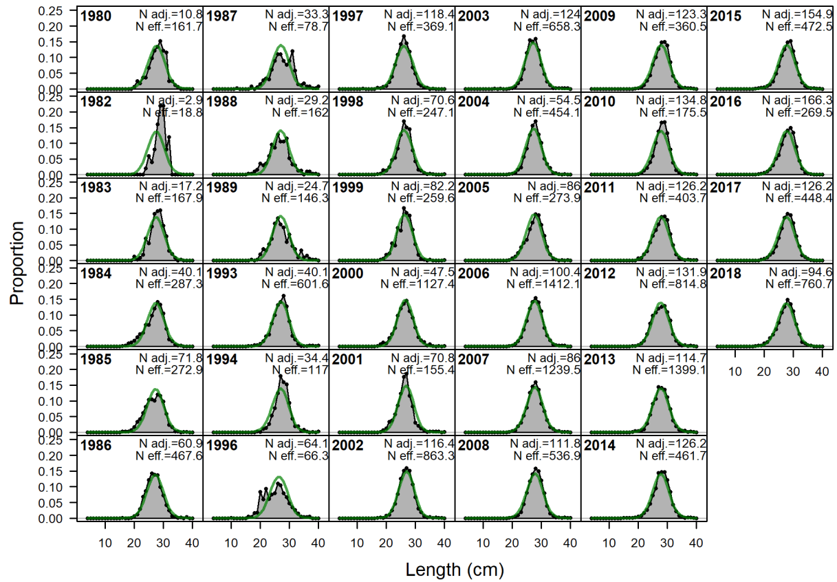
Figure C3: Length comps, whole catch, RecNorth. ‘N adj.’ is the input sample size after data_weighting adjustment. N eff. is the calculated effective sample size used in the McAllister-Jannelli tuning method.
