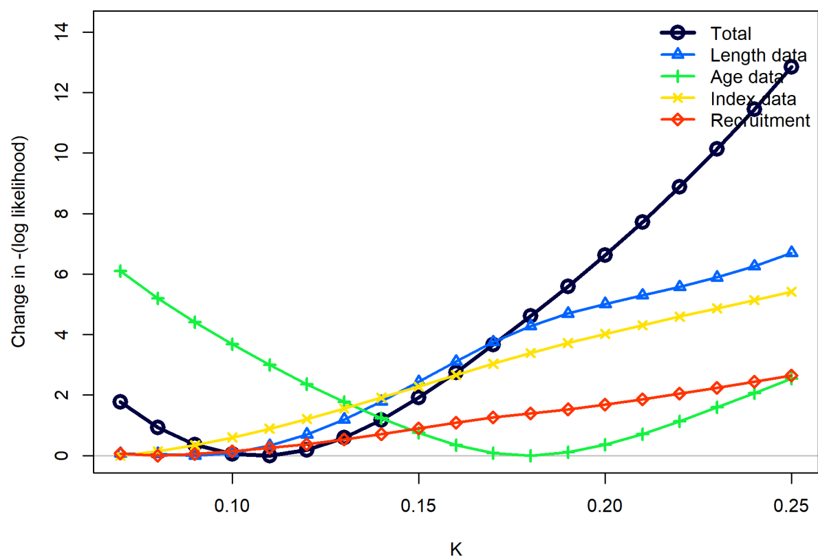
Figure 88: Likelihood profile across the growth parameter k for each data type.
