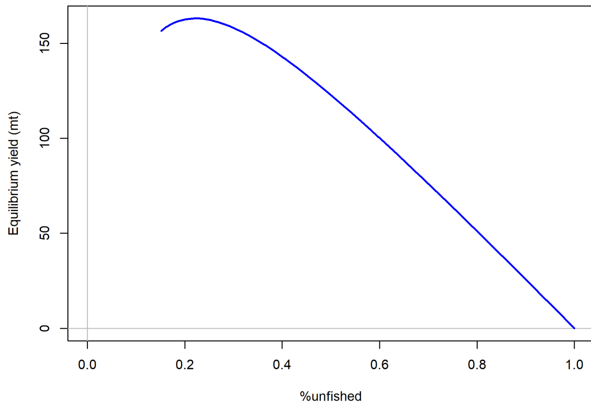
Figure i: Equilibrium yield curve for the base case model. Values are based on the 2018 fishery selectivity and with steepness fixed at 0.72.
