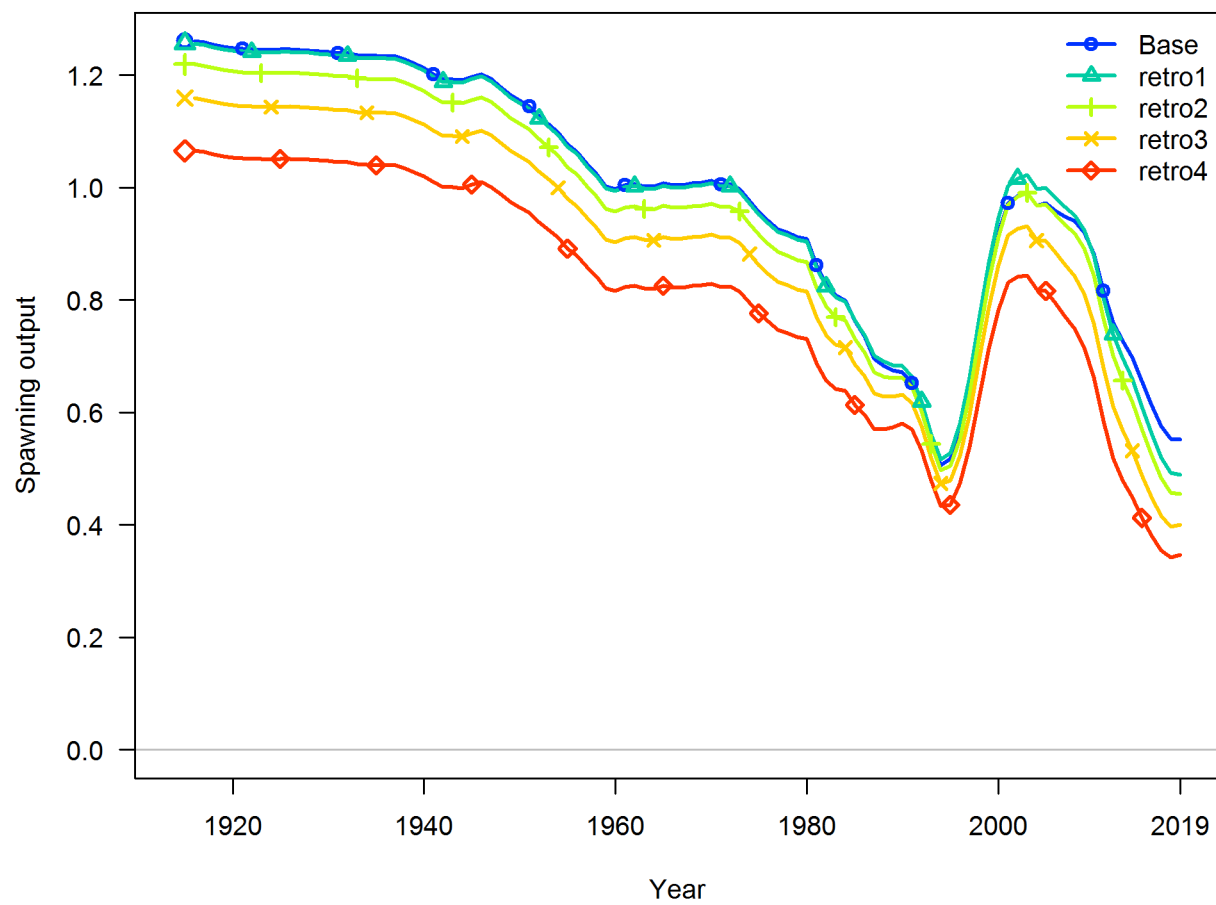
Figure 74: Retrospective pattern for spawning output.
