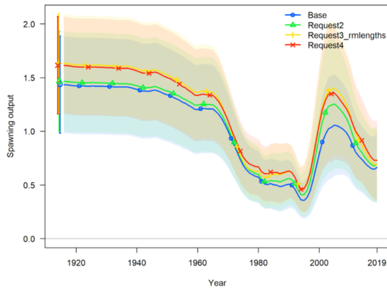
Figure 46: Comparison of time series of relative and absolute spawning output from pre-STAR base model and models from requests 2, 3a and 4.
