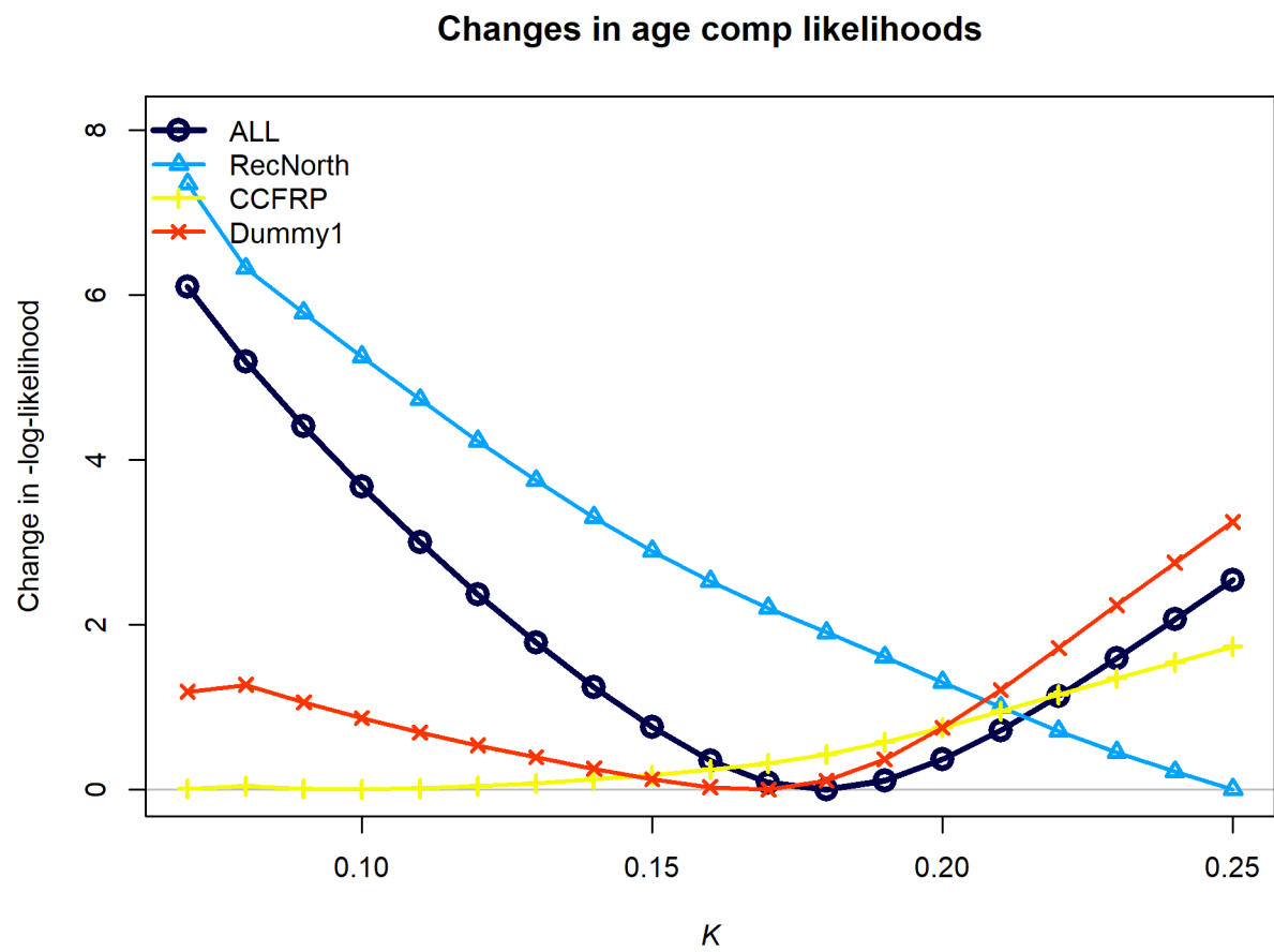
Figure 89: Likelihood profile across the growth parameter k by age composition.
