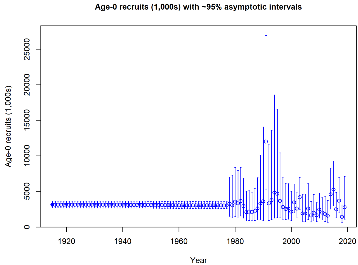
Figure 61: Time series of estimated GBYR recruitments for the base-case model with 95% confidence or credibility intervals.
