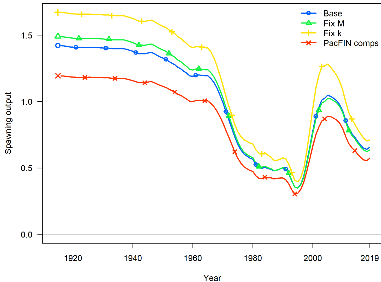
Figure 42: Sensitivity of the spawning biomass to fixing natural mortality to the prior, fixing the von Bertalanffy k parameter to the external estimate, or using commercial PacFIN length composition data instead of CALCOM, as compared to the pre-STAR base model.
