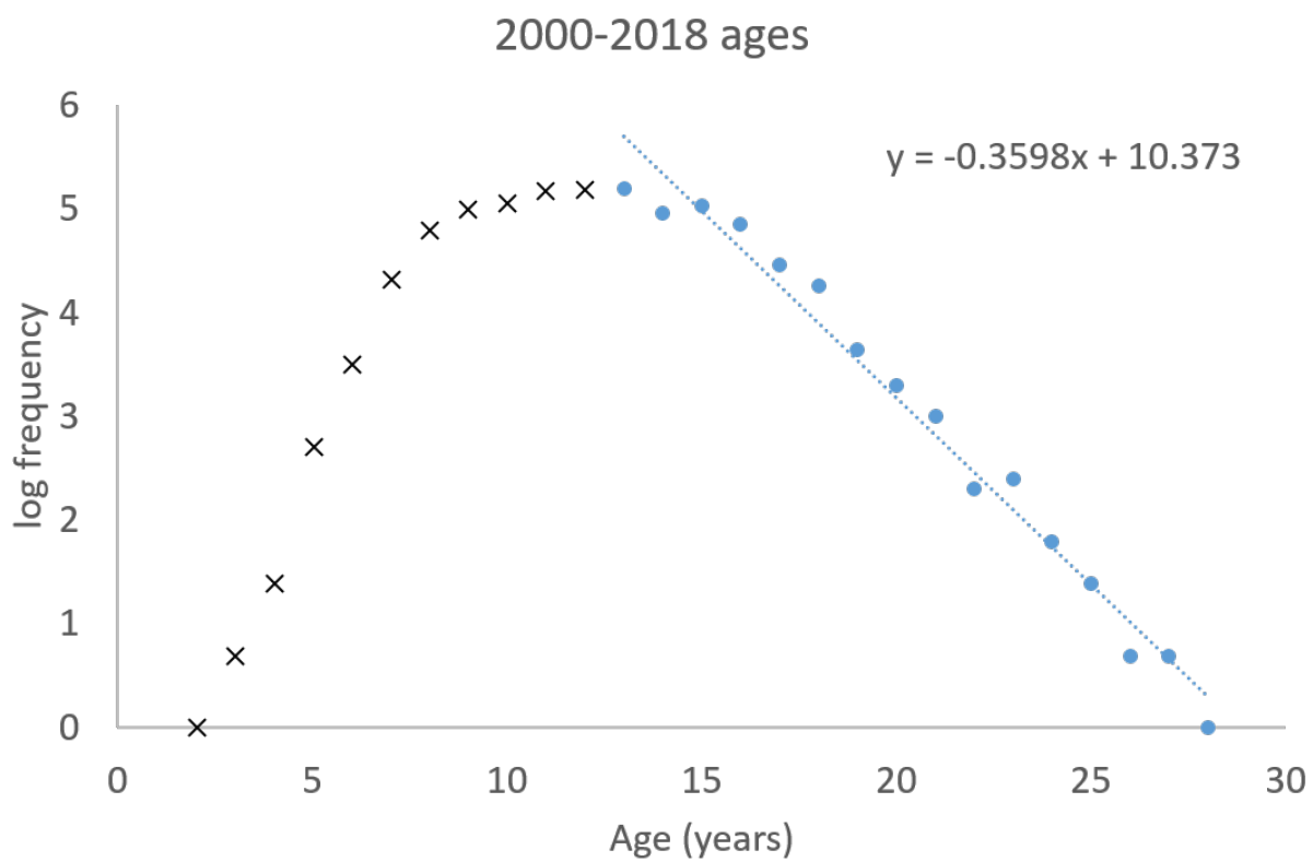
Figure 44: Catch curve analysis for age data prior to 2000 and for 2000-2018.
