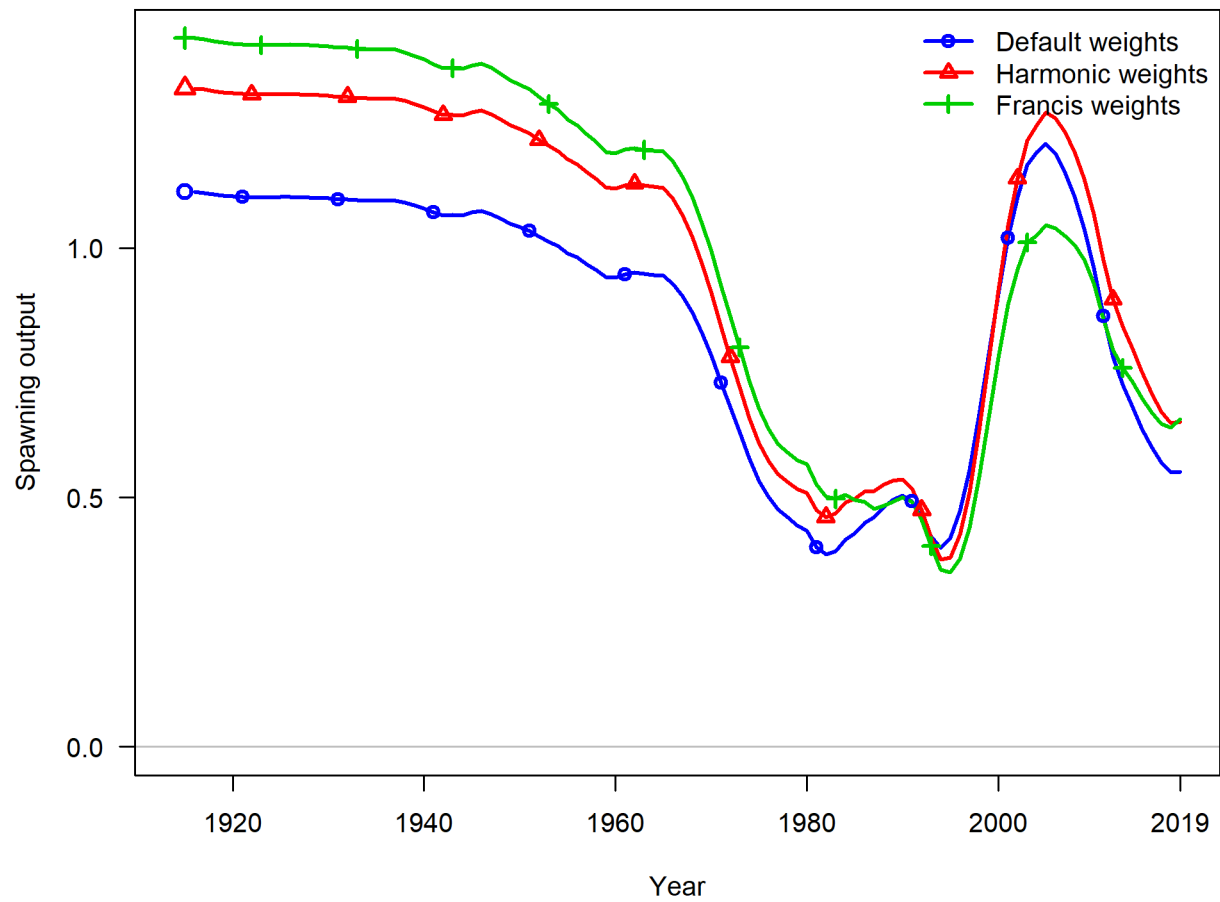
Figure 43: Sensitivity of the spawning biomass to either the default weight of composition data, the harmonic mean, or Francis weights.
