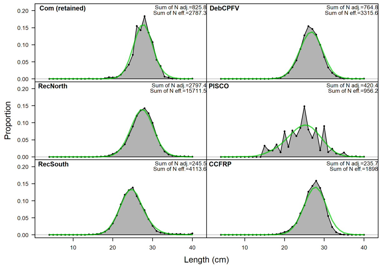
Figure 70: Length compositions aggregated across time by fleet.
