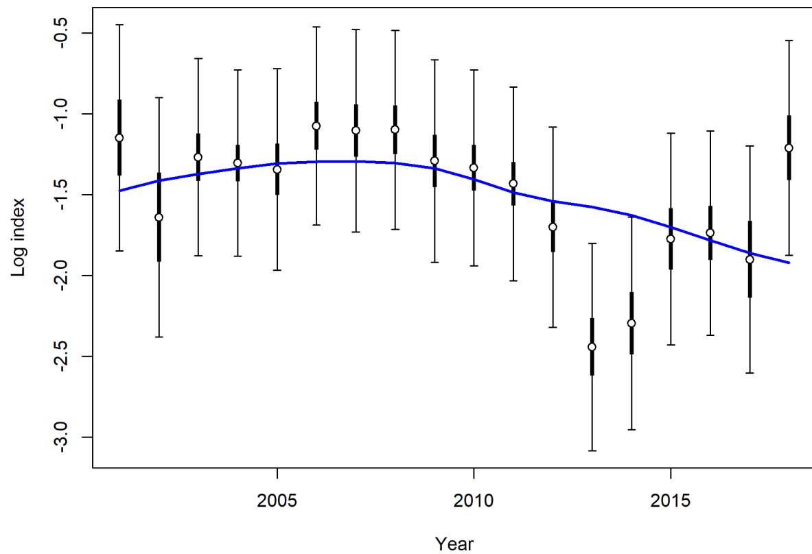
Figure 66: Fit to log index data on log scale for the CRFS/Cal Poly CPFV onboard observer survey north of Point Conception. Lines indicate 95% uncertainty interval around index values. Thicker lines indicate input uncertainty before addition of estimated additional uncertainty parameter.
