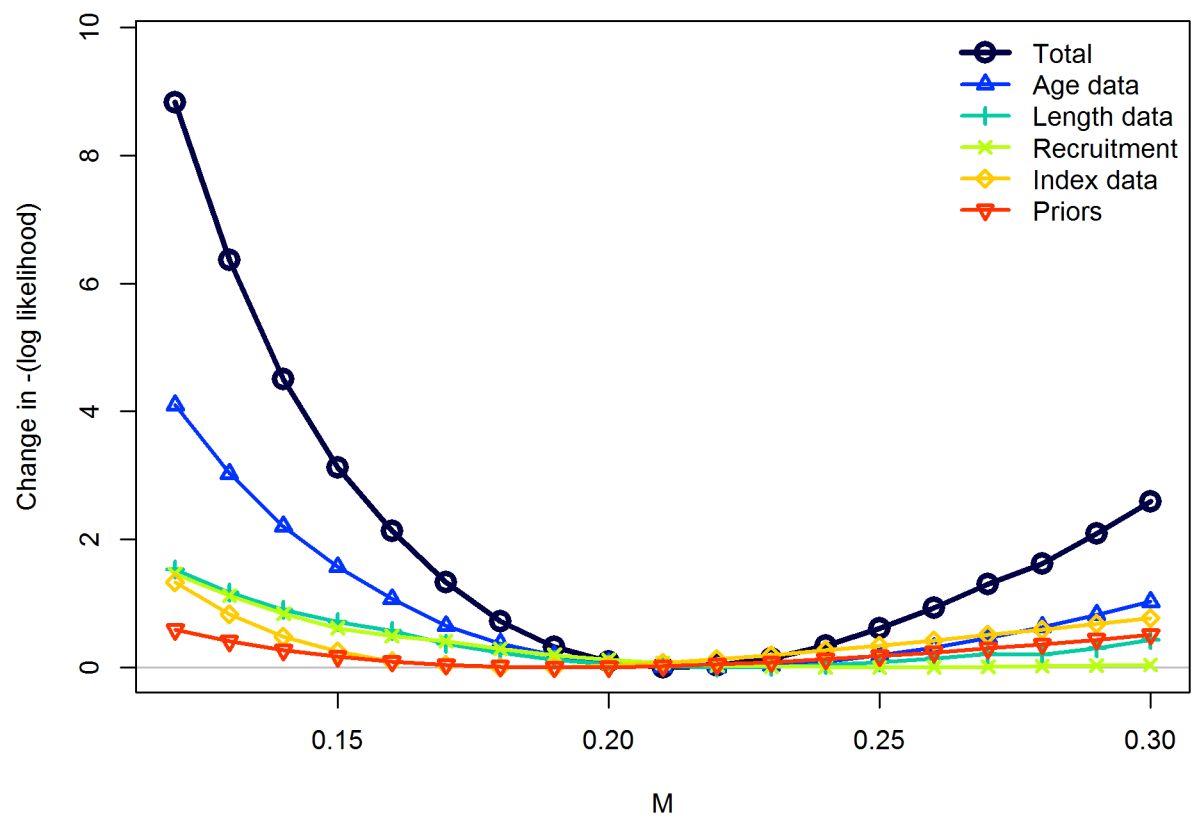
Figure 86: Likelihood profile across female natural mortality values for each data type.
