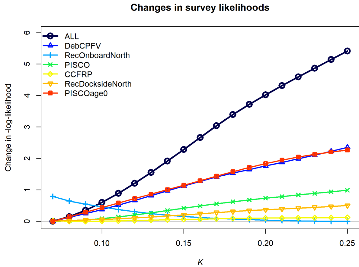
Figure 90: Likelihood profile across the growth parameter k by surveys.
