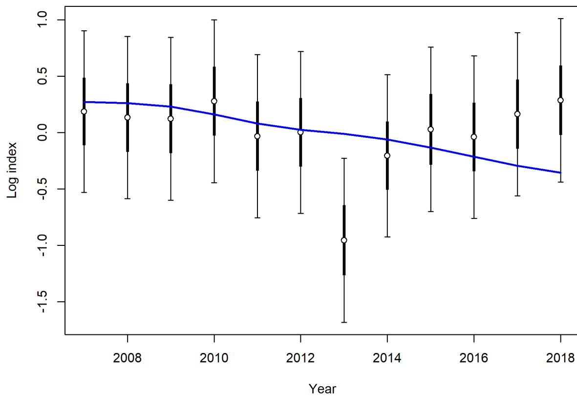
Figure 69: Fit to log index data on log scale for the fishery-independent CCFRP hook-and-line survey. Lines indicate 95% uncertainty interval around index values. Thicker lines indicate input uncertainty before addition of estimated additional uncertainty parameter.
