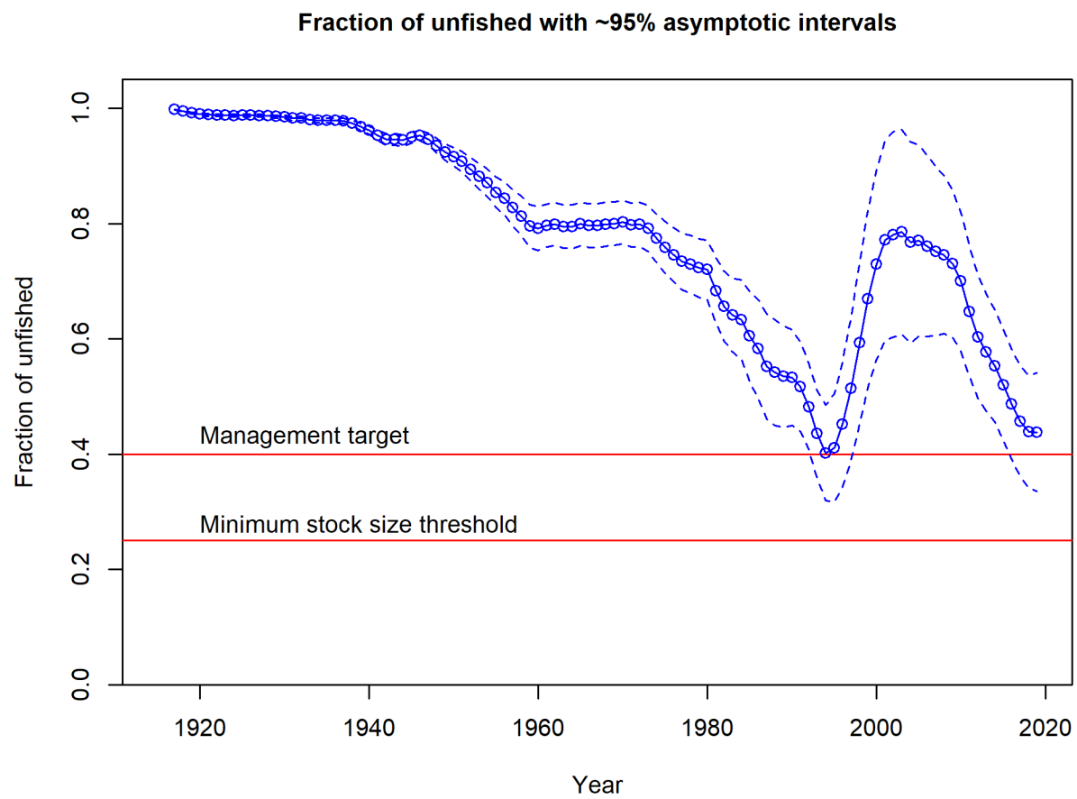
Figure 93: Estimated spawning depletion with approximate 95% asymptotic intervals.
