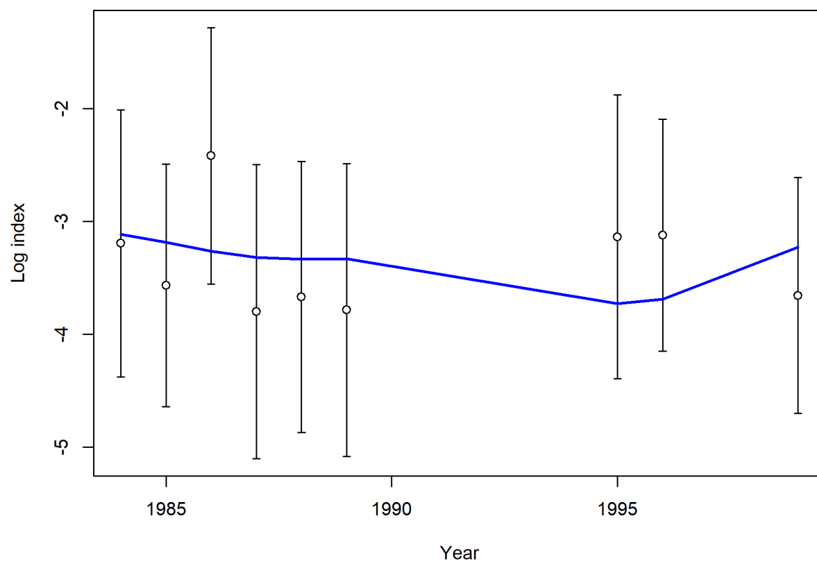
Figure 64: Fit to log index data on log scale for the recreational MRFSS dockside CPFV fishery north of Point Conception. Lines indicate 95% uncertainty interval around index values. Thicker lines indicate input uncertainty before addition of estimated additional uncertainty parameter.
