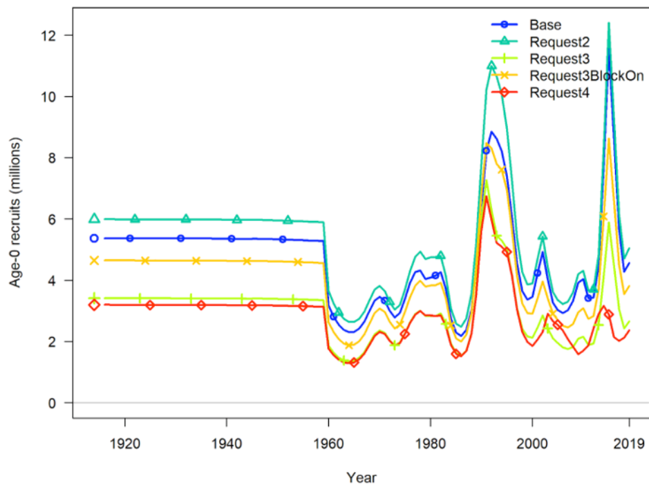
Figure 47: Comparison of time series of recruits from pre-STAR base model and models from requests 2, 3a and 4a.
