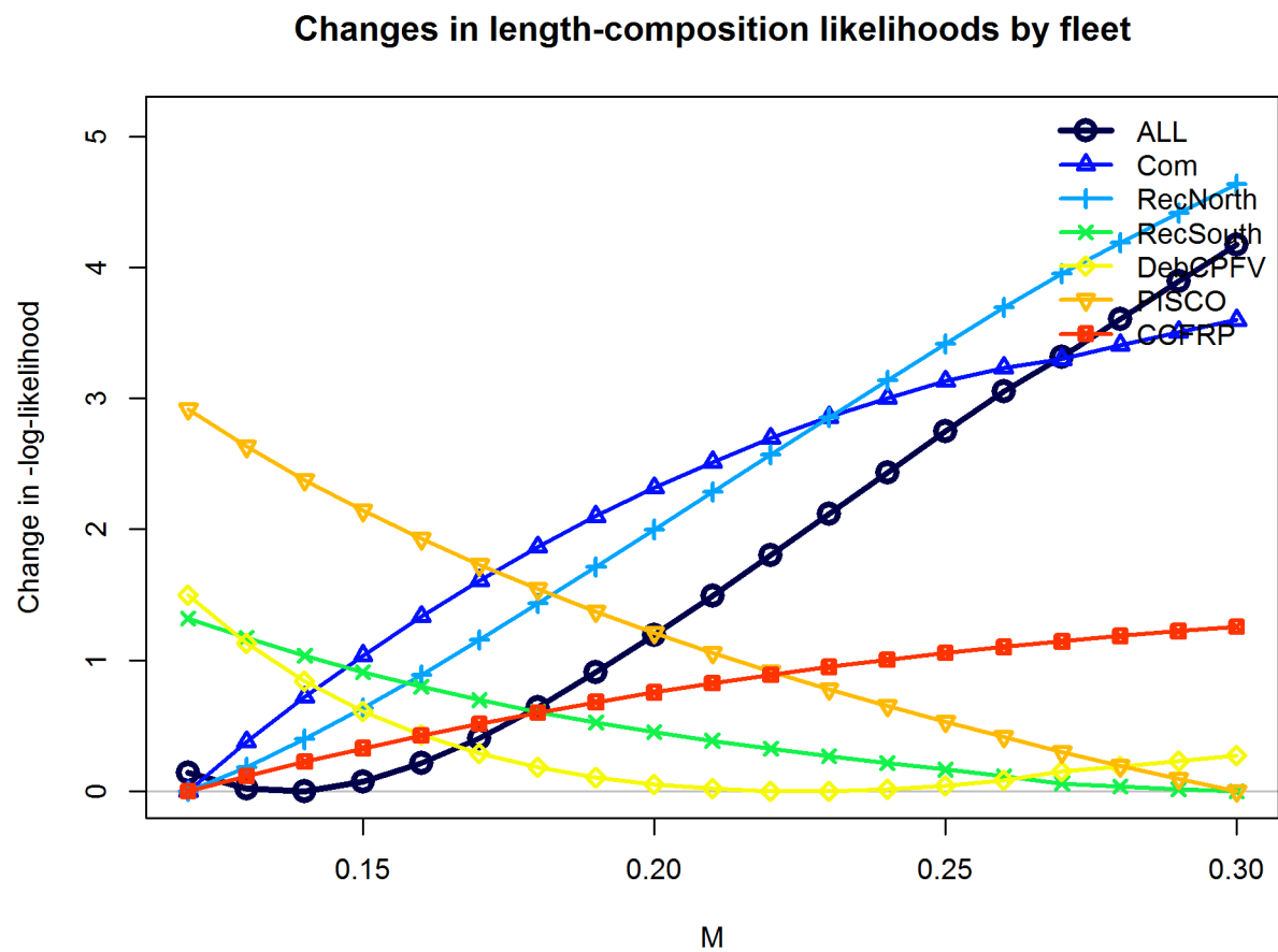
Figure 84: Likelihood profile across female natural mortality values by length composition.
