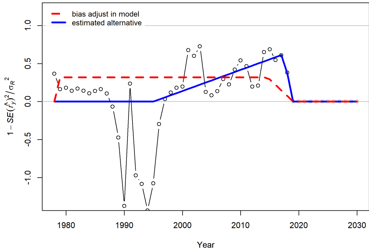
Figure 62: Bias adjustment for recruitment deviations. Points are transformed variances. Red line shows current settings for bias adjustment specified in the control file. Blue line shows the least squares estimate of alternative bias adjustment relationship for recruitment deviations.
