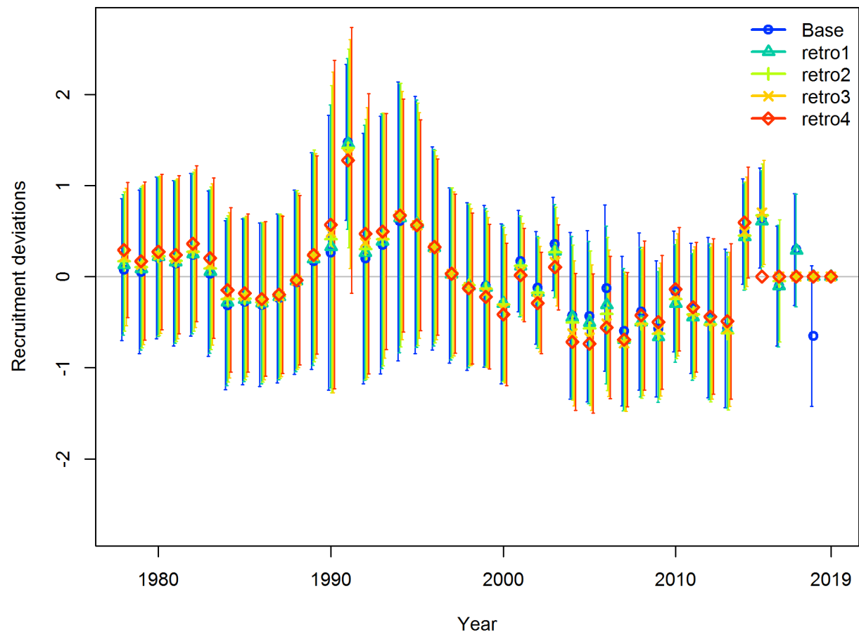
Figure 75: Retrospective pattern for estimated recruitment deviations.
