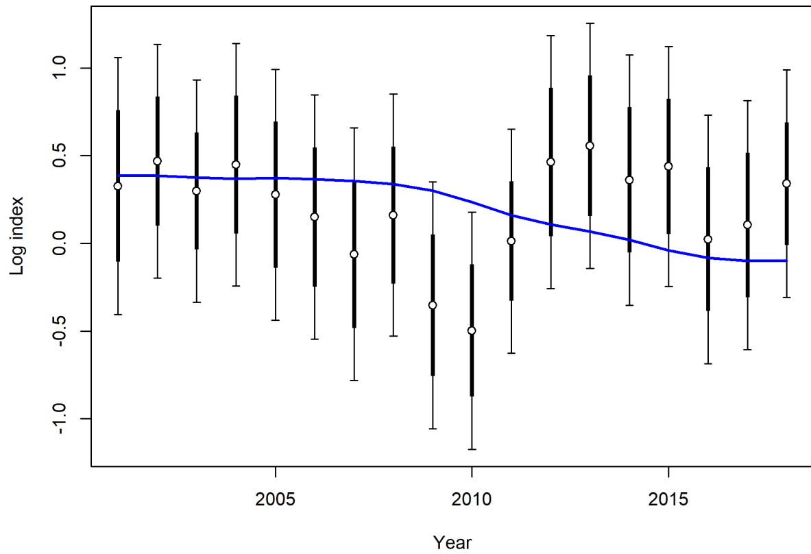
Figure 67: Fit to log index data on log scale for the fishery-independent PISCO kelp forest fish survey for fish 15 cm and larger. Lines indicate 95% uncertainty interval around index values. Thicker lines indicate input uncertainty before addition of estimated additional uncertainty parameter.
