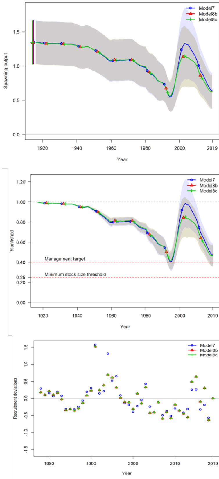
Figure 49: Results of request 7 and 8. Time series of absolute (top) and relative (middle) spawning output and recruitment deviations (now staring in 1978; bottom).
