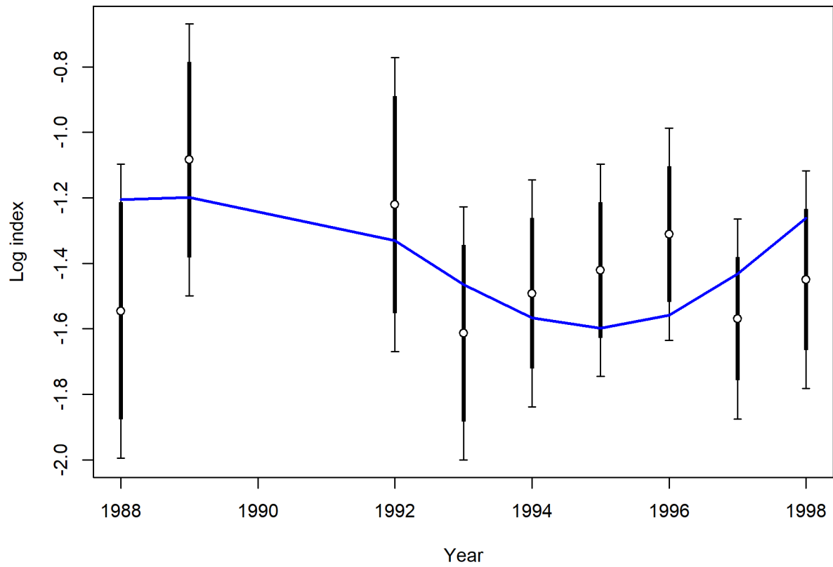
Figure 65: Fit to log index data on log scale for the recreational Deb's CPFV onboard observer program, representing north of Point Conception. Lines indicate 95% uncertainty interval around index values. Thicker lines indicate input uncertainty before addition of estimated additional uncertainty parameter.
