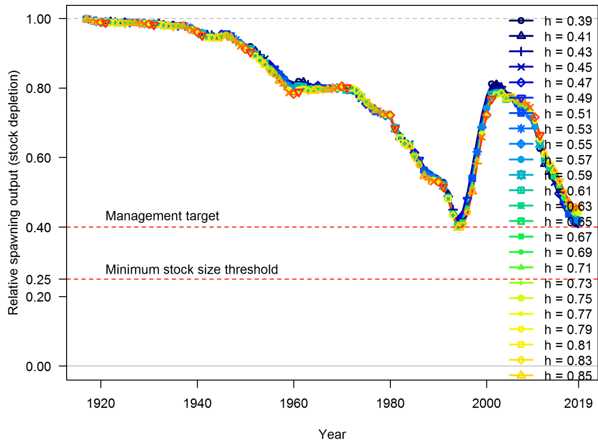
Figure 83: Trajectories of depletion across values of steepness.
