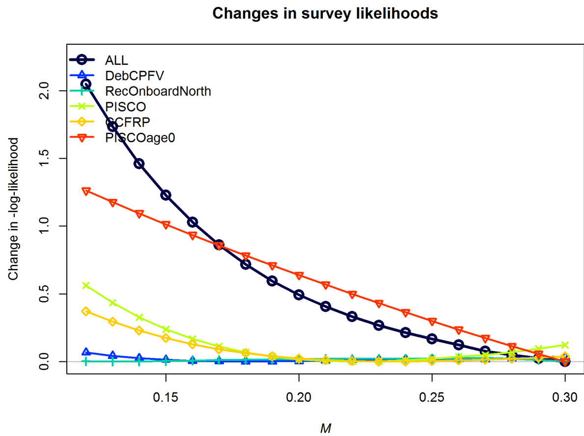
Figure 85: Likelihood profile across female natural mortality values by surveys.
