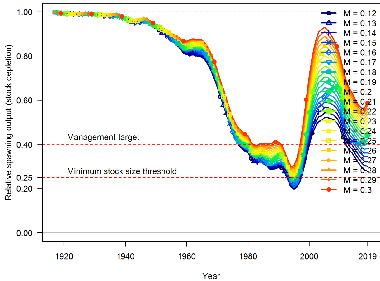
Figure 87: Trajectories of depletion across values of female natural mortality.
