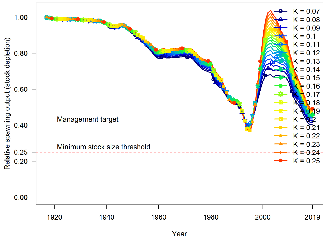
Figure 91: Trajectories of depletion across values of the growth parameter k .
