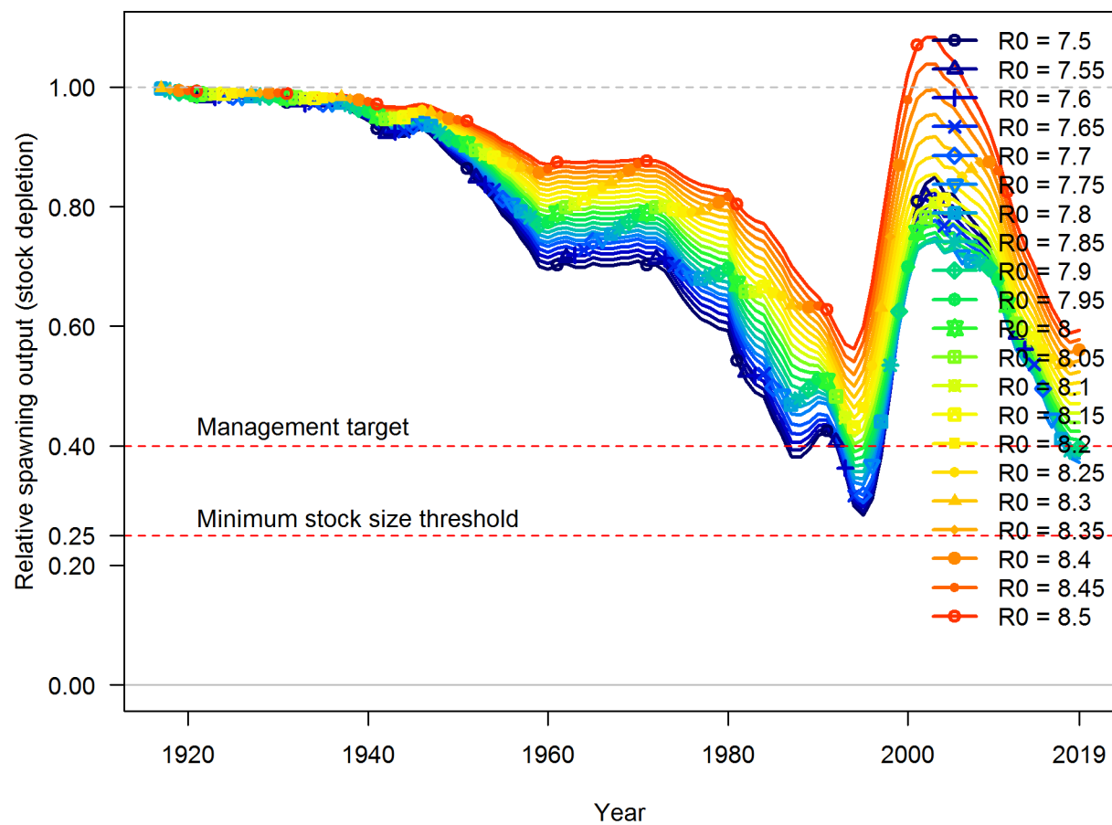
Figure 79: Trajectories of depletion across values of R_0 .
