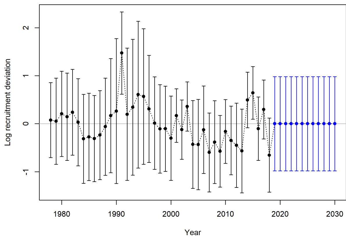
Figure 60: Estimated time-series of recruitment deviations for GBYR with 95% intervals.
