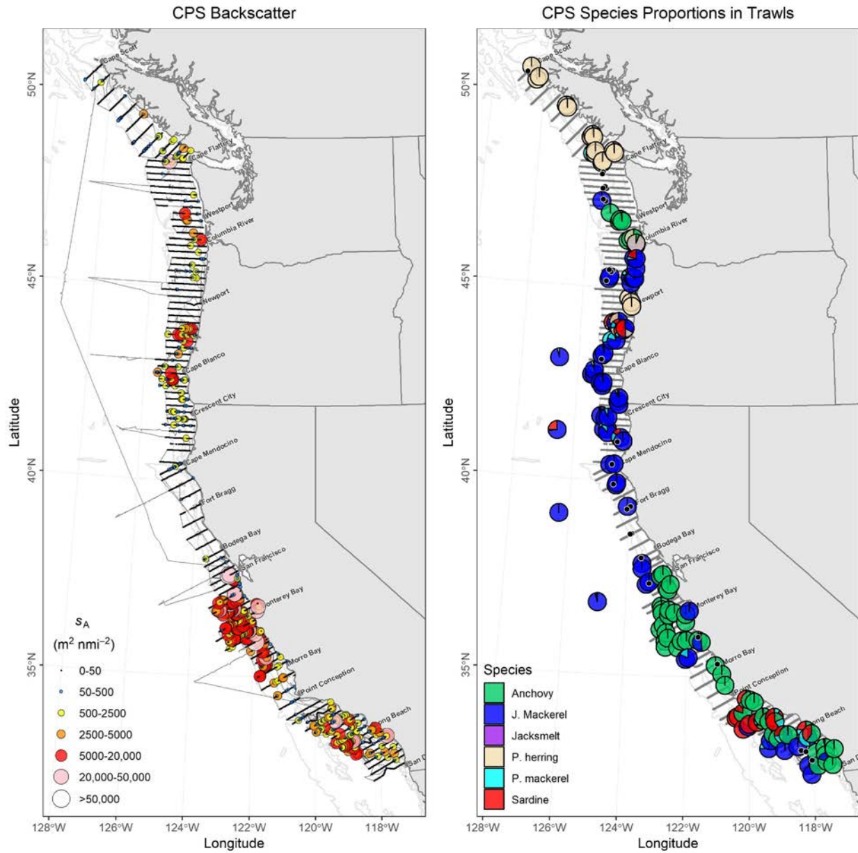
Fig. 7. Results from the AT survey for summer 2018 (Stierhoff et al. 2019b). A map of the distribution of 38-kHz integrated backscattering coefficients ( s_A , m^2 \text{ nmi}^{-2} ) averaged over 2,000-m distance intervals and from 5 to 70-m deep ascribed to CPS (left), and proportions of CPS in trawls (black points indicate trawls with no CPS (right)).
