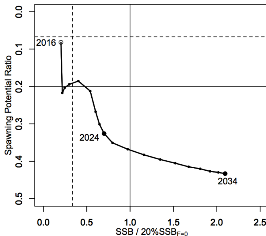
Figure 6-15. A projection result (scenario 1 from Table 4) for Pacific bluefin tuna ( Thunnus orientalis ) in a form of Kobe plot. The X axis shows the SSB value relative to 20%SSB F=0 (second rebuilding target) and the Y axis shows the spawning potential ratio as a measure of fishing intensity. Vertical and horizontal solid lines indicate the second rebuilding target (20%SSB F=0 ) and the corresponding fishing intensity, respectively, while vertical and horizontal dashed lines indicate the initial rebuilding target (SSB MED = 6.7%SSB F=0 ) and the corresponding fishing intensity, respectively.
