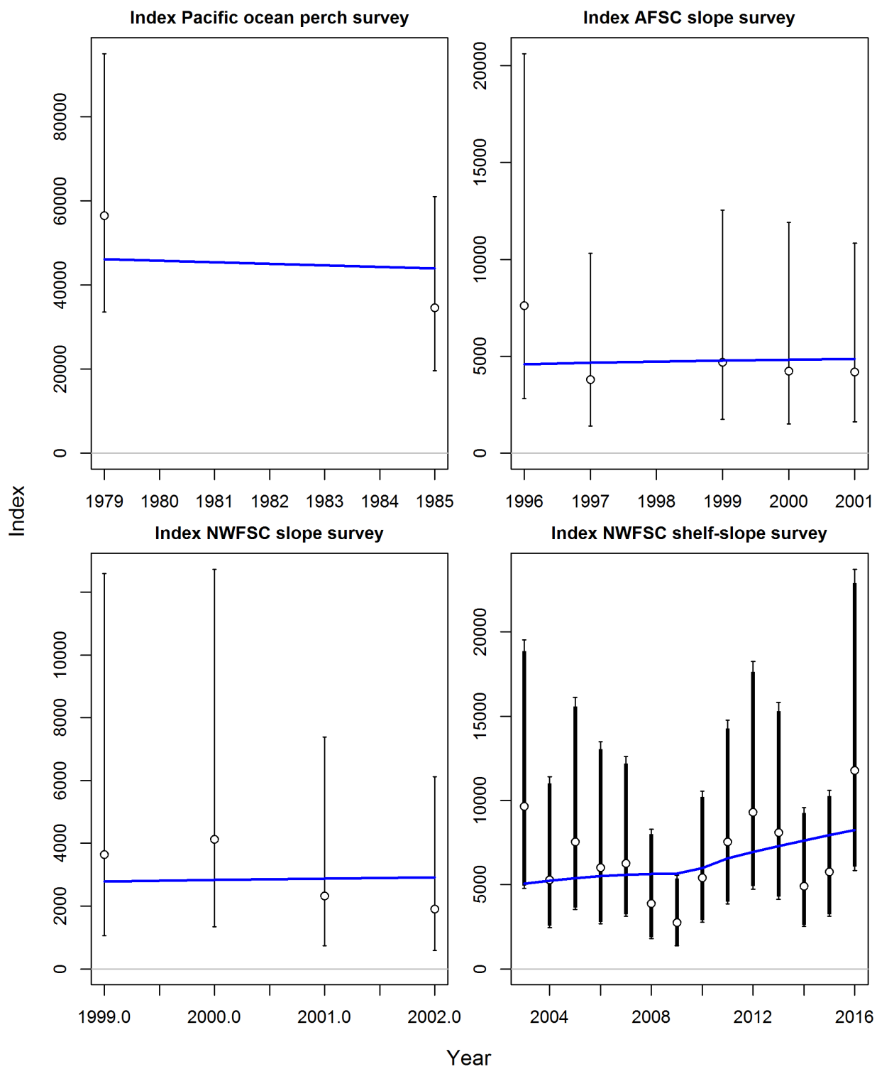
Figure 39: Estimated fits to the survey indices for Pacific ocean perch.
