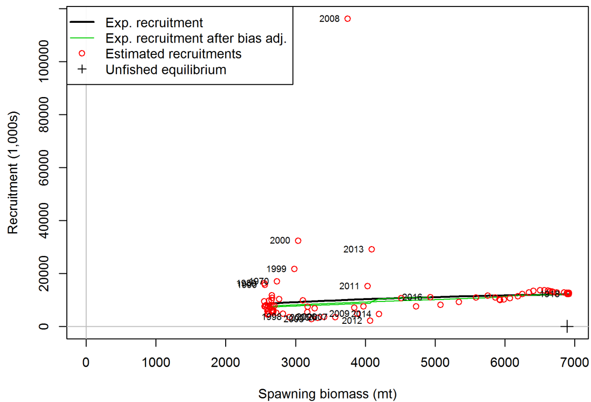
Figure 73: Estimated recruitment (red circles) and the assumed stock-recruit relationship (black line). The green line shows the effect of the bias correction for the lognormal distribution
