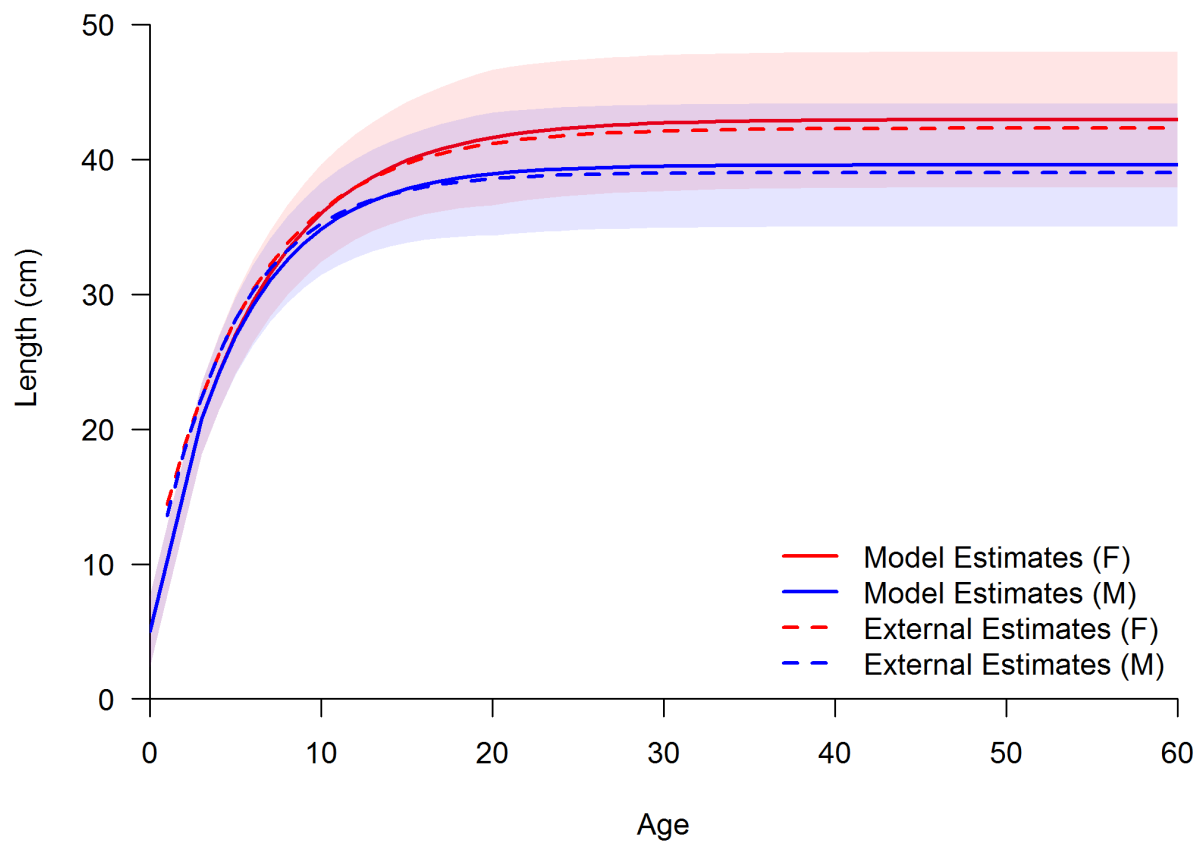
Figure 34: Comparison between the estimated length-at-age for male and female (solid lines) for Pacific ocean perch with estimated CV to the external estimates based on the data (dashed lines).
