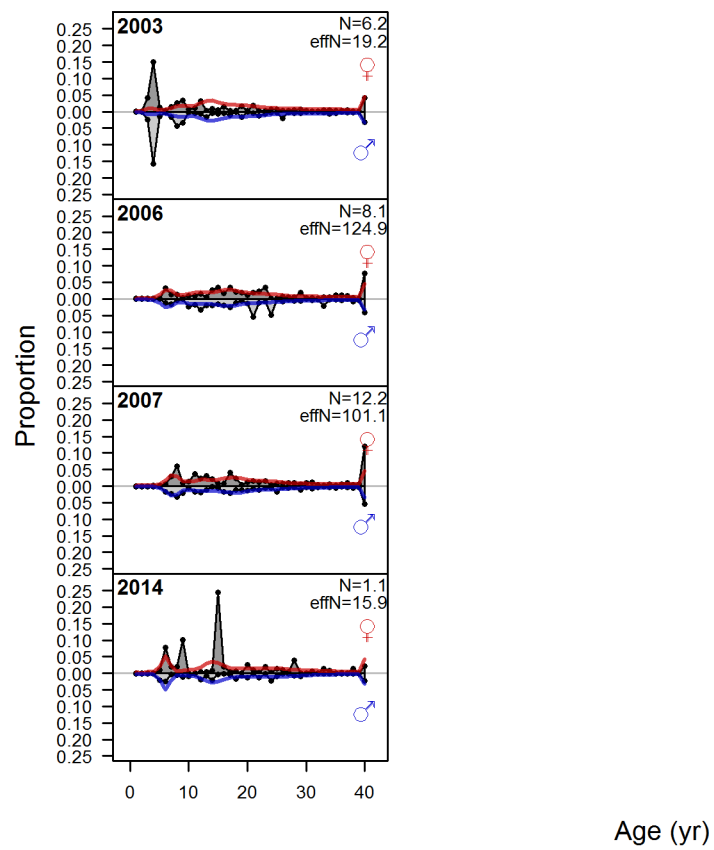
Figure 99: Age comps, whole catch, At_sea hake
