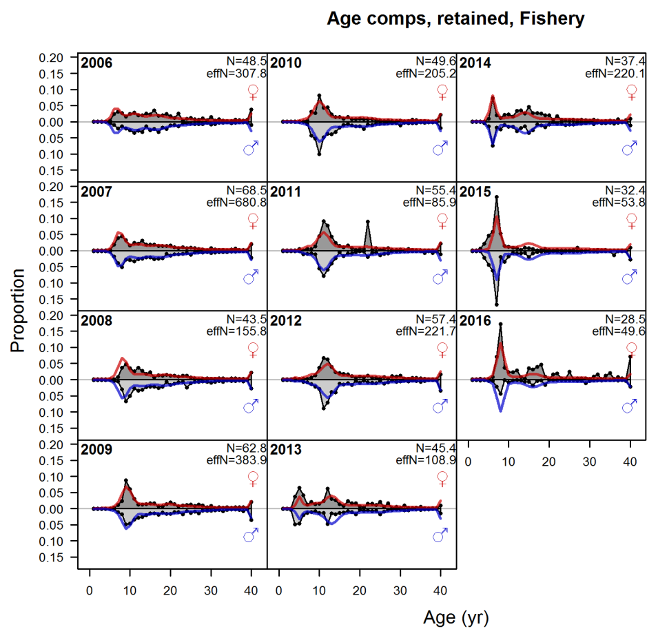
Figure 98: Age comps, retained, Fishery (plot 2 of 2)
