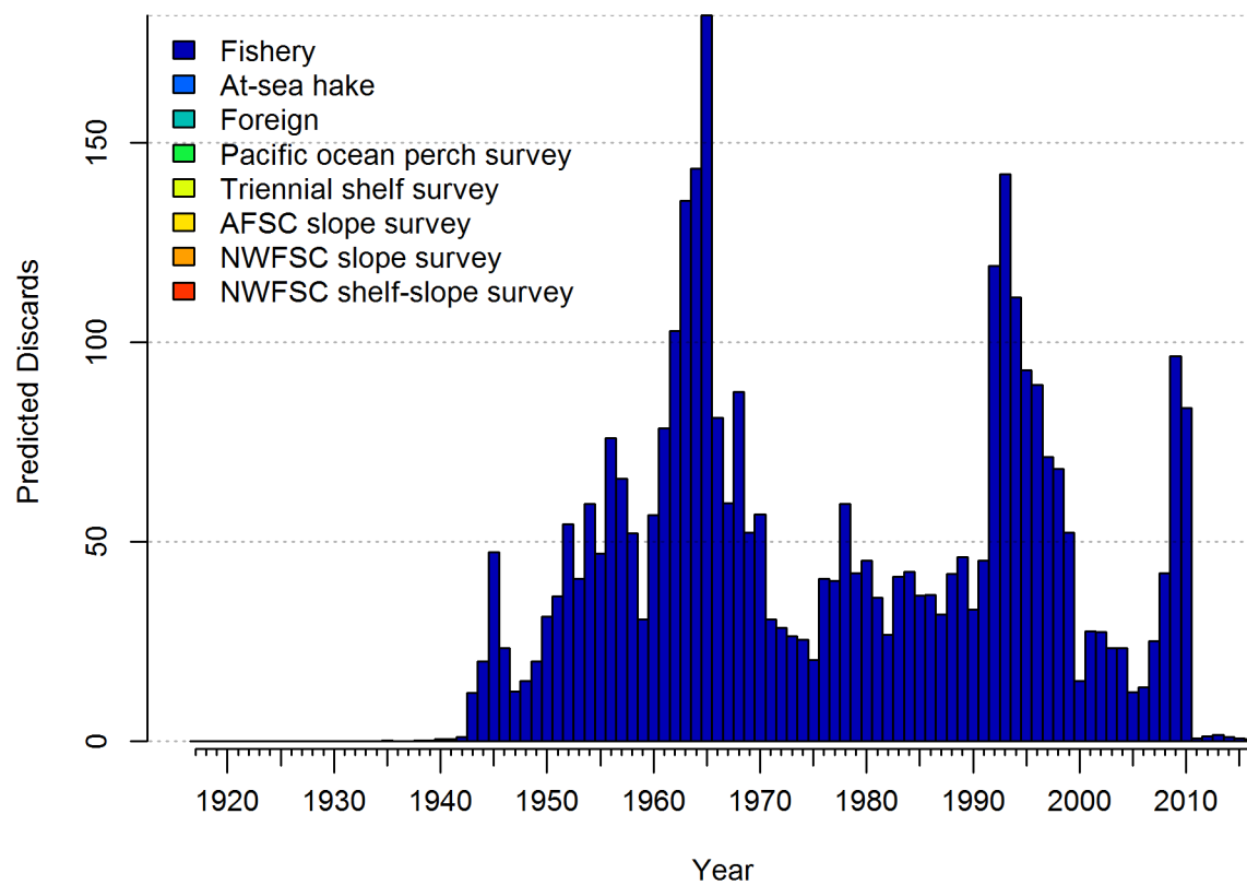
Figure 41: Estimated total discards for Pacific ocean perch. Estimated discard contributes less than 3.5 percent of the total mortality across all years from the fishery.
