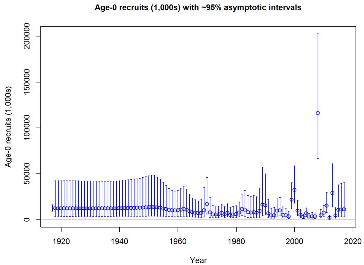
Figure 37: Estimated time-series of recruitment for Pacific ocean perch.
