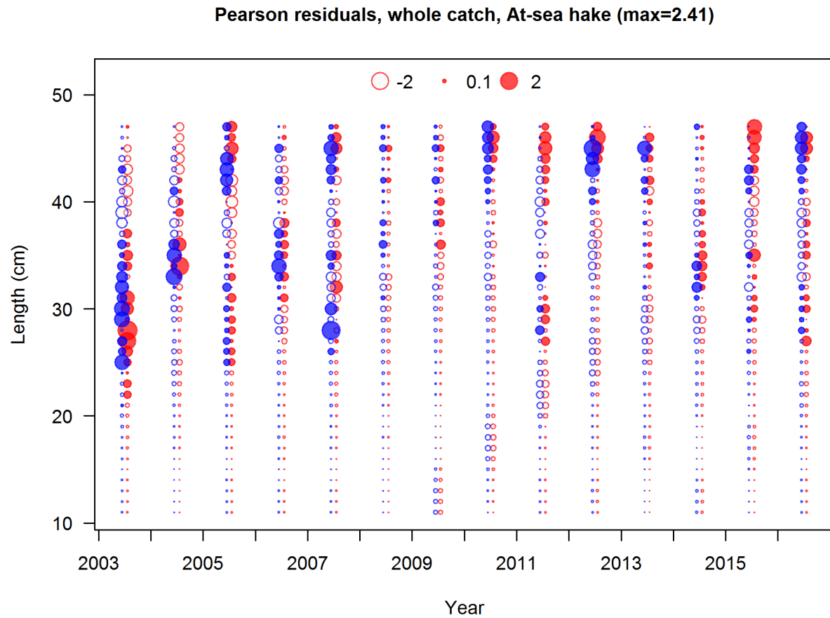
Figure 45: Pearson residuals, whole catch, At-sea hake (max=2.41) Closed bubbles are positive residuals (observed > expected) and open bubbles are negative residuals (observed < expected).
