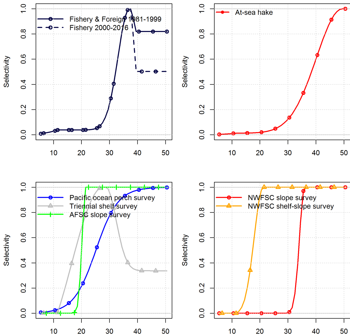
Figure 35: Estimated selectivity by length by each fishery and survey for Pacific ocean perch. The Triennial selectivity was fixed at the estimated selectivity from preliminary models using the Triennial data. The final selectivity was only used to remove Triennial catch from the population.
