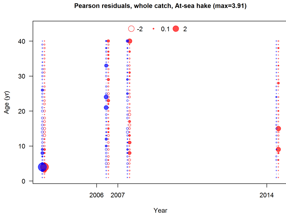
Figure 58: Pearson residuals, whole catch, At-sea hake (max=3.91) Closed bubbles are positive residuals (observed > expected) and open bubbles are negative residuals (observed < expected).
