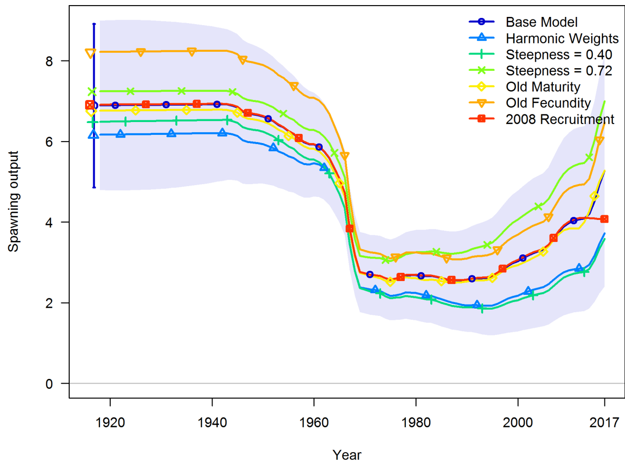
Figure 74: Time-series of spawning output for model sensitivities for Pacific ocean perch.
