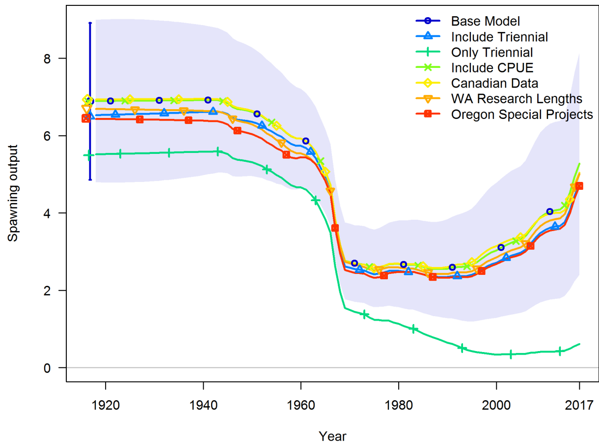
Figure 76: Time-series of spawning output for model sensitivities for Pacific ocean perch.
