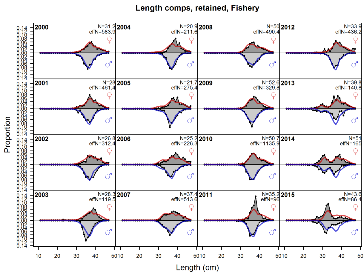
Figure 90: Length comps, retained, Fishery (plot 3 of 4)
