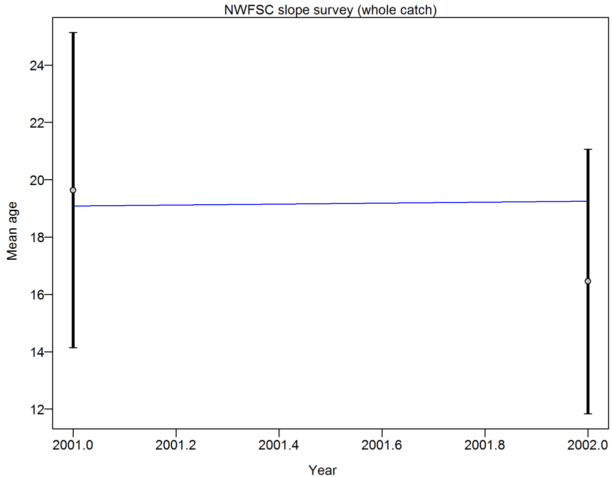
Figure 68: Mean age for NWFSC slope survey with 95% confidence intervals based on current samples sizes. Francis data weighting method TA1.8: thinner intervals (with capped ends) show result of further adjusting sample sizes based on suggested multiplier (with 95% interval) for age data from NWFSC slope survey: 1.0004 (1.0004_Inf) For more info, see Francis, R.I.C.C. (2011). Data weighting in statistical fisheries stock assessment models. Can. J. Fish. Aquat. Sci. 68: 1124_1138.
