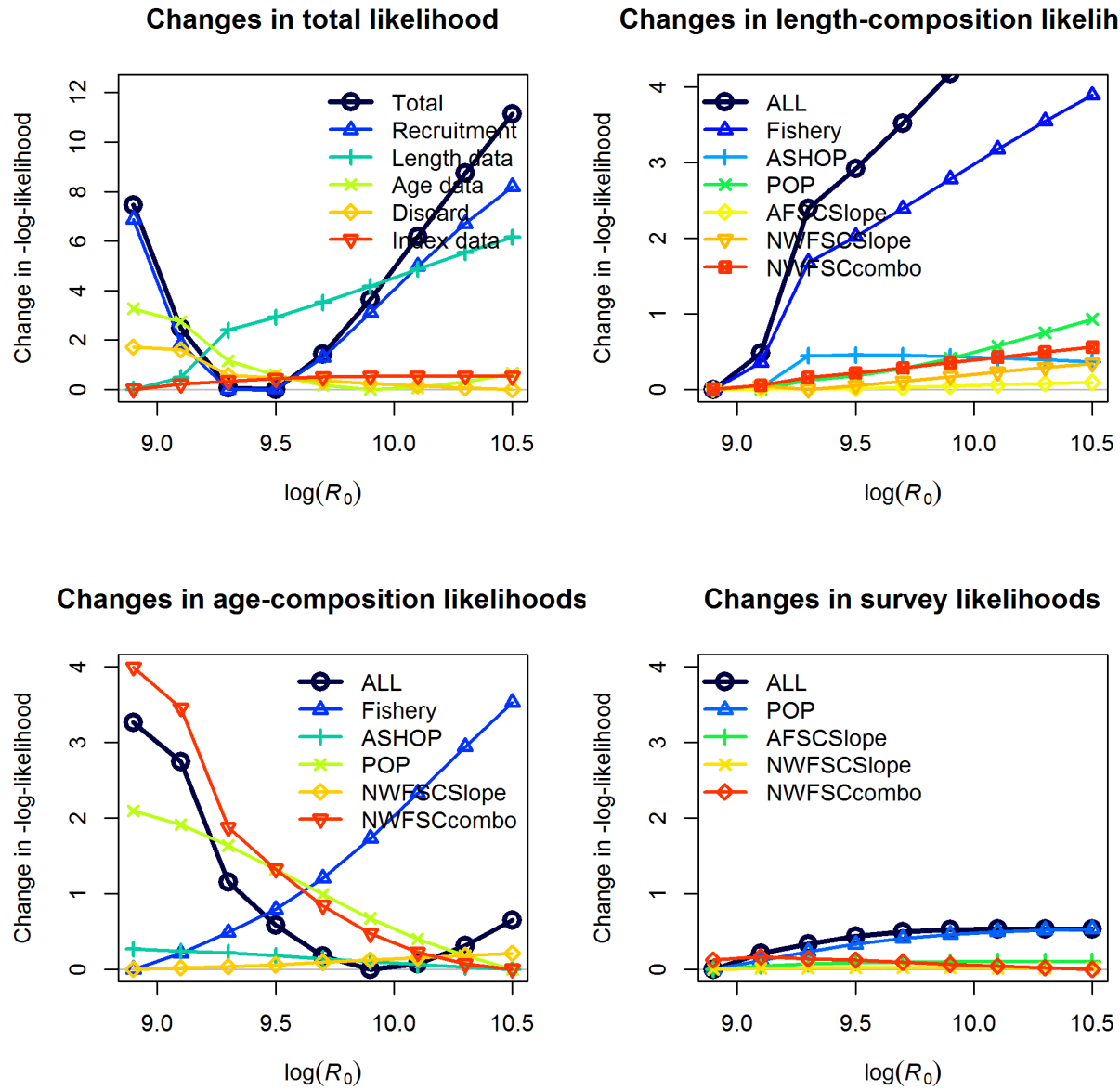
Figure 84: Likelihood profile across R_0 values.
