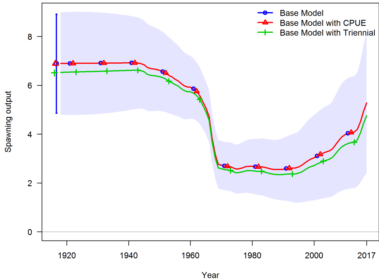
Figure 105: Plot comparison of spawning output when either the fishery CPUE or the Triennial shelf survey data are included in the base model for Pacific ocean perch.
