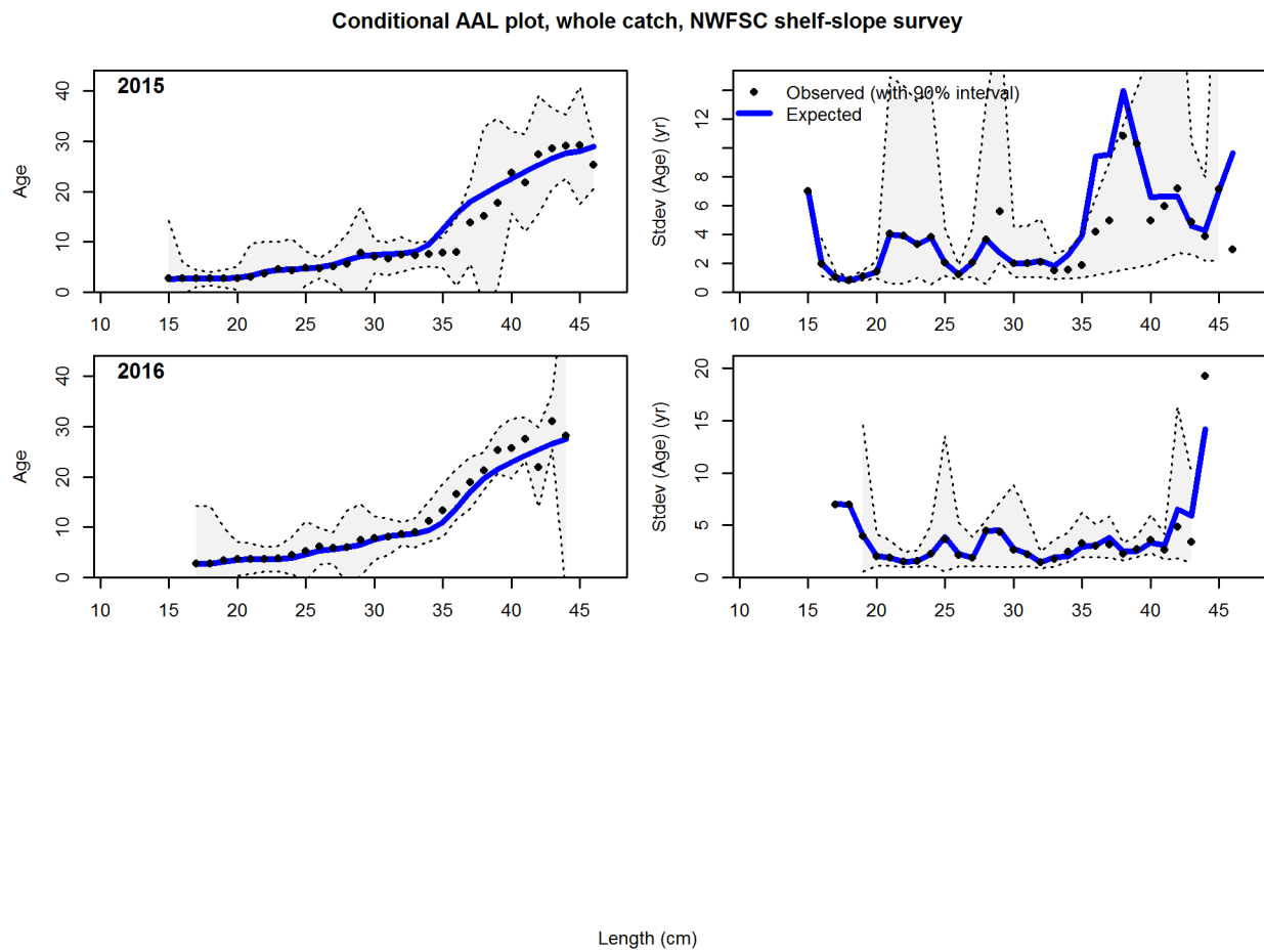
Figure 65: Conditional AAL plot, whole catch, NWFSC shelf_slope survey (plot 5 of 5)
