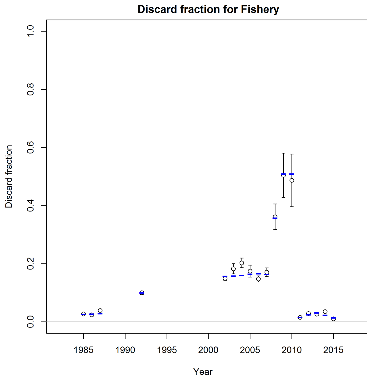
Figure 40: Estimated fits to the discard rates for Pacific ocean perch.
