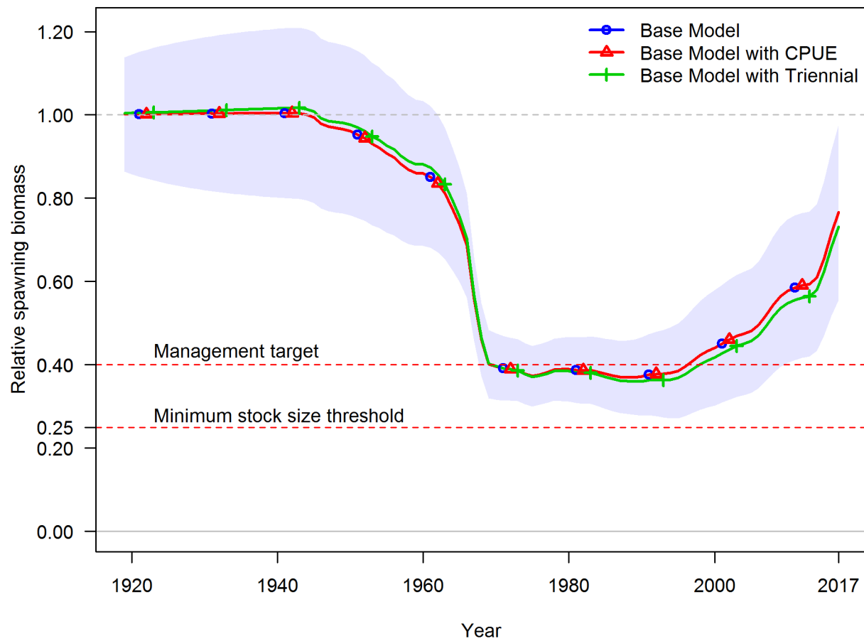
Figure 106: Plot comparison of relative spawning output (depletion) when either the fishery CPUE or the Triennial shelf survey data are included in the base model for Pacific ocean perch.
