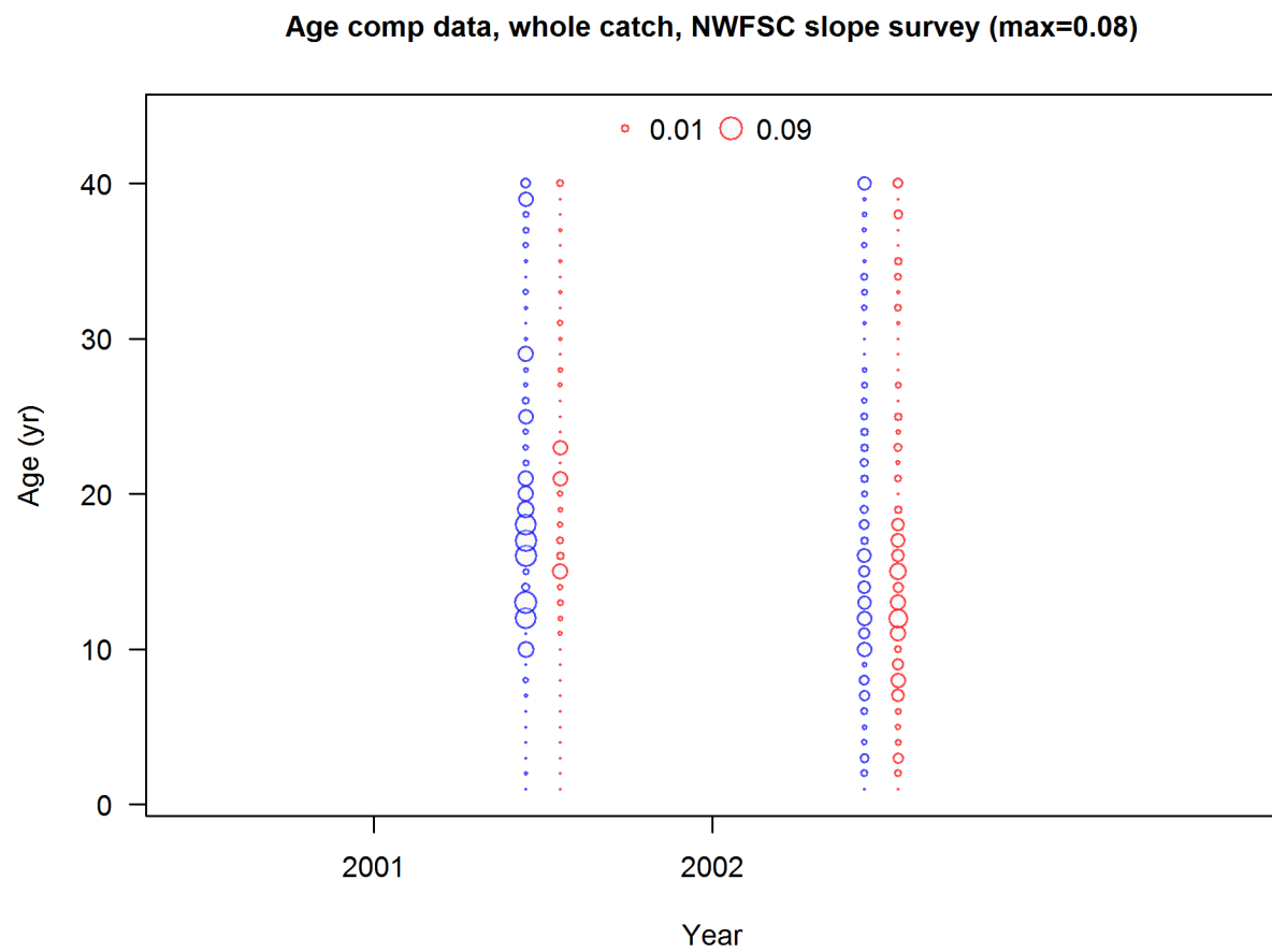
Figure 9: NWFSC slope survey age frequency distributions for Pacific ocean perch.
