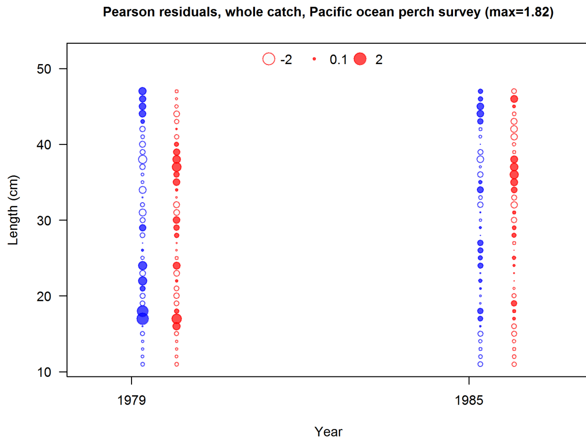
Figure 46: Pearson residuals, whole catch, Pacific ocean perch survey (max=1.82) Closed bubbles are positive residuals (observed > expected) and open bubbles are negative residuals (observed < expected).
