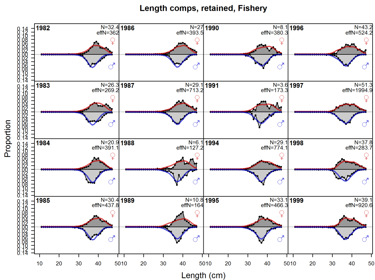
Figure 89: Length comps, retained, Fishery (plot 2 of 4)
