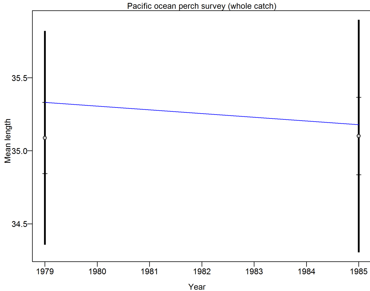
Figure 52: Mean length for Pacific ocean perch survey with 95% confidence intervals based on current samples sizes. Francis data weighting method TA1.8: thinner intervals (with capped ends) show result of further adjusting sample sizes based on suggested multiplier (with 95% interval) for len data from Pacific ocean perch survey: 9.0018 (9.0018_Inf) For more info, see Francis, R.I.C.C. (2011). Data weighting in statistical fisheries stock assessment models. Can. J. Fish. Aquat. Sci. 68: 1124_1138.
