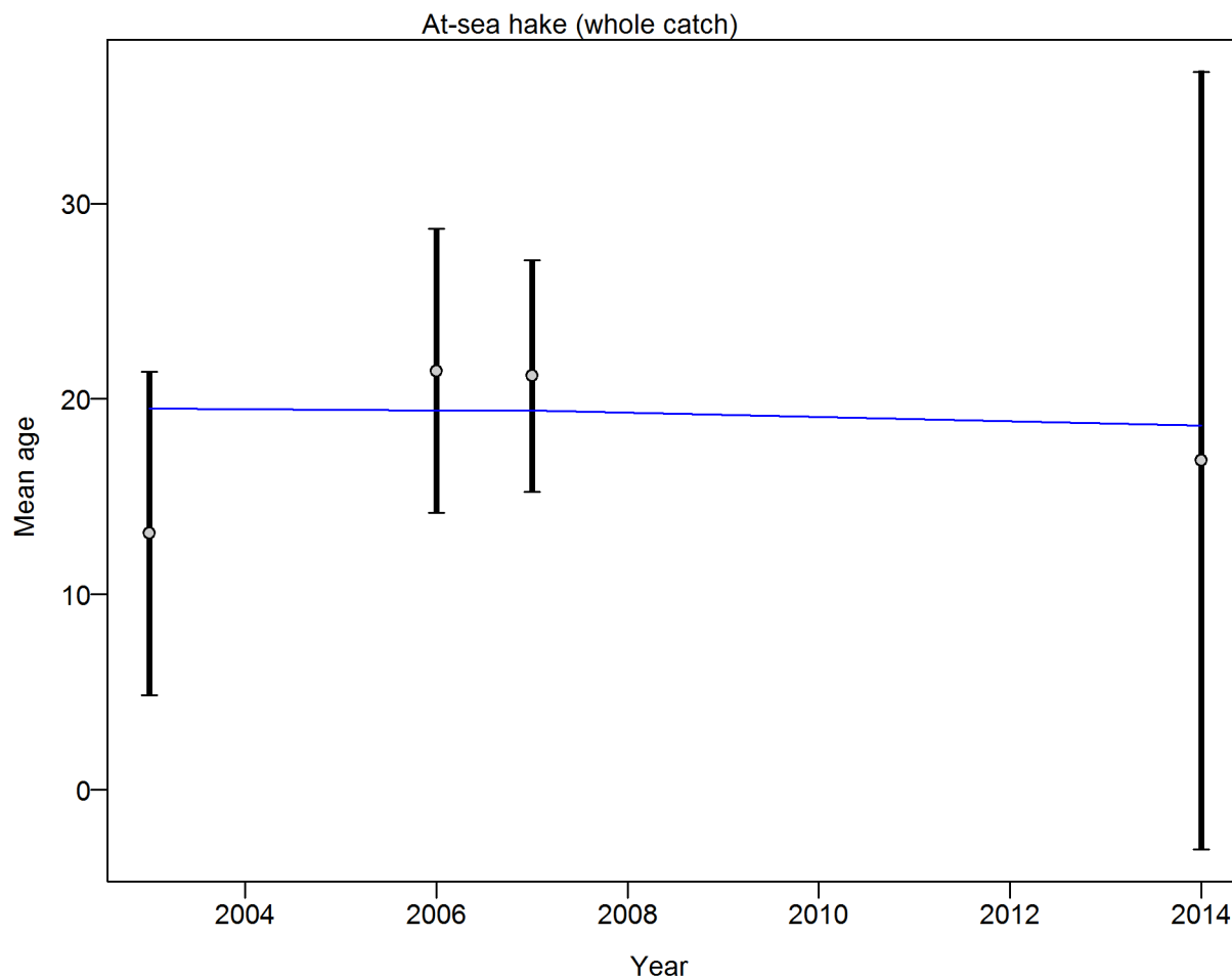
Figure 67: Mean age for At-sea hake with 95% confidence intervals based on current samples sizes. Francis data weighting method TA1.8: thinner intervals (with capped ends) show result of further adjusting sample sizes based on suggested multiplier (with 95% interval) for age data from At-sea hake: 1.0068 (0.6598_2756.7898) For more info, see Francis, R.I.C.C. (2011). Data weighting in statistical fisheries stock assessment models. Can. J. Fish. Aquat. Sci. 68: 1124_1138.
