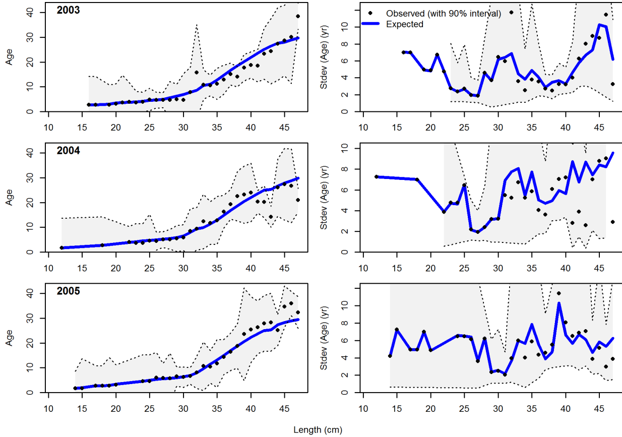
Figure 61: Conditional AAL plot, whole catch, NWFSC shelf_slope survey (plot 1 of 5) These plots show mean age and std. dev. in conditional AAL. Left plots are mean AAL by size_class (obs. and pred.) with 90% CIs based on adding 1.64 SE of mean to the data. Right plots in each pair are SE of mean AAL (obs. and pred.) with 90% CIs based on the chi-square distribution.
