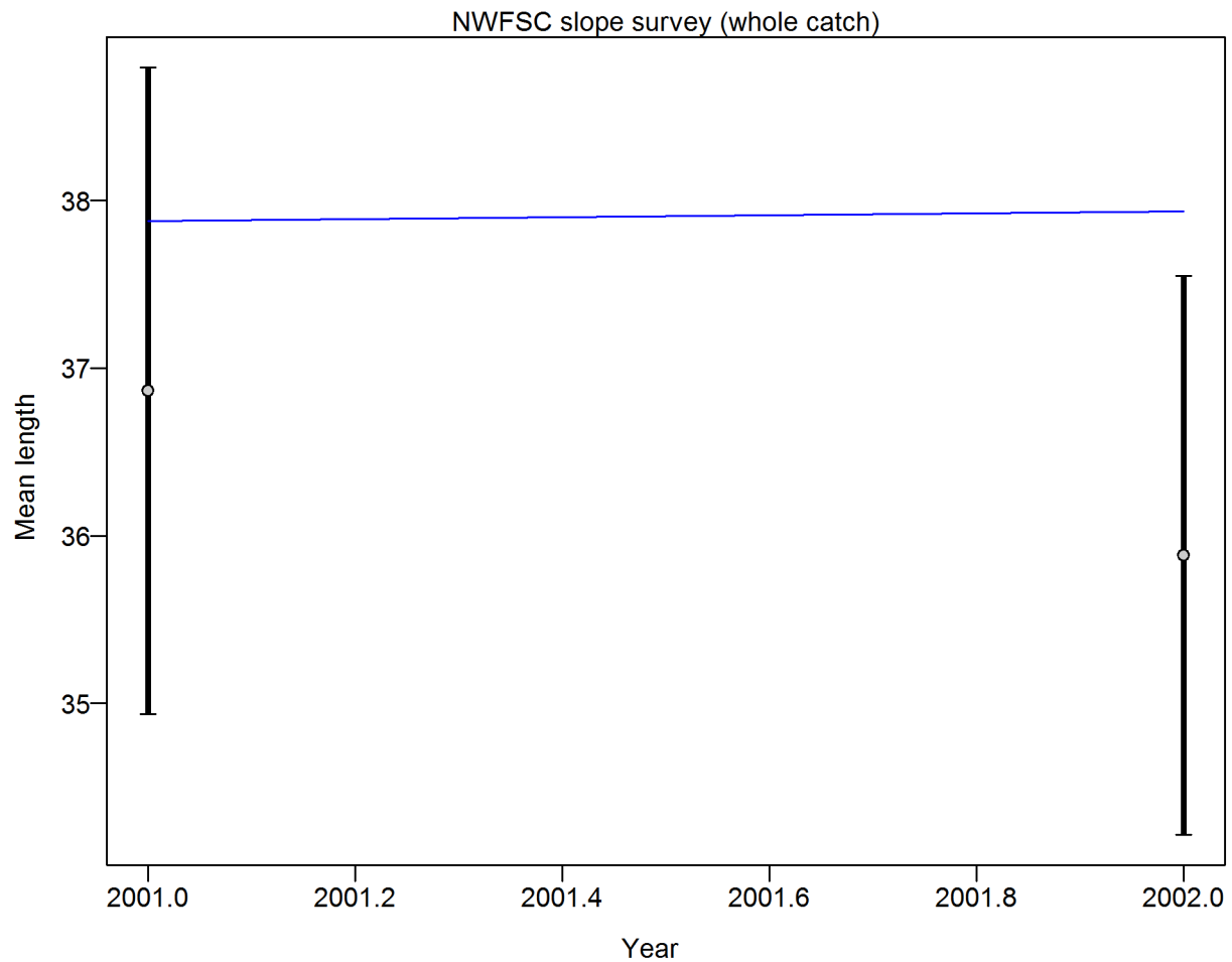
Figure 54: Mean length for NWFSC slope survey with 95% confidence intervals based on current samples sizes. Francis data weighting method TA1.8: thinner intervals (with capped ends) show result of further adjusting sample sizes based on suggested multiplier (with 95% interval) for len data from NWFSC slope survey: 0.9971 (0.9971_Inf) For more info, see Francis, R.I.C.C. (2011). Data weighting in statistical fisheries stock assessment models. Can. J. Fish. Aquat. Sci. 68: 1124_1138.
