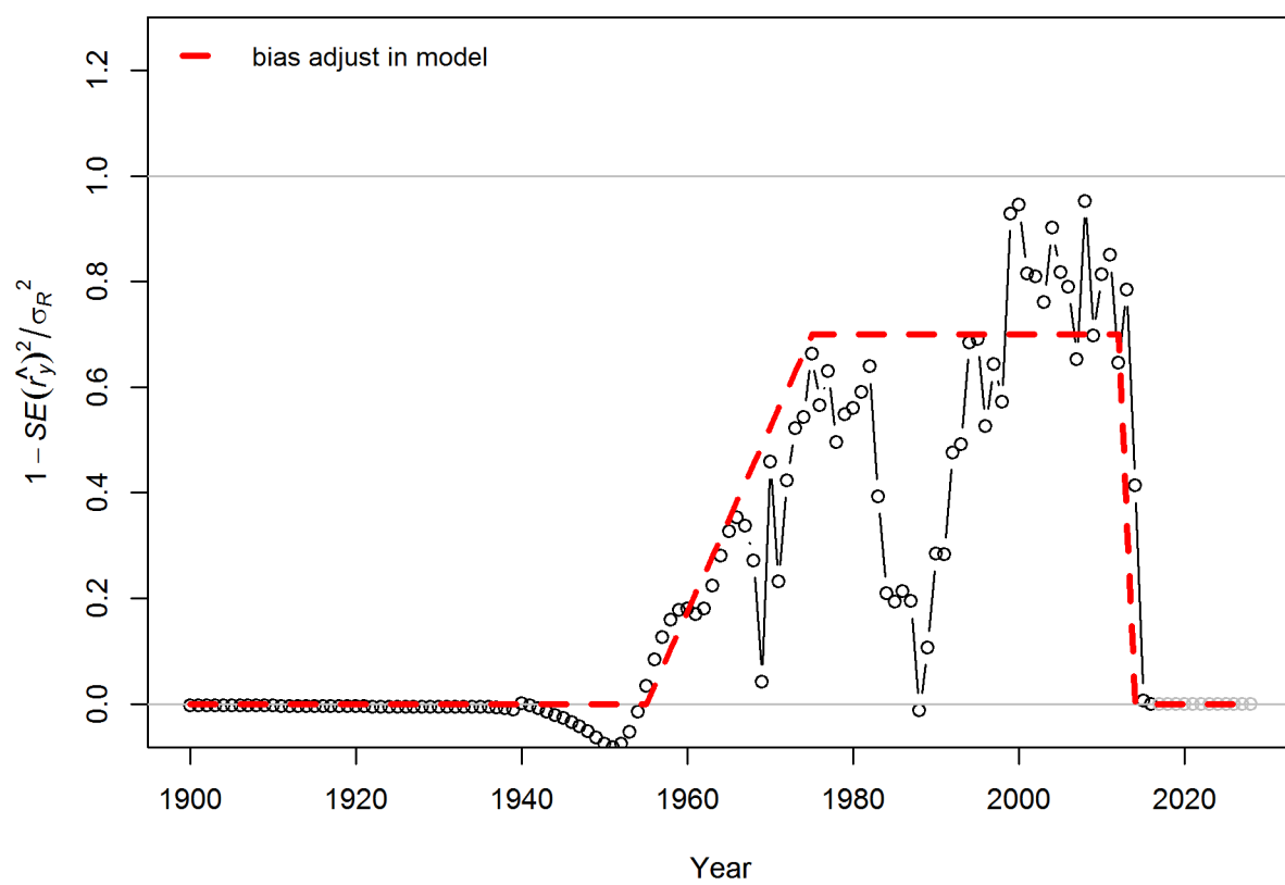
Figure 29: Recruitment bias ramp applied in the base model.
