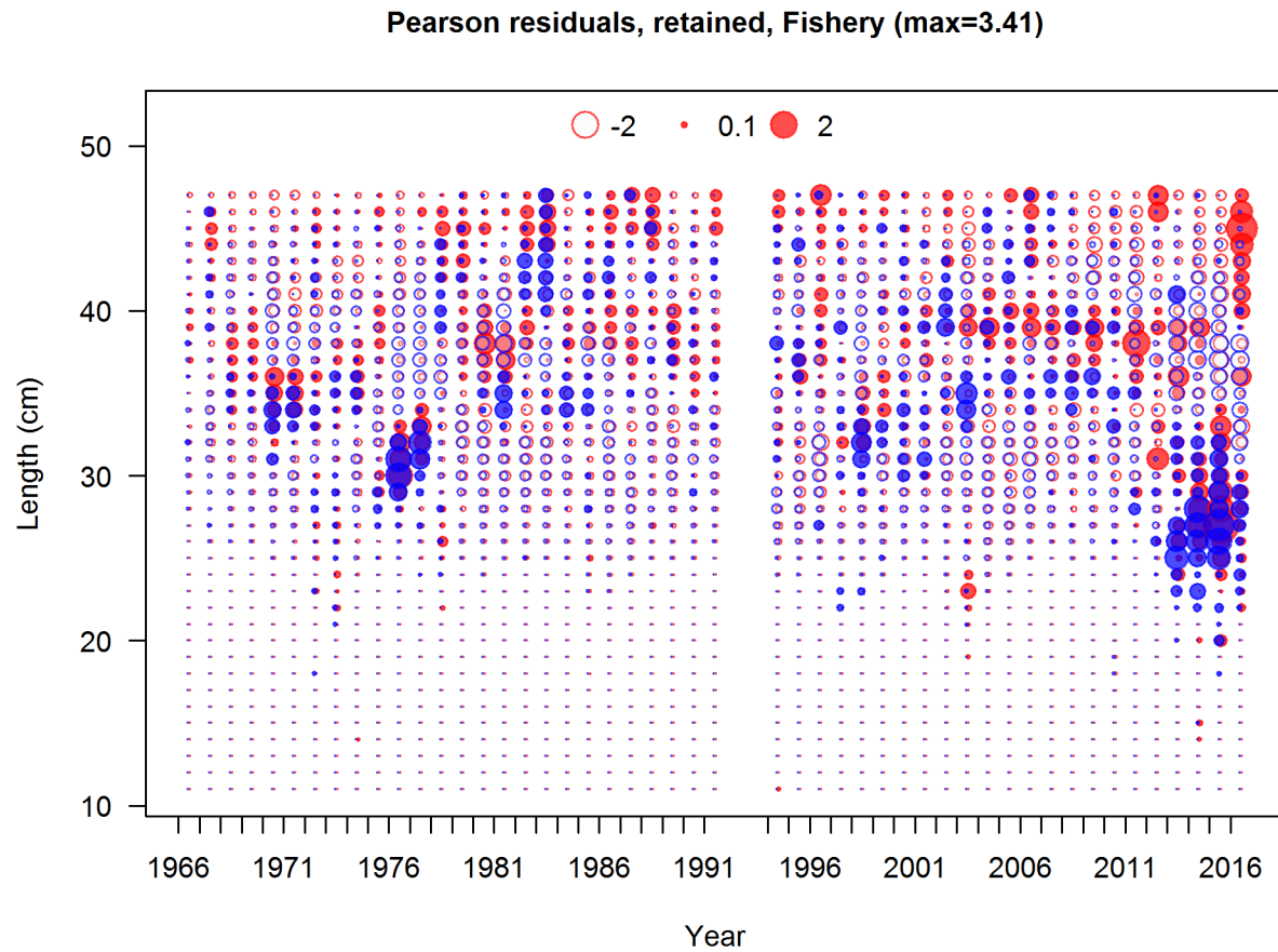
Figure 44: Pearson residuals, retained, Fishery (max=3.41) Closed bubbles are positive residuals (observed > expected) and open bubbles are negative residuals (observed < expected).
