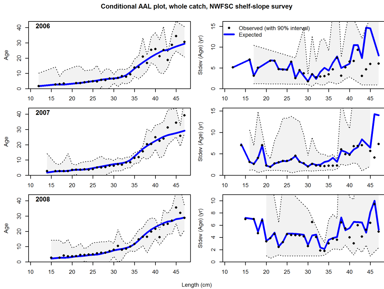
Figure 62: Conditional AAL plot, whole catch, NWFSC shelf_slope survey (plot 2 of 5)
