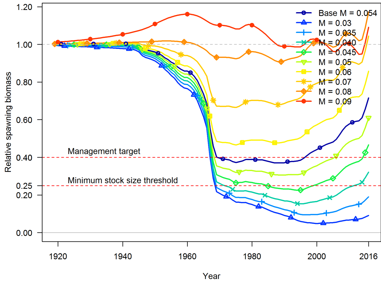
Figure 83: Trajectories of relative spawning output (depletion) across values of natural mortality.
