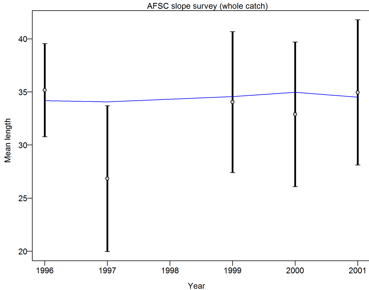
Figure 53: Mean length for AFSC slope survey with 95% confidence intervals based on current samples sizes. Francis data weighting method TA1.8: thinner intervals (with capped ends) show result of further adjusting sample sizes based on suggested multiplier (with 95% interval) for len data from AFSC slope survey: 0.9963 (0.5782_16.165) For more info, see Francis, R.I.C.C. (2011). Data weighting in statistical fisheries stock assessment models. Can. J. Fish. Aquat. Sci. 68: 1124_1138.
