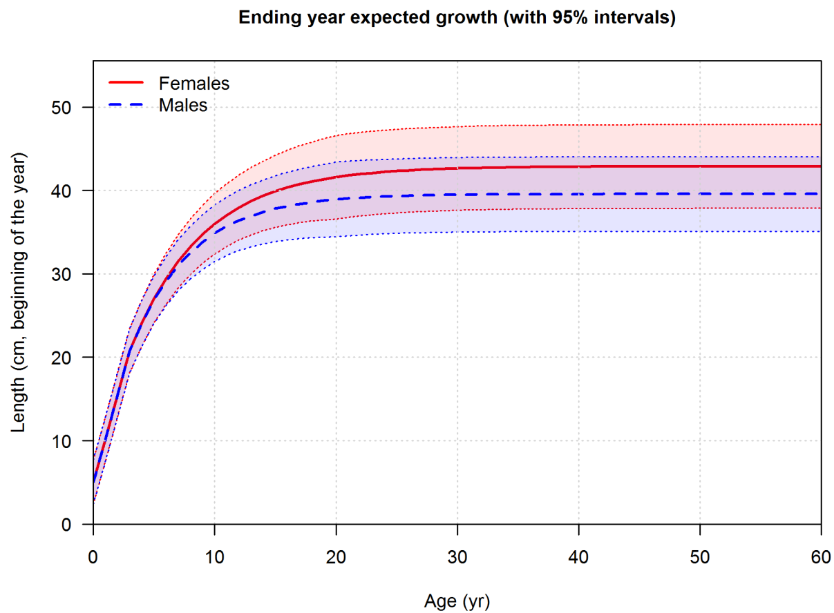
Figure 33: Estimated length-at-age for male and female for Pacific ocean perch with estimated CV.
