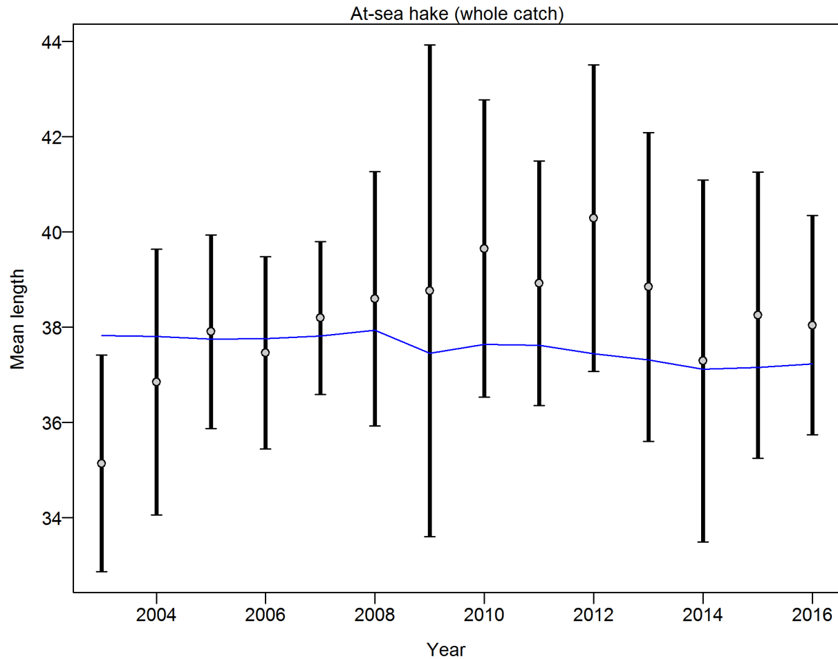
Figure 51: Mean length for At-sea hake with 95% confidence intervals based on current samples sizes. Francis data weighting method TA1.8: thinner intervals (with capped ends) show result of further adjusting sample sizes based on suggested multiplier (with 95% interval) for len data from At-sea hake: 0.9939 (0.4994_5.6181) For more info, see Francis, R.I.C.C. (2011). Data weighting in statistical fisheries stock assessment models. Can. J. Fish. Aquat. Sci. 68: 1124_1138.
