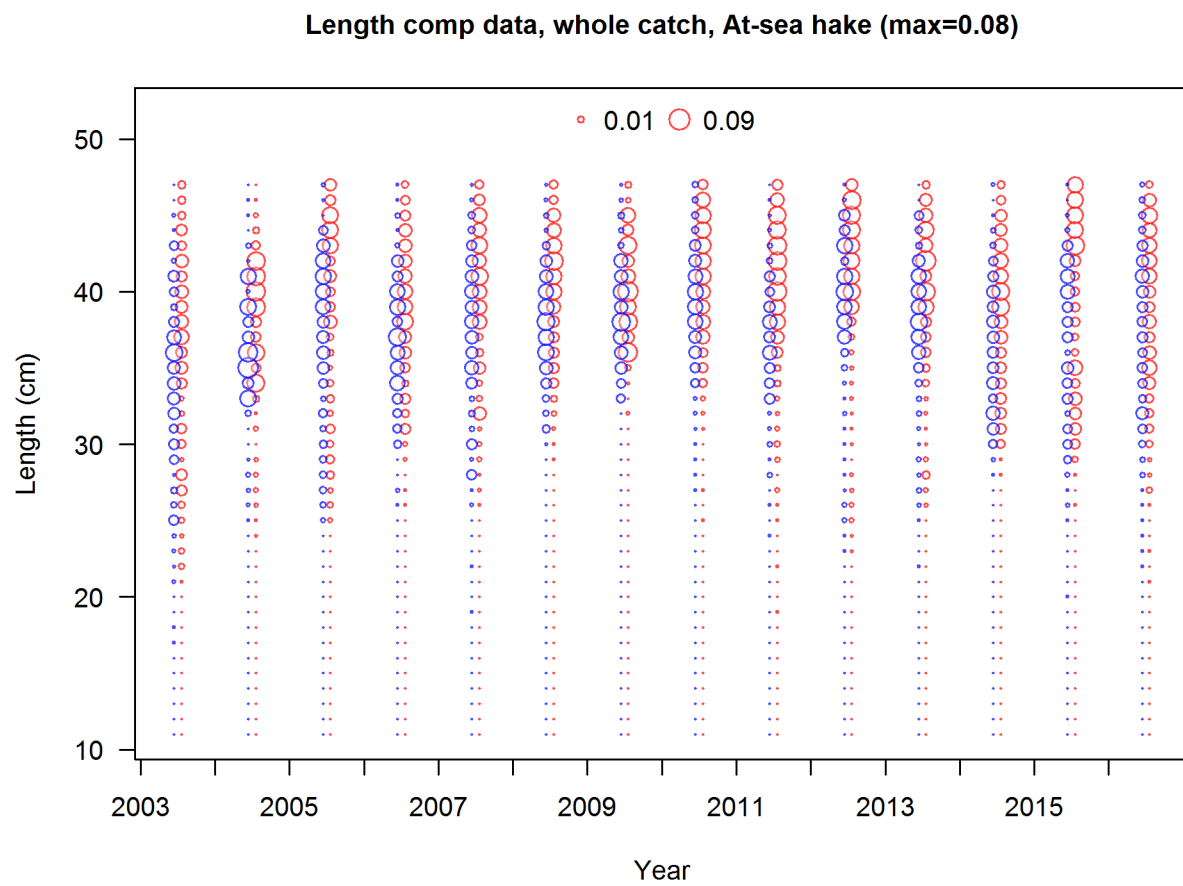
Figure 18: At-sea hake fishery length frequency distributions for Pacific ocean perch.
