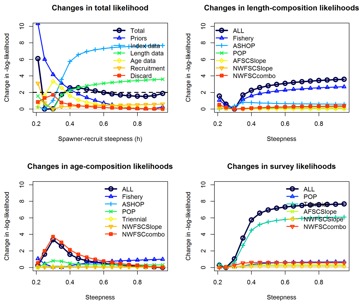
Figure 107: Profile over steepness with the inclusion of the Triennial shelf survey when treated as a single time-series for Pacific ocean perch.
