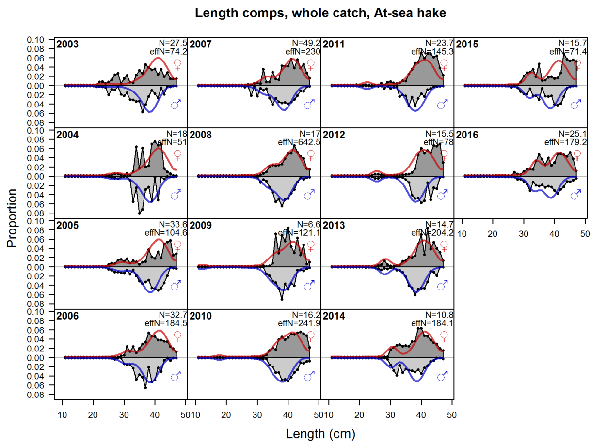
Figure 92: Length comps, whole catch, At-sea hake
