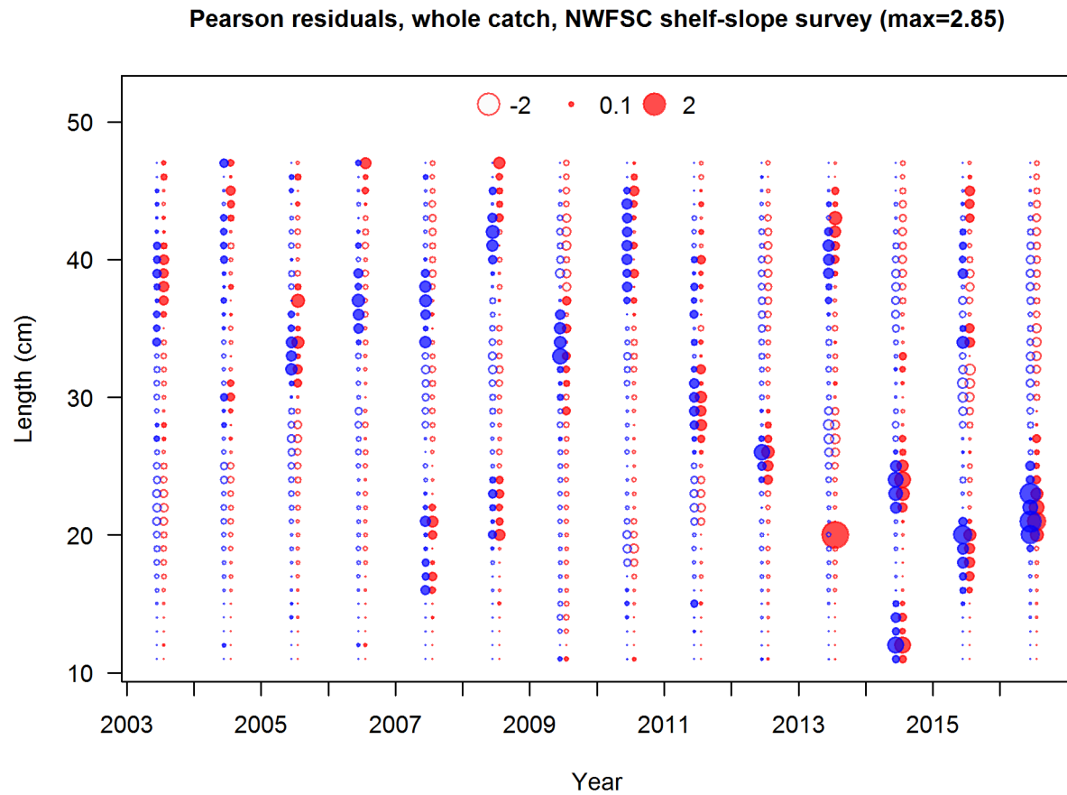
Figure 49: Pearson residuals, whole catch, NWFSC shelf_slope survey (max=2.85) Closed bubbles are positive residuals (observed > expected) and open bubbles are negative residuals (observed < expected).
