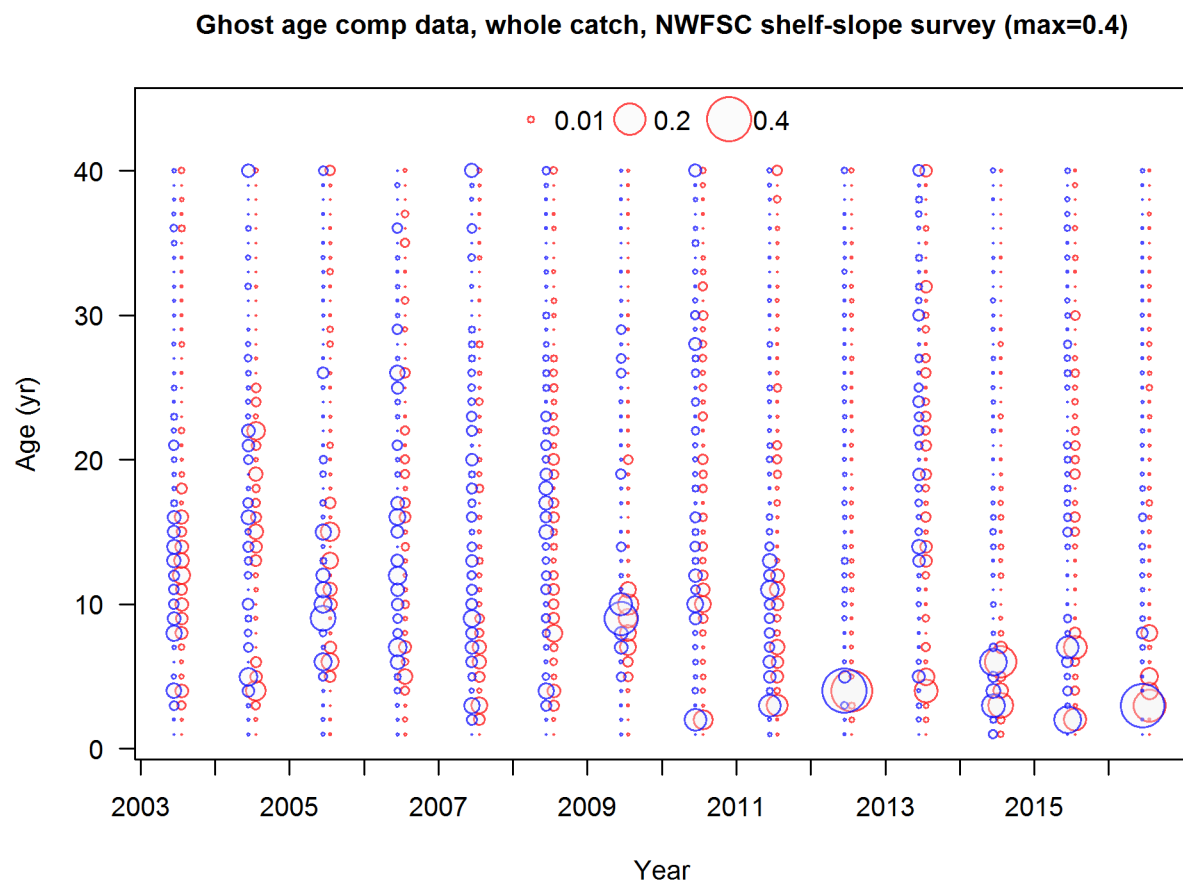
Figure 6: NWFSC shelf-slope survey age frequency distributions for Pacific ocean perch.
