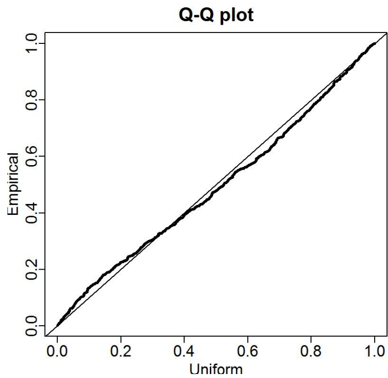
Figure 4: Q-Q plots for the VAST lognormal distribution for the NWFSC shelf-slope survey.
