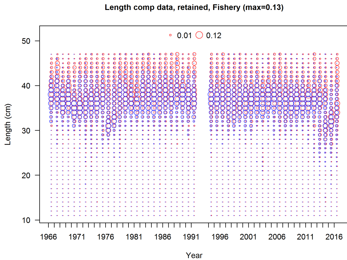
Figure 16: Commercial fishery length frequency distributions for Pacific ocean perch.
