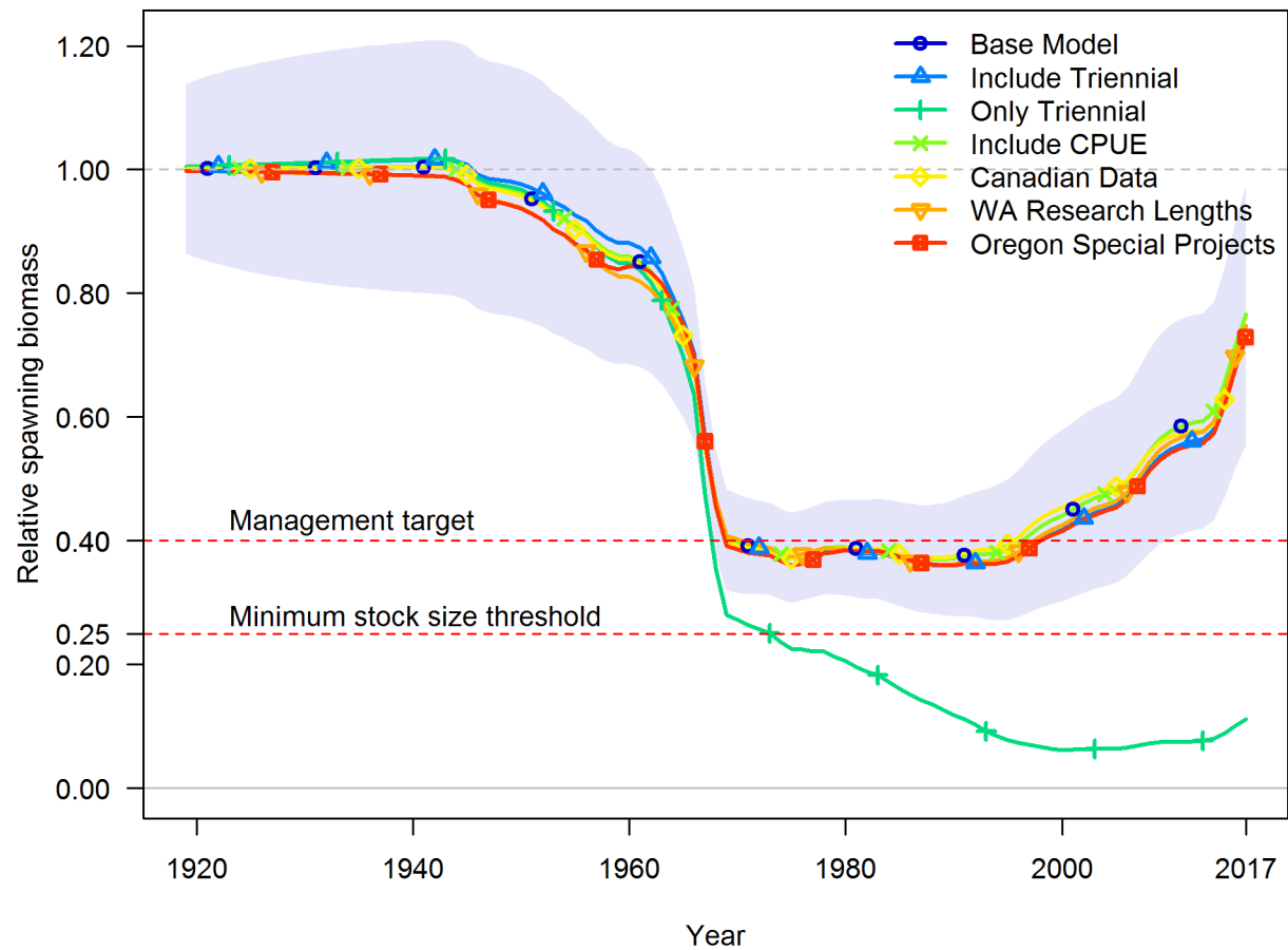
Figure 77: Time-series of relative spawning output (depletion) for model sensitivities for Pacific ocean perch.
