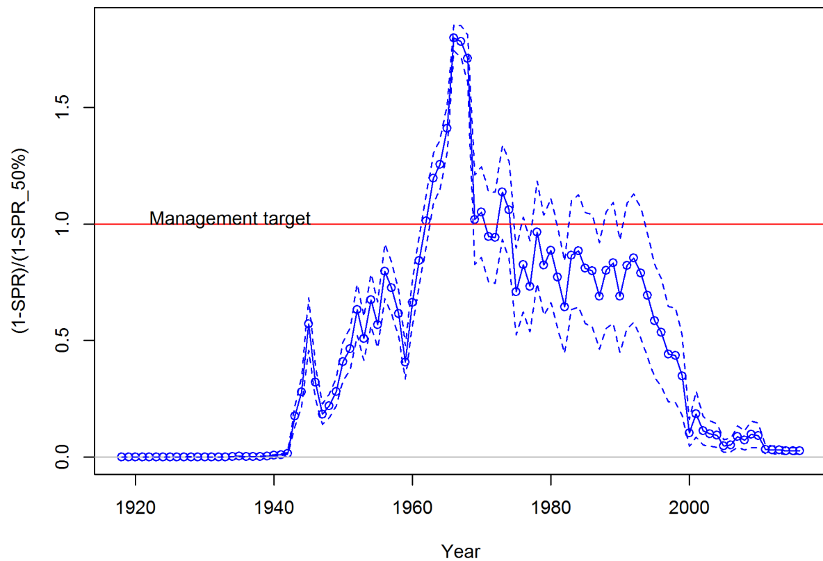
Figure 85: Estimated spawning potential ratio (1-SPR)/(1-SPR_{50\%}) for the base-case model. One minus SPR is plotted so that higher exploitation rates occur on the upper portion of the y-axis. The management target is plotted as a red horizontal line and values above this reflect harvests in excess of the overfishing proxy based on the SPR50% harvest rate. The last year in the time series is 2016.
