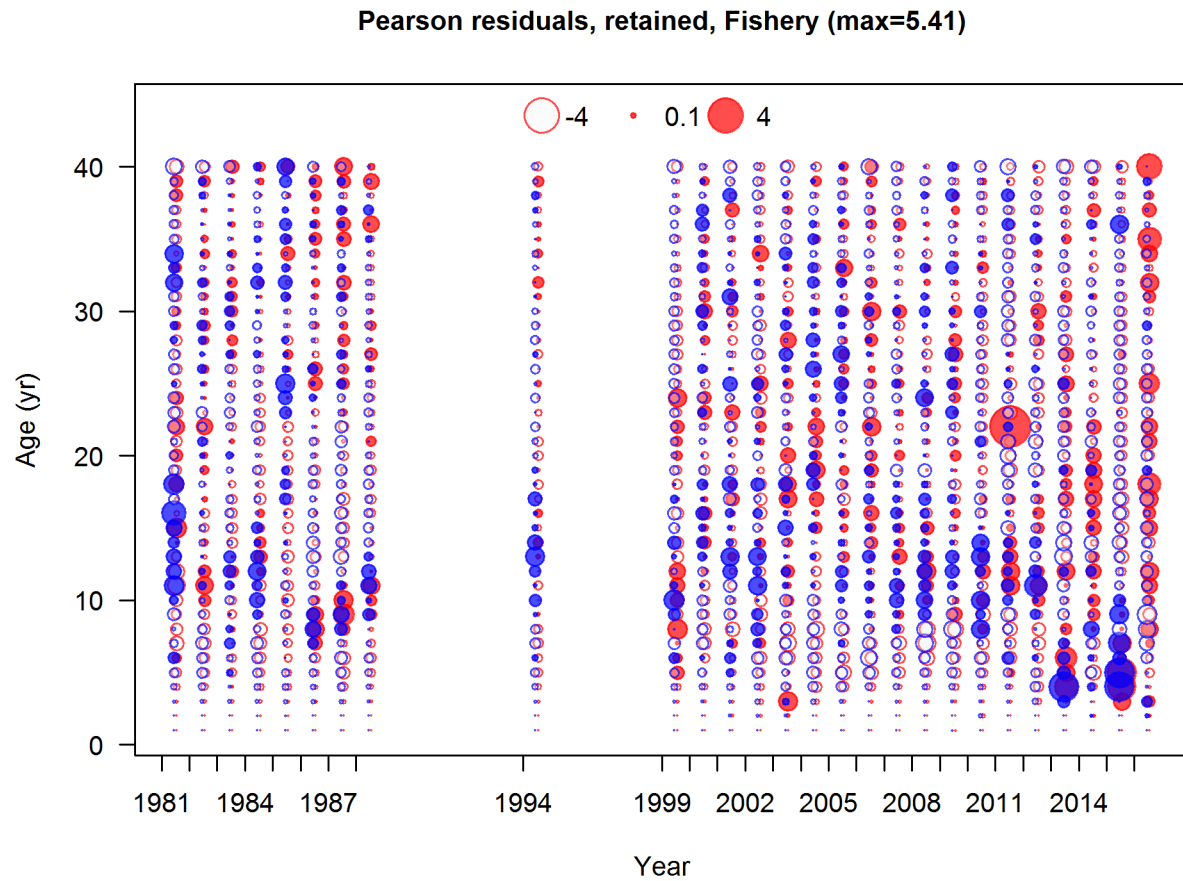
Figure 57: Pearson residuals, retained, Fishery (max=5.41) Closed bubbles are positive residuals (observed > expected) and open bubbles are negative residuals (observed < expected).
