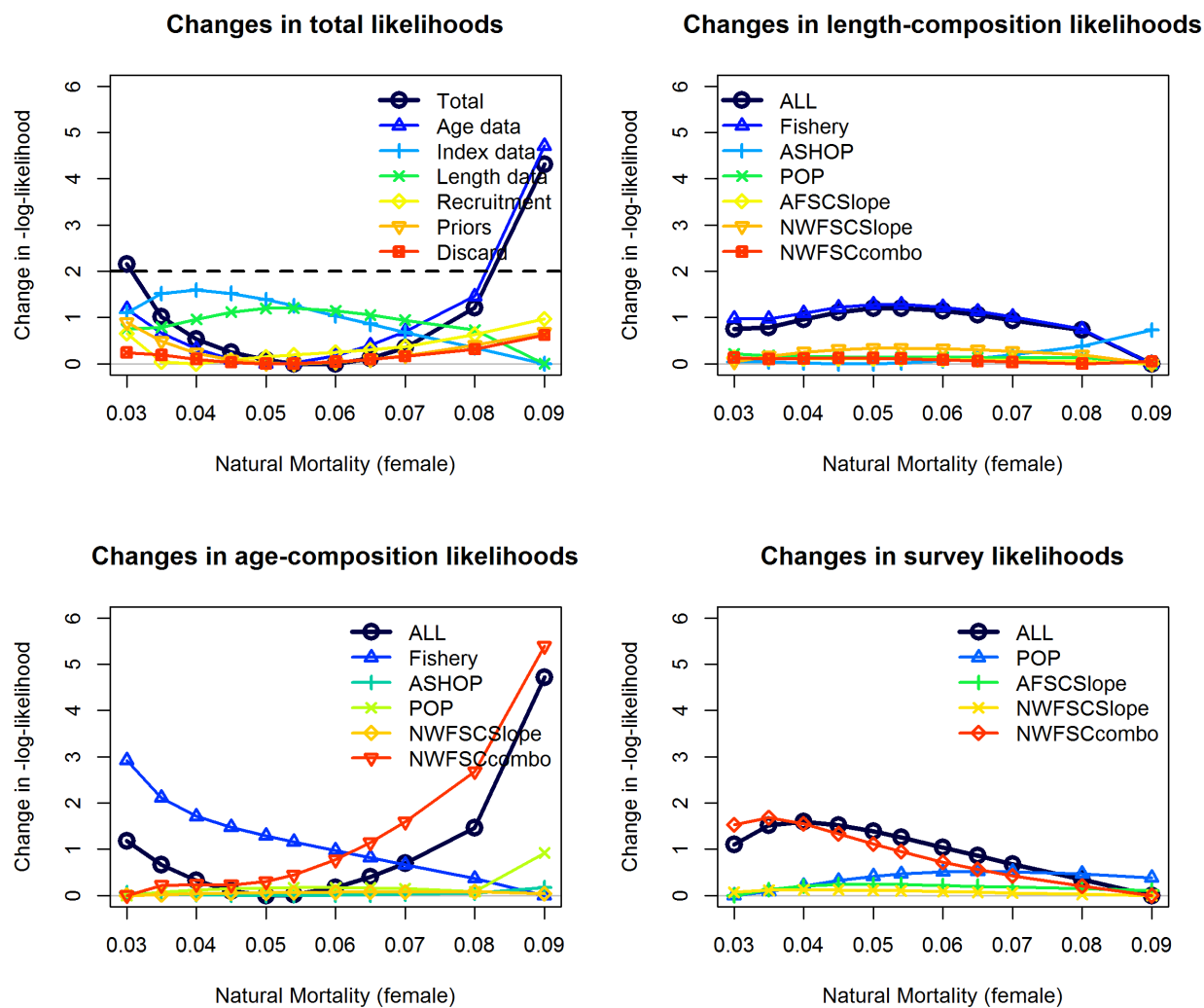
Figure 82: Likelihood profile across natural mortality values.
