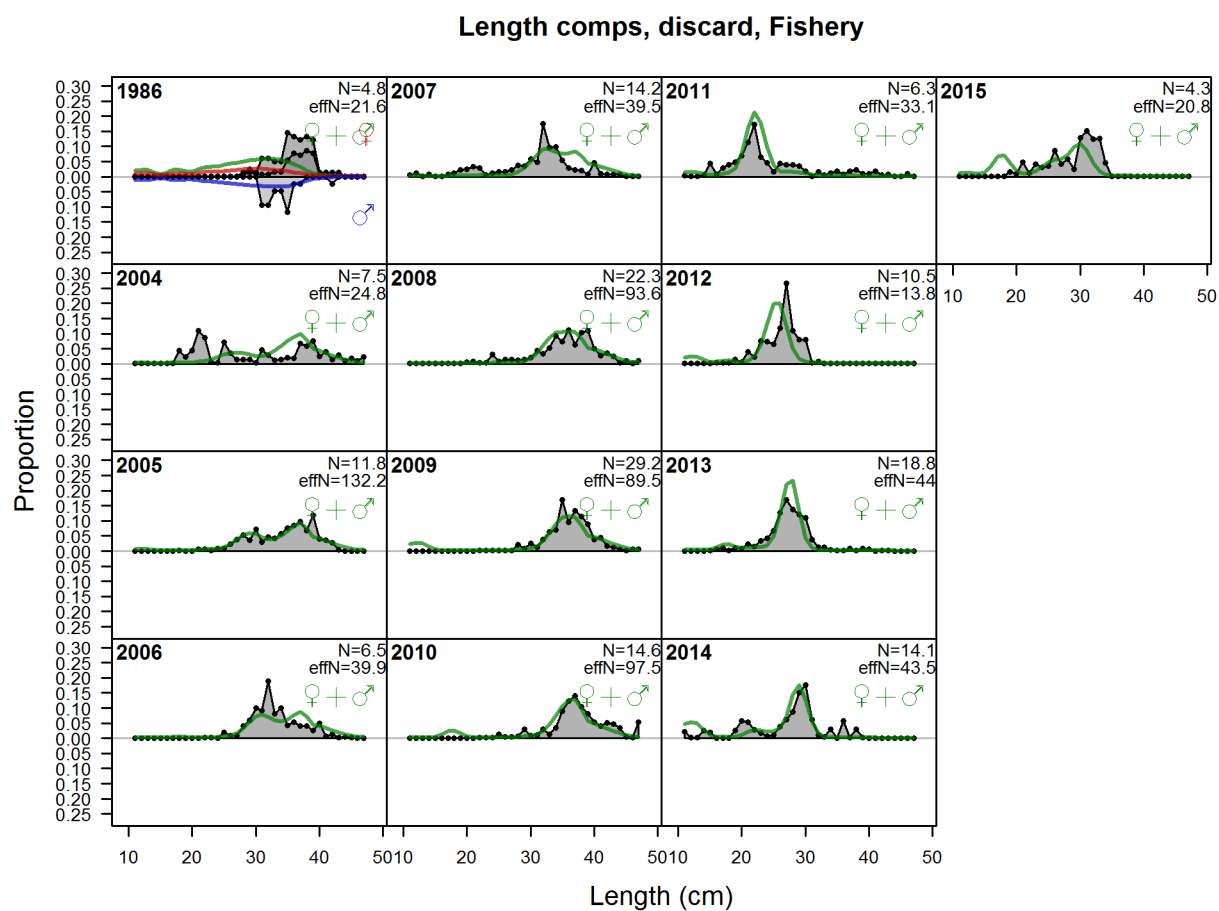
Figure 87: Length comps, discard, Fishery
