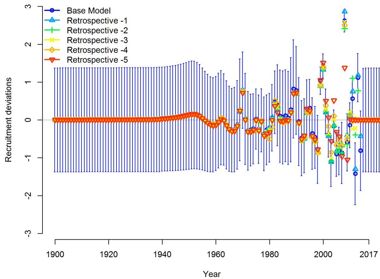
Figure 79: Retrospective pattern for estimated recruitment deviations.
