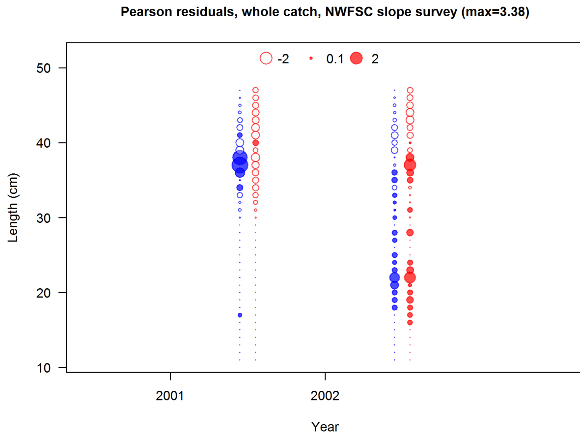
Figure 48: Pearson residuals, whole catch, NWFSC slope survey (max=3.38) Closed bubbles are positive residuals (observed > expected) and open bubbles are negative residuals (observed < expected).
