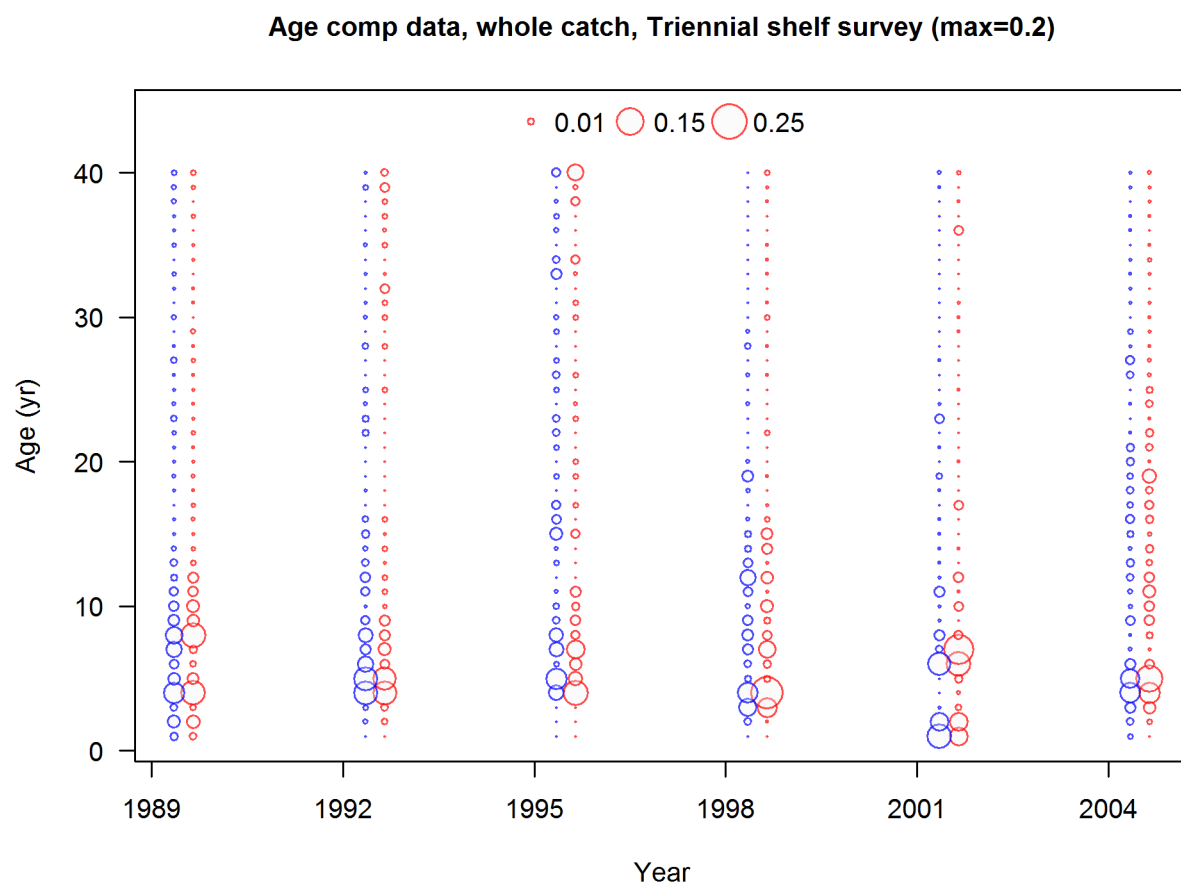
Figure 104: Triennial shelf survey age frequency distributions for Pacific ocean perch.
