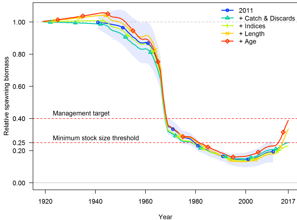
Figure 32: Each of the data sets used in the current assessment was added to the 2011 model without updating model assumptions. Each data source was included in an additive fashion where the final model “+ Age” is the 2011 model with all data sources updated.
