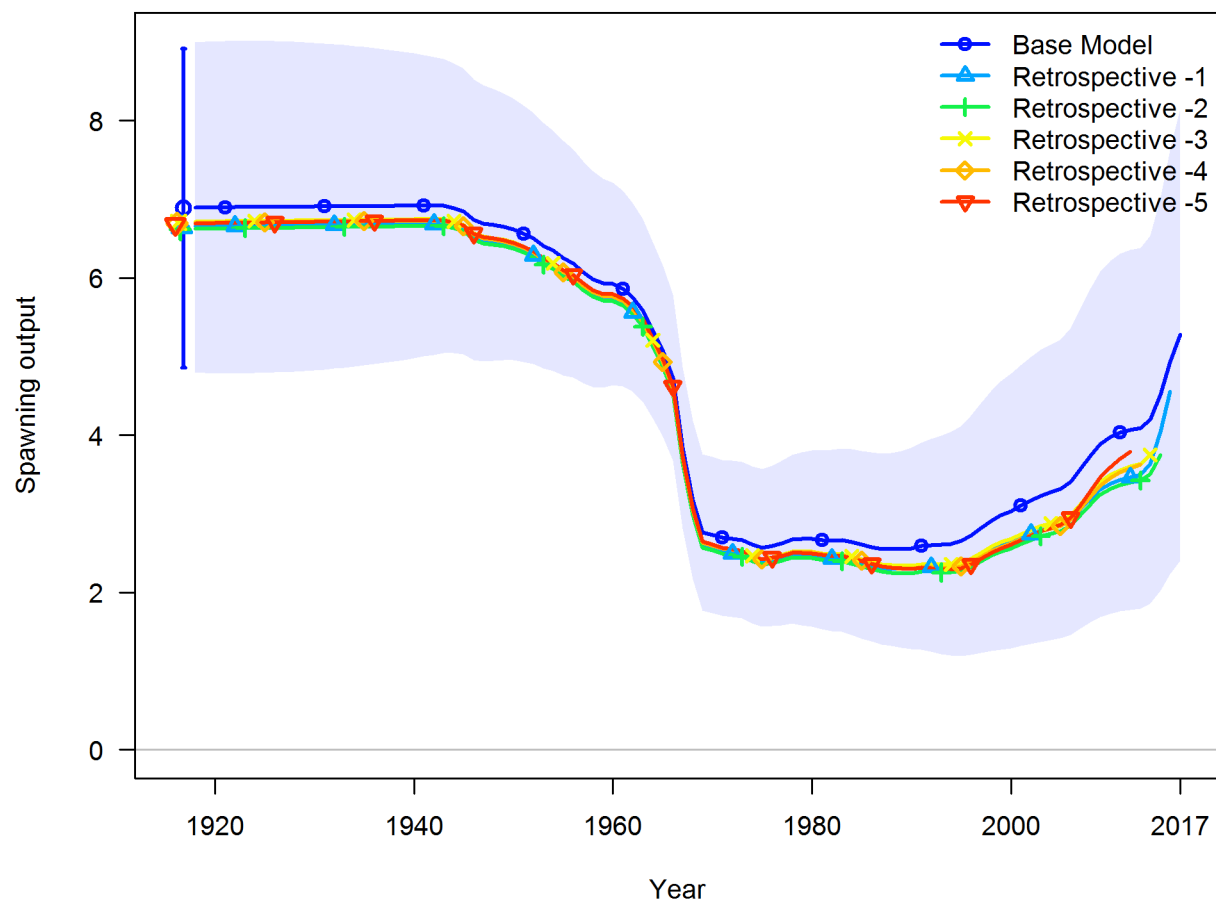
Figure 78: Retrospective pattern for spawning output.
