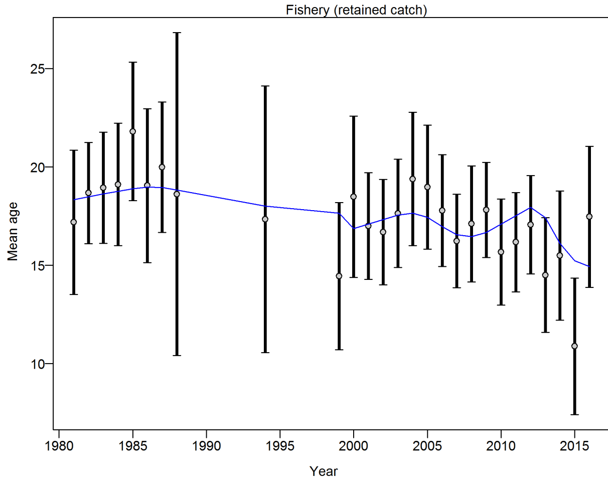
Figure 66: Mean age for Fishery with 95% confidence intervals based on current samples sizes. Francis data weighting method TA1.8: thinner intervals (with capped ends) show result of further adjusting sample sizes based on suggested multiplier (with 95% interval) for age data from Fishery: 0.9999 (0.6705_2.0064) For more info, see Francis, R.I.C.C. (2011). Data weighting in statistical fisheries stock assessment models. Can. J. Fish. Aquat. Sci. 68: 1124_1138.
