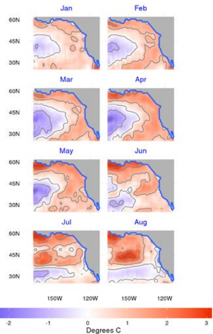
Figure 8. Monthly sea surface temperature anomalies in 2016. NOAA OISST V2 data provided by the NOAA/OAR/ESRL PSD, Boulder, Colorado, USA, from their Web site at http://www.esrl.noaa.gov/psd/ .
