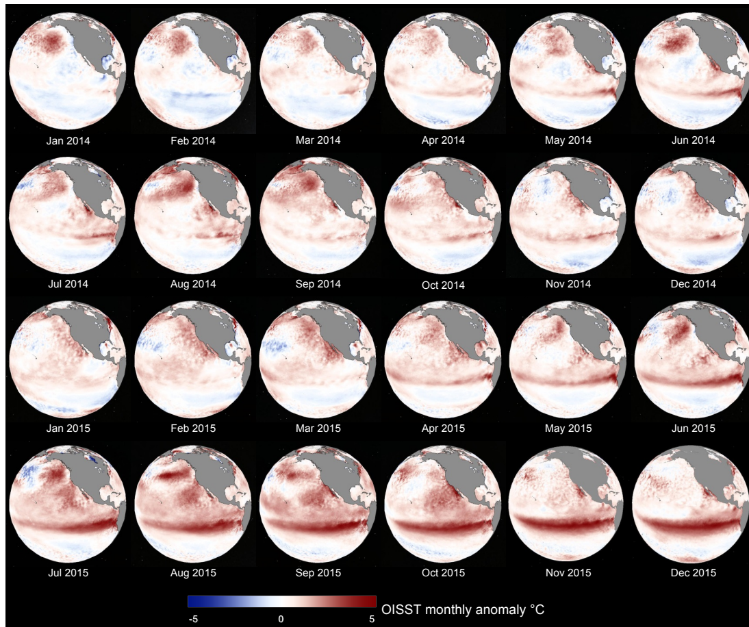
Figure B1. Observed monthly SST anomalies during the 2014-15 northeast Pacific Ocean heat wave from OISST.v2 data using the 1981-2010 climatology. Image produced by P. Fiedler (NOAA/NMFS/SWFSC).
