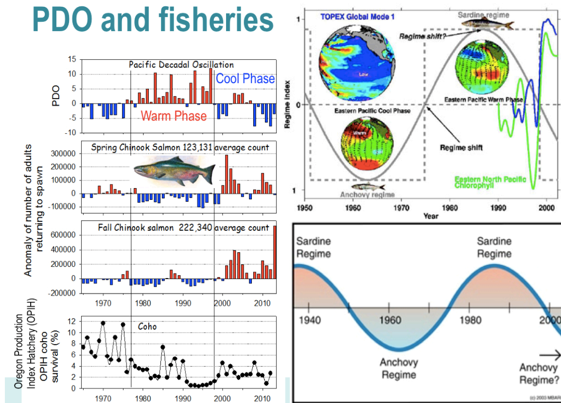
Figure 3. Pacific Decadal Oscillation (PDO) from the 1950s to present and its recent correlation to fluctuations with salmonid and small pelagics in the CCLME.
