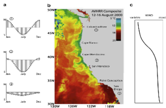
Figure 1. Winds and sea-surface temperature in the California Current System (CCS). (a) Seasonal variation of alongshore winds in three regions of the CCS; (b) sea-surface temperature from August 2000; (c) variability of wind forcing as a function of latitude. From Checkley and Barth (2009).
