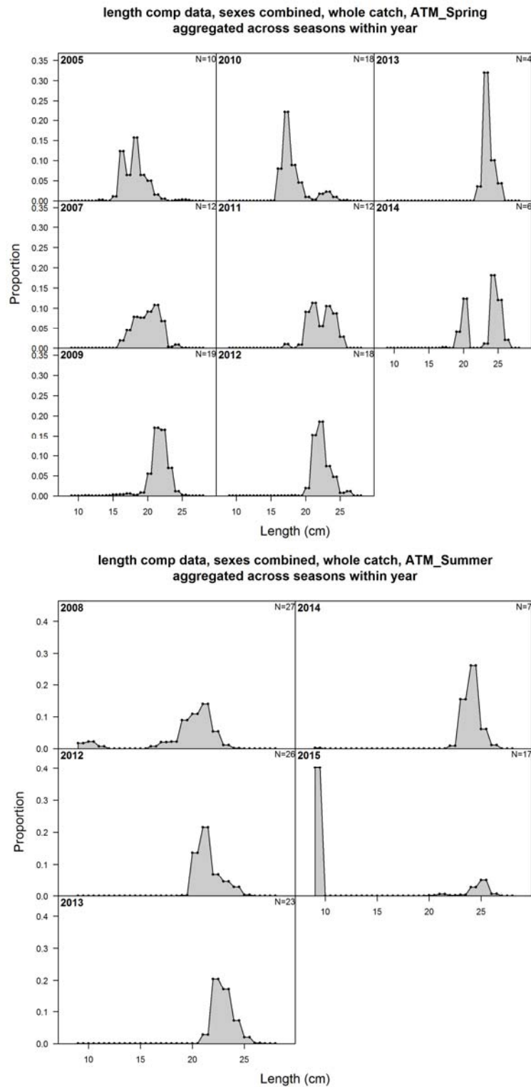
Figure 16. Length-composition data (1-cm resolution) for the ATM Spring (upper panel) and Summer (lower panel) surveys. The summer 2015 length composition was excluded from the proposed update model.
