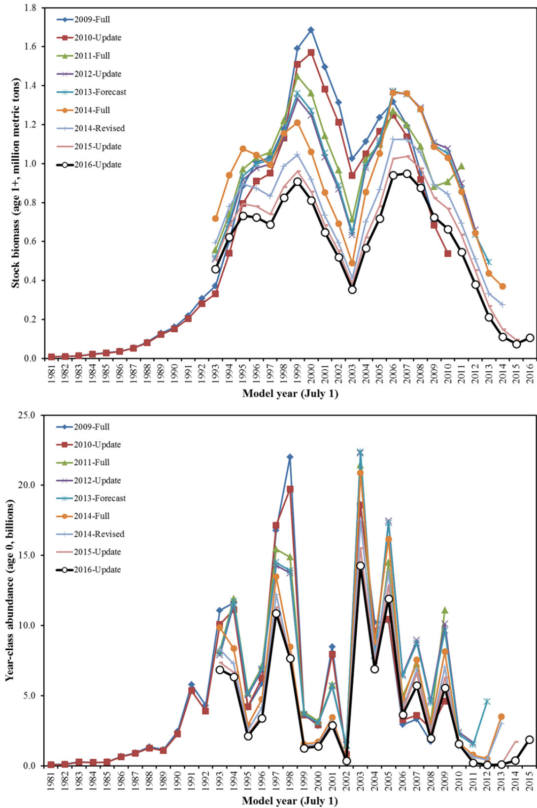
Figure 40. Estimated stock biomass (upper) and recruitment (lower) time series for the proposed update model and past management models.
