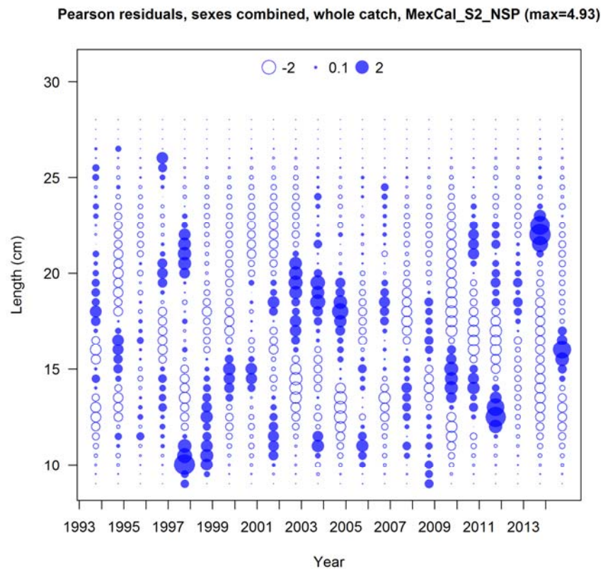
Figure 24a. Proposed update model fit to length compositions and residual plot for the MexCal_S2 fleet.
