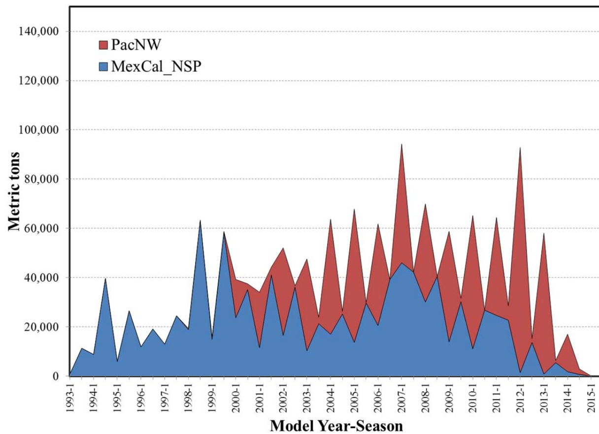
Figure 7. Pacific sardine NSP landings (mt) by fleet, model year and semester as used in all model scenarios.
