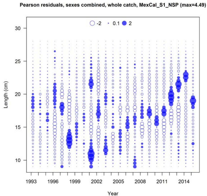
Figure 23a. Proposed update model fit to length compositions and residual plot for the MexCal_S1 fleet.
