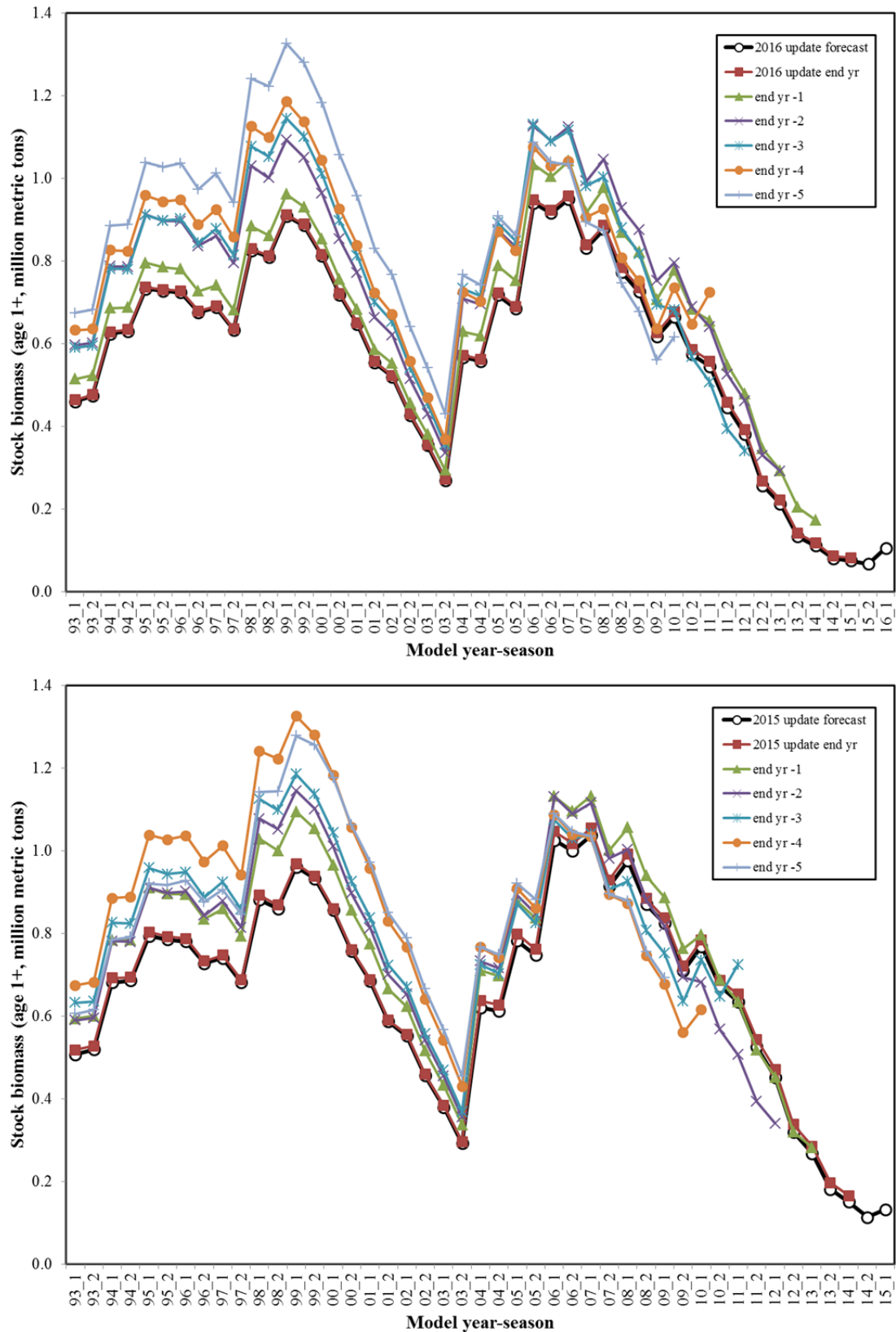
Figure 37. Retrospective analyses of stock biomass (age 1+) for the 2016 proposed update (upper) and 2015 update (lower) models.
