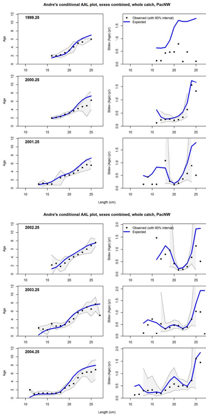
Figure 21. Proposed update model fit to conditional age-at-length compositions for the PacNW fleet.
