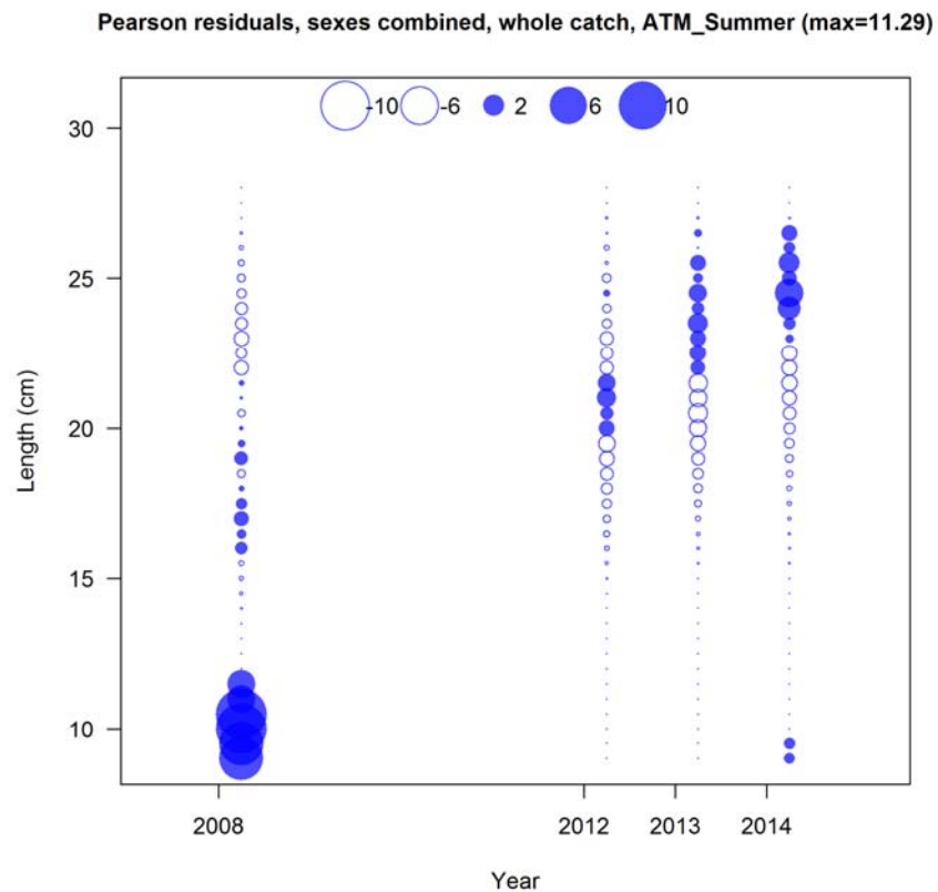
Figure 28. Proposed update model fit to length compositions and residual plot for the Summer ATM survey.
