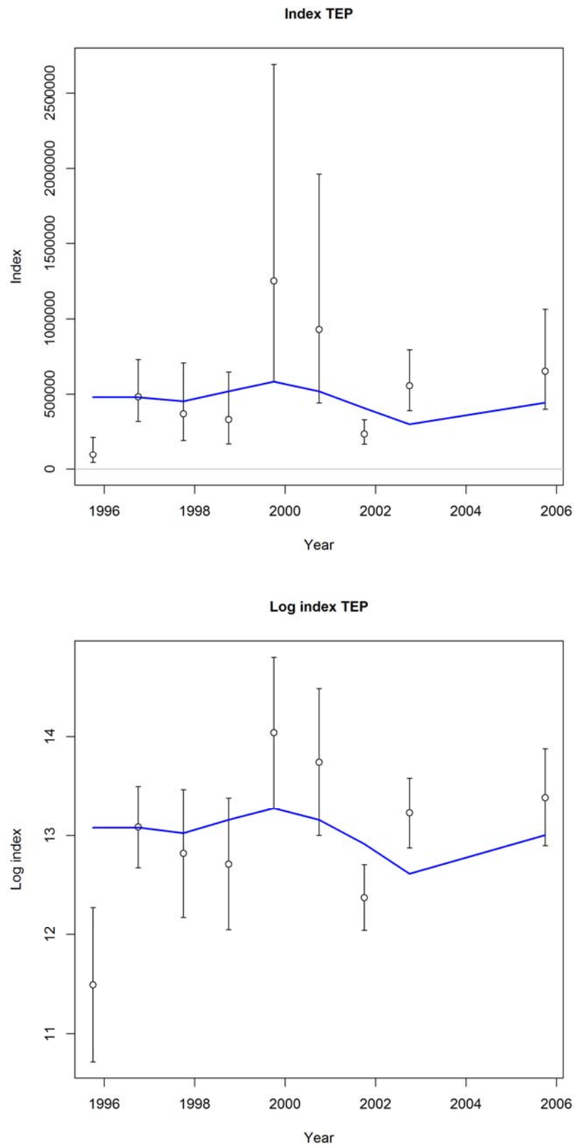
Figure 32. Proposed update model fit to the TEP survey abundance index of total spawning biomass in arithmetic (upper) and log (lower) scales. q=0.760 .
