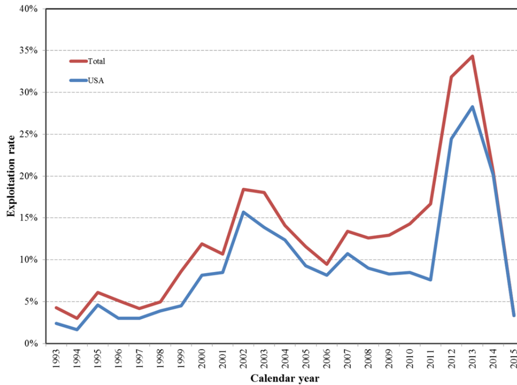
Figure 35b. Annual exploitation rate (CY landings / July total biomass) for the proposed update model.
