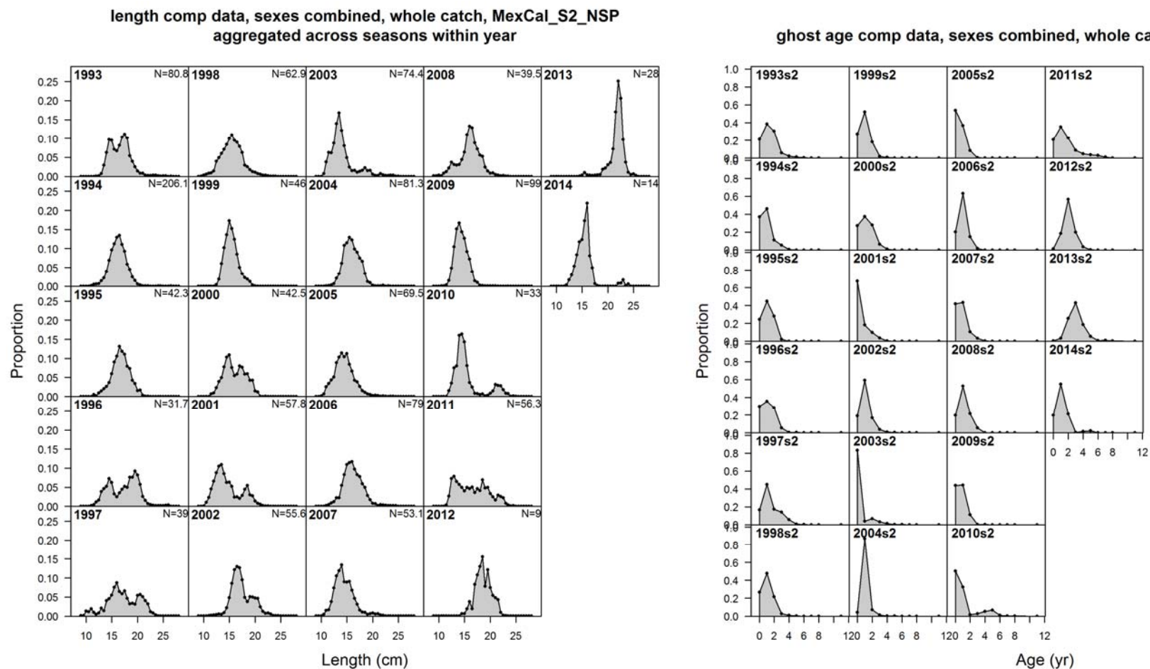
Figure 9. Length-composition (left panel) and implied age composition (right panel) data for the MexCal_S2 fleet.
