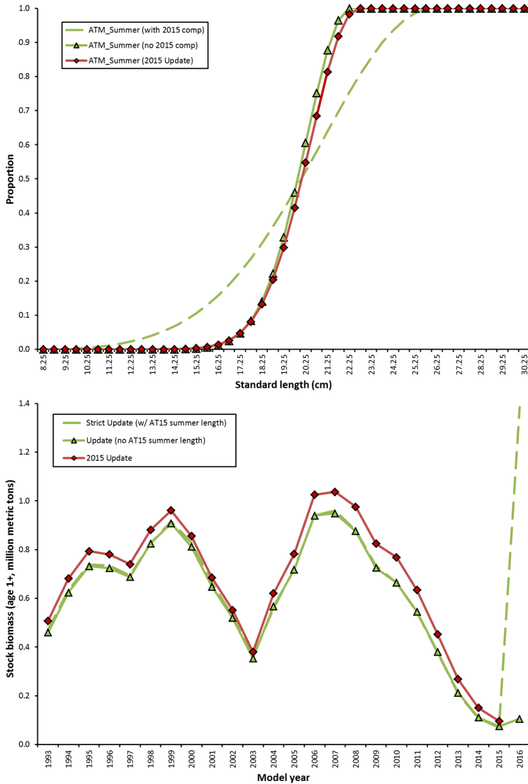
Figure 39. ATM summer survey selectivities (upper panel) for the final 2015 model, strict update (w/ AT summer 2015 length), and proposed update model. Stock biomass series for these models are displayed in the lower panel.
