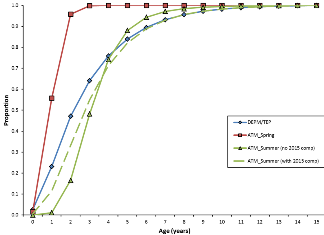
Figure 26b. Implied age-selectivity patterns for surveys in the update models.
