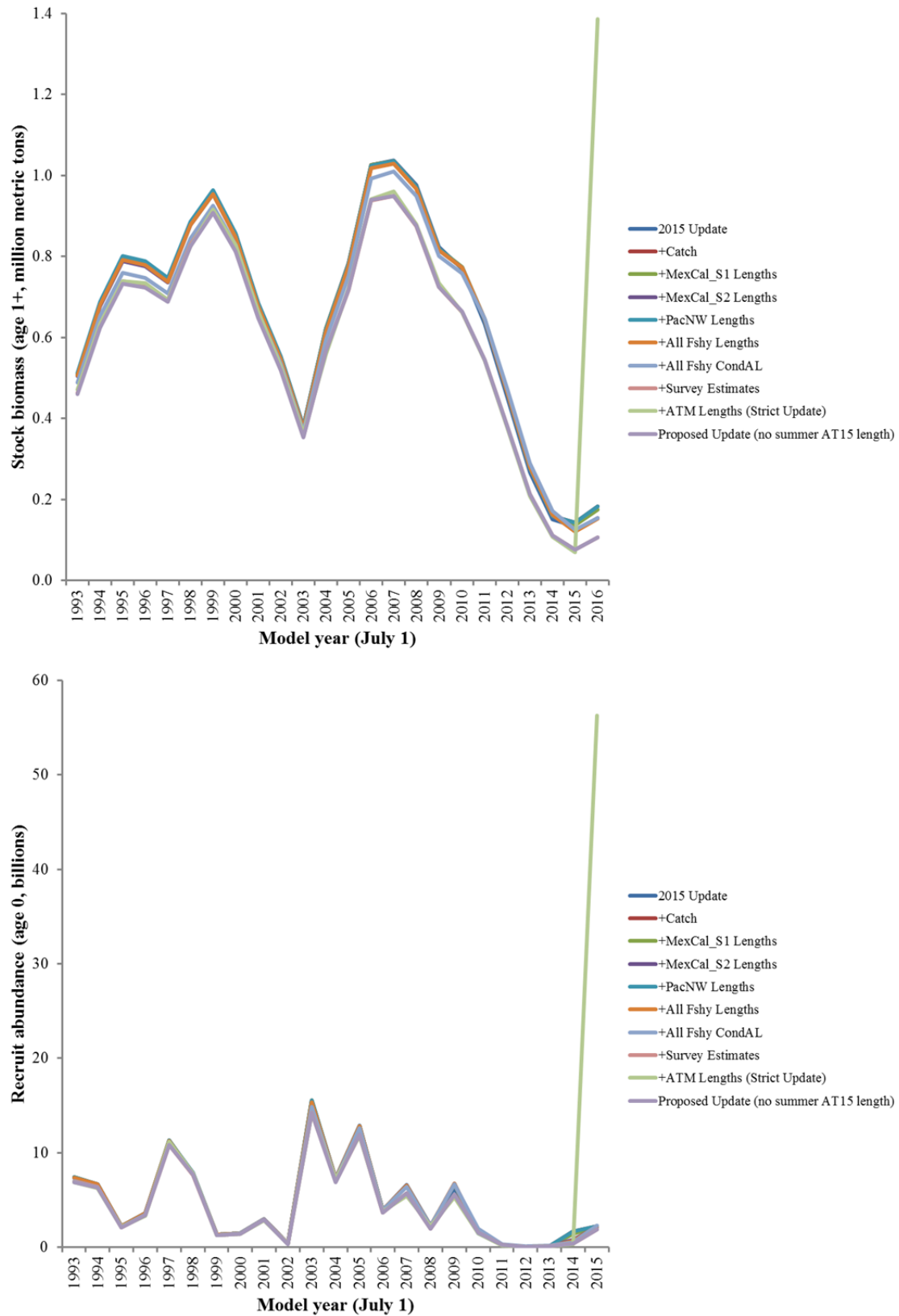
Figure 38. Biomass and recruitment trajectories for the 2015 update model with the sequential addition of new data for 2016 (see Table 9).
