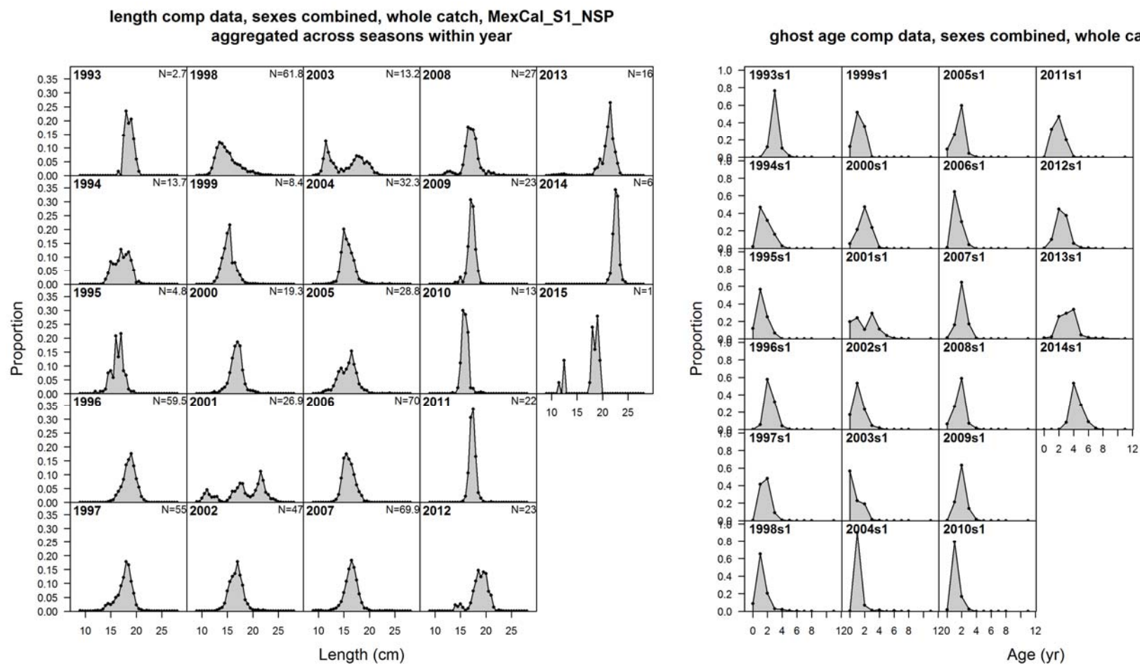
Figure 8. Length-composition (left panel) and implied age composition (right panel) data for the MexCal_S1 fleet.
