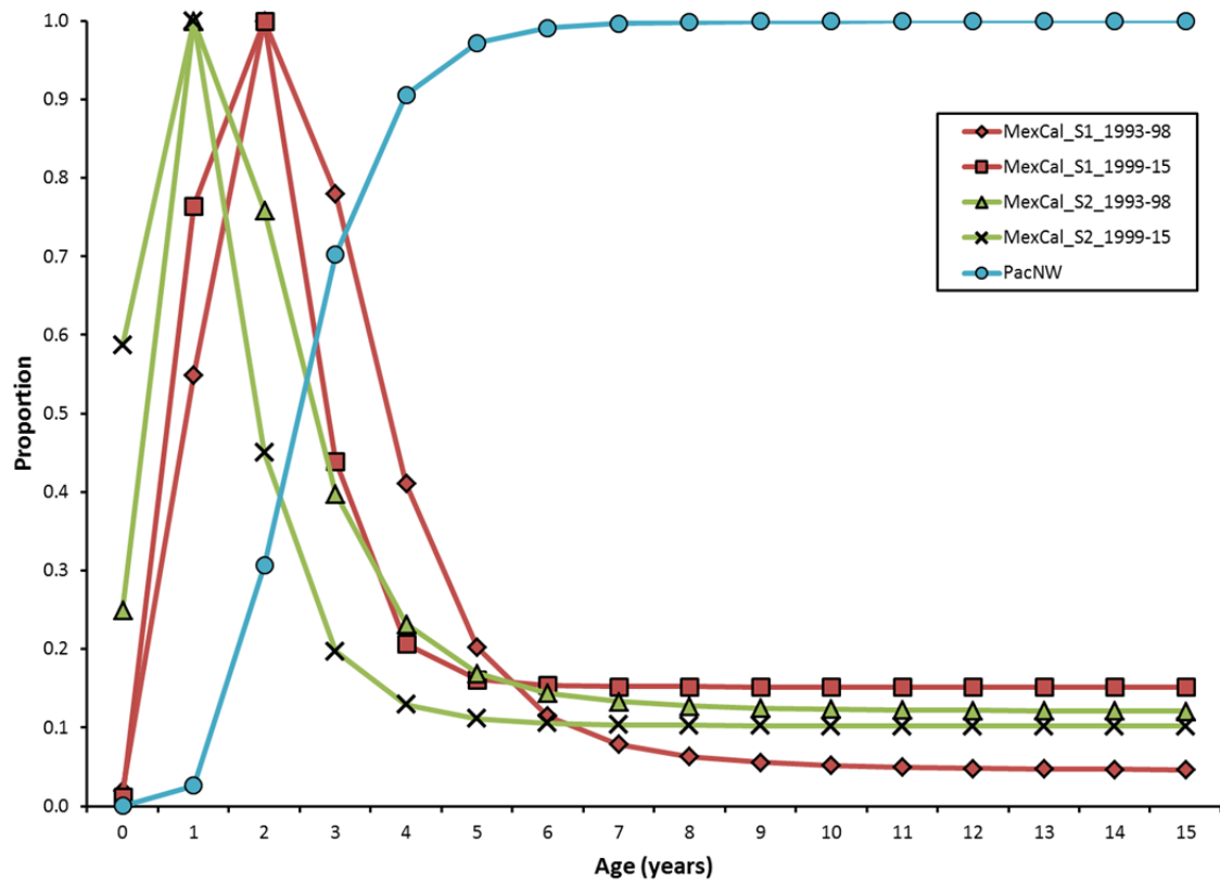
Figure 22b. Implied age-selectivity patterns for fleets in the proposed update model.
