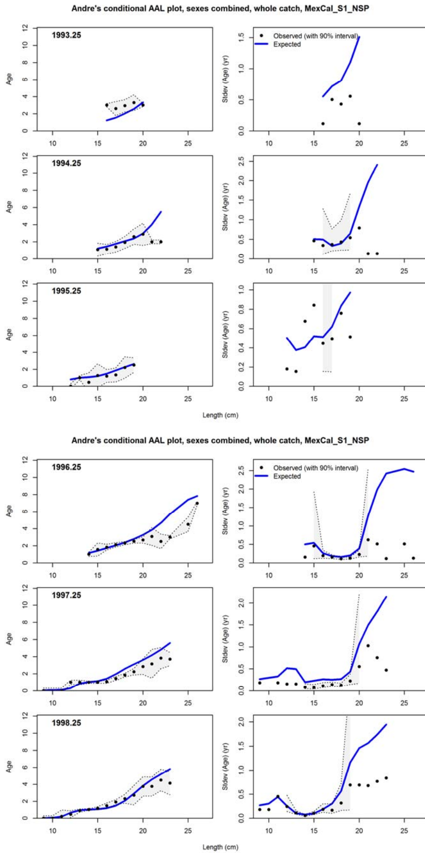
Figure 19. Proposed update model fit to conditional age-at-length compositions for the MexCal_S1 fleet.
