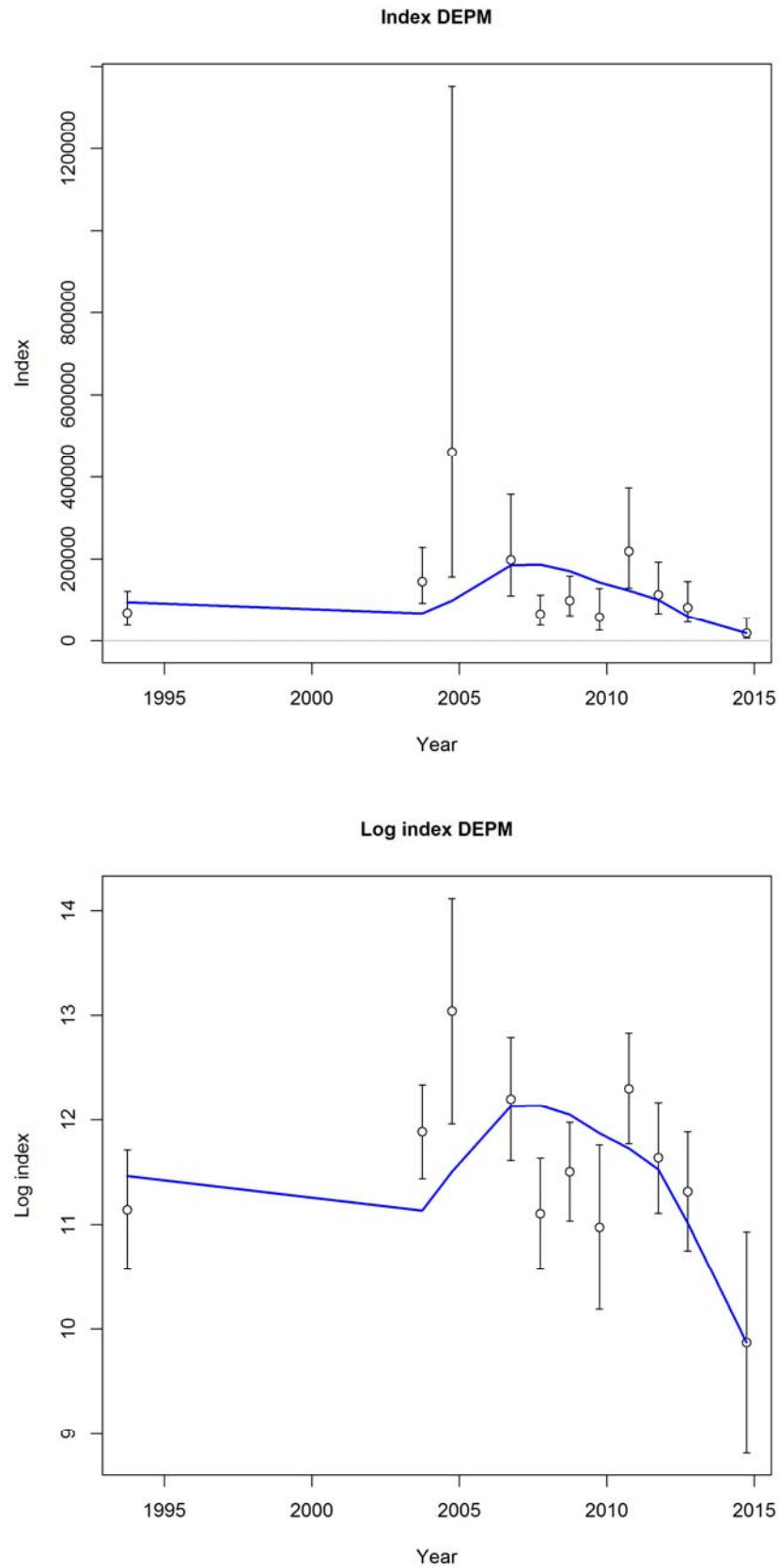
Figure 31. Proposed update model fit to the DEPM survey abundance index of female spawning biomass in arithmetic (upper) and log (lower) scales. q=0.244 .
