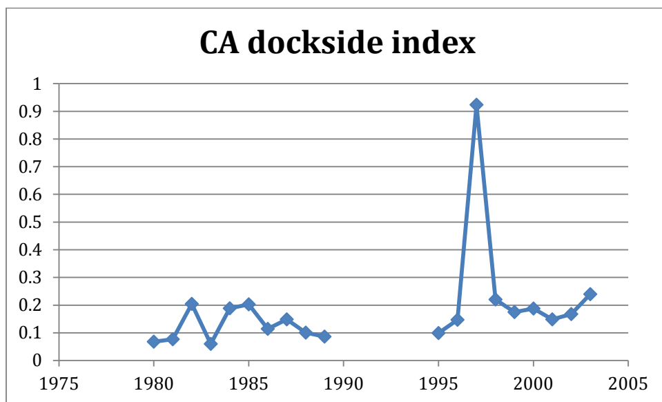
Figure 24. Resulting California dockside index from the delta-GLM model.
