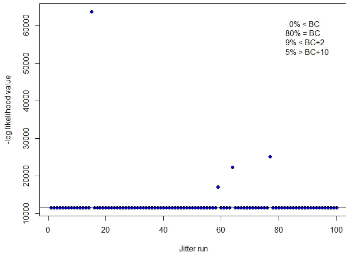
Figure 192. Results from 100 Washington model base case runs when starting values are jittered (0.1). Horizontal line indicates base model value.
