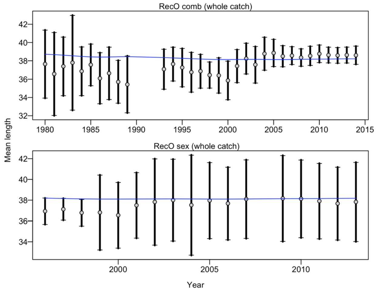
Figure 126. Francis weighting fits to the mean lengths by year for the Oregon Ocean boat recreational fleet.
