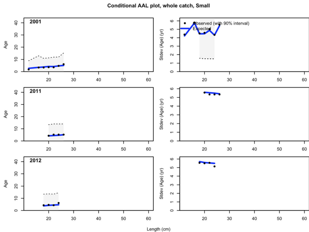
Figure 143. Age composition samples and predictions for the Oregon Small-fish survey, 2 of 2.
