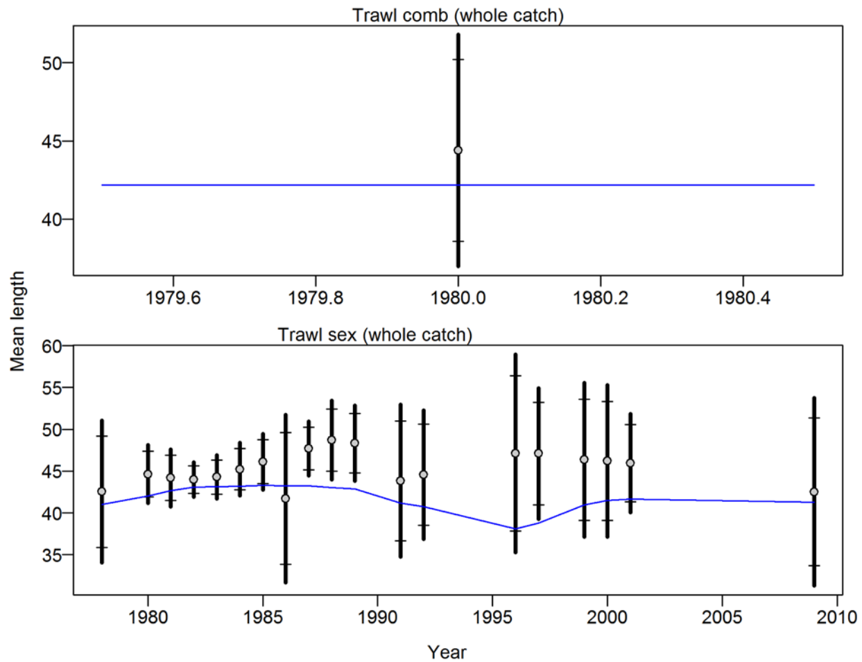
Figure 44. Francis weighting fits to the mean lengths by year for the California commercial trawl fleet. Vertical lines indicate 95% confidence intervals.
