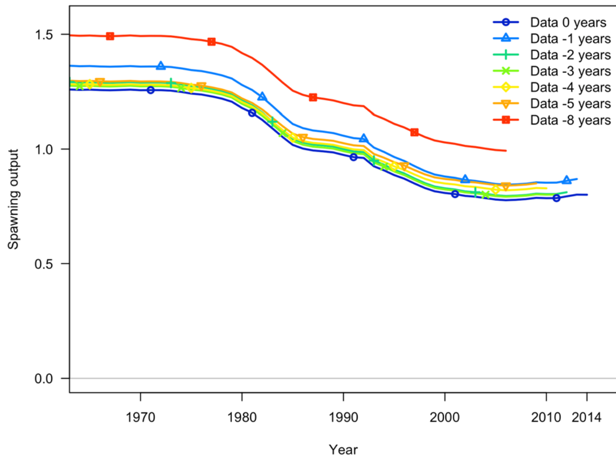
Figure 167. Retrospective model runs from the base case model of Oregon (“Data 0 years”) for stock spawning output.
