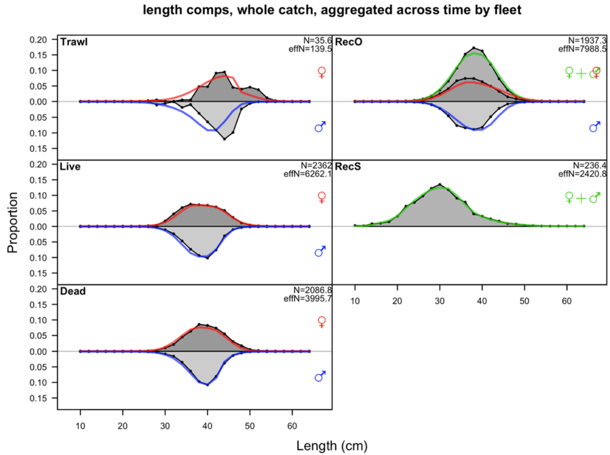
Figure 122. Composite fits to the length composition by fleet and sex for the Oregon base model.
