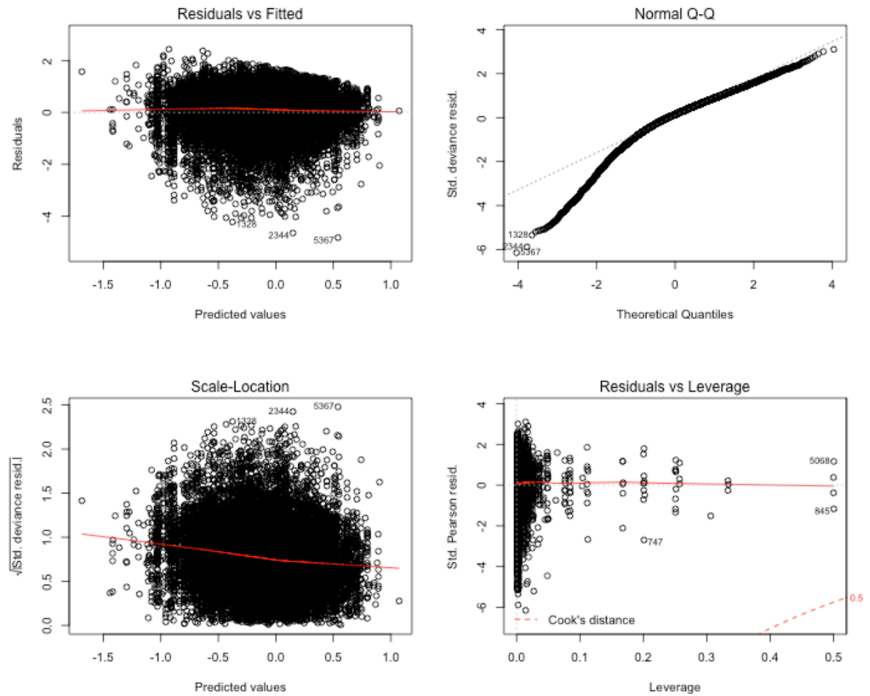
Figure 94. Diagnostic plots for the black rockfish positive catch component lognormal delta-GLM model for the ORBS dockside dataset. These are used to evaluate model fit (top left), assumptions of normality (top right), assumptions of constant variance (bottom left), and the presence of outliers (bottom right).
