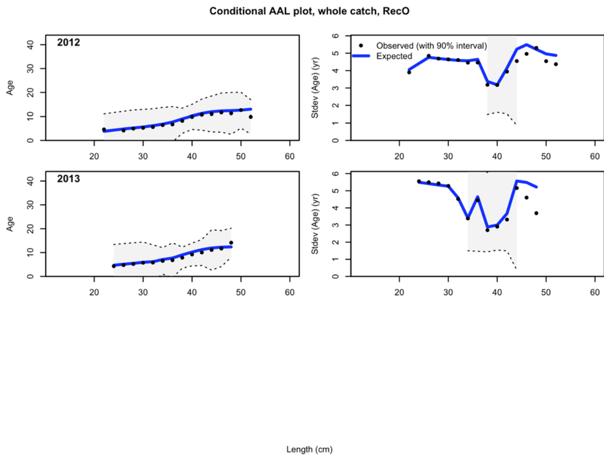
Figure 141. Age composition samples and predictions for the Oregon Ocean boat recreational fishery, 6 of 6.
