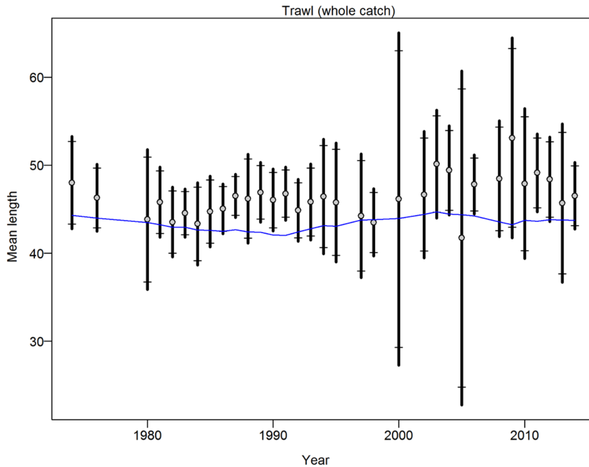
Figure 204. Francis weighting fits to the mean lengths by year for the Washington trawl commercial fleet. Vertical lines are 95% confidence intervals.
