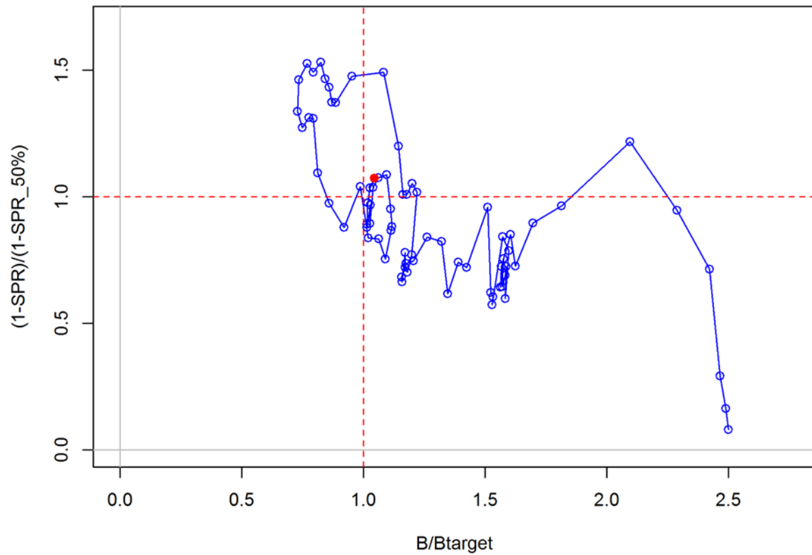
Figure 235. Phase plot of relative spawning output vs fishing intensity for the Washington base case model. The relative fishing intensity is (1-SPR) divided by 50% (the SPR target). The vertical red line is the relative spawning output target defined as the annual spawning output divided by the spawning output corresponding to 40% of the unfished spawning output.
