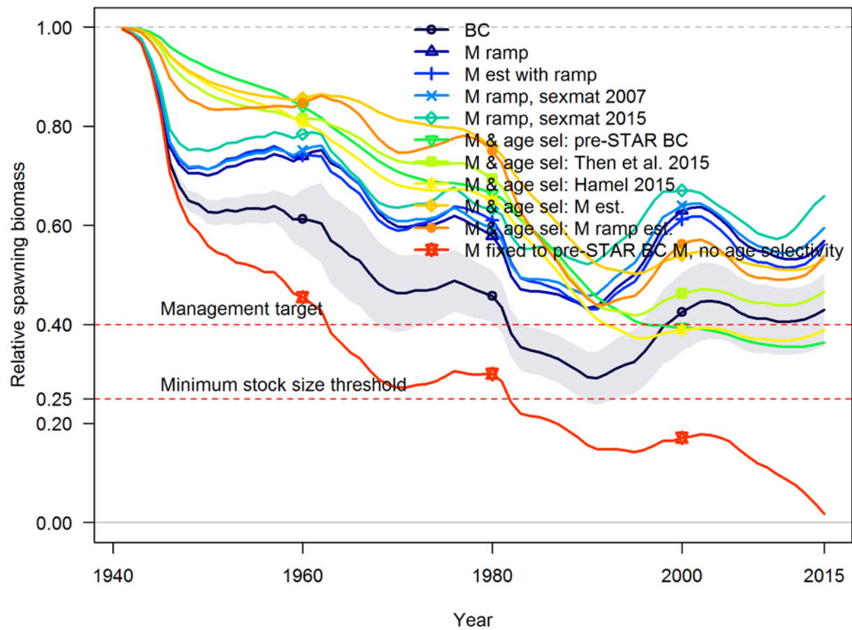
Figure 223. Comparison of relative stock output for sensitivity runs that alter natural mortality specification in the Washington model. Shading indicates 95% confidence intervals. BC = base case model.
