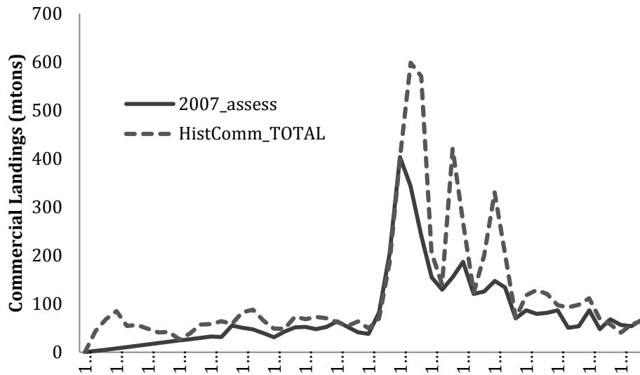
Figure 14: Comparing the California historical commercial landings reconstruction to the 2007 assessment estimates.
