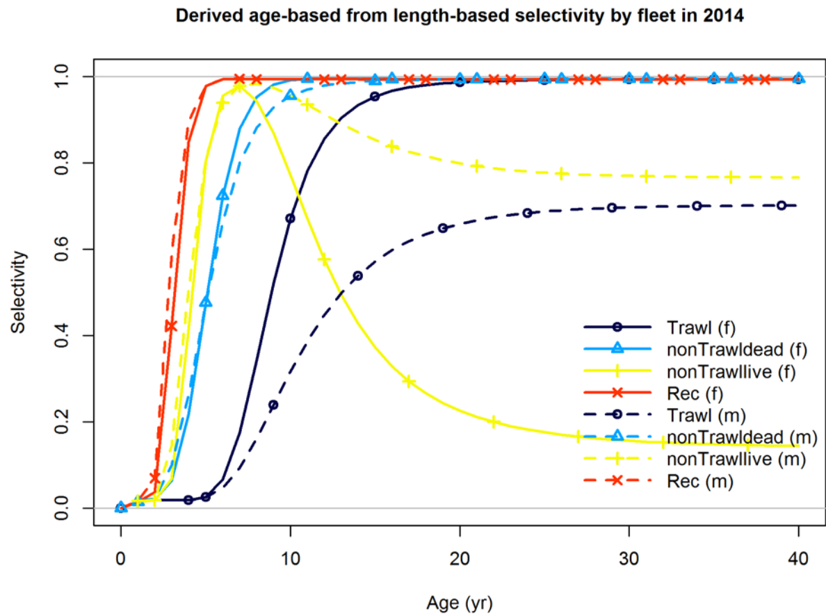
Figure 60. California base case estimated realized selectivity curves for each gear by sex.
