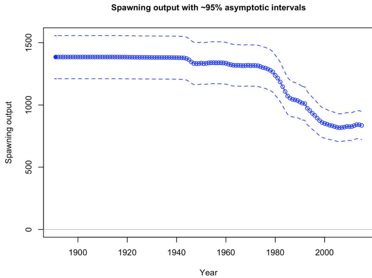
Figure 154. Oregon base case estimate of spawning biomass with 95% confidence intervals.
