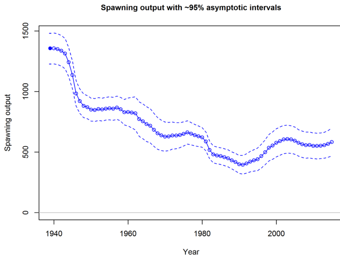
Figure 218. Washington base model estimate of spawning output with 95% confidence intervals.
