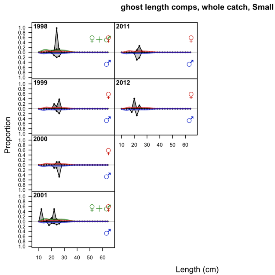
Figure 121. Fits to the Oregon “small” fish length compositions by sex and year.
