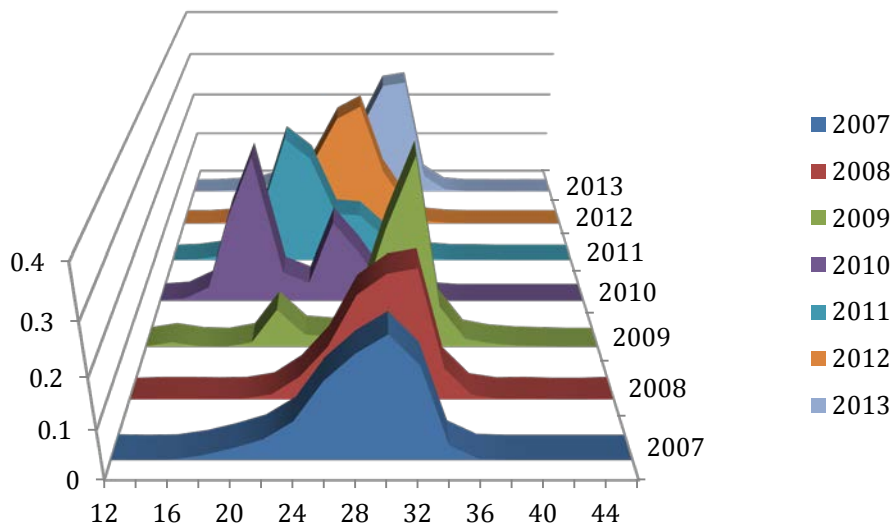
Figure 20: Length compositions from the CCFRP (California), 2007-2013.
