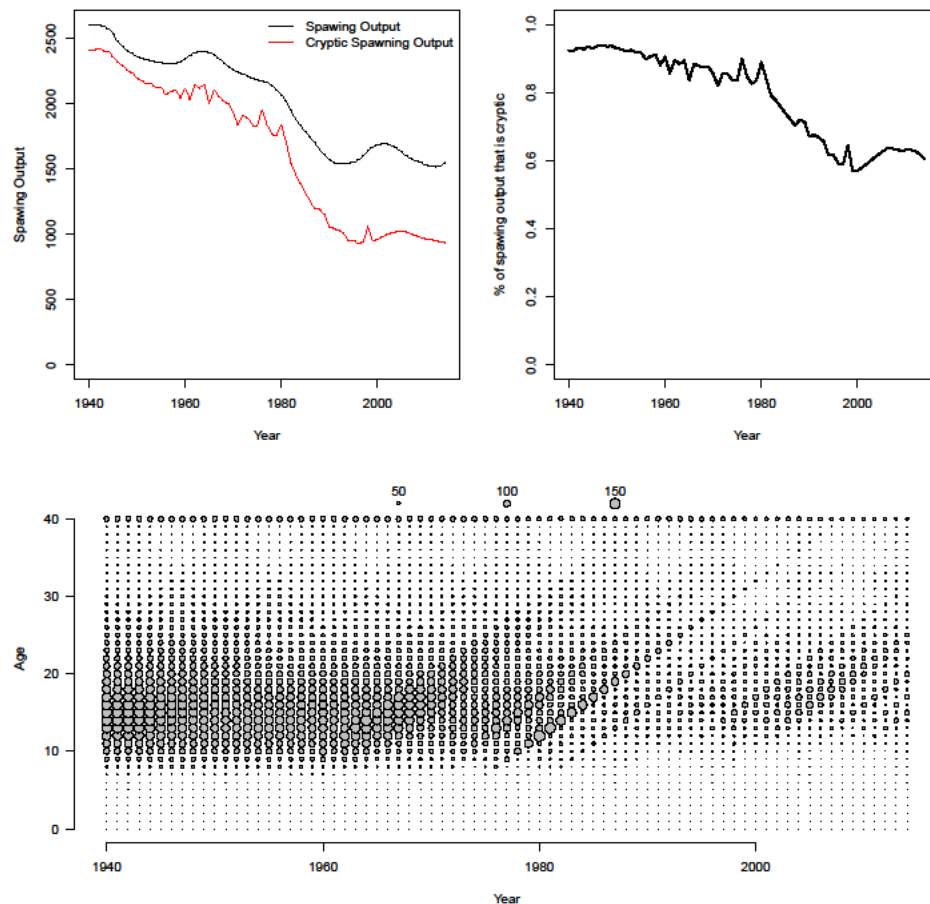
Figure 7. The measure of cryptic spawning biomass output compared to spawning output (top left panel), relative cryptic spawning output (top right panel) and the resultant age structure for the Washington black rockfish model that assumes low fixed M and dome-shaped age based selectivity.
