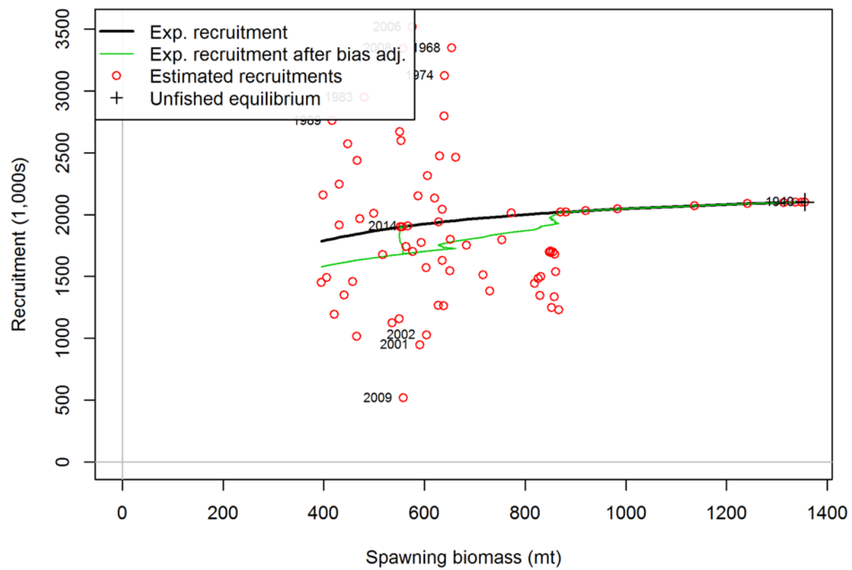
Figure 221. Stock-recruitment relationship from the Washington base case model.
