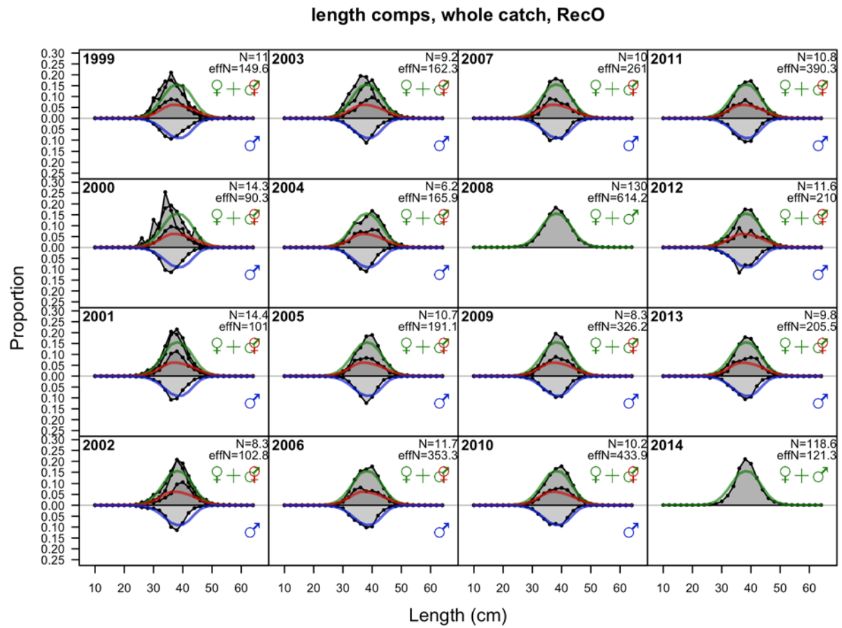
Figure 118. Fits to the Oregon Ocean boat recreational length compositions by sex and year, 2 of 2.
