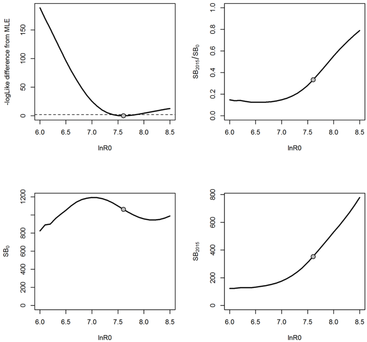
Figure 72. Likelihood profile in the California model for initial equilibrium recruitment ( \ln R_0 ) and resultant derived quantities (initial spawning output ( SB_0 ); spawning output in 2015 ( SB_{2015} ) and stock status ( SB_{2015}/SB_0 )).
