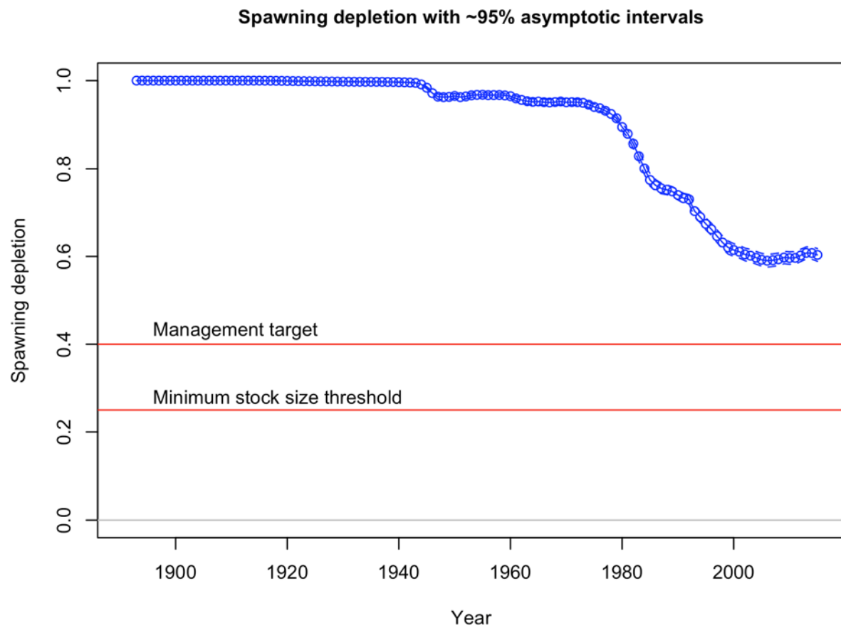
Figure 155. Oregon base case estimate of stock status (i.e., spawning depletion) with 95% confidence intervals.
