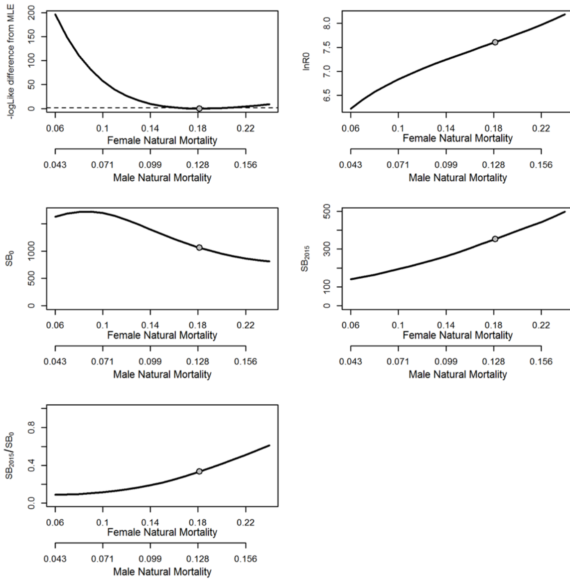
Figure 70. Likelihood profile in the California model for female and male natural mortality and resultant estimated ( \ln R_0 ) and derived quantities (initial spawning output ( SB_0 ); spawning output in 2015 ( SB_{2015} ) and stock status ( SB_{2015}/SB_0 )).
