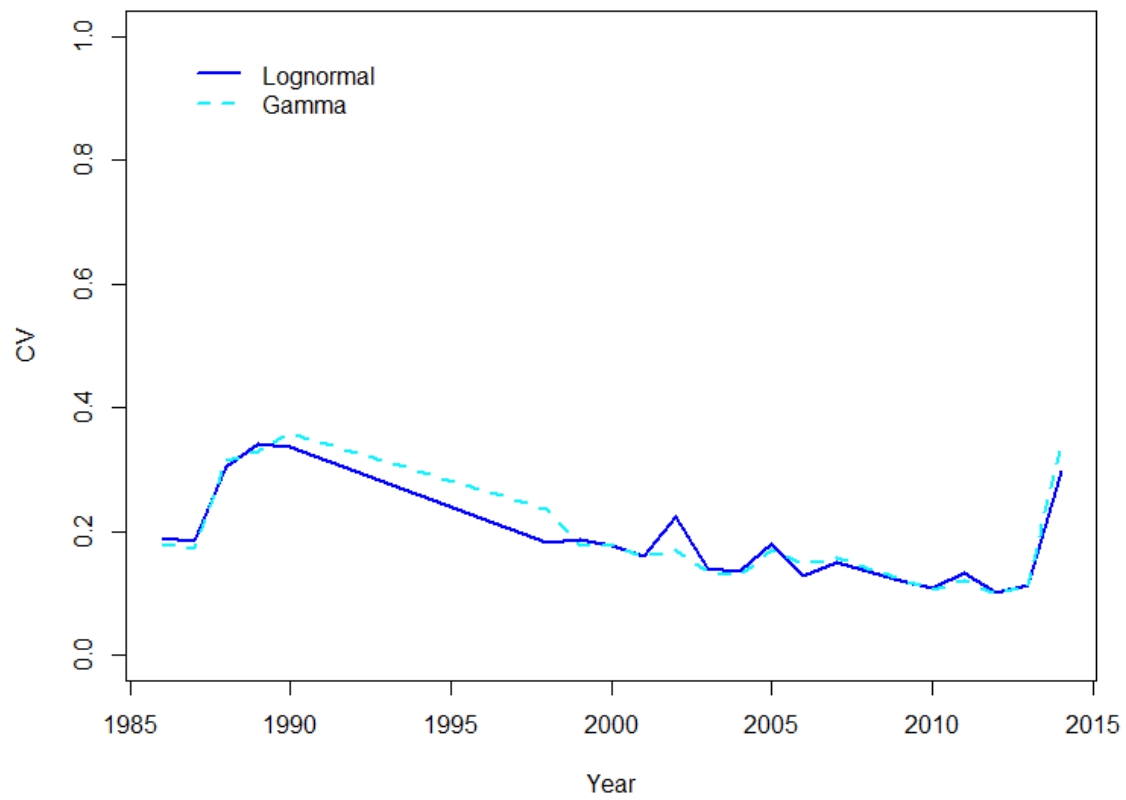
Figure 188. Jackknifed estimates of variation for each model of the Washington tagging CPUE index.
