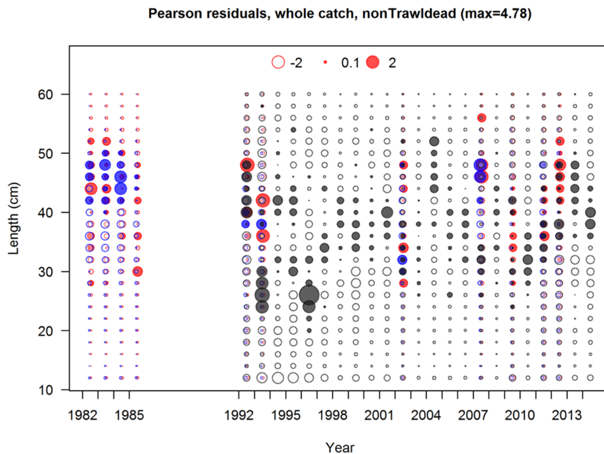
Figure 32. Pearson residuals plots for male (blue) and female (red) length compositions for the California non-trawl (dead) commercial fleet. Residuals < 2 are generally considered non-significant.
