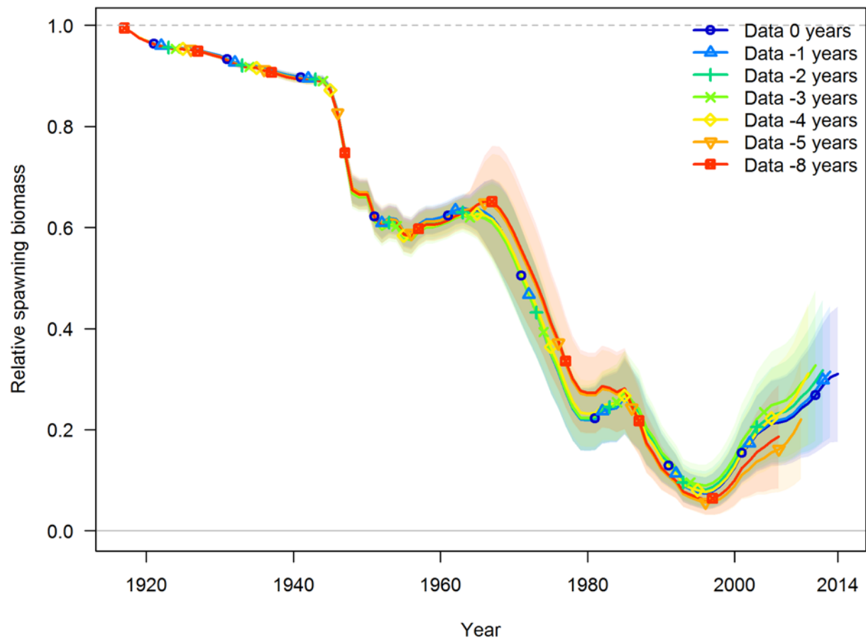
Figure 77. Retrospective model runs from the base case model of California (“Data 0 years”) for relative stock output (stock status). Shading indicates 95% confidence intervals.
