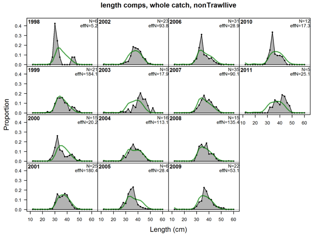
Figure 39. Fits to the California non-trawl commercial live fish fishery length compositions and year.
