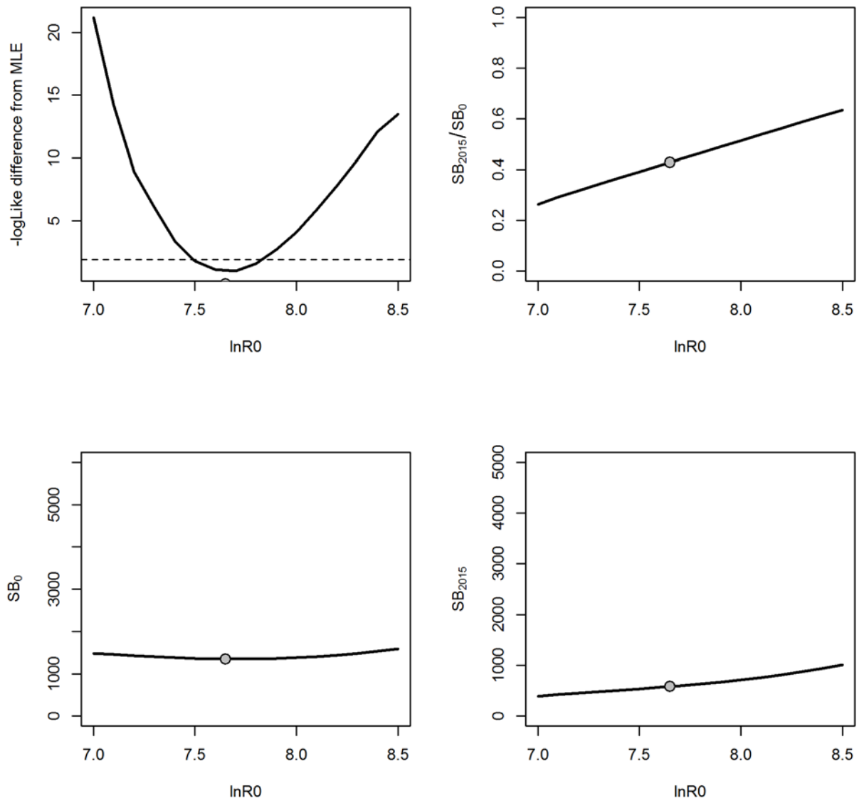
Figure 228. Likelihood profile in the Washington model for initial equilibrium recruitment ( \ln R_0 ) and resultant derived quantities (initial spawning output ( SB_0 ); spawning output in 2015 ( SB_{2015} ) and stock status ( SB_{2015}/SB_0 )).
