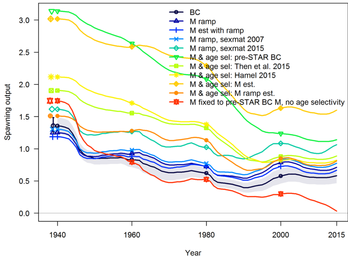
Figure 222. Comparison of stock output for sensitivity runs that alter natural mortality specification in the Washington model. Shading indicates 95% confidence intervals. BC = base case model.
