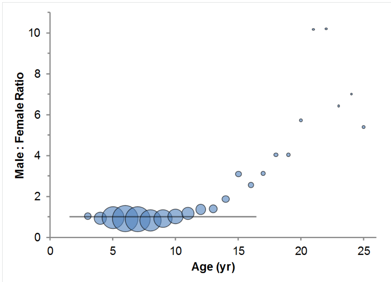
Figure 101. Male to female sex ratio based on all available conditional age-at-length observations in the Oregon black rockfish Synthesis model. The areas of the bubble are proportional to the number of fish in each age-class. The compositional data were not adjusted to reflect differences in sampling rates.
