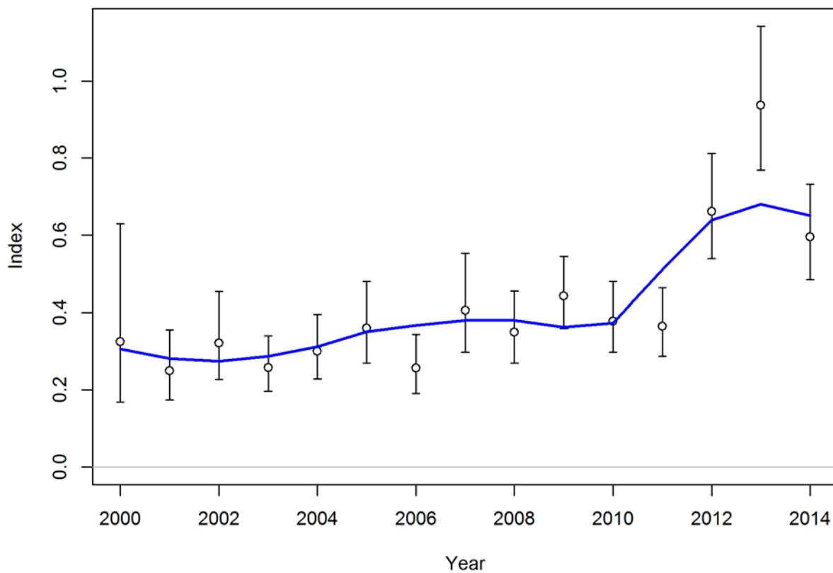
Figure 29. Base case fit to the California recreational CPFV onboard index (2000-2014). Vertical lines indicate 95% confidence intervals.
