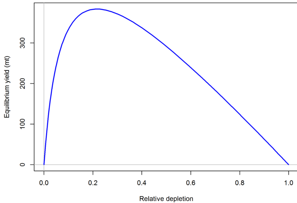
Figure 236. Equilibrium yield curve for the Washington base case model. Values are based on 2014 fishery selectivity and distribution with steepness fixed at 0.773. The depletion is relative to unfished spawning biomass.
