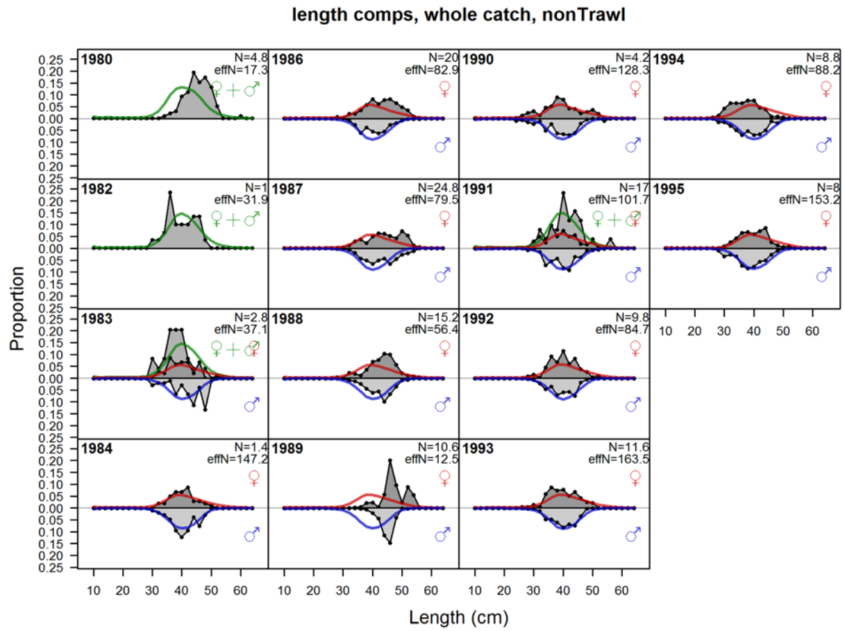
Figure 200. Fits to the Washington non-trawl length compositions by sex and year.
