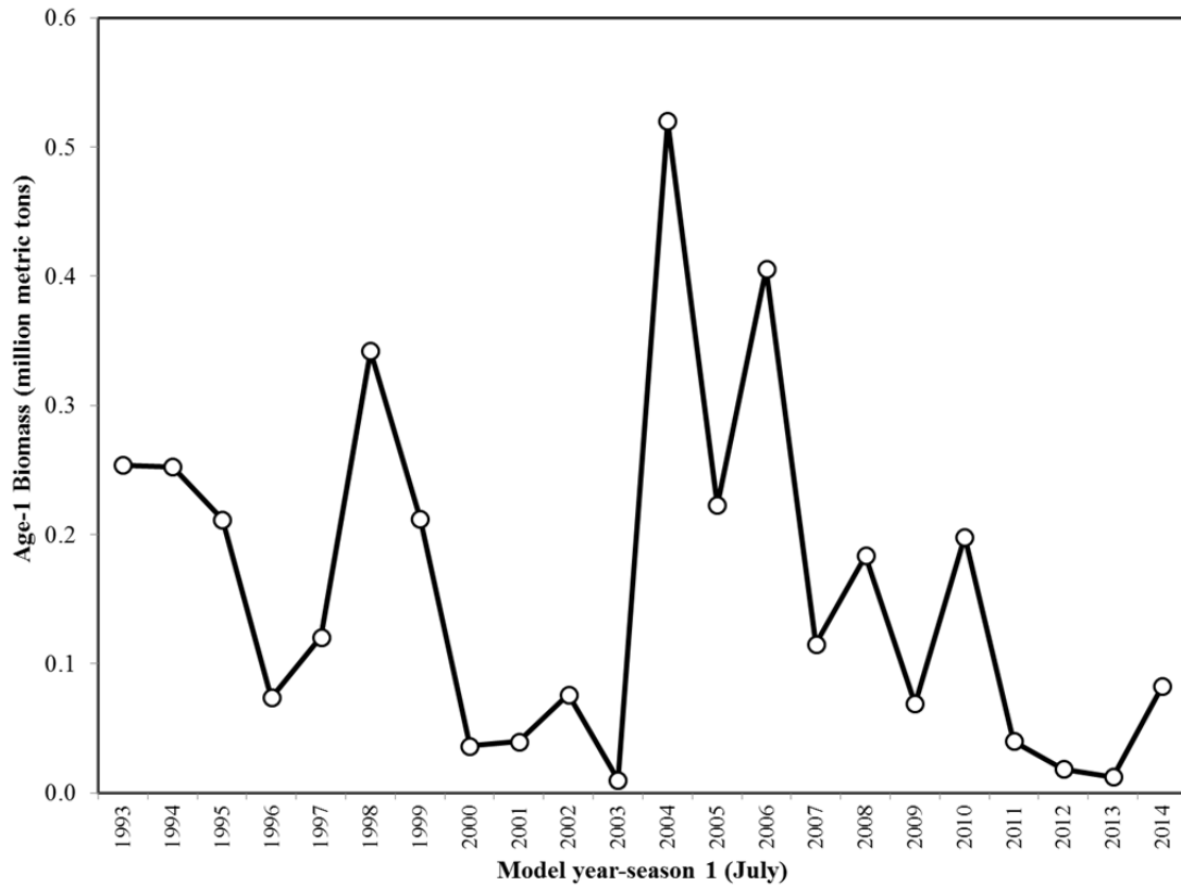
Figure 48. Biomass of age-1 sardine (base model T).
