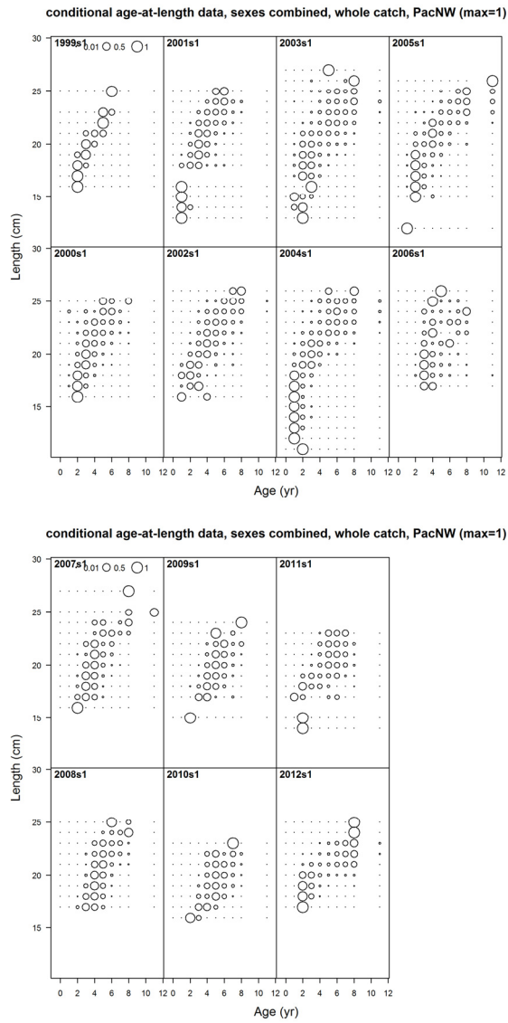
Figure 12. Conditional age-at-length data for the PacNW fleet.
