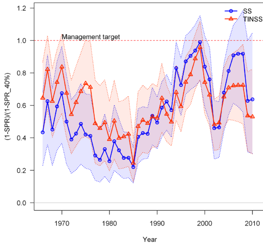
Figure e. Trend in relative spawning potential ratio through 2010 ( 1\text{-SPR}/1\text{-SPR}_{\text{Target}=0.4} ) for both models.
