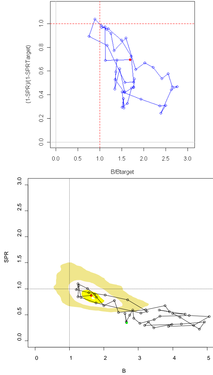
Figure f. Temporal pattern (phase plot) of relative spawning potential ratio ( 1-SPR/1-SPR_{Target=0.4} ) vs. estimated spawning biomass relative to the proxy 40% level through 2010 for the SS model (upper panel, note this calculation is based on the MLE). Lower panel shows relative spawning potential ratio ( 1-SPR/1-SPR_{MSY} ) vs. estimated spawning biomass relative to the B_{MSY} level through 2010 for the TINSS model. The filled circle denotes 2010 and the line connects years through the time-series.
