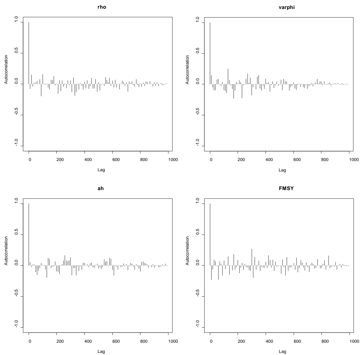
Figure 34. Autocorrelation plots for key TINSS model parameters (left to right): \rho , \phi^{-2} , \hat{a} and F_{MSY} .
