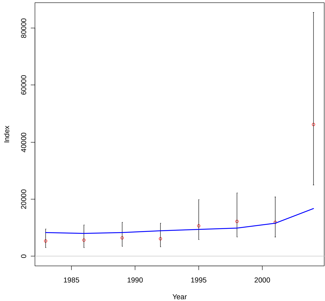
Figure 48. Observed and expected values of biomass index (mt) for the AFSC triennial survey.
