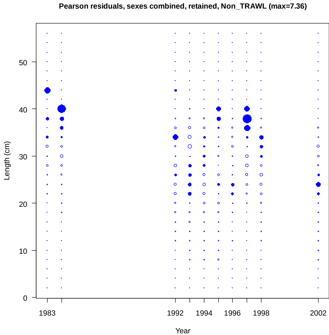
Figure 68. Pearson residuals for the fit of the length-frequency distributions (both sexes combined) for the non- trawl fishery.
