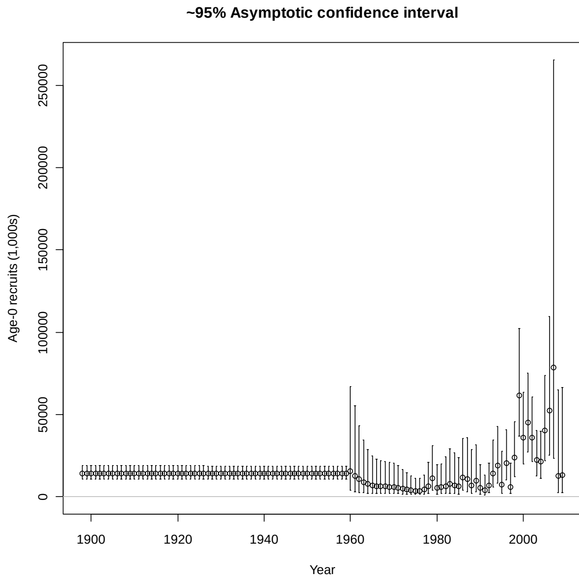
Figure 103. Time-series of the recruitment of splitnose rockfish with 95% confidence interval.
