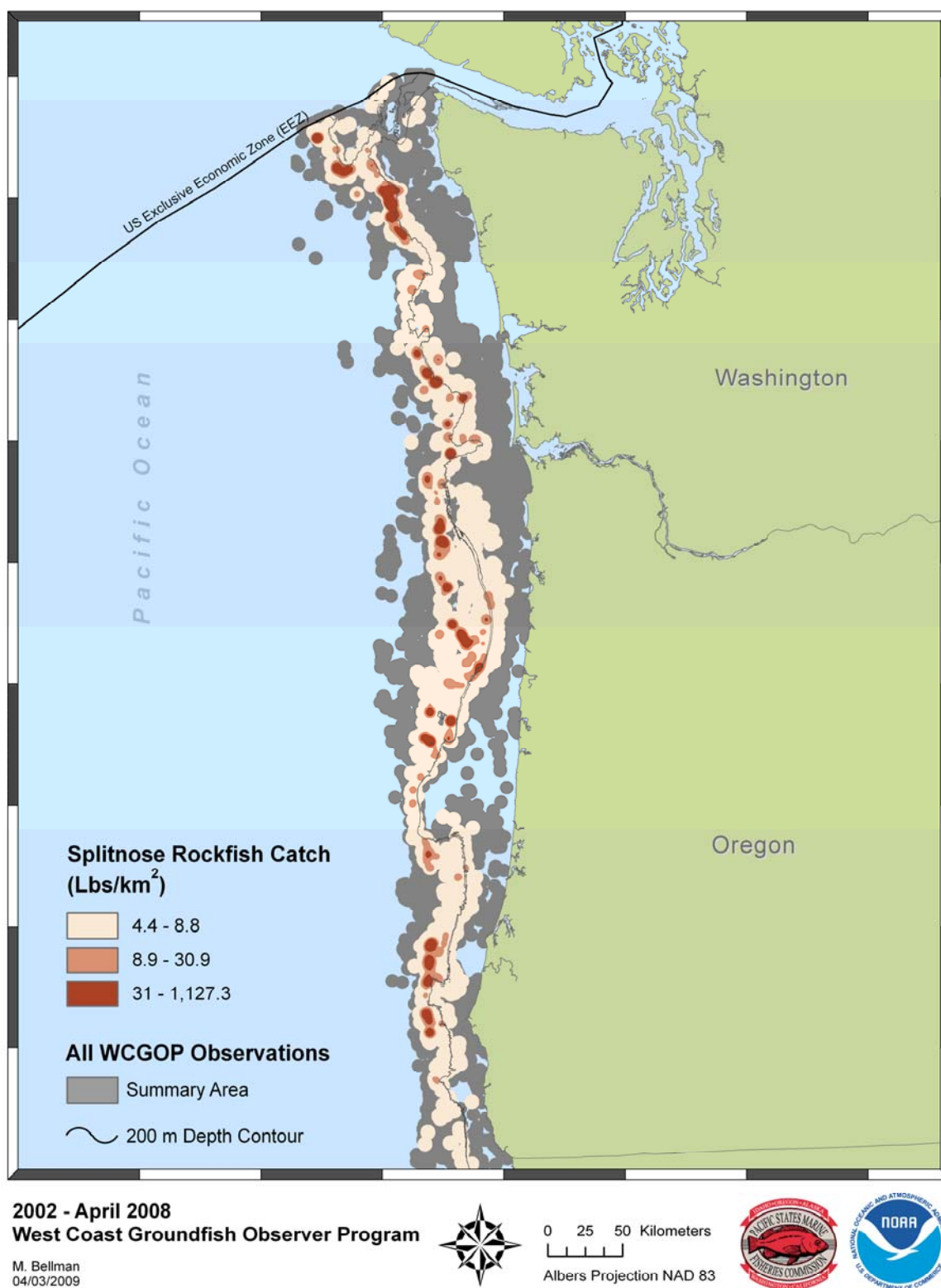
Figure 2. Spatial distribution of splitnose rockfish catch (lbs/km 2 ) observed by the West Coast Groundfish Observer Program from 2002 – April 2008 and the summary area of all observed fishing events off of Washington and Oregon.
