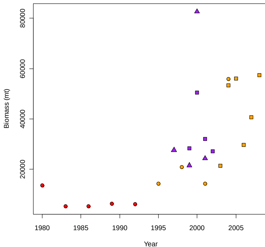
Figure 25. A composite biomass trajectory for each of the survey-based estimates of splitnose abundance. Circles represent AFSC triennial survey, triangles represent AFSC slope survey, and squares correspond to NWFSC surveys with purple (dark) squares representing NWFSC slope survey and orange (light) squares - NWFSC shelf-slope survey.
