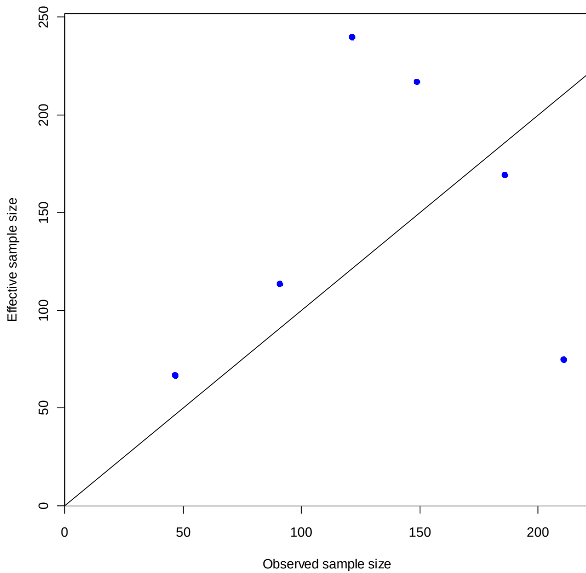
Figure 84. Observed and effective sample sizes for the sex-specific NWFSC shelf-slope survey length-frequency observations.
