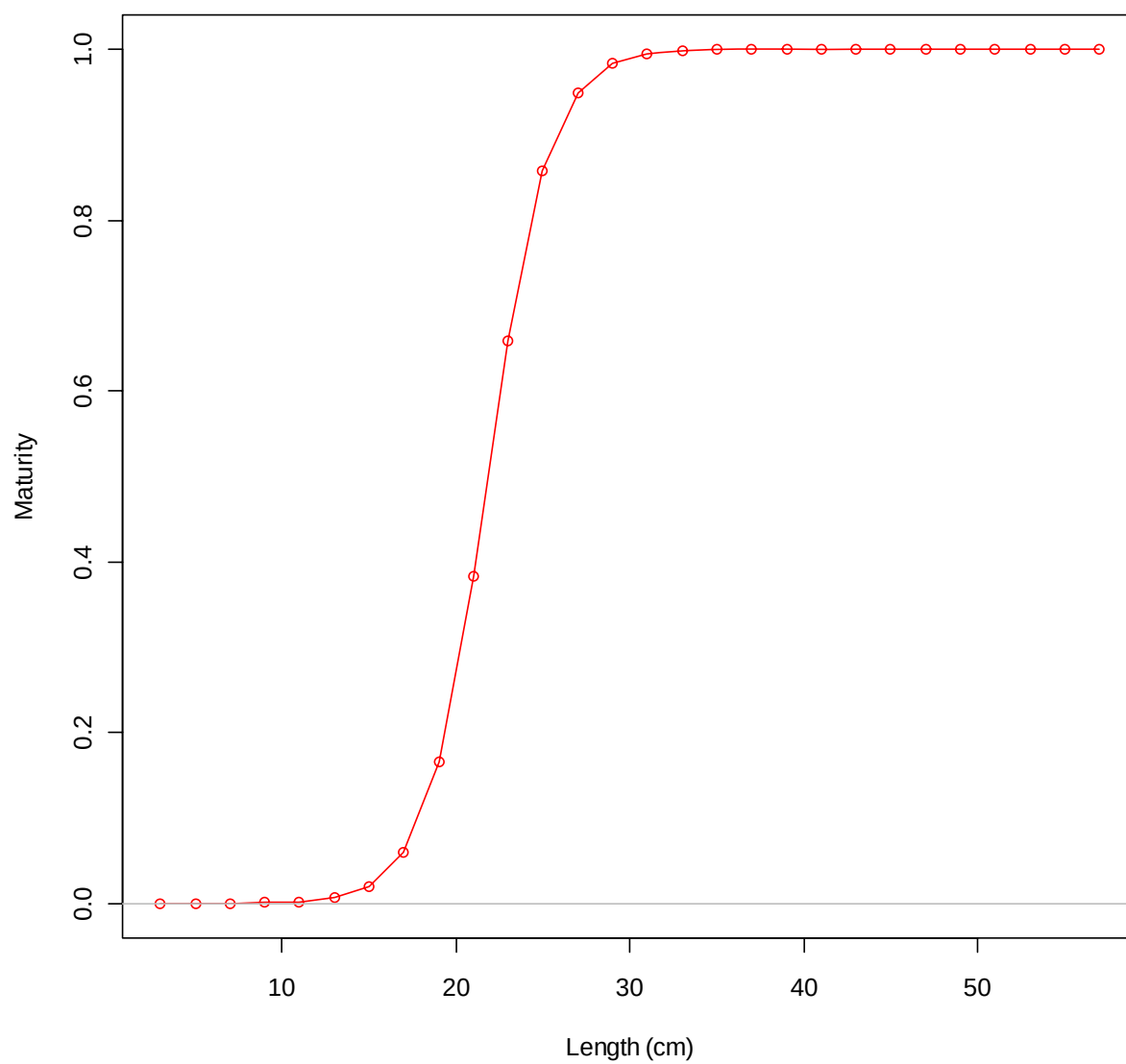
Figure 55. Female-maturity-at-length relationship used in the base model.
