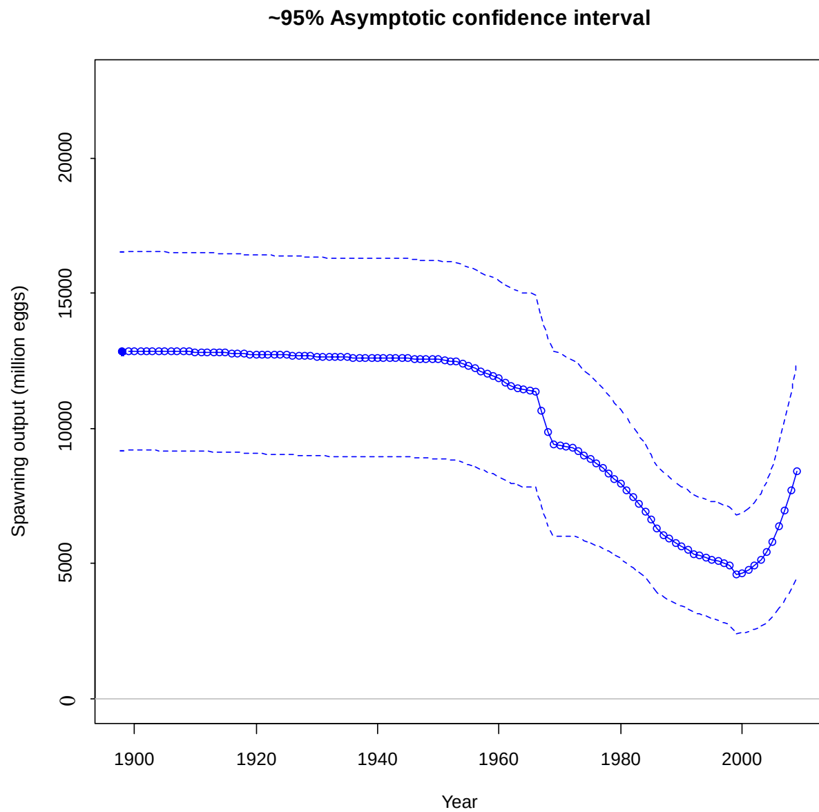
Figure 105. Time-series of the estimated spawning biomass of splitnose rockfish with 95% confidence interval.
