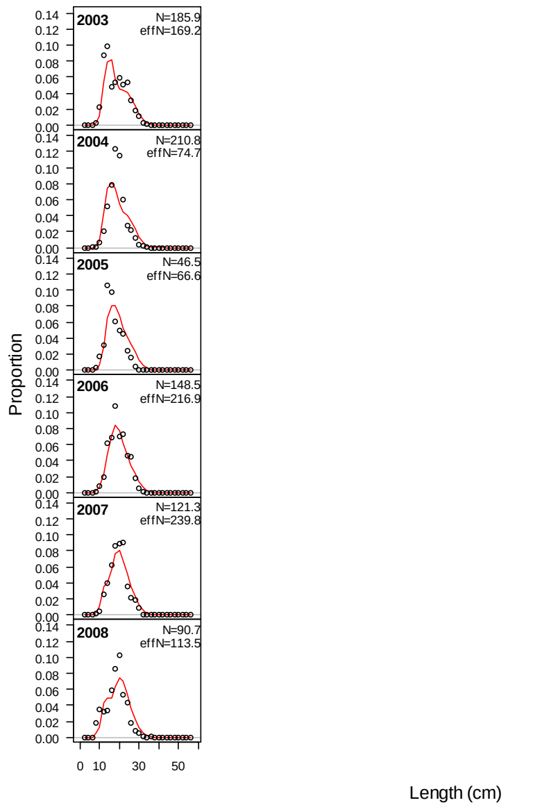
Figure 87. Fit to length-frequency distributions of the male splitnose rockfish for the NWFSC shelf-slope survey.
