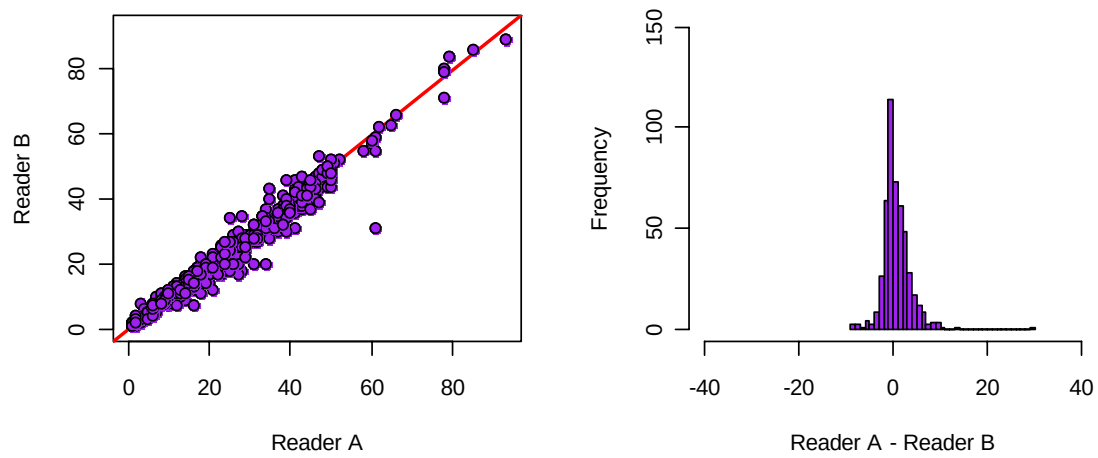
Figure 40. Comparison of age reads between Readers A and B corresponding to ageing error matrix 3. Left panel is the 1:1 plots with the red solid line indicating perfect agreement; right panel is a histogram of the age read differences between each reader.
