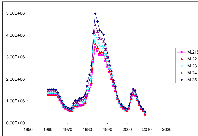
Figure 11. Predicted spawning stock biomass over a range of fixed rates of natural mortality under the proposed base model configuration.
