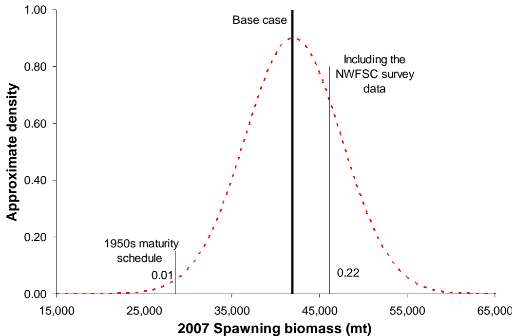
Figure i. Approximate distribution of uncertainty in estimated 2007 spawning biomass from the base case model (dashed line) density function based on the normal approximation. Bold vertical line indicates the maximum likelihood estimate from the base case, light lines the less likely alternate model including the 1950s maturity and, for comparative purposes, the alternate including NWFSC survey data.
