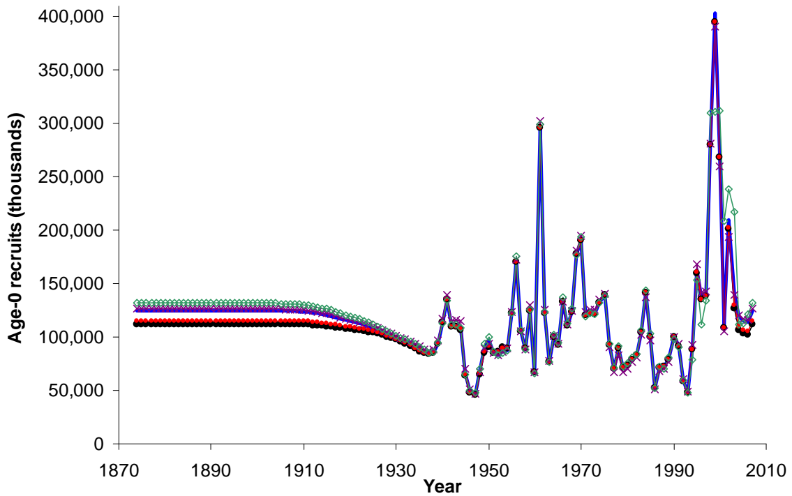
Figure 38. Comparison of the base case model results with the four alternate sensitivity models.
