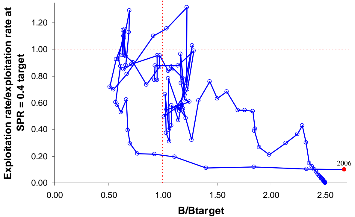
Figure 46. Relative exploitation rate/exploitation rate at SPR = 0.4 target vs. estimated spawning biomass relative to the proxy 40% level.
