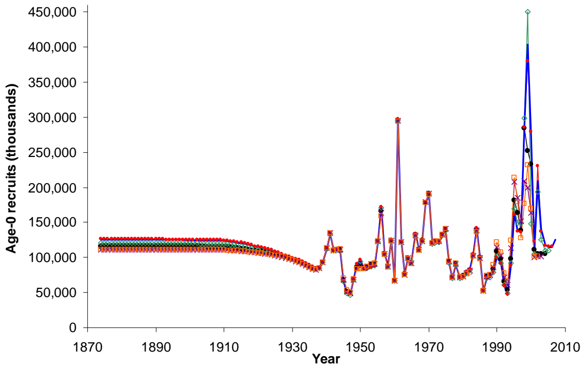
Figure 40. Results from a 5-year retrospective analysis. Each year of retrospective is performed as if the assessment were conducted in that year (i.e., retrospective in 2006 includes data through 2005).
