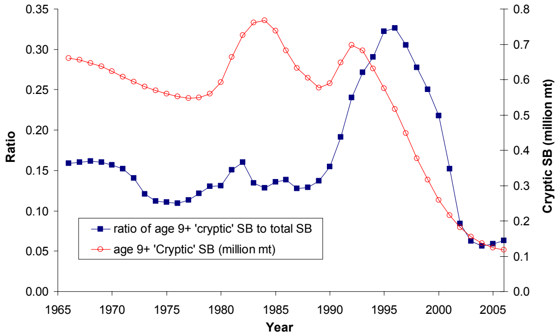
Figure 4. Age 9+ cryptic spawning biomass (SB) and proportion of total SB that is cryptic (i.e. not sampled by the acoustic survey or any of the U.S. or Canadian hake fisheries) from Model 2, 1966-2005.
