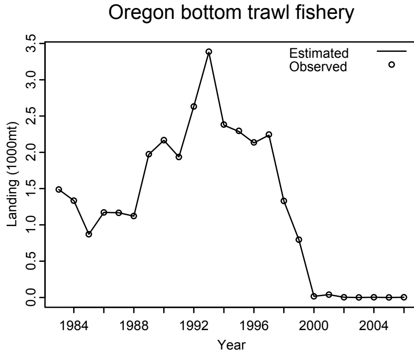
Figure 20. Model fits to the Oregon bottom trawl and Eureka-Conception fisheries landings data.
