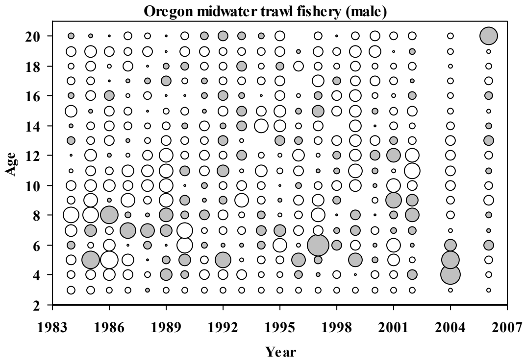
Figure 27b. Age composition residuals for the Oregon midwater trawl fishery from the base model. Residuals are standardized differences (observed – estimated). Dark circles are positive residuals and open circles are negative residuals.
