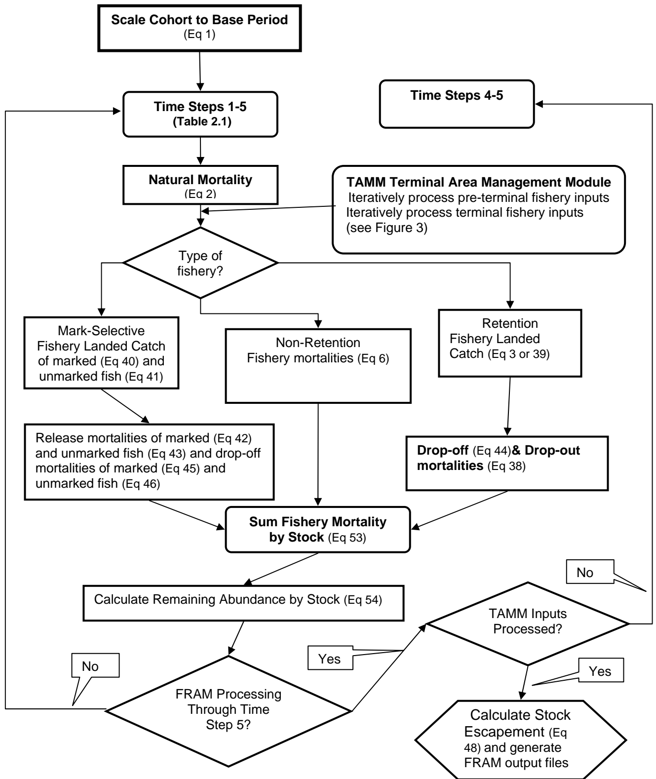
Figure 1. Flow chart for FRAM coho model
