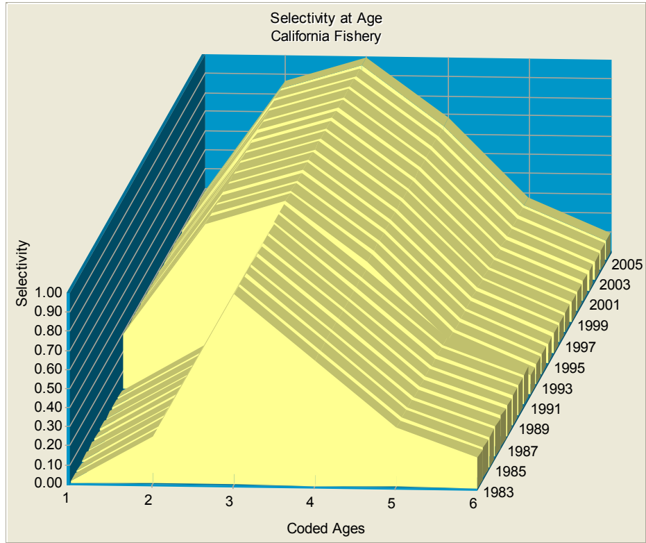
Figure 13. Estimated selectivity for the California fishery (Fishery 1) from the ASAP baseline model. Selectivity was estimated for two periods: 1983-92 and 1993-2005.
