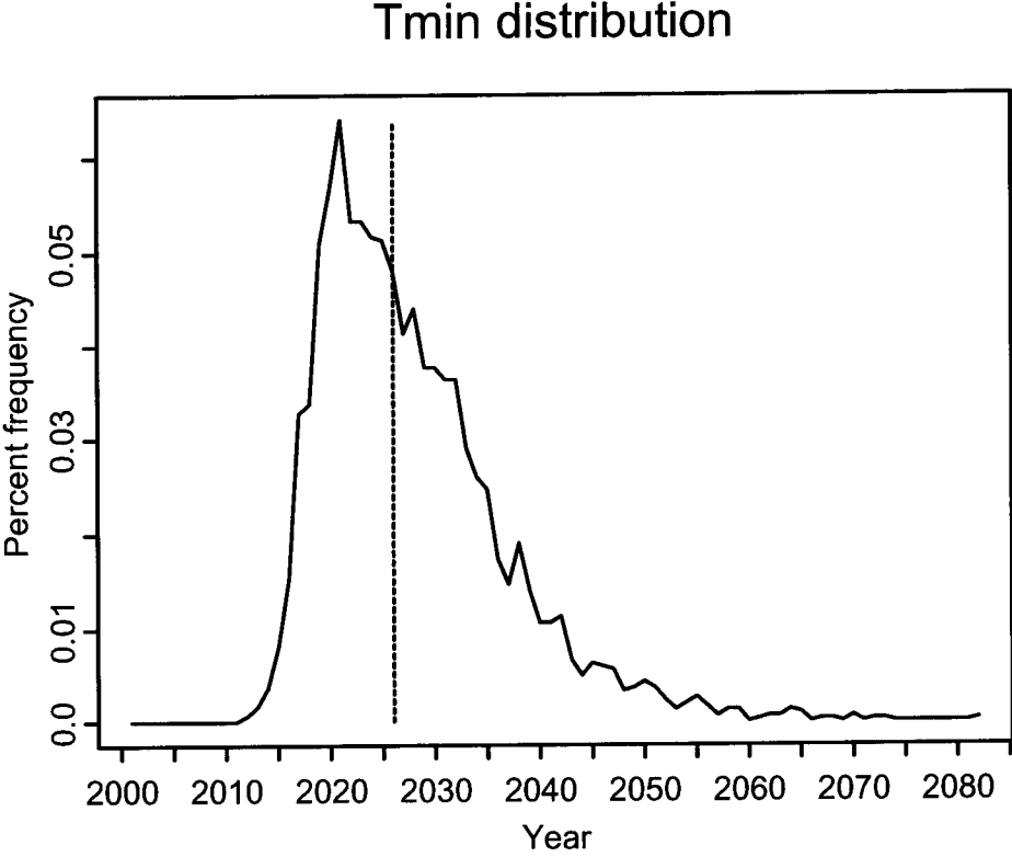
Figure 4. Simulated frequency distribution of the time to recover to 0.4 B_0 from 2001 with fishing ( T_{min} ), computed from 3,000 simulations based on the specifications of the Model 8. The vertical line represents the value of T_{min} used in the rebuilding analyses.
