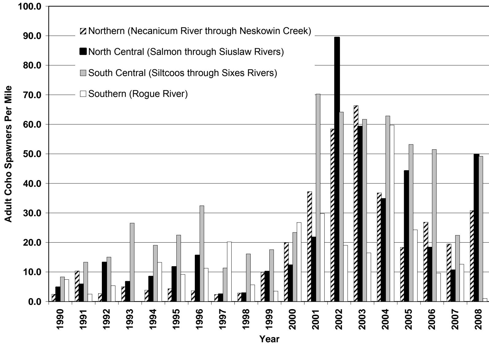
Figure III-2. Oregon coastal natural (OCN) adult coho spawners per habitat mile by coastal region based on SRS accounting methods, 1990-2008.
