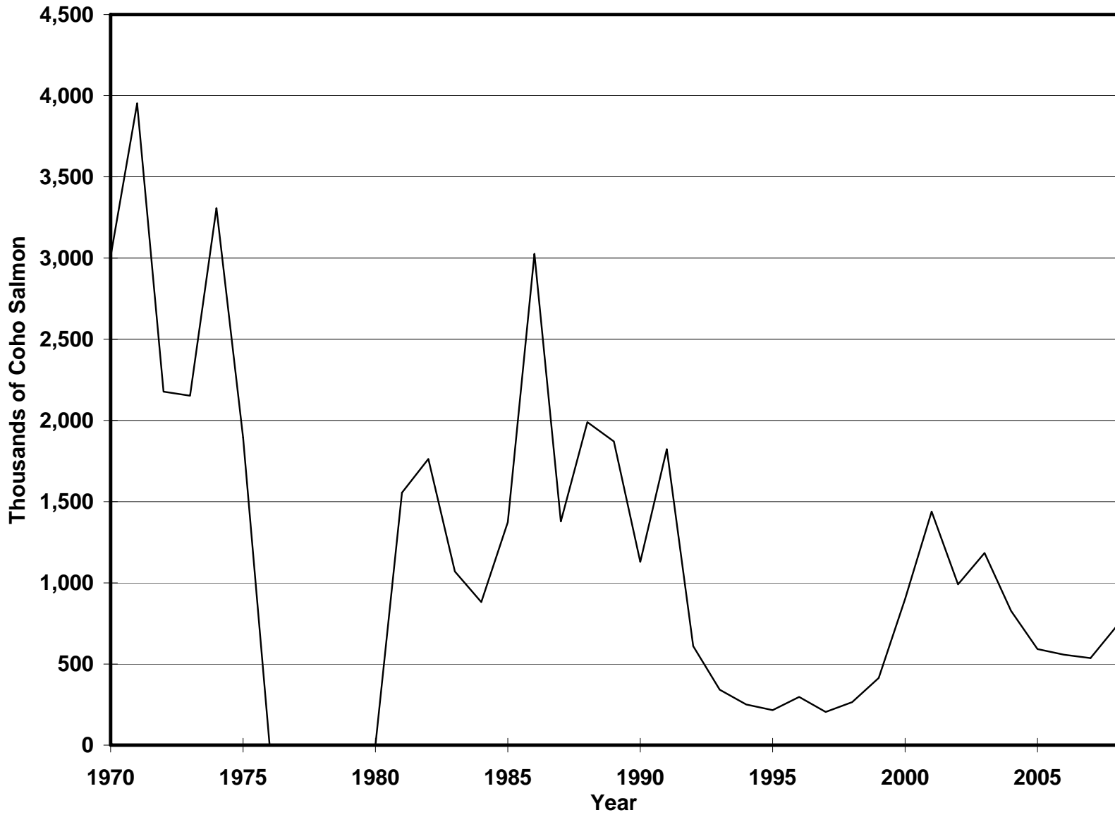
Figure III-1. Oregon Production Index (OPI) area coho abundance estimates by stratified random surveys (SRS) accounting methods (1970-2008).
